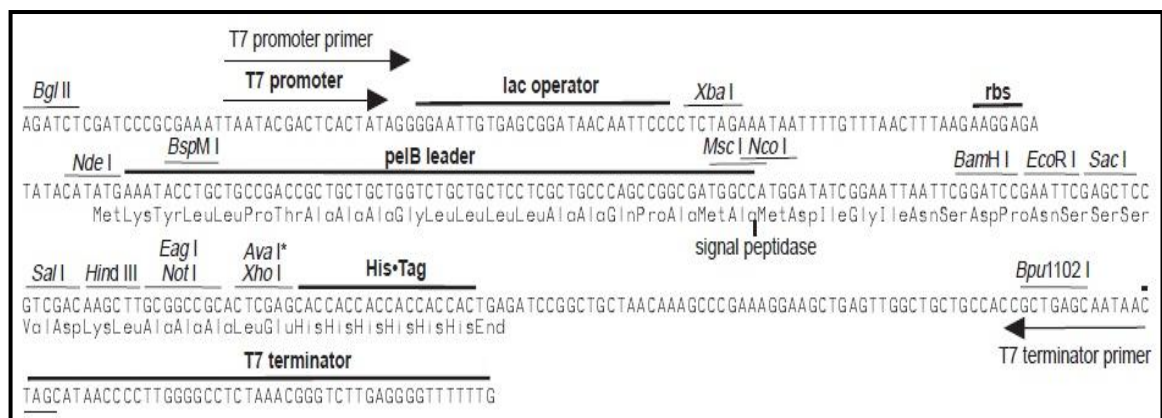
Figure 2.10. Expression region of pET-26b(+) vector.
