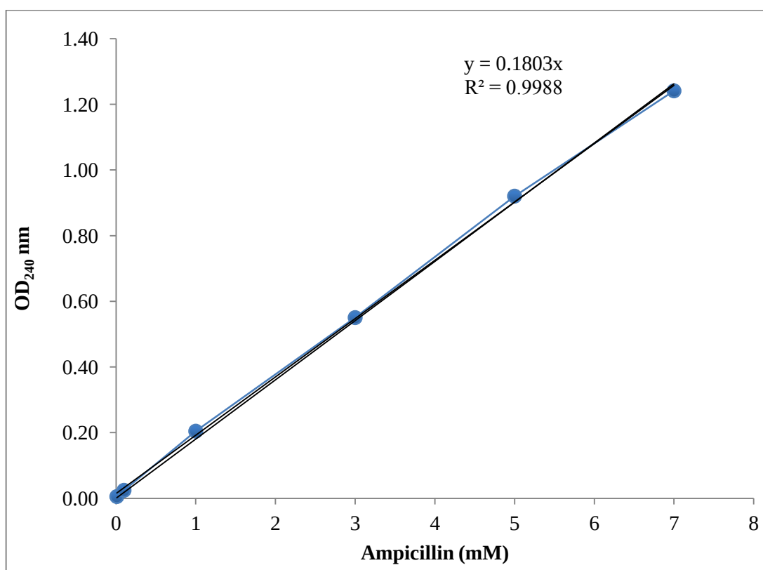
Figure B.1. Ampicillin calibration curve.
