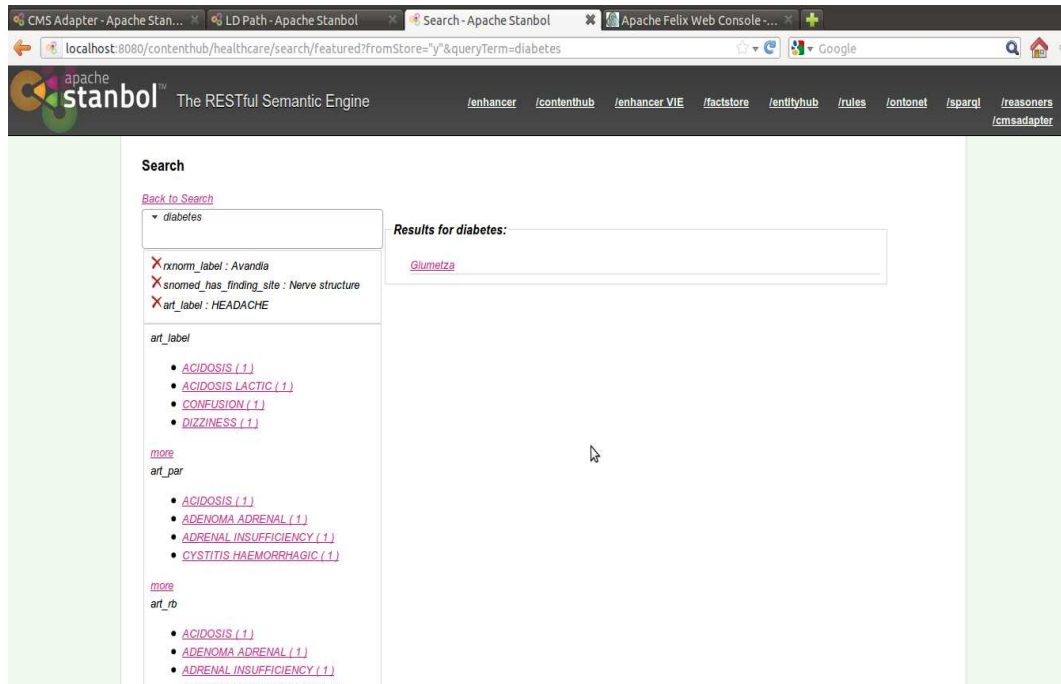
Figure 5.8: Constrained search results after selecting headache constraint
