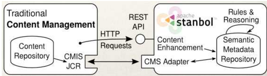
Figure 2.3: CMS - Stanbol interaction
