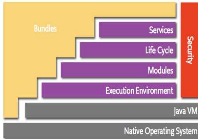
Figure 2.2: Layered OSGi architecture [18]
