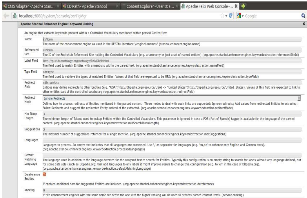
Figure 5.1: Configuring a Keyword Linking Engine for RxNORM Dataset
