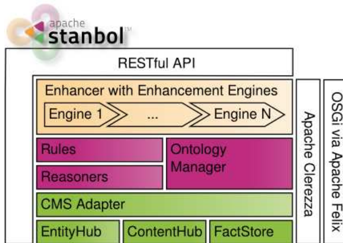
Figure 2.1: Stanbol components [15]
