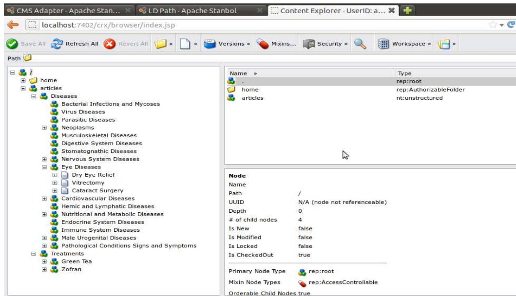
Figure 5.3: CMS Structure
