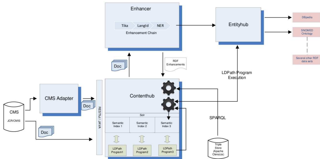
Figure 4.2: Semantic content management with Stanbol framework
