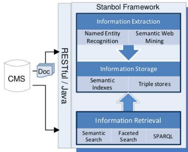
Figure 2.4: Semantic content management overview
