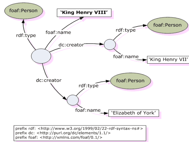
Figure 3.2: Representing persons with RDF [47]
