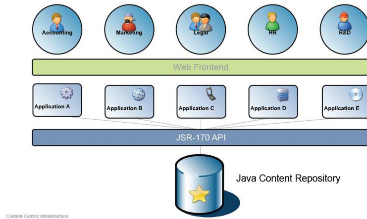
Figure 4.1: Standards-based content repository [90]
