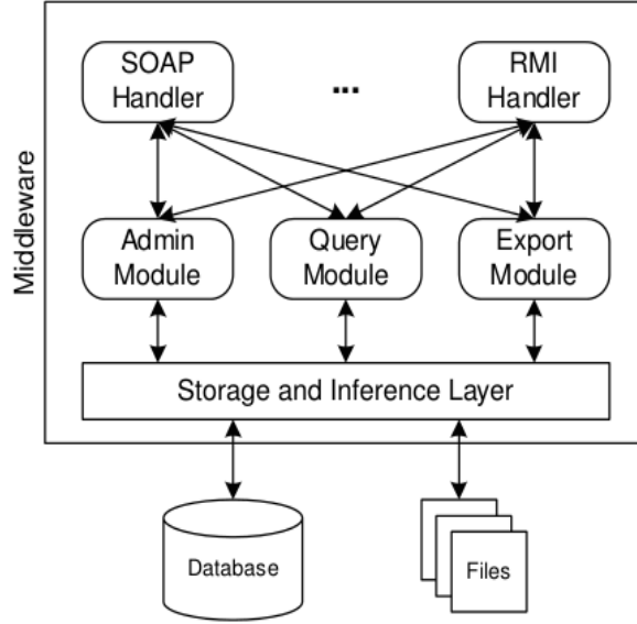
Figure 3.3: Generic Architecture of an RDF Store(Sesame) [64]
