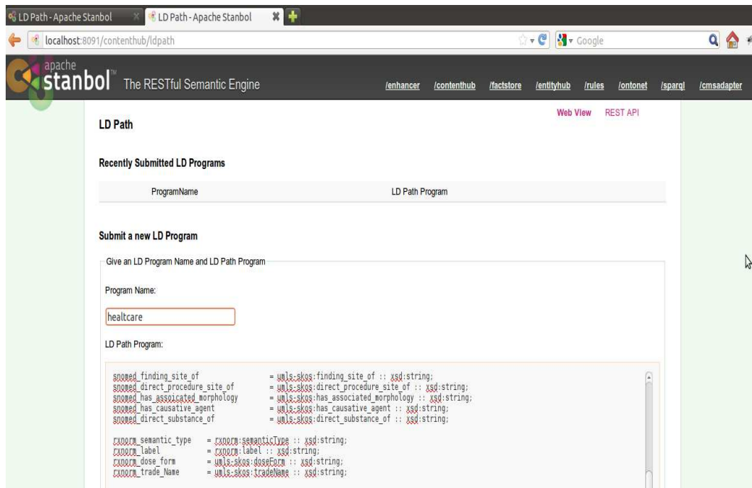
Figure 5.2: Submitting an LDPath program
