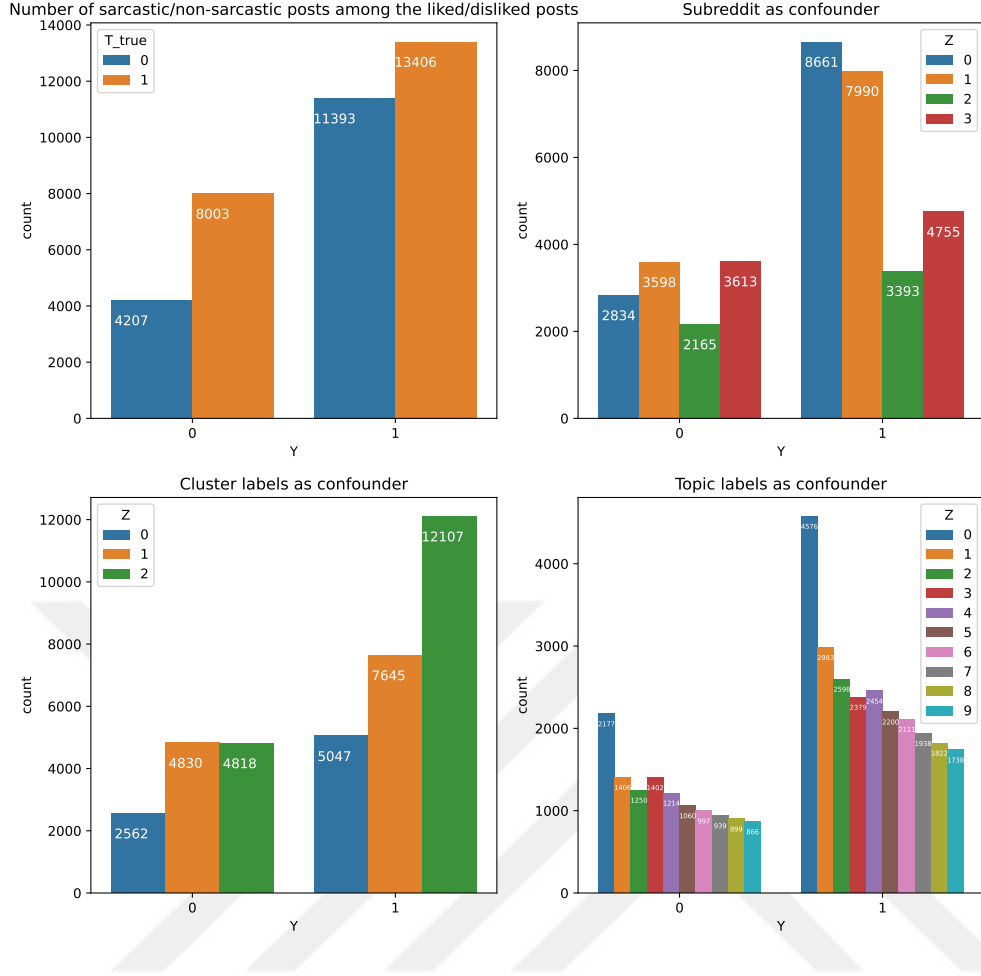
Figure 6.2: Number of Reddit posts for each confounder settings
