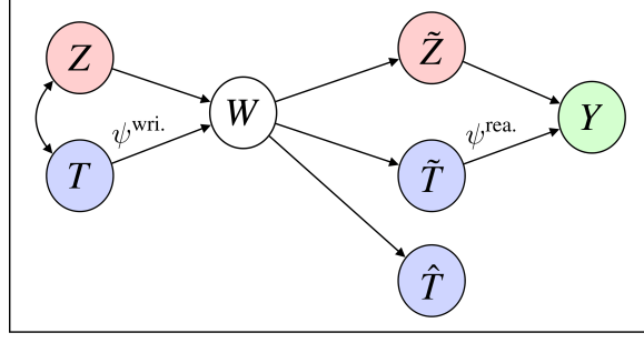
Figure 6.1: The structural causal model in Pryzant et al. [1]
