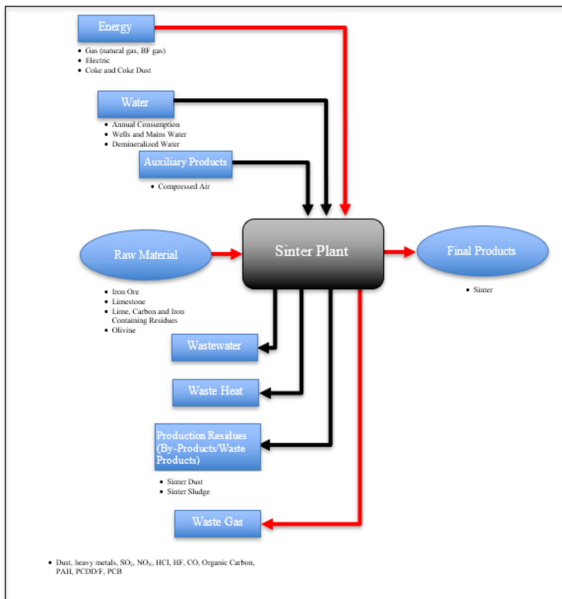
Figure 5. Sinter Plant Key Inputs and Outputs
