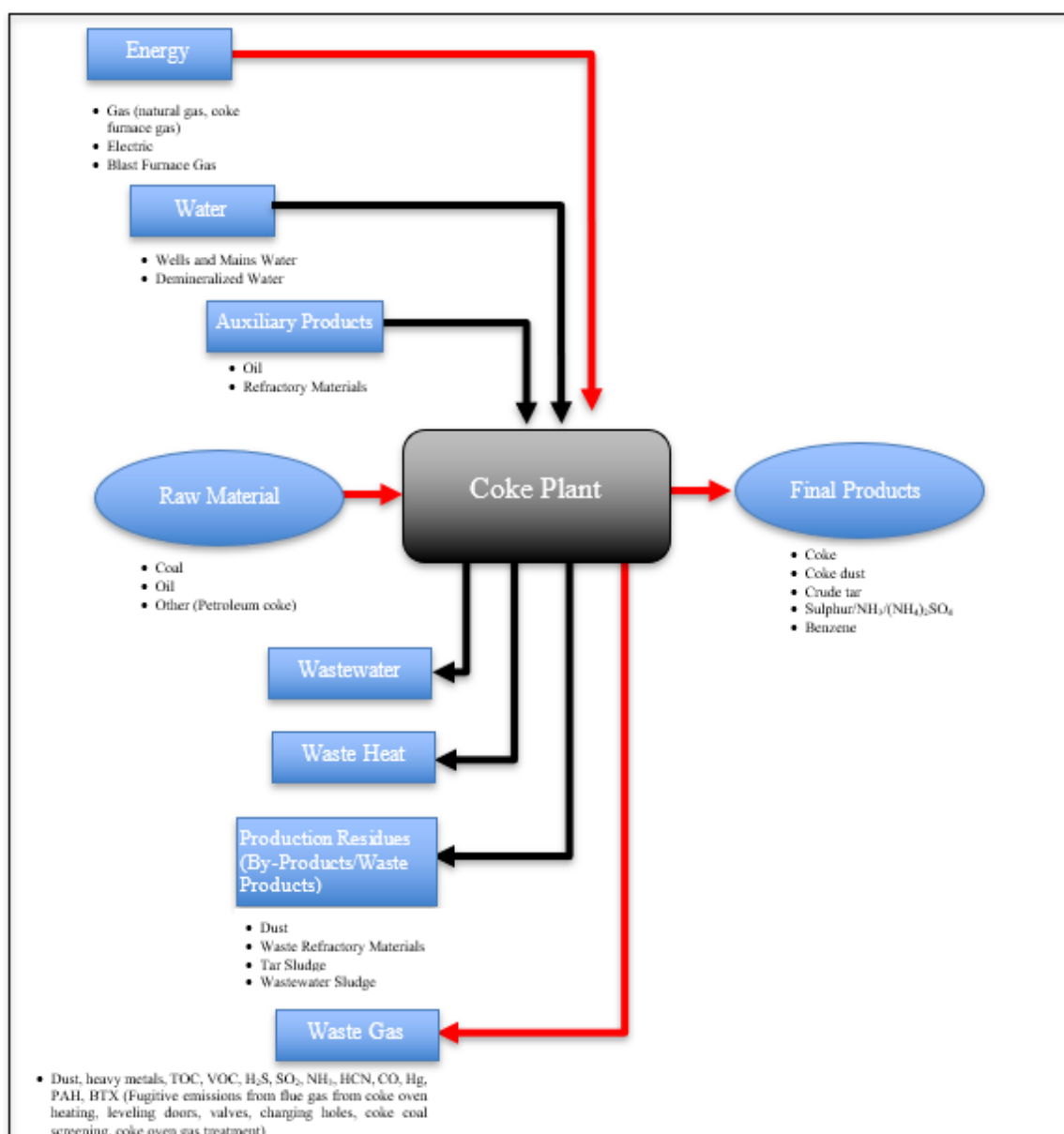
Figure 4. Coke Plant Key Inputs and Outputs
