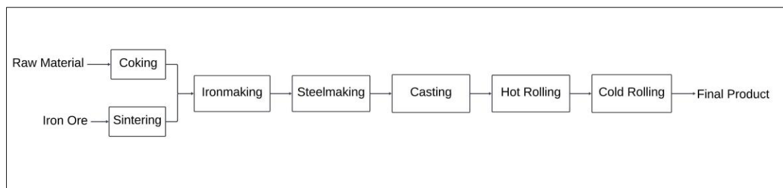
Figure 3. Flow Chart of Integrated Plants
