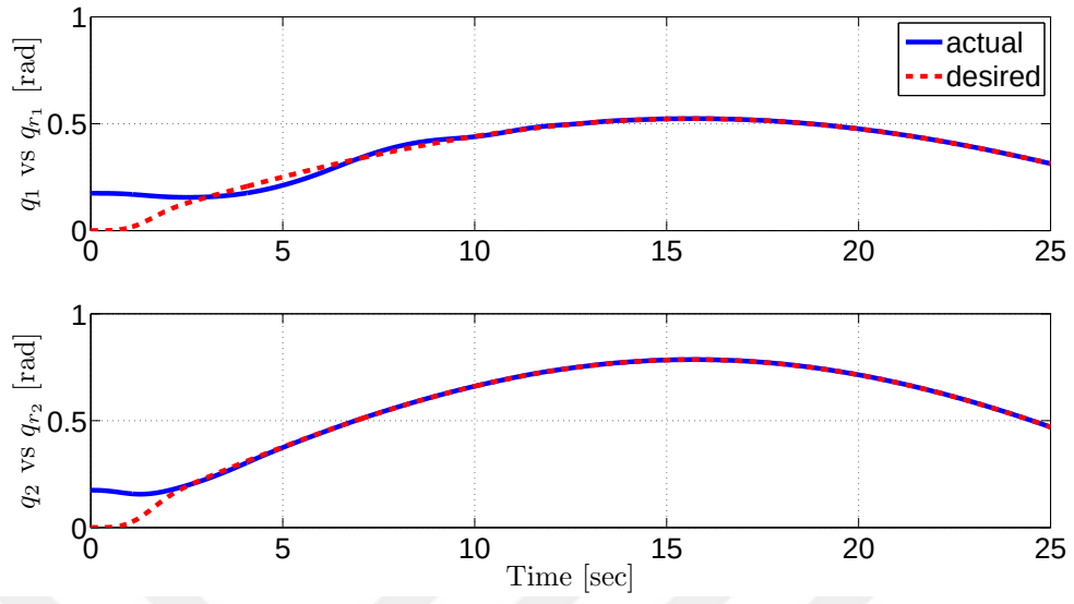
Figure 5.1. Positions for \omega_r = 0.1 rad/sec and for \beta_2 = k_c = 10^{-6}I_2
