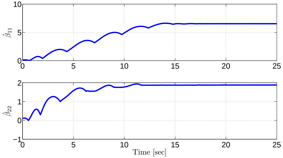
Figure 5.14. Entries of the time-varying gain matrix \hat{\beta}(t) for \omega_r = 1 rad/sec and for \beta_2 = k_c = 0.1I_2
