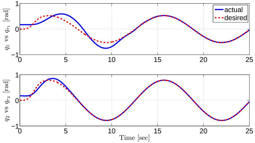
Figure 5.6. Positions for \omega_r = 0.5 rad/sec and for \beta_2 = k_c = 10^{-3}I_2
