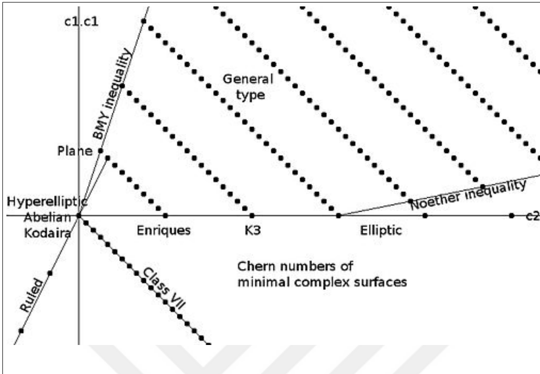
Figure 2.1: Enriques–Kodaira classification of compact complex surfaces, Wikipedia
