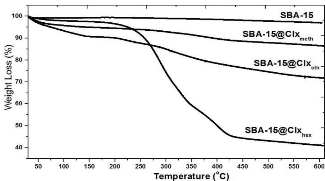
Figure 28 % Weight loss of SBA-15, SBA-15@Clx eth , SBA-15@Clx meth , and SBA-15@Clx hex .
