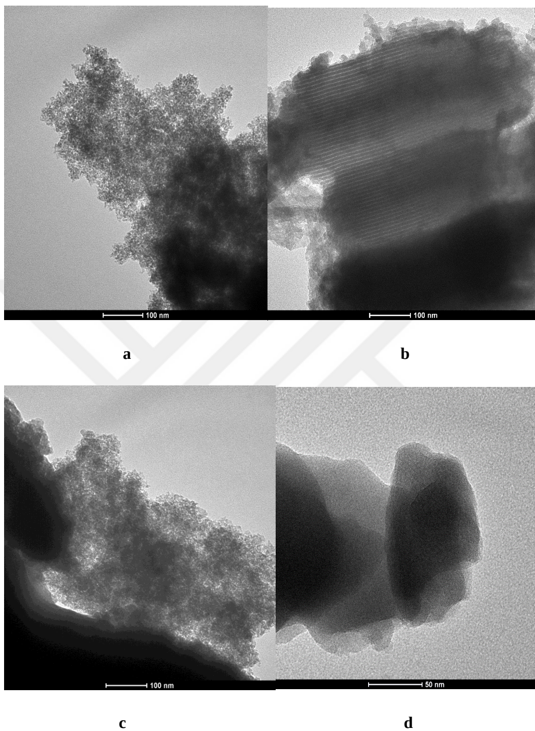
Figure 33 TEM images of a) SBA-15-B (100 nm), b) SBA-15-B@Cl x eth (100 nm), c) SBA-15-B@Cl x meth (100 nm), d) SBA-15-B@Cl x hex (50 nm).
