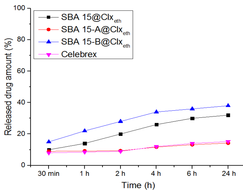
Figure 45 Amount of Celecoxib released from 1.0 g of Celebrex loaded to SBA-15, SBA-15-A and SBA-15-B in ethanol in 24 hours at pH=5.0.
