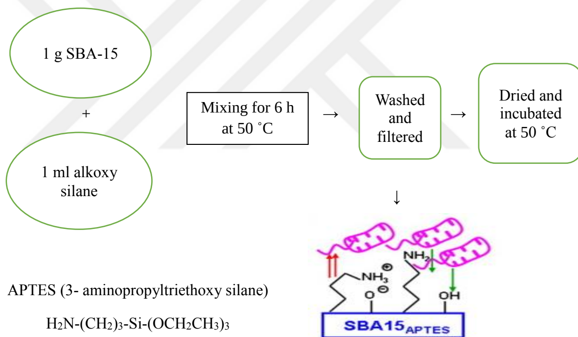
Figure 9 Schematic representation of synthesis of SBA-15-A.
