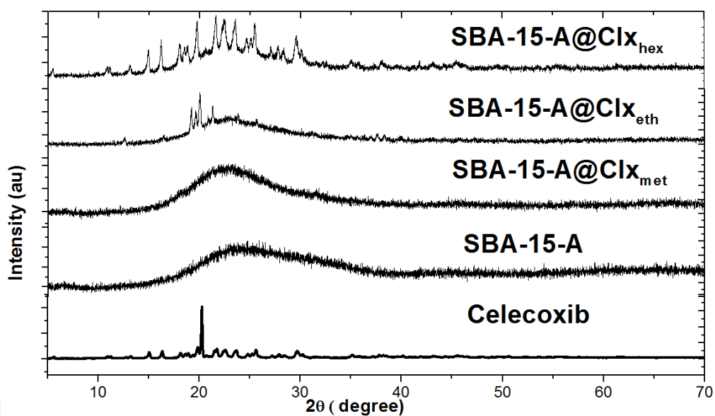
Figure 12 Wide angle powder XRD pattern of SBA-15-A, SBA-15-A@Clx eth , SBA-15-A@Clx meth , SBA-15-A@Clx hex and Celecoxib.
