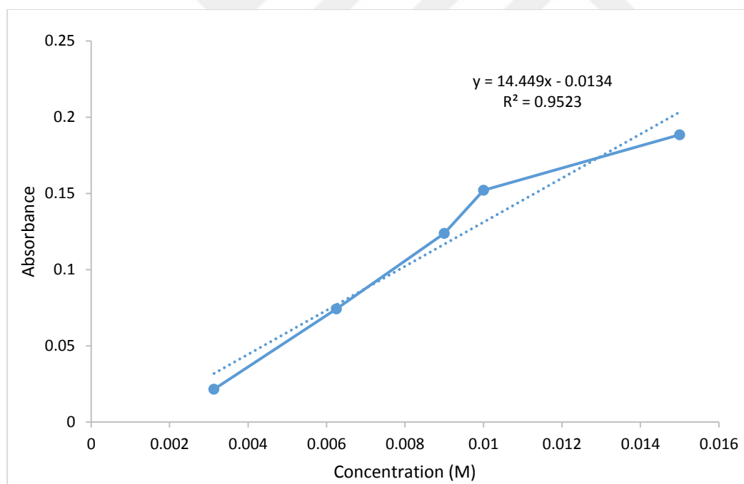
Figure 39 Calibration curve of loading process of Celecoxib in hexane.
