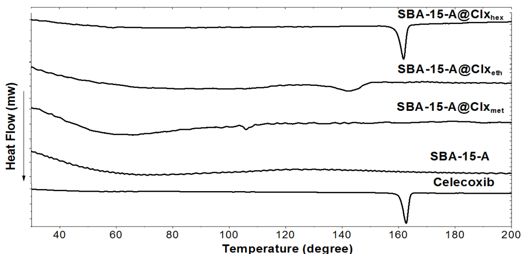
Figure 26 DSC thermograms of SBA-15-A, SBA-15-A@Clx eth , SBA-15-A@Clx met , and SBA-15-A@Clx hex .
