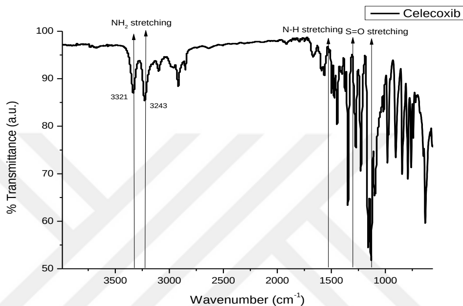
Figure 15 The chemical groups of Celecoxib in FT-IR spectra.
