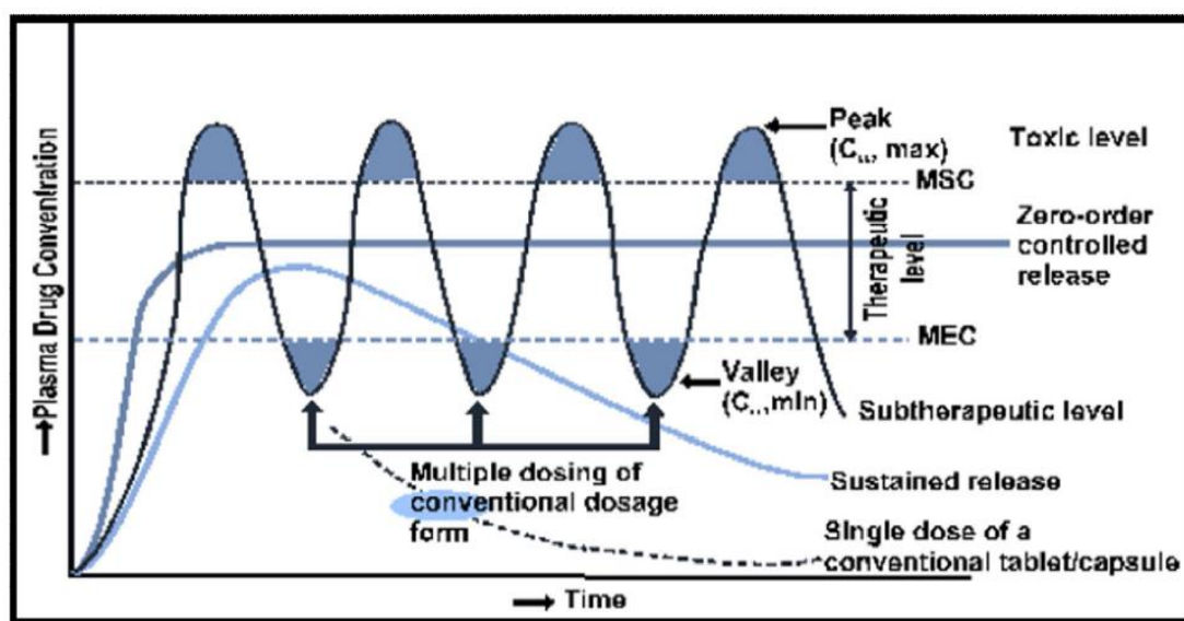
Figure 5 A hypothetical plasma concentration-time profile from conventional multiple dosing and single doses of sustained and controlled delivery formulations [28].
