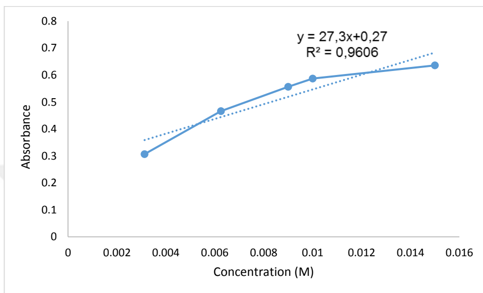
Figure 40 Calibration curve of release process of Celecoxib in PBS at pH=7.4.
