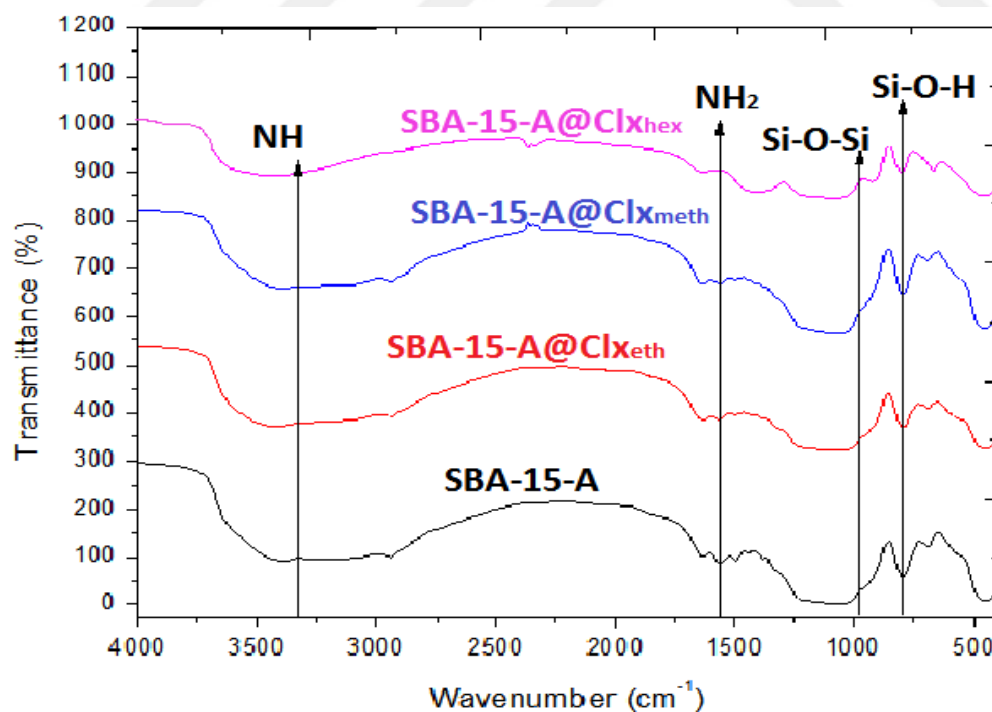
Figure 17 FT-IR spectra of SBA-15-A, SBA-15-A@Cl x eth, SBA-15-A@Cl x meth, and SBA-15-A@Cl x hex.
