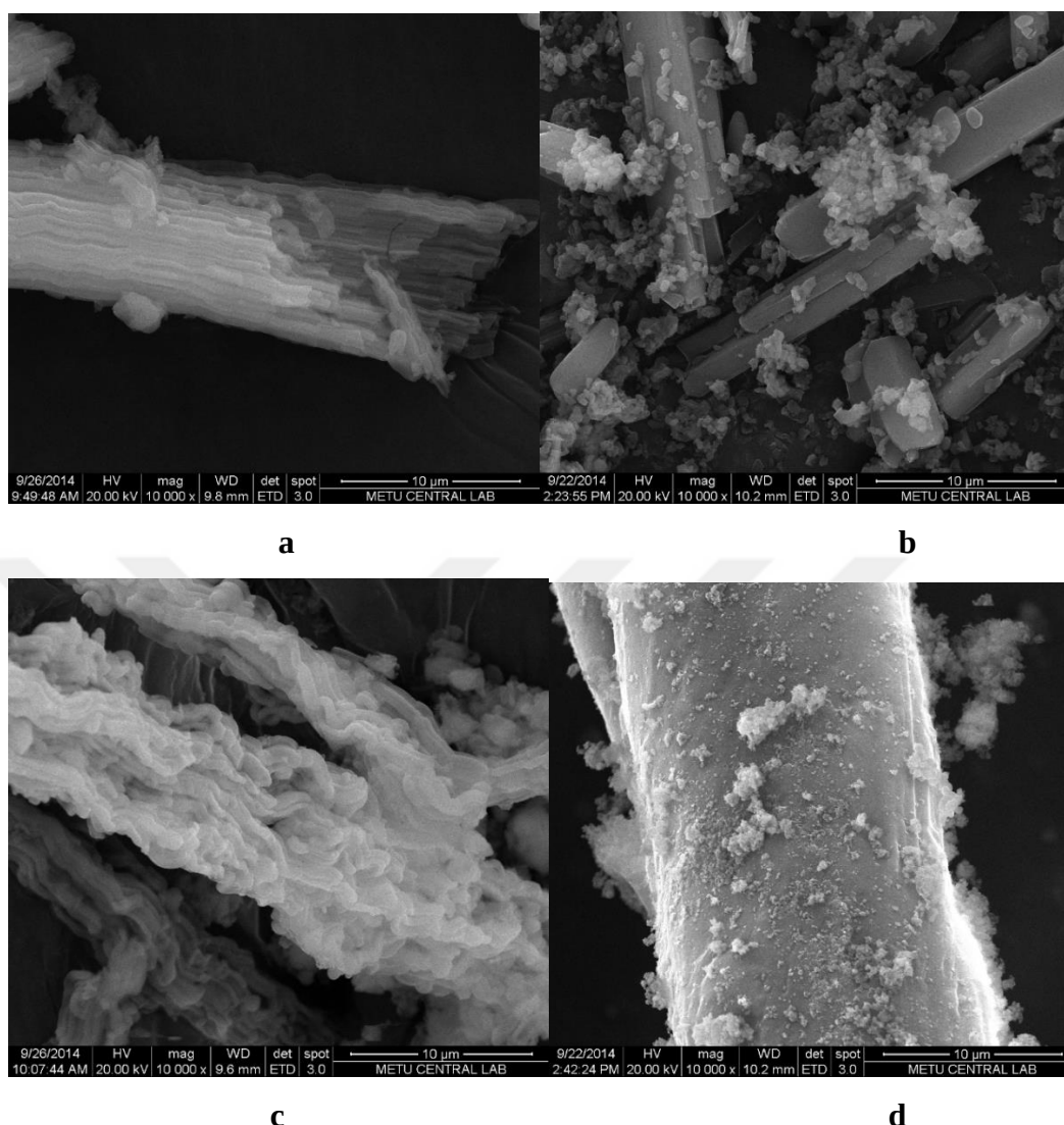
Figure 35 SEM images of a) SBA-15-A, b) SBA-15-A@Clx eth , c) SBA-15-A@Clx meth , d) SBA-15-A@Clx hex .
