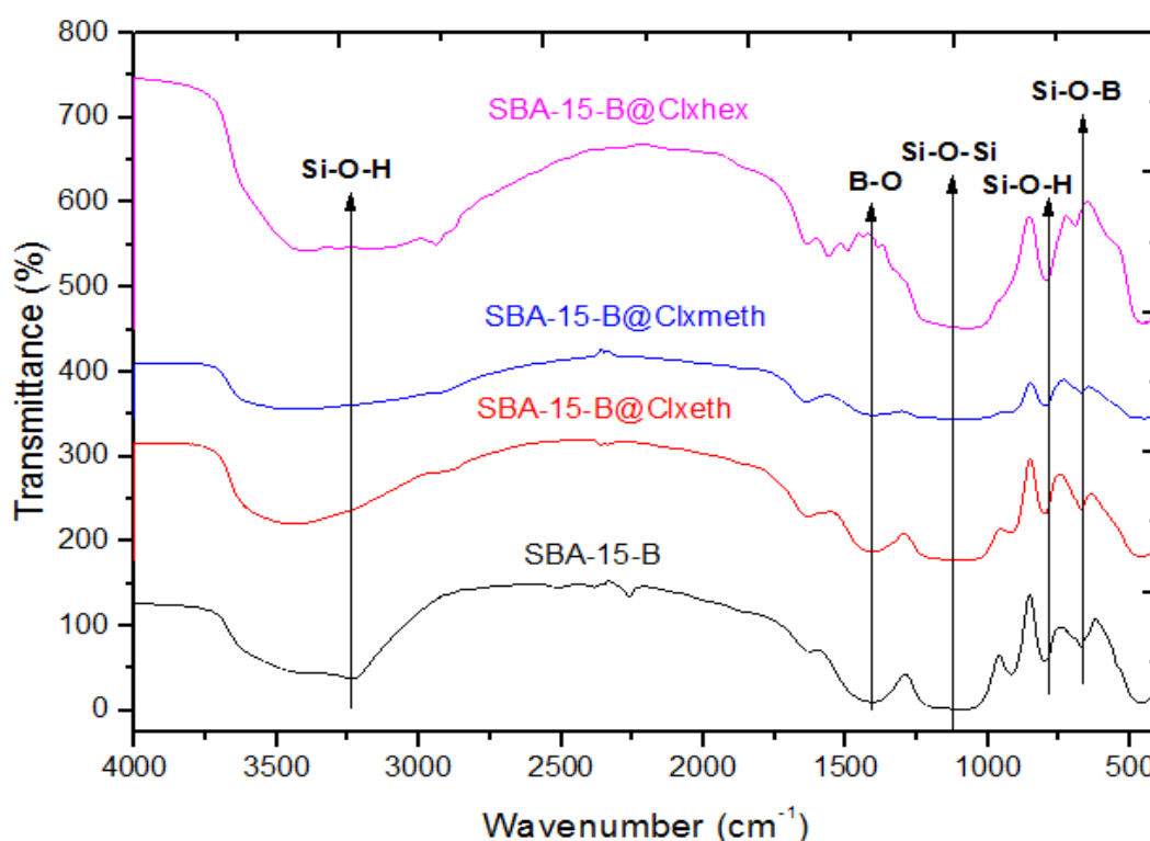
Figure 18 FT-IR spectra of SBA-15-B, SBA-15-B@Clx eth , SBA-15-B@Clx meth , and SBA-15-B@Clx hex .
