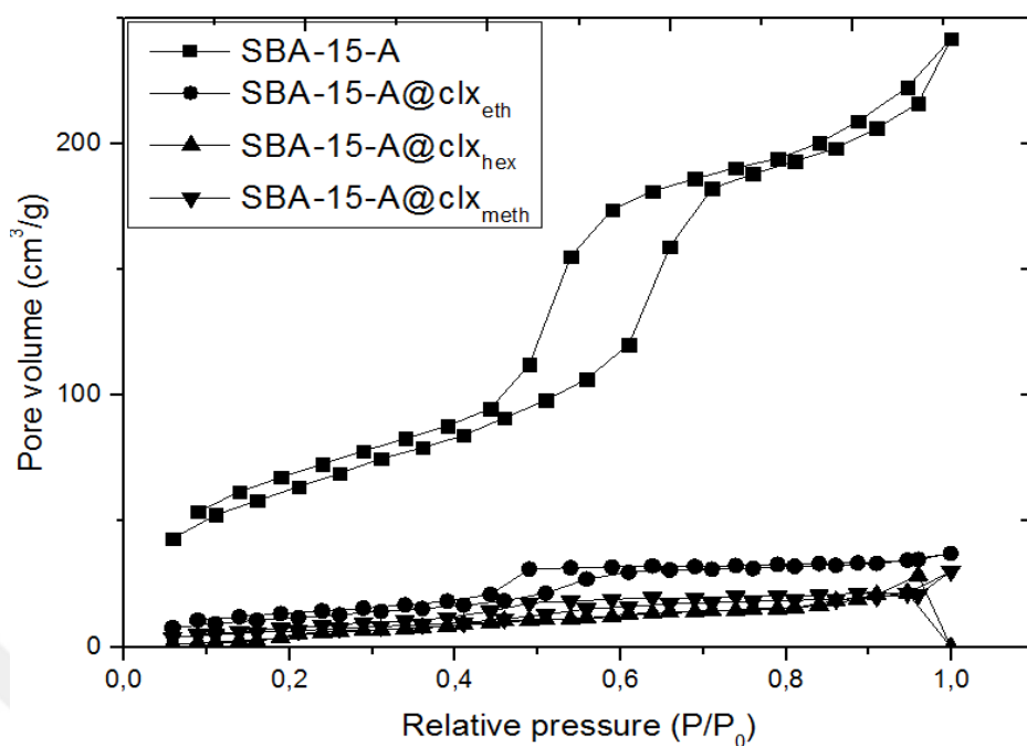
Figure 20 BET isotherms of SBA-15-A, SBA-15-A@Cl x eth , SBA-15-A@Cl x meth , and SBA-15-A@Cl x hex .
