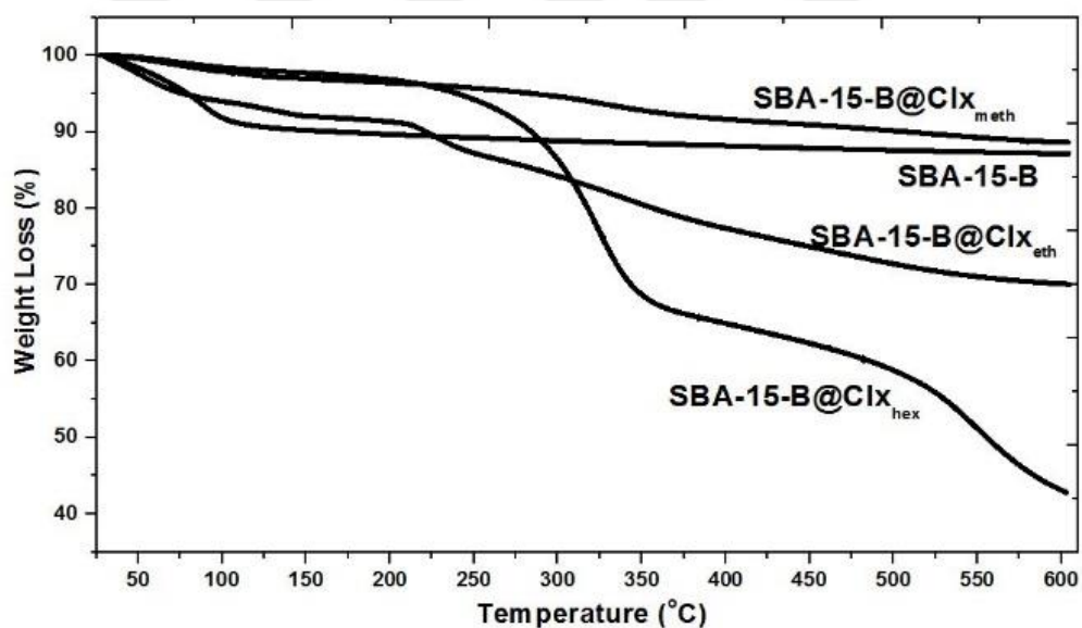
Figure 30 % Weight loss of SBA-15-B, SBA-15-B@Cl x eth , SBA-15-B@Cl x meth , and SBA-15-B@Cl x hex .
