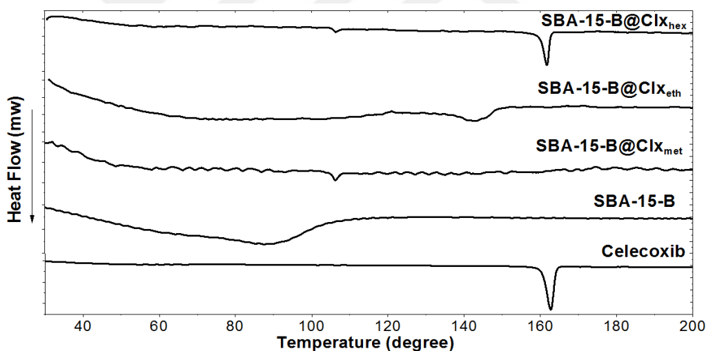
Figure 27 DSC thermograms of SBA-15-B, SBA-15-B@Clx eth , SBA-15-B@Clx met , and SBA-15-B@Clx hex .
