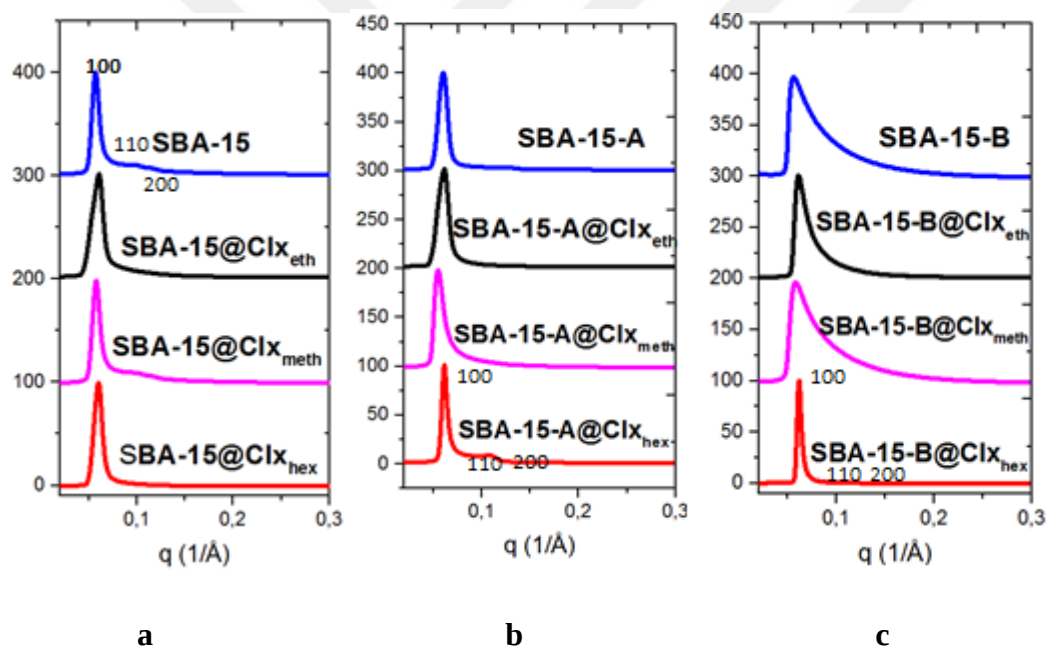
Figure 14 Small angle powder XRD patterns of a) SBA-15, SBA-15@Clx eth , SBA-15@Clx meth , SBA-15@Clx hex ; b) SBA-15-A, SBA-15-A@Clx eth , SBA-15-A@Clx meth , SBA-15-A@Clx hex ; c) SBA-15-B, SBA-15-B@Clx eth , SBA-15-B@Clx meth , SBA-15-B@Clx hex .
