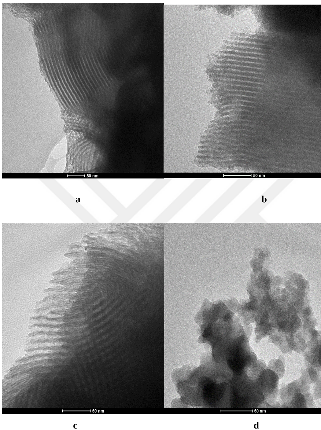
Figure 32 TEM images of a) SBA-15-A (50 nm), b) SBA-15-A@Cl x eth (50 nm), c) SBA-15-A@Cl x meth (50 nm), d) SBA-15-A@Cl x hex (50 nm).
