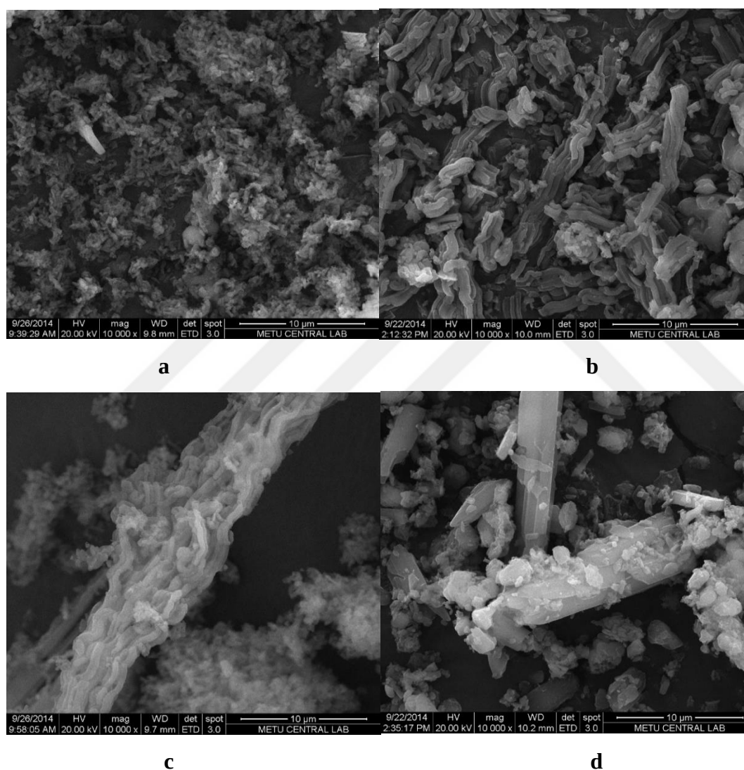
Figure 34 SEM images of a) SBA-15, b) SBA-15@Clx eth , c) SBA-15@Clx meth , d) SBA-15@Clx hex .
