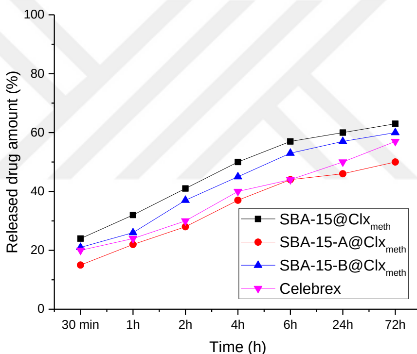
Figure 43 Amount of Celecoxib released from 1.0 g of Celebrex loaded to SBA-15, SBA-15-A and SBA-15-B in methanol in 72 hours at pH=7.4.
