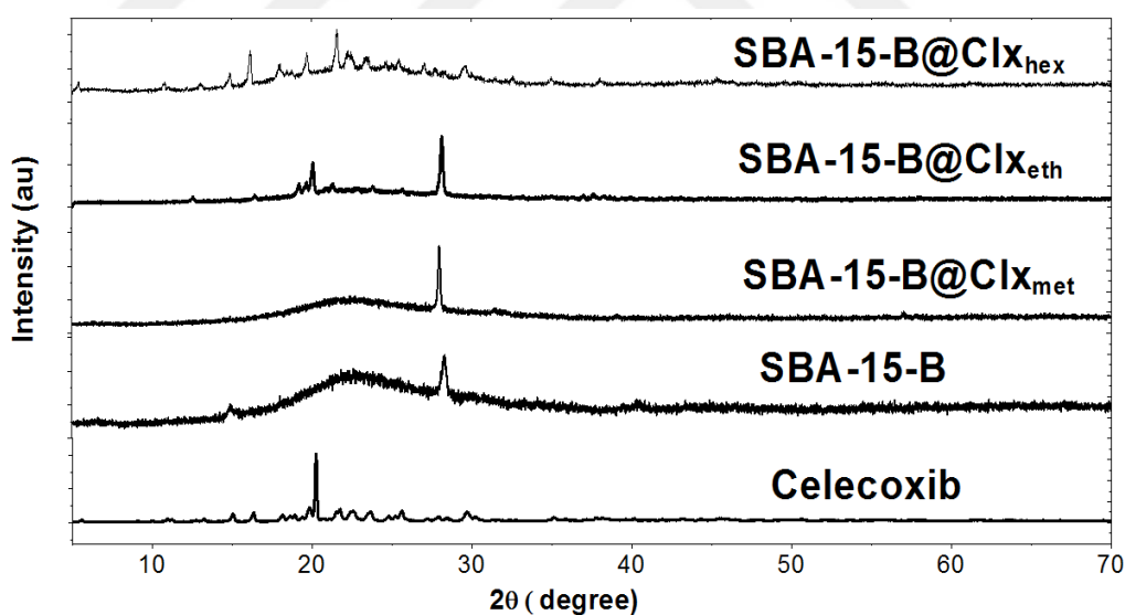
Figure 13 Wide angle powder XRD pattern of SBA-15-B, SBA-15-B@Clx eth , SBA-15-B@Clx meth , SBA-15-B@Clx hex and Celecoxib.
