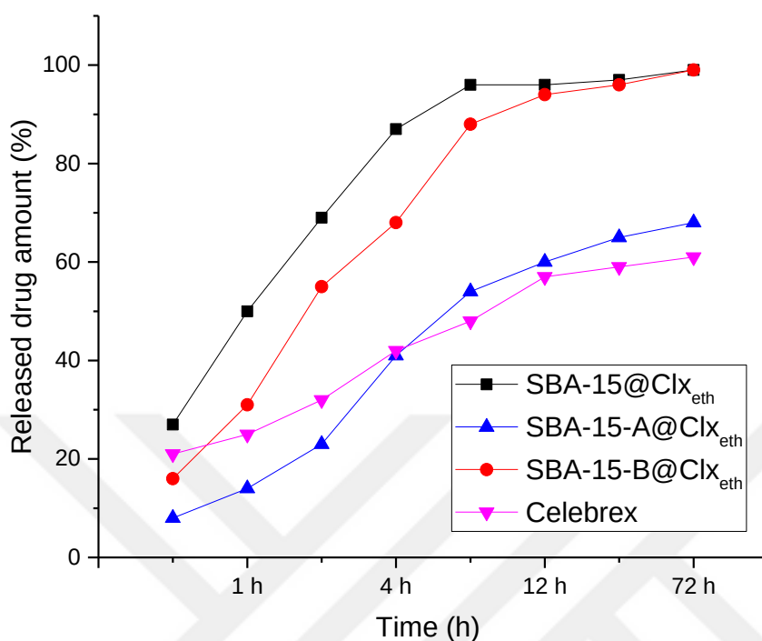
Figure 42 Amount of Celecoxib released from 1.0 g of Celebrex loaded to SBA-15, SBA-15-A and SBA-15-B in ethanol in 72 hours at pH=7.4.
