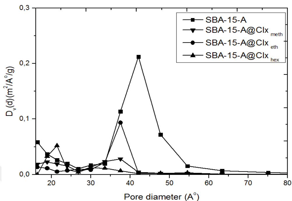
Figure 23 Pore size distribution of SBA-15-A, SBA-15-A@Clx eth , SBA-15-A@Clx meth , and SBA-15-A@Clx hex .
