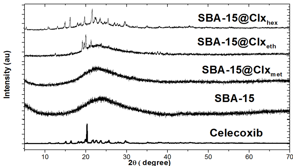
Figure 11 Wide angle powder XRD pattern of SBA-15, SBA-15@Clx ethyl , SBA-15@Clx methyl , SBA-15@Clx hex and Celecoxib.
