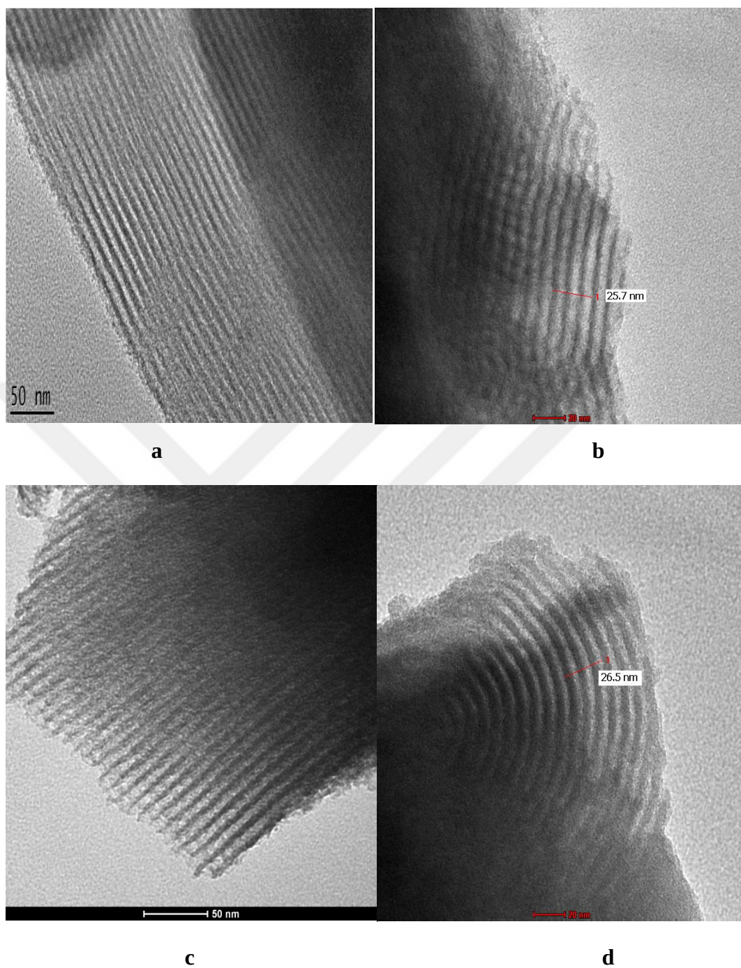
Figure 31 TEM images of a) SBA-15 (50 nm), b) SBA-15@Clx eth , (20 nm), c) SBA-15@Clx meth (50 nm), d) SBA-15@Clx hex (20 nm).
