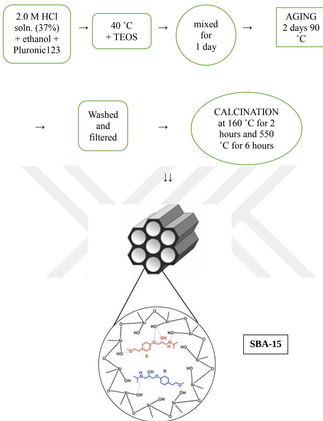
Figure 8 Schematic representation of synthesis of SBA-15.
