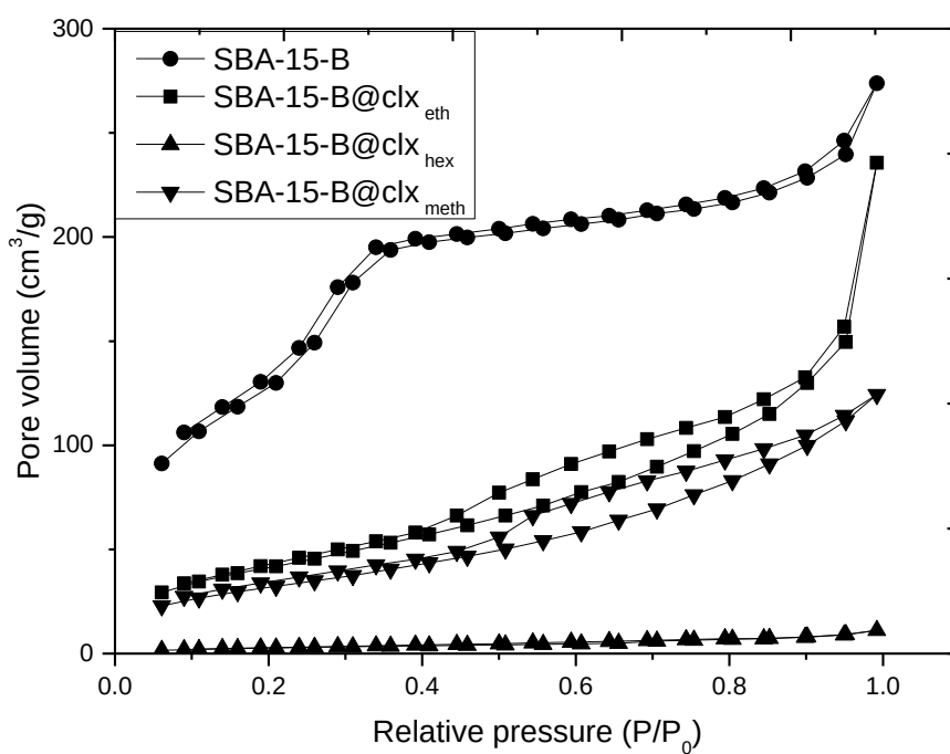
Figure 21 BET isotherms of SBA-15-B, SBA-15-B@Cl x eth , SBA-15-B@Cl x meth , and SBA-15-B@Cl x hex .
