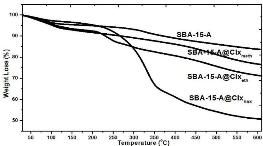
Figure 29 % Weight loss of SBA-15-A, SBA-15-A@Cl x eth , SBA-15-A@Cl x meth , and SBA-15-A@Cl x hex .
