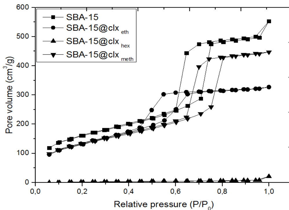
Figure 19 BET isotherms of SBA-15, SBA-15@Clx eth , SBA-15@Clx meth , and SBA-15@Clx hex .
