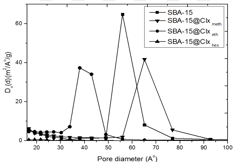
Figure 22 Pore size distribution of SBA-15, SBA-15@Clx eth , SBA-15@Clx meth , and SBA-15@Clx hex .
