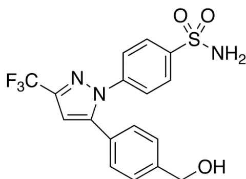
Figure 7 Structure of Celecoxib, 4-[5-(4-methylphenyl)-3-trifluoromethyl]-1H-pyrazol-1-yl] benzene sulfonamide [43].
