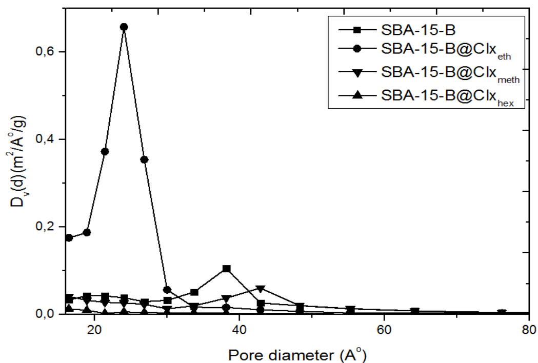
Figure 24 Pore size distribution of SBA-15-B, SBA-15-B@Clx eth , SBA-15-B@Clx meth , and SBA-15-B@Clx hex .
