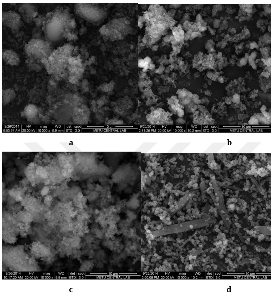
Figure 36 SEM images of a) SBA-15-B, b) SBA-15-B@Clx eth , c) SBA-15-B@Clx meth , d) SBA-15-B@Clx hex .
