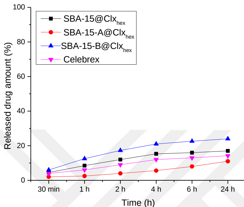
Figure 47 Amount of Celecoxib released from 1.0 g of Celebrex loaded to SBA-15, SBA-15-A and SBA-15-B in hexane in 24 hours at pH=5.0.
