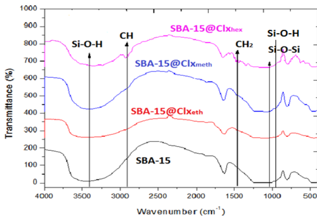
Figure 16 FT-IR spectra of SBA-15, SBA-15@Cl x eth, SBA-15@Cl x meth, and SBA-15@Cl x hex.
