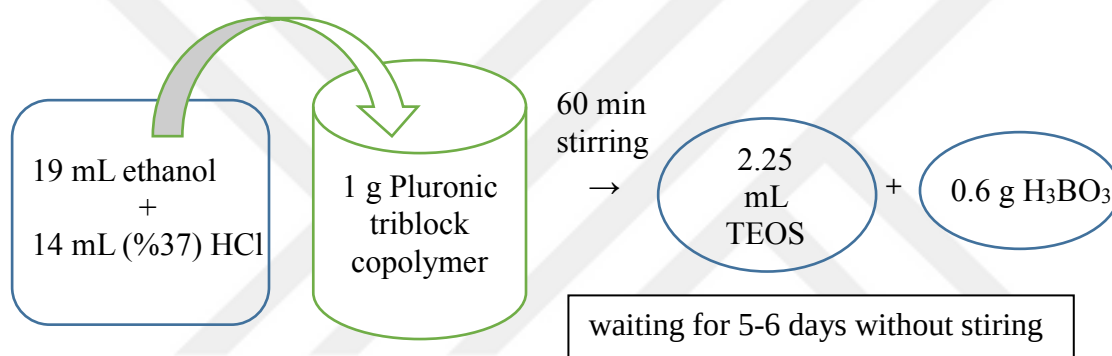
Figure 10 Schematic representation of synthesis of SBA-15-B.
