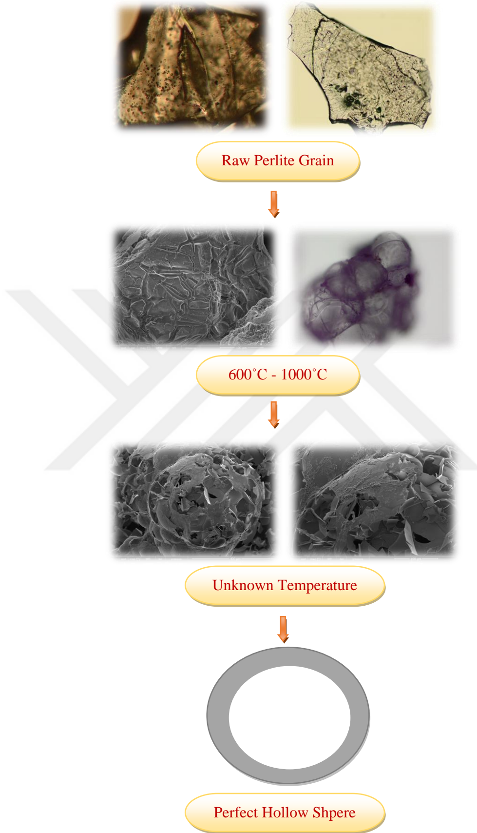
Figure 3.42. Stages of perlite expansion as morphological.
