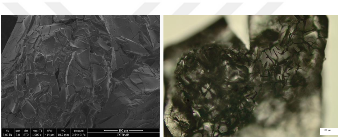
Figure 3.36. SEM and Transmitted Light Optical Microscopy images of Avdan expanded perlite samples at 1000 °C, magnifications 1000x and 20x, respectively.
