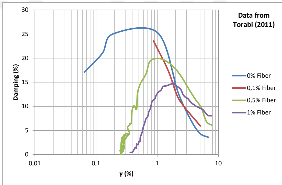
Figure 5.5: Damping vs. \gamma , Akpınar sand with fiber content of 0%, 0.1%, 0.5% and 1%
