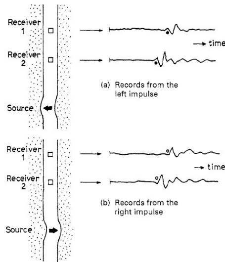
Figure 2.12: Monitoring of fronts of wave propagation by the suspension method (Kitsunozaki, 1982) (Ishihara, 1996)
