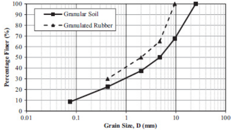
Figure 4.6: The particle size distribution for granular soil and granulated rubber (Nakhaei et al., 2012)
