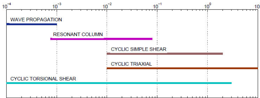
Figure 2.15: Deformation range in dynamic laboratory tests (Houbrechts et al., 2011)
