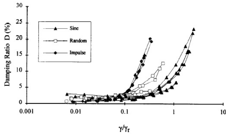
Figure 3.14: Damping Ratio vs. \gamma/\gamma_r from different loading tests (Zhang and Aggour, 1996)
