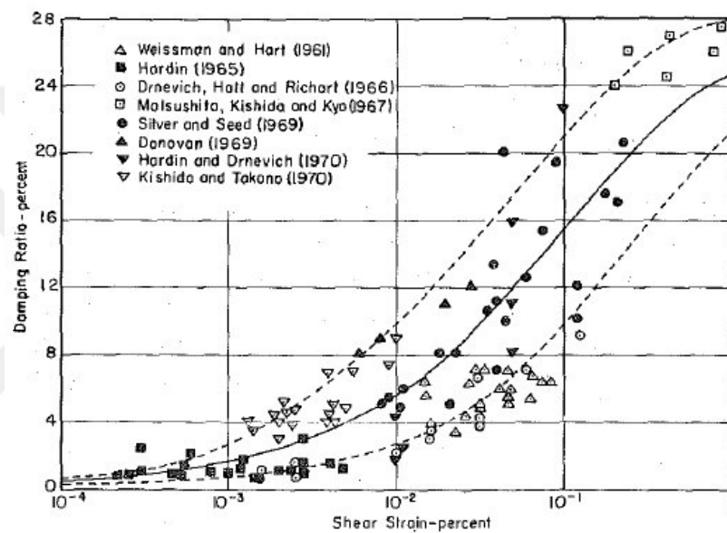
Figure 3.20: Damping ratios for sands (Seed et al., 1986)
