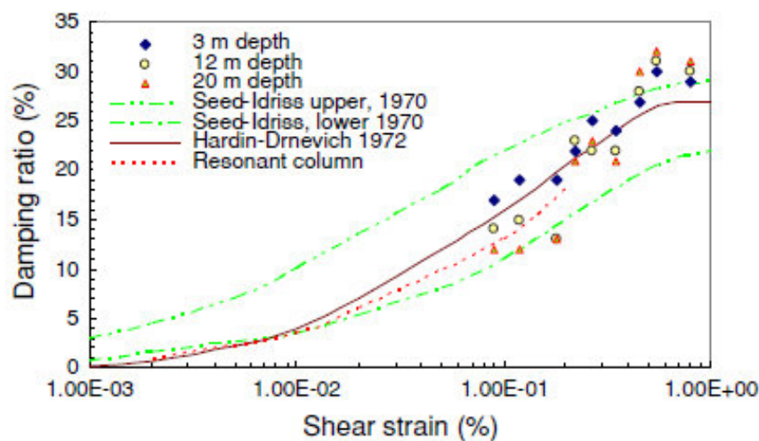
Figure 3.43: Calculated damping and emperical relationships for dry sand (Rayhani and El Naggar, 2008)
