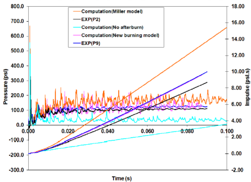
Figure 2-2 Pressure and Impulse Histories obtained from Experiments and Computed Results [5]
