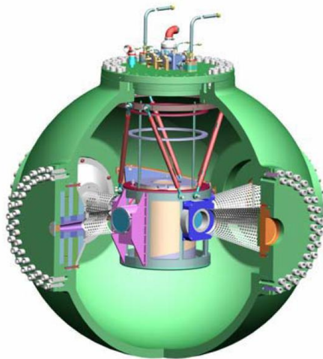
Figure 2-22 Containment Vessel [13]
