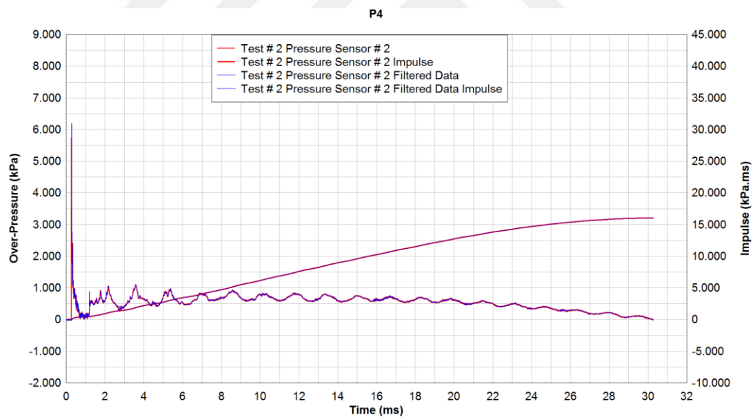
Figure 5-13 Raw and Filtered Data for P-4 (0-32 ms)
