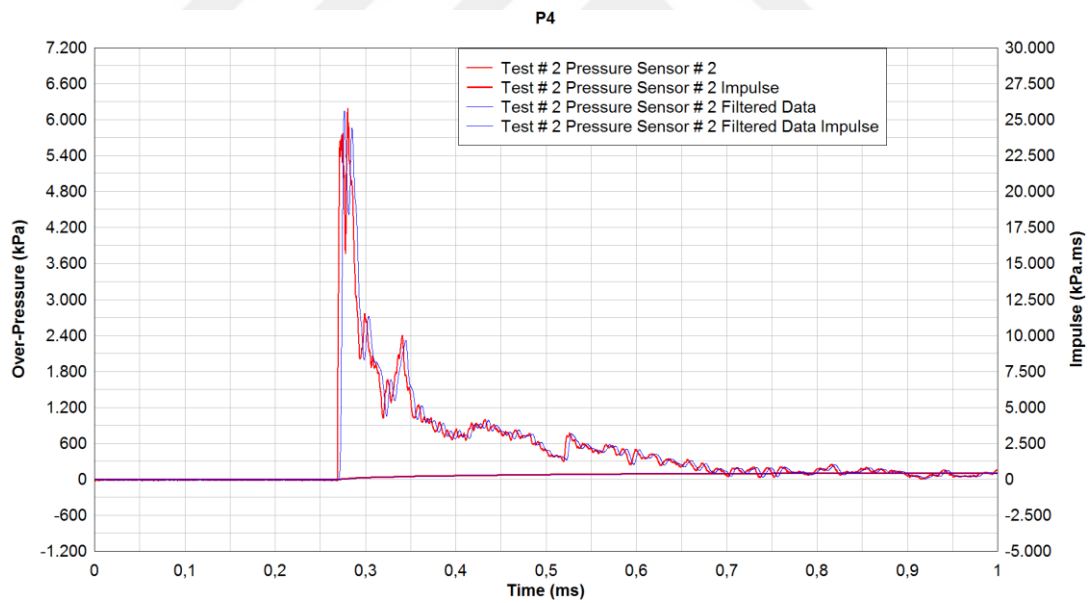
Figure 5-15 Raw and Filtered Data for P-4 (0-1 ms)
