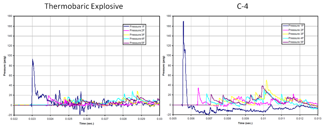
Figure 2-29 Pressure Profiles for Thermobaric Explosive and C-4 [15]
