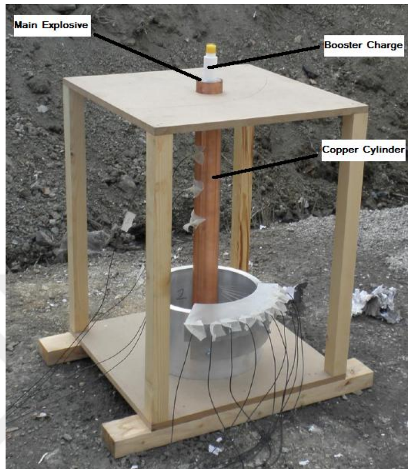
Figure 4-6 Cylinder Expansion Test Setup [31]
