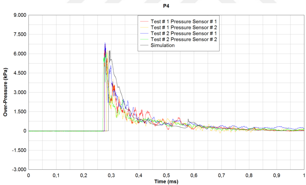
Figure 5-12 Pressure Curves for 0-1 ms
