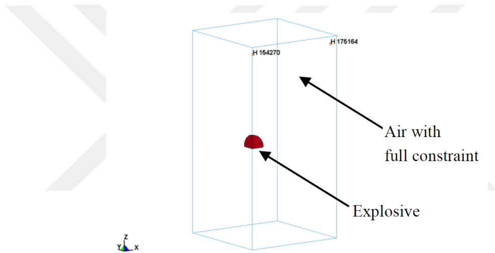
Figure 2-20 Quarter Model for Explosion Study [12]
