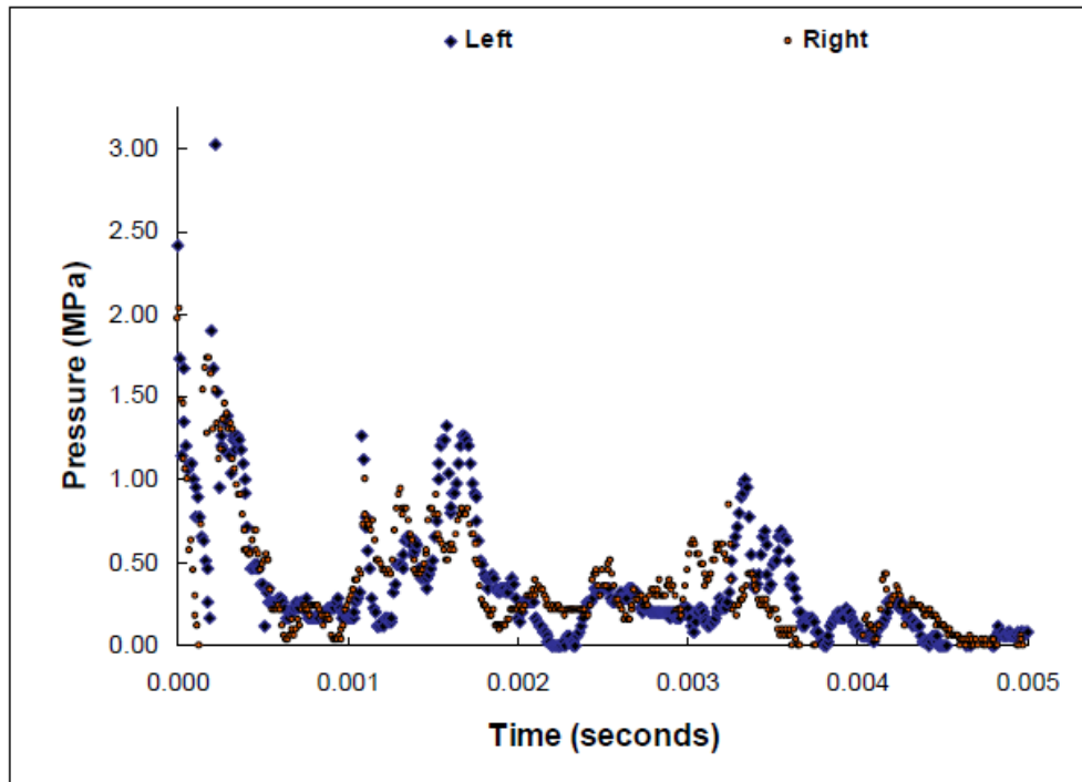
Figure 2-9 Over-Pressure vs. Time Plot of Oppositely Located Sensors [7]
