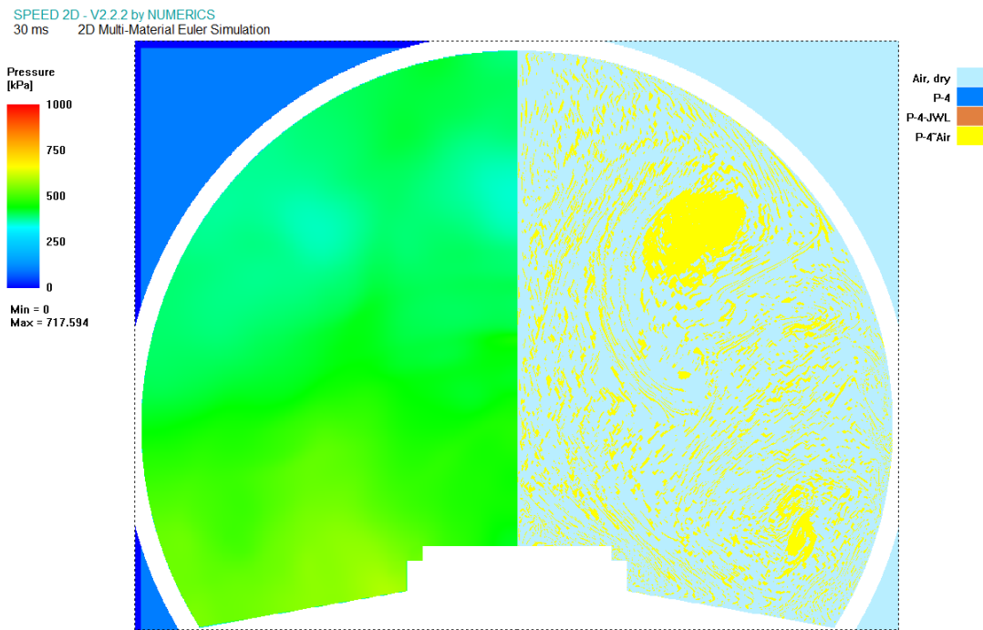
Figure A-3 Pressure and Material Distribution after Detonation of Explosive P-4 at Different Times:
