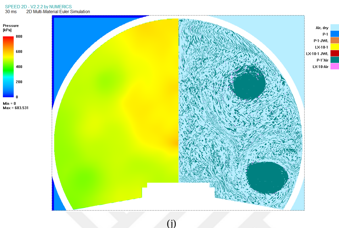
Figure 5-7 Pressure and Material Distribution after Detonation of Explosive P-1 at Different Times:
