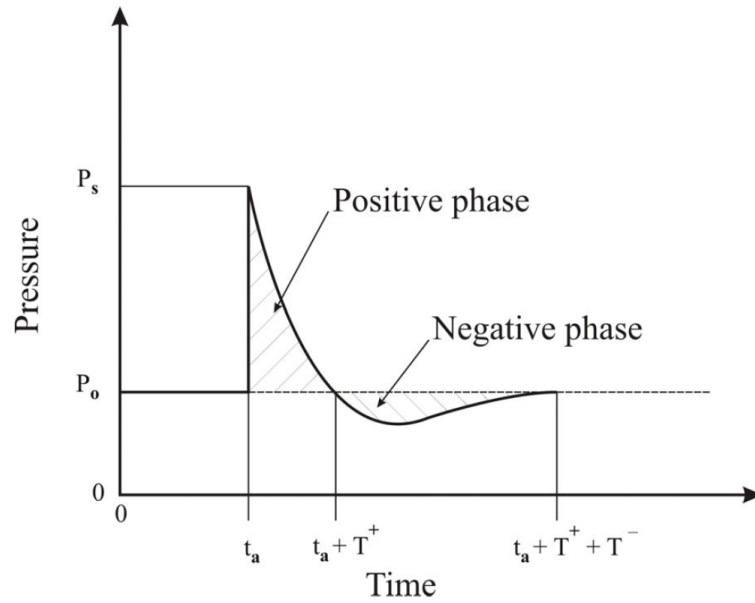
Figure 4-5 Typical Air Blast Curve [28]
