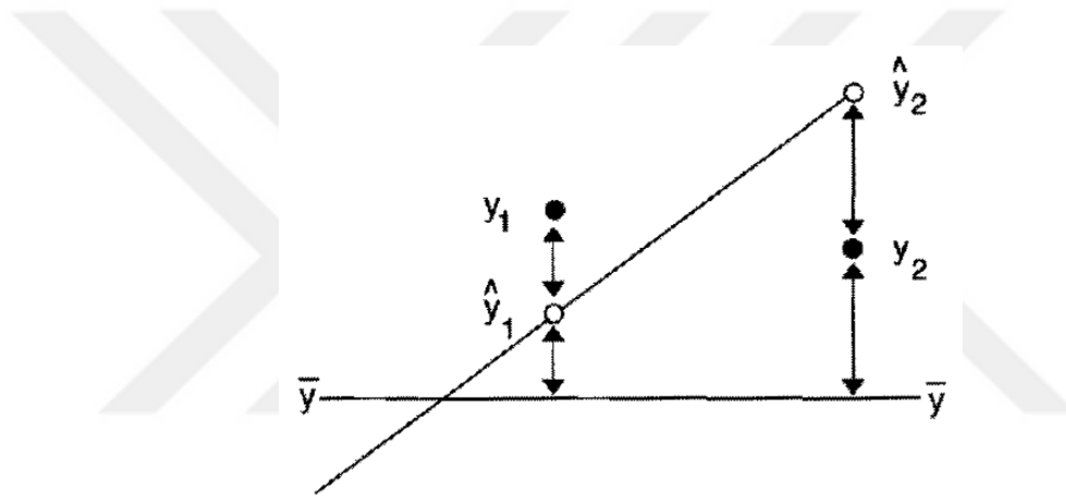
Figure 2.9. The decomposition of residuals from the mean (Source: Cohen, 1995).
