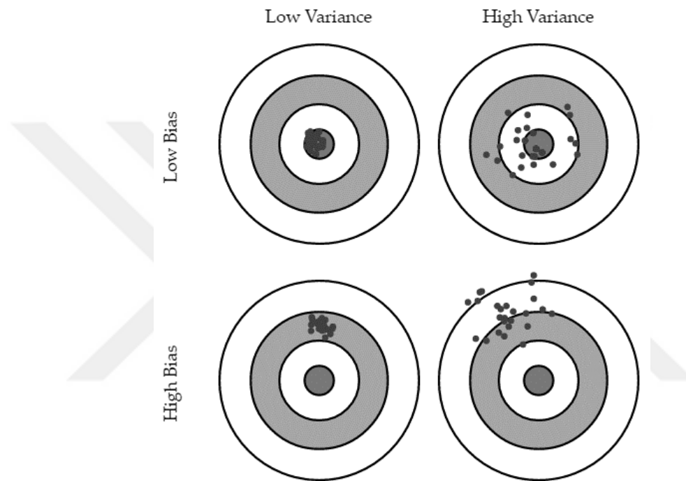
Figure 2.6. Illustration of bias and variance (Source: Fortmann-Roe S, 2013)
