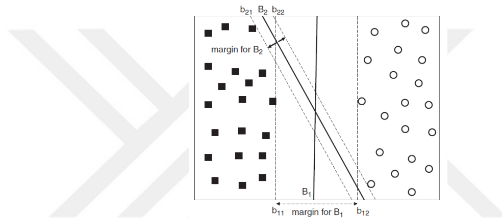
Figure 2.4. Possible decision boundaries (Source: Steinbach, 2006)
