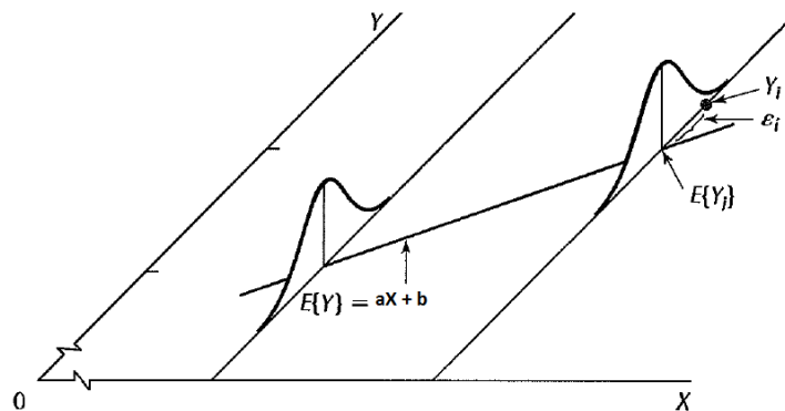
Figure 1.1. Linear regression model
