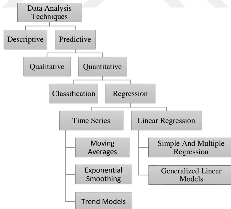
Figure 3.1. Data analysis techniques
