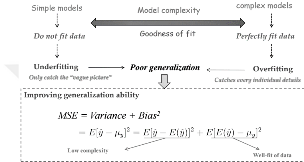
Figure 2.8. Bias and Variance Trade-off with Model complexity (Source: Li, 2011)
