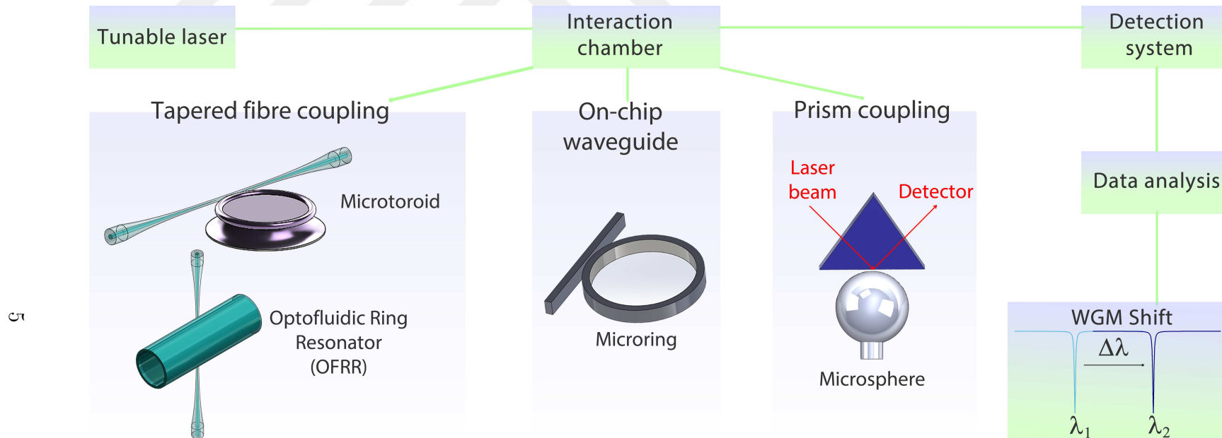
Figure 1.1: Schematic diagram summarizing the WGM based biosensing approaches using various optical resonators (microtoroids, optofluidic ring resonators (OFRRs), microrings and microspheres). Light incoming from a continuously sweeping laser source is coupled to an optical resonator via a tapered fiber, an on - chip waveguide or a prism coupler. The intensity of the transmitted light is traced using a detection system. The resonance wavelength shift (from \lambda_1 to \lambda_2 ) of the traced WGM is analyzed. The biosensing module, in which coupling and analyte infusion through the surface modified resonator occur, can be either a microfluidic or a flow system.[25]
