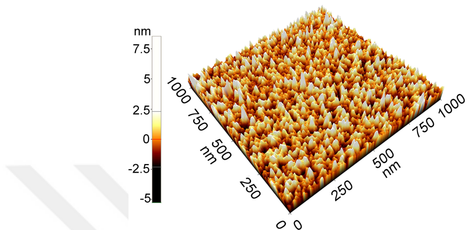
Figure 5.6: The 3D, NC - AFM scan showing the morphology of unspecifically adsorbed BSA molecules onto the Piranha treated \text{SiO}_2 surface. The R_q value was calculated as 1.23 \pm 0.19 nm. The \text{SiO}_2 surfaces having dimensions of 1 \times 1 \mu\text{m} , were used during this study. The scan rate was kept as 0.65 Hz.
