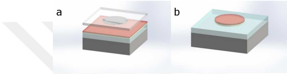
Figure 2.2: (a) A Cr mikrodisk written on the photomask (transparent layer) during the photolithography process and (b) the imprinted mikrodisk shape after the process on the wafer.
