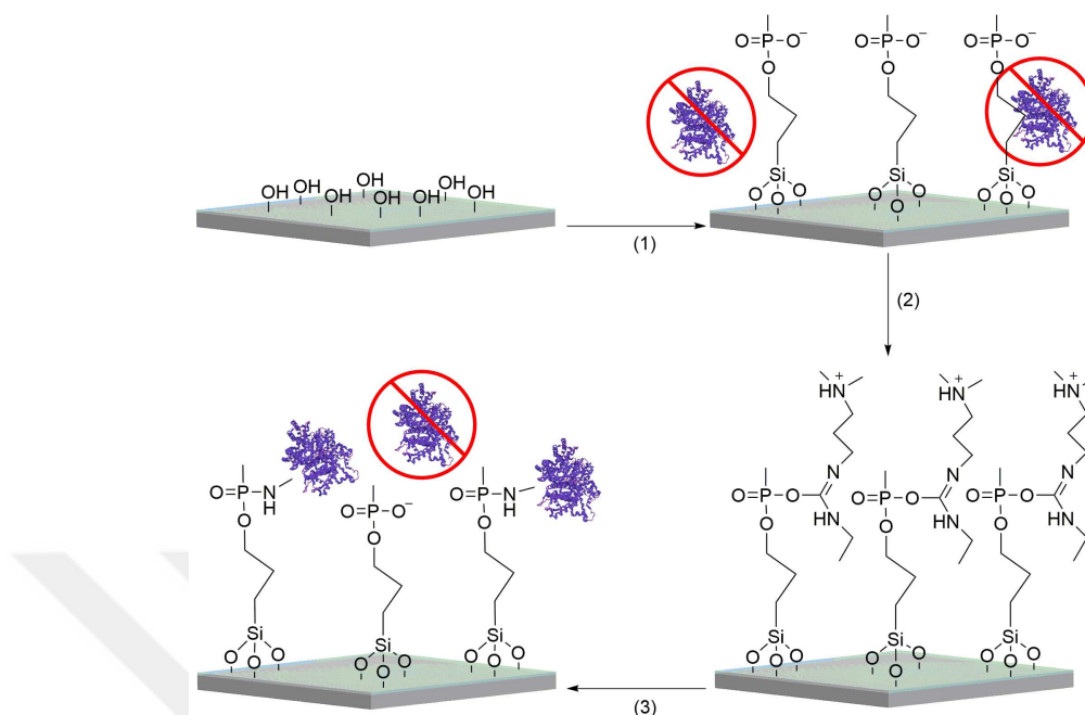
Figure 5.4: The Piranha treated \text{SiO}_2 surface is coated with THPMP molecules forming an anti - fouling coating (1). Then, \text{CH}_3\text{O}_3\text{P} groups are activated using EDC molecules, which form o - Acylisourea intermediates, which are very unstable over the surface (2). Following covalent conjugation of primary amine containing molecules to the intermediates (3), the THPMP coating gains its anti - fouling property again. The crystal structure of the BSA (purple ribbons) is shown as a primary amine containing molecule.
