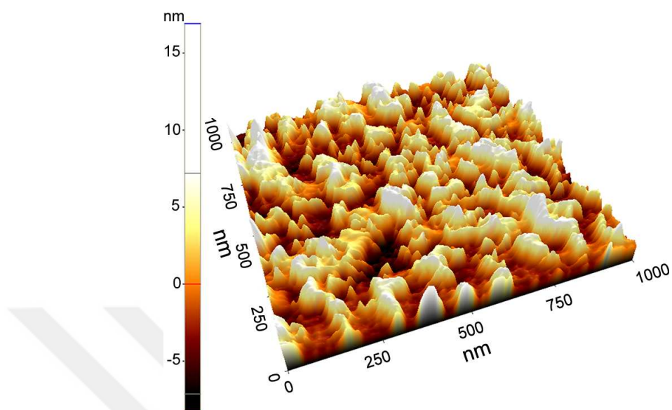
Figure 7.5: 3D, NC - AFM image of APTES / TMMS coated microtoroid surface. R_q value was calculated as 3.92 \pm 0.21 nm. Scan rate was 0.75 Hz.
