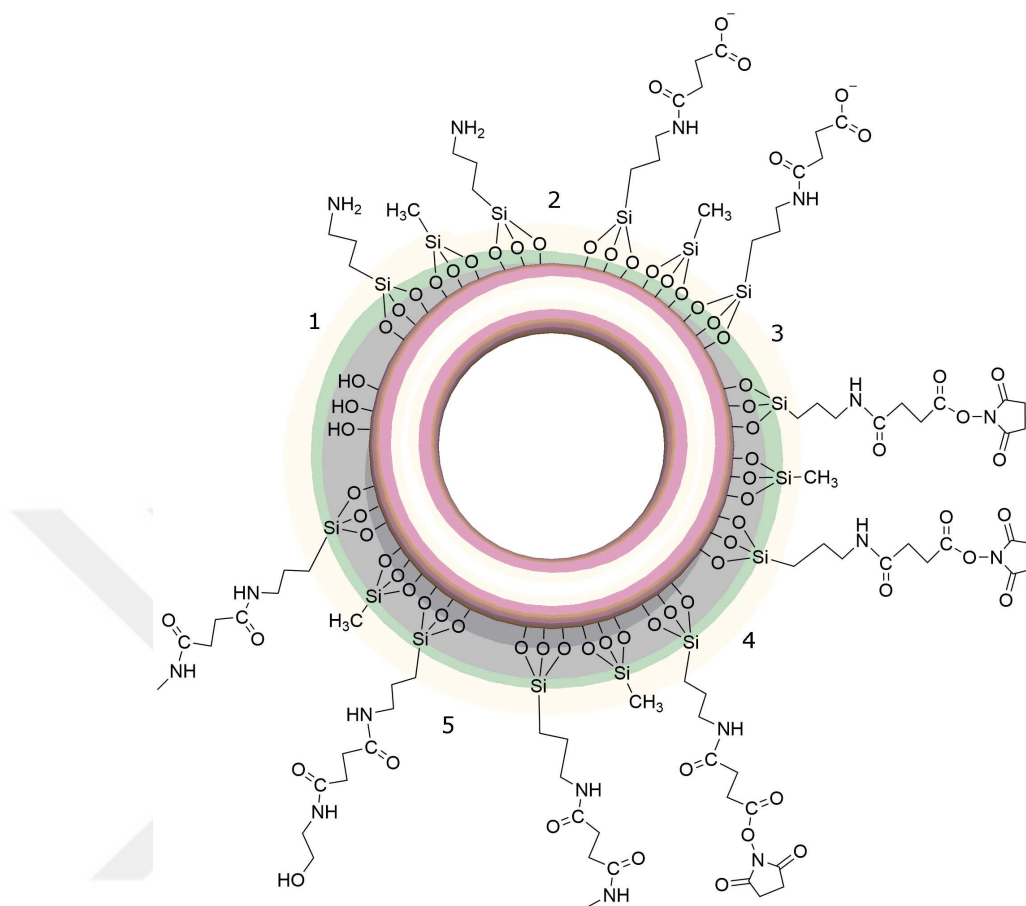
Figure 7.1: Chemical modification of the microtoroid surfaces. (1) APTES / TMMS coating of UV / Ozone pretreated surfaces, (2) Succinic anhydride incubation in DMF for 4 hrs, (3) EDC / NHS incubation in DMF for 2 hr, (4) Covalent \text{NH}_2 - modified probe ss - DNA conjugation in 1 M \text{KH}_2\text{PO}_4 at 37 °C overnight, and (5) ethanolamine capping to remove residual NHS - esters.
