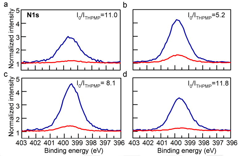
Figure 5.13: The detailed region scans for N1s, from Piranha cleaned and THPMP having SiO 2 samples incubated in (a) BSA, (B) \gamma - globulin, (c) fibrinogen, and (d) lysozyme having buffers. The coating showed a dramatic anti - fouling property in all measurements. The intensities from the Piranha treated ( I_0 ) and THPMP coated ( I_{THPMP} ) samples were also obtained.
