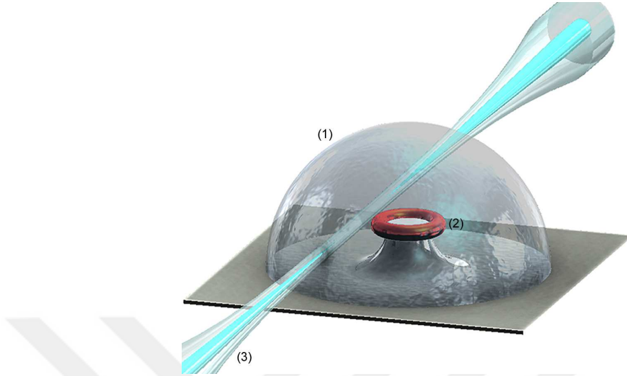
Figure 3.5: A schematic drawing showing in (1) a micro - aquarium, (2) a microtoroidal optical resonator is coupled to (3) a tapered fiber with its core (blue) and cladding (transparent).
