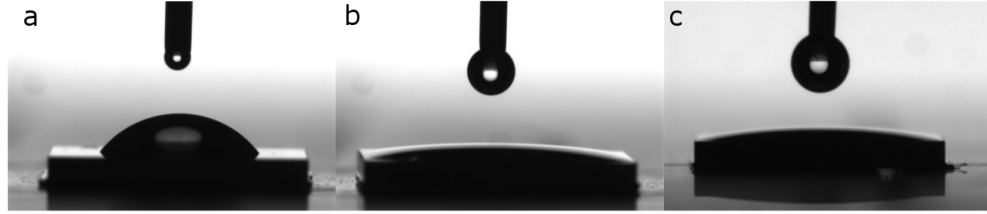
Figure 5.2: The photographs of 0.3 \mu\text{l} water droplets on (a) Cleaned, (b) Piranha cleaned and (c) UV / Ozone treated \text{SiO}_2 wafers.
