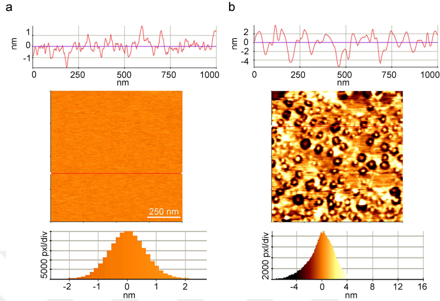
Figure 5.5: The 2D, NC - AFM scans of (a) bare and (b) THPMP having SiO 2 surfaces. For each AFM image, red line profiles (above) and histograms (below) were also provided. The SiO 2 surfaces having dimensions of 1 x 1 \mu\text{m} , were used during this study. The scan rate was kept as 0.65 Hz.
