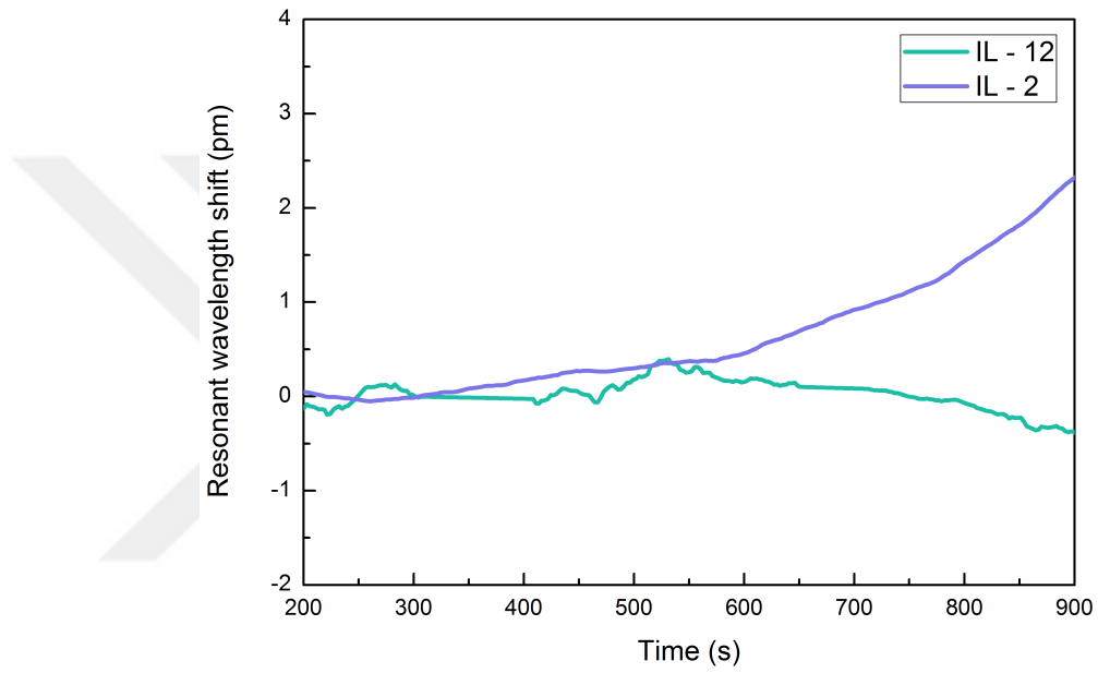
Figure 6.6: The human IL - 2 antigen was detected in 10 v/v % FBS having 1 X PBS buffer. As a control, mouse IL - 12 antigens were infused in complex media. The infusions were both started at t = 0 with an infusion rate of 10 \mu\text{l} / \text{s} , and continued for 600 secs. The functionalized microtoroids showed a significant WGM resonance shift during IL - 2 infusion in complex media (purple line), while no significant WGM shift was observed due to the IL - 12 infusion (teal line). The cumulative data were smoothed by adjacent averaging, considering an averaging time of 1 min.
