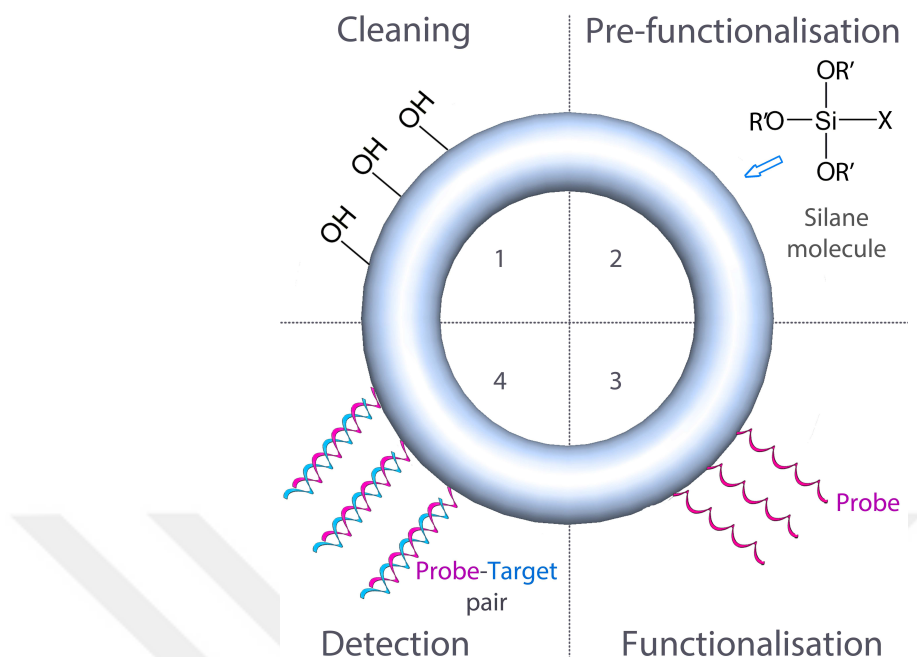
Figure 5.3: Surface modification of an optical resonator for specific target detection. Schematic drawing shows a general approach to the chemical modification of a \text{SiO}_2 based optical resonator for specific oligonucleotide based detection. (1) Cleaning of biosensor via UV / Ozone or chemical (Piranha) treatment to induce reactive silanol groups. (2) Pre - functionalization of the biosensor surface with a silane molecule via silane condensation reaction. Where \text{OR}' can be a methoxy, ethoxy or acetoxy and \text{X} can be an alkyl, aryl or organofunctional group. (3) Surface functionalization by covalently conjugating an oligonucleotide probe (either modified or non - modified) to the silane coated biosensor. Also, in between a silane molecule and a probe, a linker molecule can be used. (4) Specific target detection using probe - target interactions.
