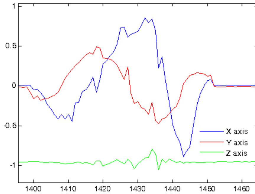
Figure 16. The raw data signals of 'c' character
