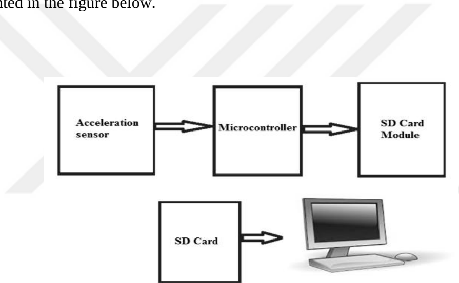
Figure 25. Overall Structure of the Hardware
