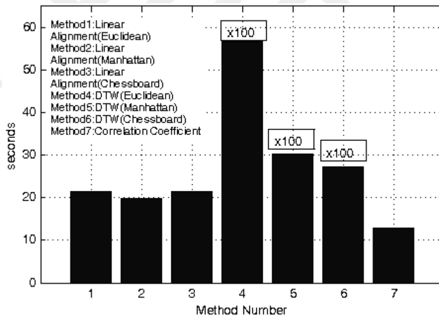
Figure 53. Time duration of each method for raw data (user independent)
