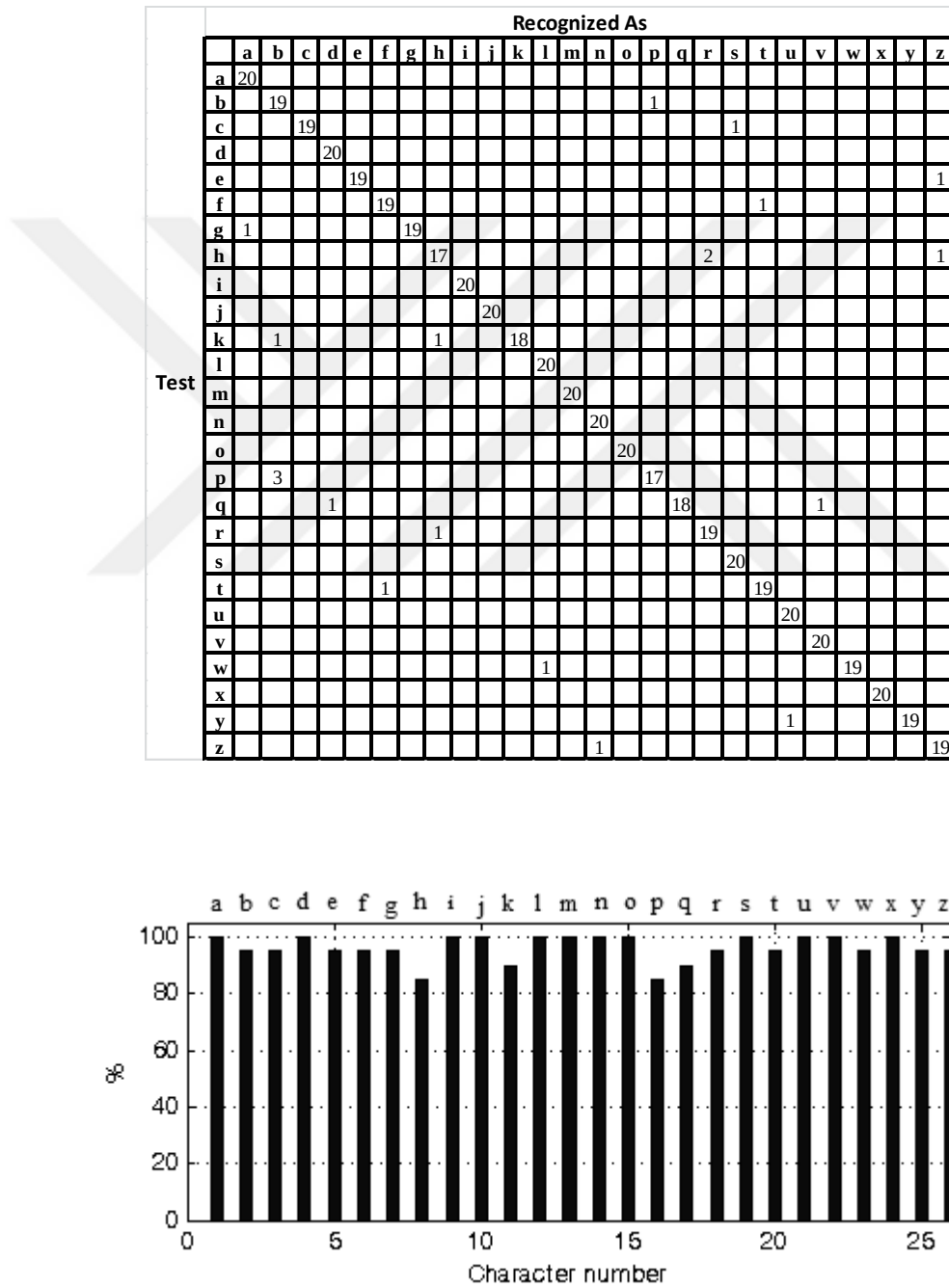
Figure 43. Accuracy of each character (linear alignment with Euclidean)
