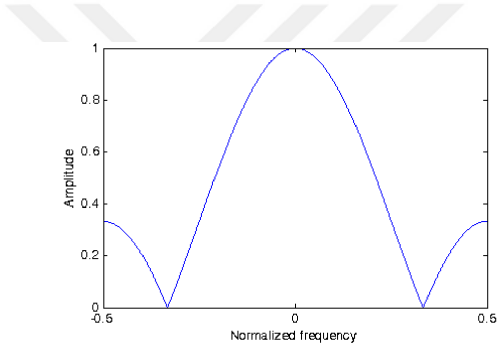
Figure 34. Frequency response of the MAF
