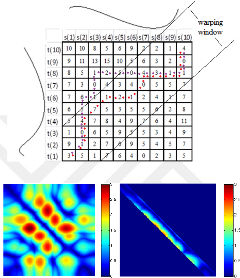
Figure 23. Warping path restricted by a warping window
