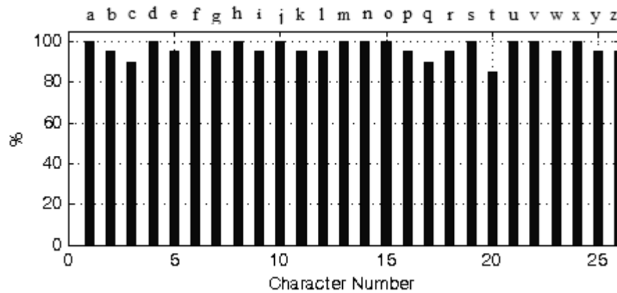
Figure 67. Accuracy of each character (DTW with Manhattan)
