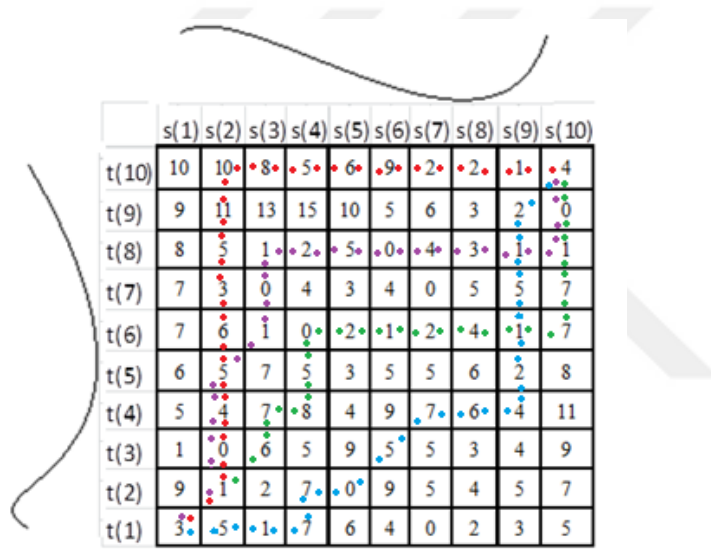
Figure 22. Some of the possible warping paths
