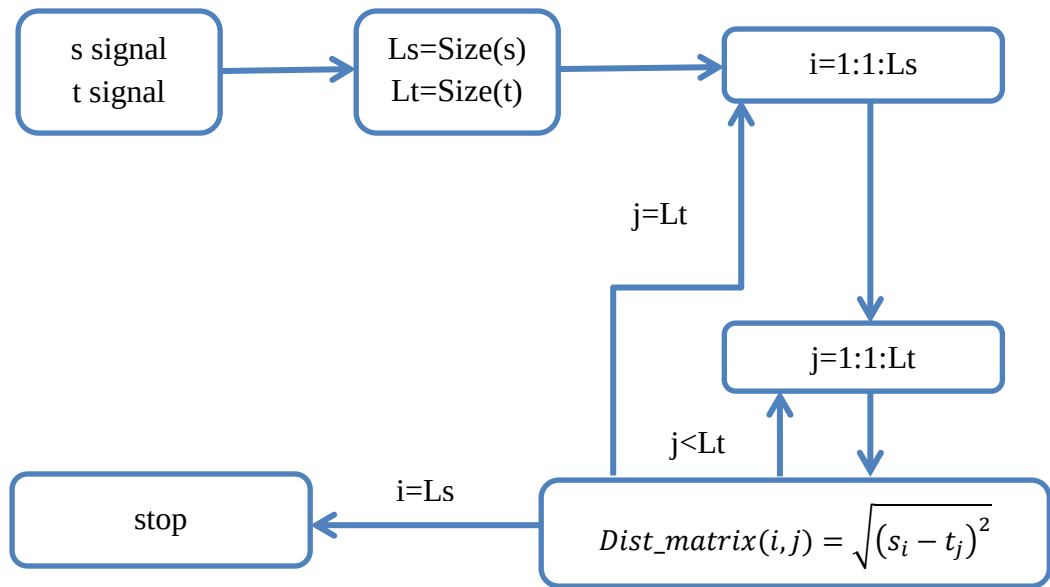
Figure 21. Flowchart for creating the Distance matrix
