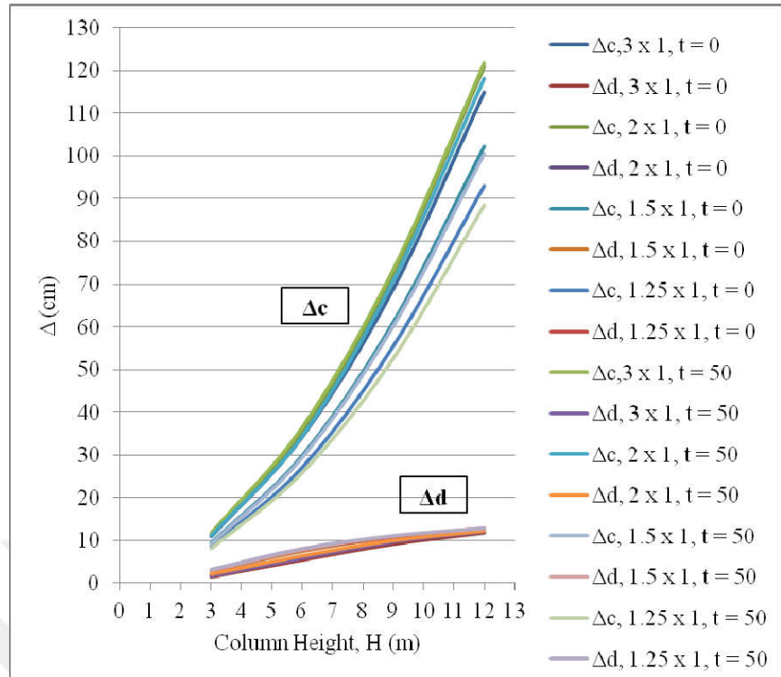
Figure 5.3: \Delta_c & \Delta_d versus Column Height (Set – 2 bridges)
