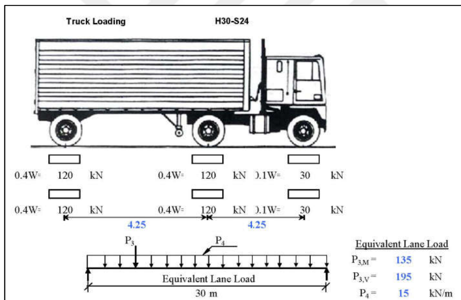
Figure 3.16: H30S24 Loading
