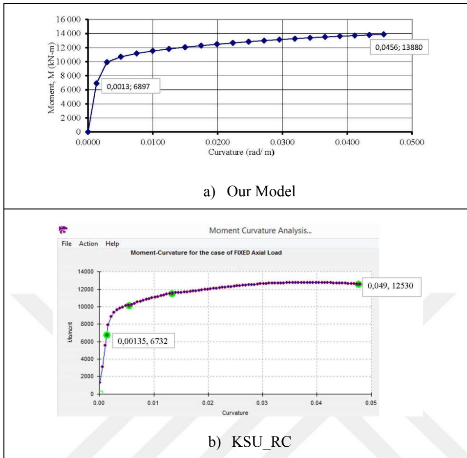
Figure A.4: Moment – Curvature Diagrams
