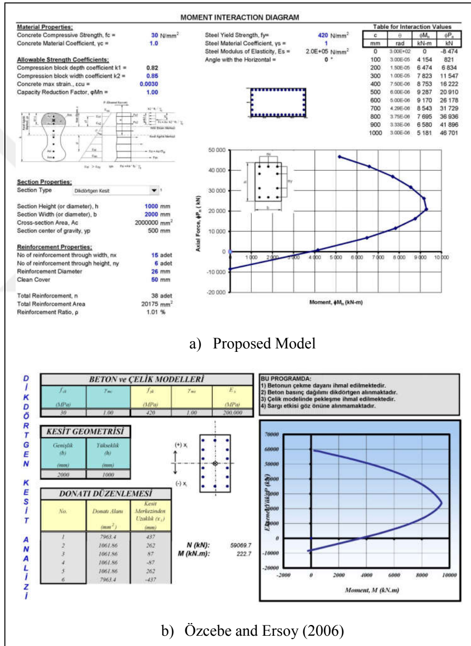
Figure A.5: Moment – Axial Load Interaction Diagrams
