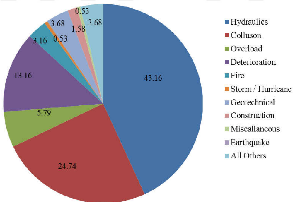
Figure 2.4: Reasons of Bridge Partial Failures in the United States in 1987 – 2011
