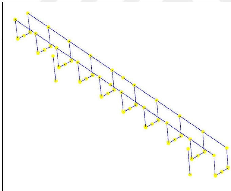
Figure 3.9: Rigid Elements
