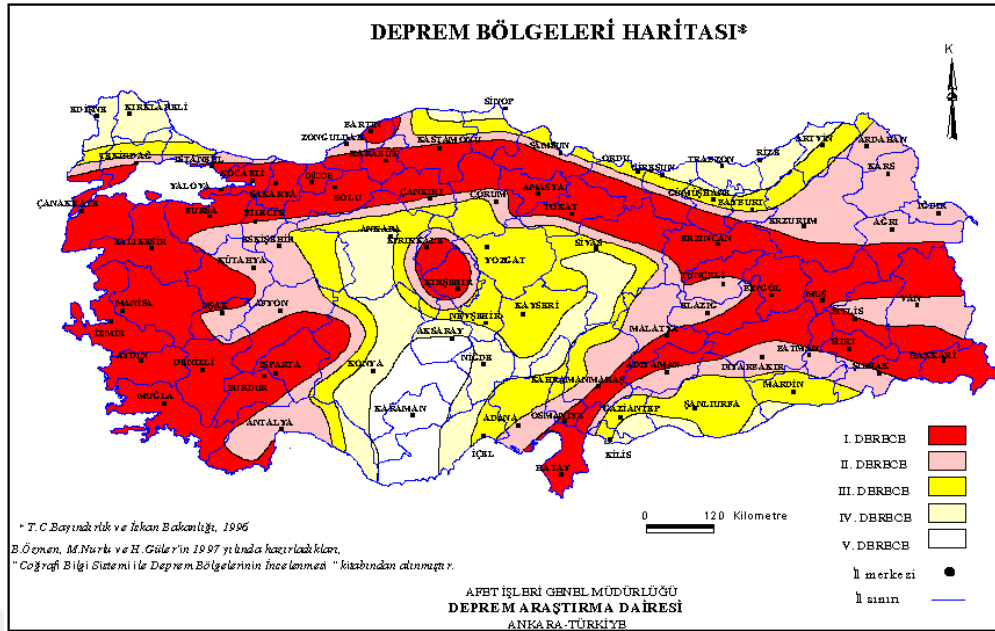
Figure 3.17: Turkey Seismic Zone Map (1996)
