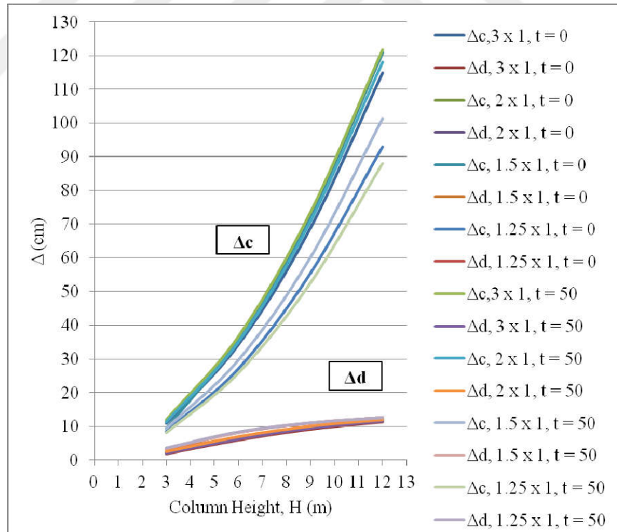
Figure 5.4: \Delta_c & \Delta_d versus Column Height (Set – 3 bridges)
