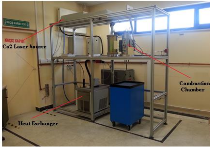
Figure 8 Laser Ignition Test Setup used in Roketsan
