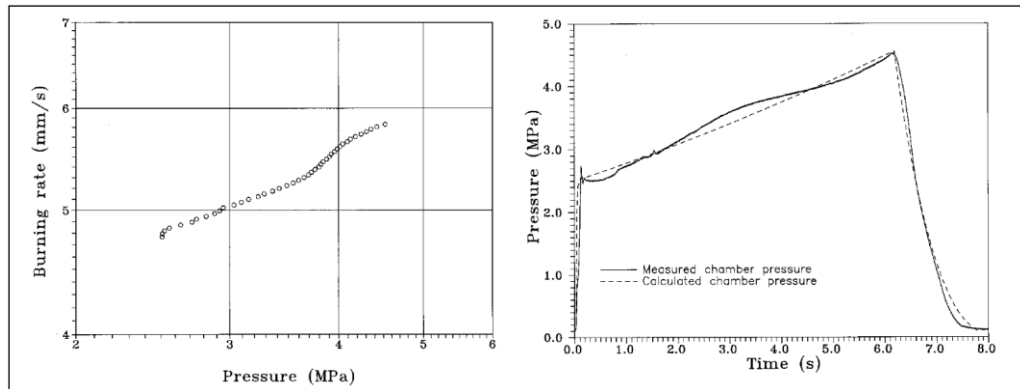
Figure 23 Test results obtained from burning rate evaluation motor [15]
