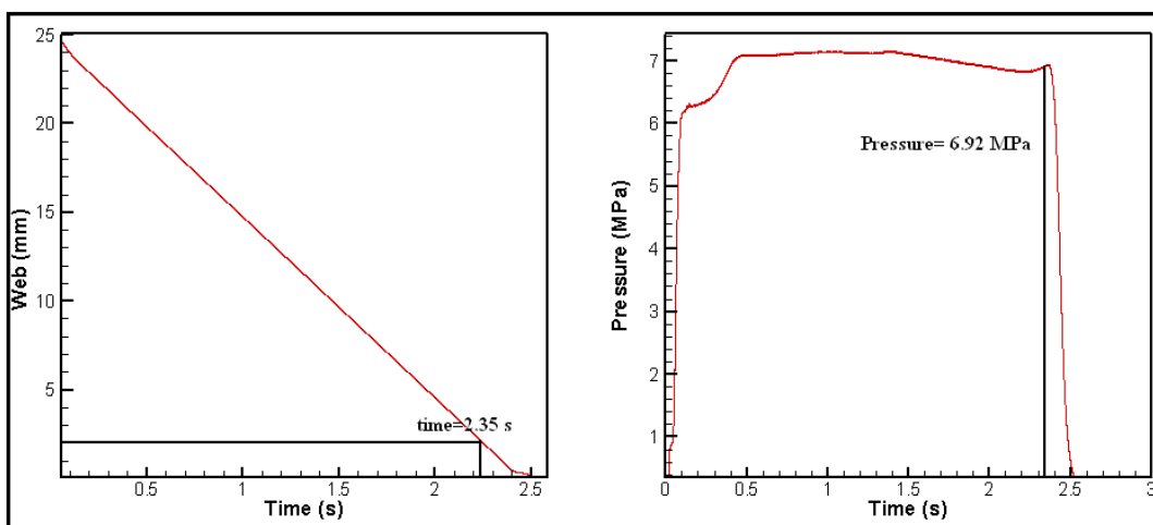
Figure 96 Test results obtained from test 3
