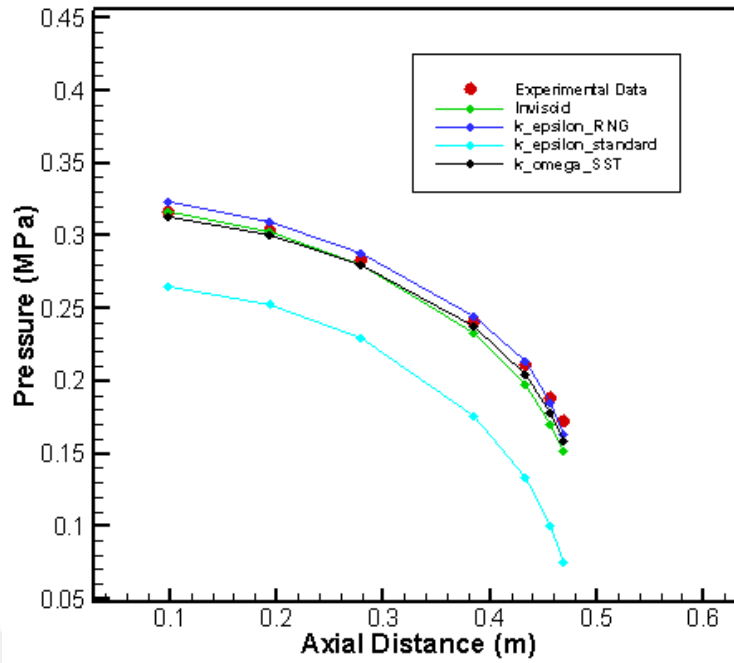
Figure 90 Axial pressure distribution
