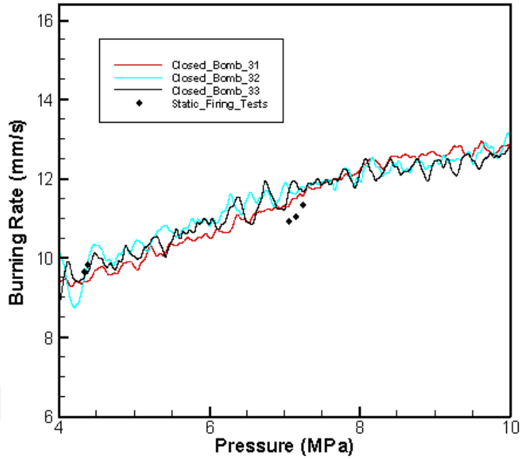
Figure 62 Burning rate versus pressure that belongs to BTYP1
