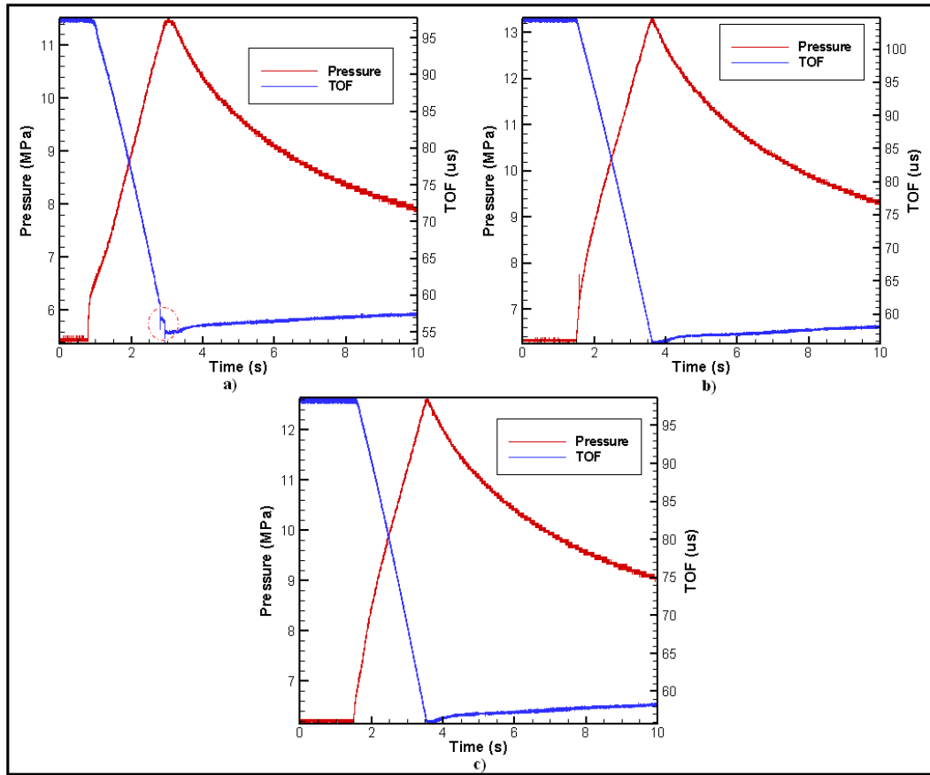
Figure 55 Measured pressure and time of flight versus time for a) Test 10 b) Test 11 c) Test12
