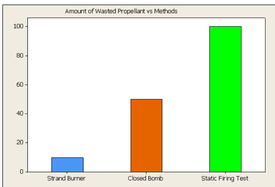
Figure 71 Amount of Wasted Propellant versus Methods
