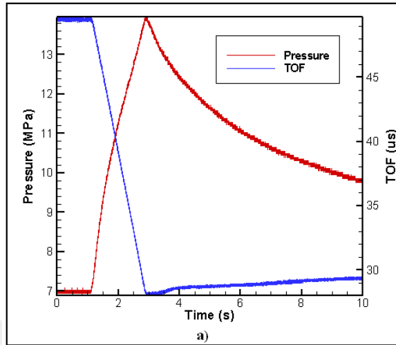
Figure 53 a) Measured pressure and time of flight versus time for Test 9
