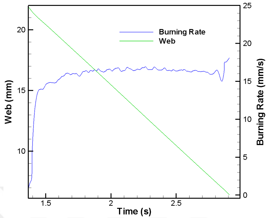
Figure 82 Burning rate and web thickness with respect to time for test 2
