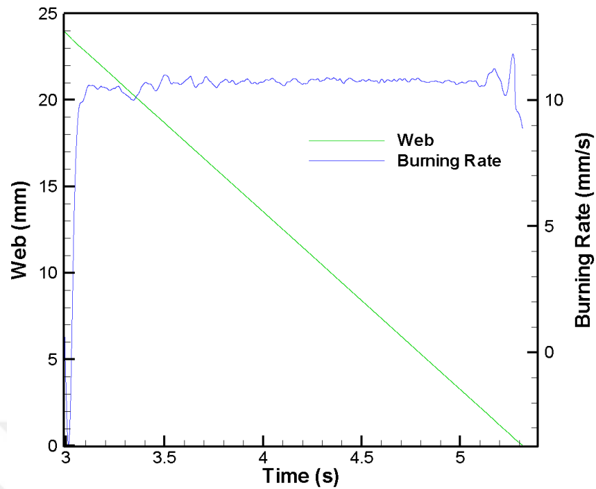
Figure 85 Burning rate and web thickness with respect to time for test 3
