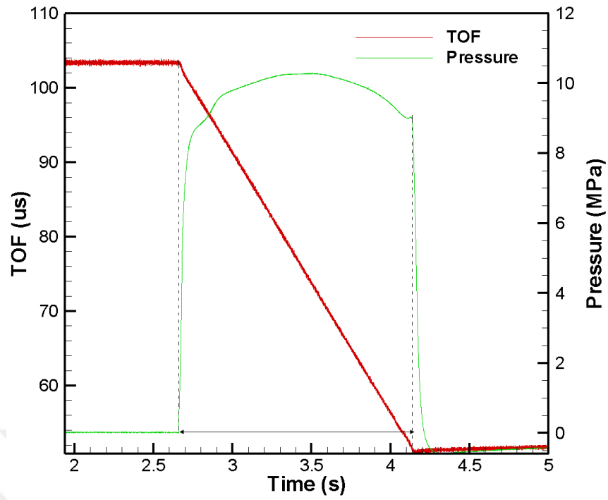
Figure 77 Pressure and Time of Flight data with respect to time for test 1
