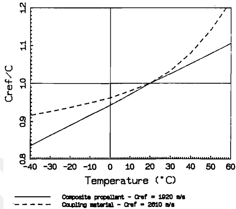
Figure 13 Ultrasonic wave velocities belong to AP/HTPB composite propellant with respect to temperatures [14]
