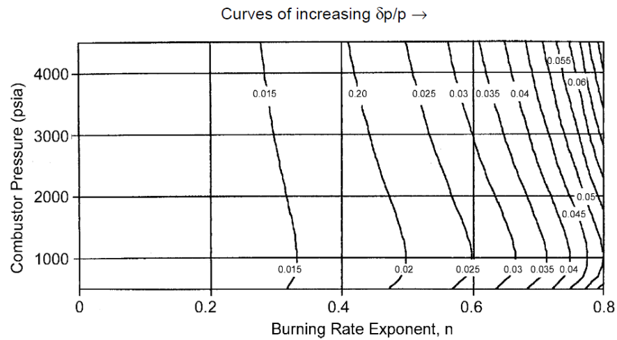
Figure 3 Variability in Reference Burning Rate and Exponent Effect on Performance [4]
