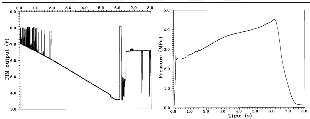
Figure 22 Voltage output and chamber pressure of the test motor [15]
