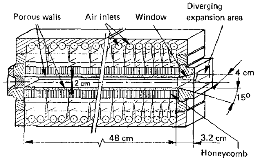
Figure 87 Experimental setup used for test case [36]
