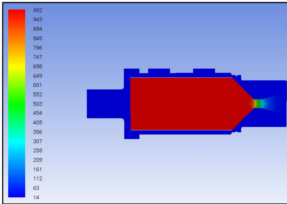
Figure 95 Static pressure distribution in test motor
