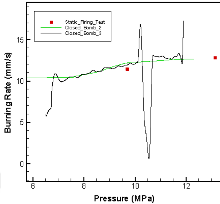
Figure 48 Burning Rates versus pressure belong to OMTYPE2
