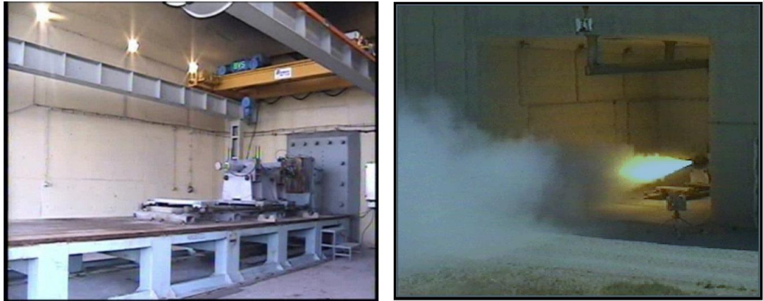
Figure 5 Static firing tests carried by Roketsan
