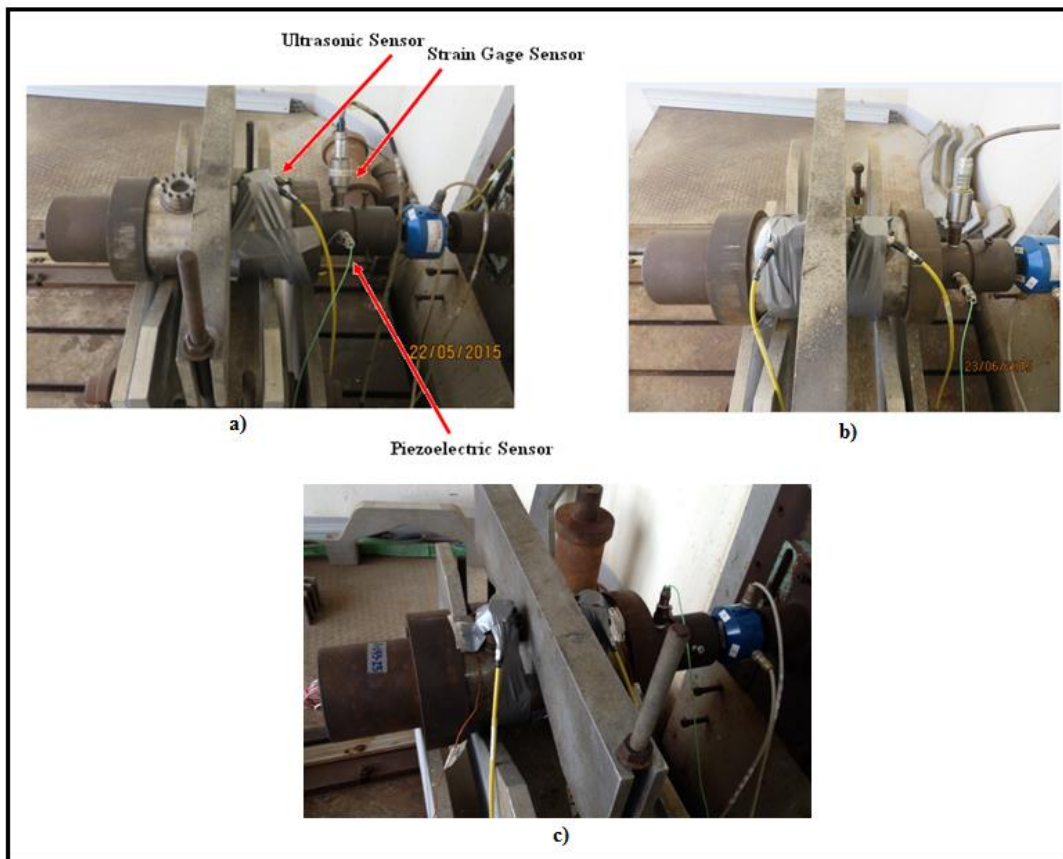
Figure 76 Test Motor Firings that belong to a) Test 1 b) Test 2 c) Test 3 placed at ground test platform
