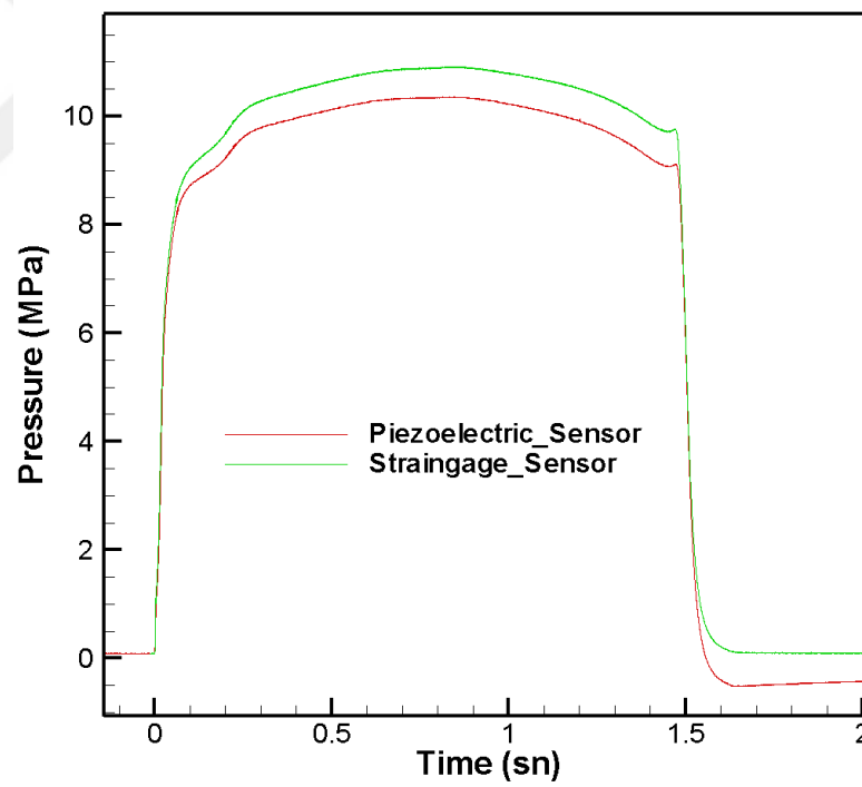
Figure 78 Pressure data collected by two types of sensor for test 1
