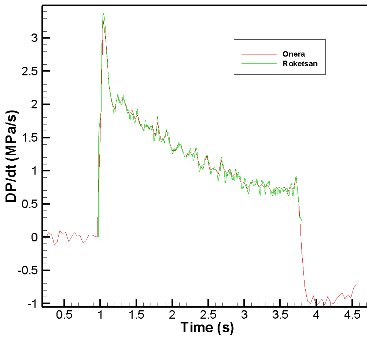
Figure 110 Derivative of Pressure with Respect to Time
