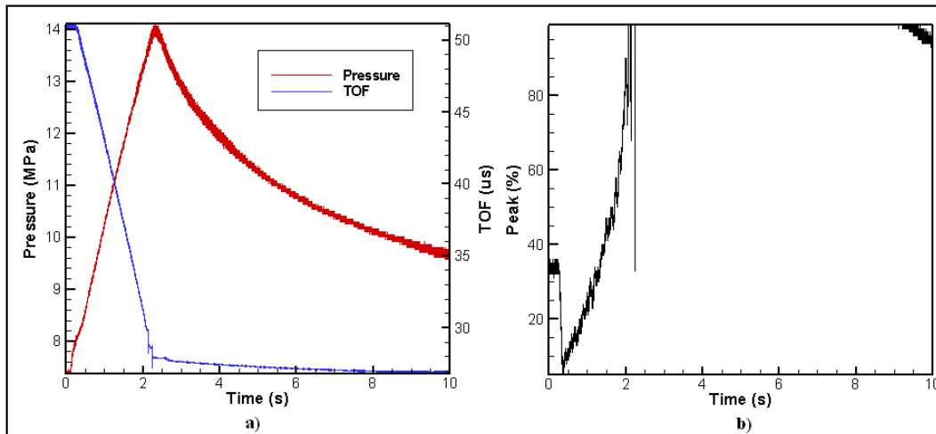
Figure 52 a) Measured pressure and time of flight versus time for Test 8 b) Peak data versus time for Test 8
