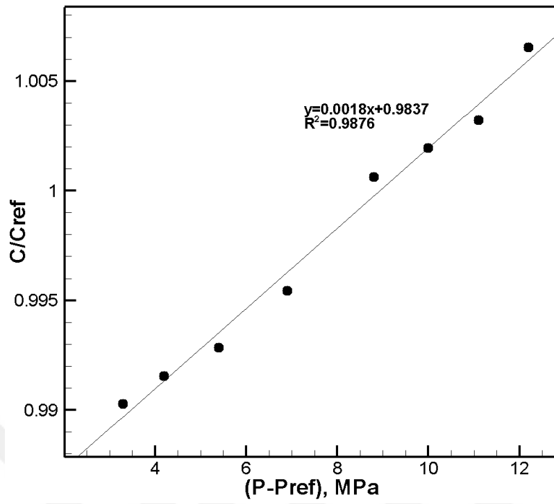
Figure 111 Wave velocity variation with pressure for propellant
