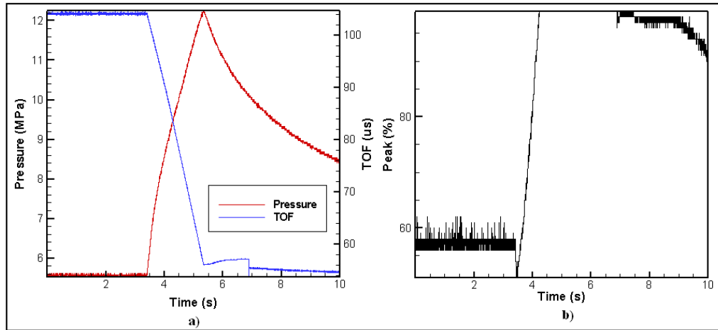
Figure 45 a) Measured pressure and time of flight versus time for Test 2 b) Peak data versus time for Test 2
