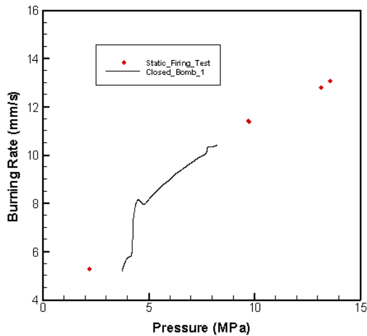
Figure 44 Burning rate versus pressure for Test 1
