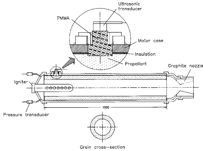
Figure 21 Test motor for burning rate evaluation [15]
