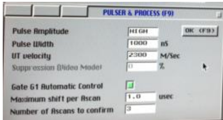
Figure 117 Pulser& Process
