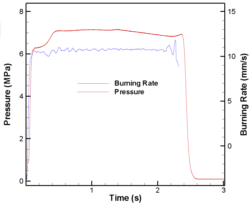
Figure 86 Burning rate and pressure with respect to time for test 3
