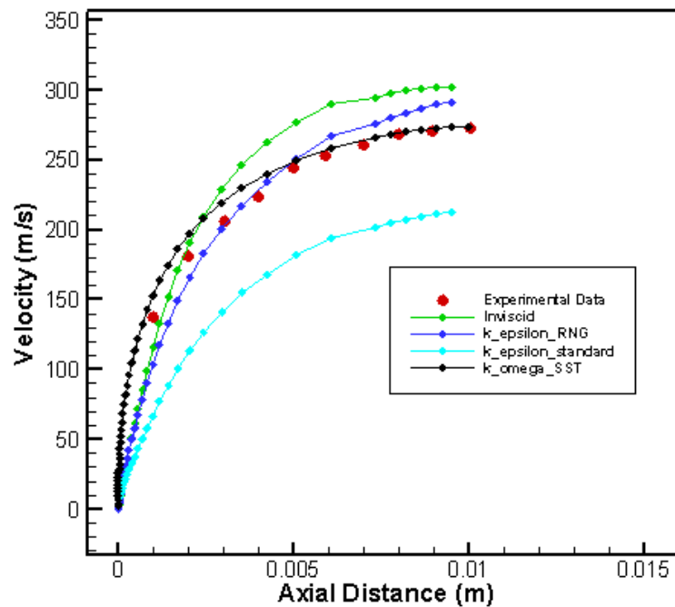
Figure 92 Velocity profile at location 0.461 m
