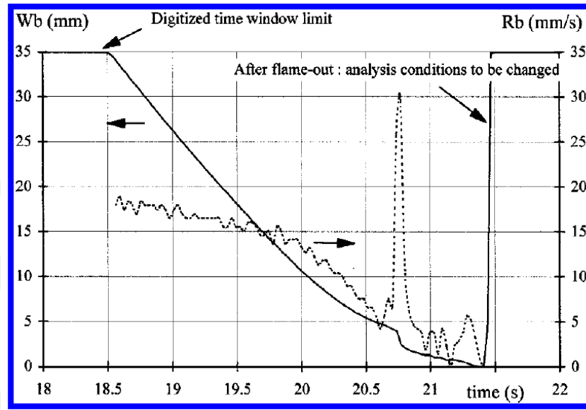
Figure 26 Web thickness and burning rate with respect to time [30]
