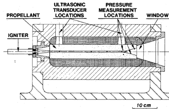
Figure 16 Two-dimensional setup that was used in [1]
