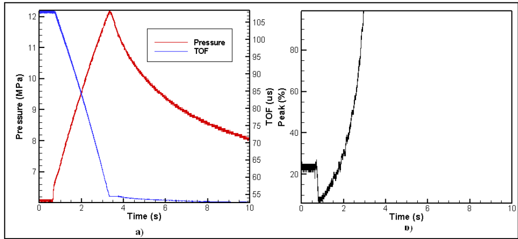
Figure 49 a) Measured pressure and time of flight versus time for Test 5 b) Peak data versus time for Test 5
