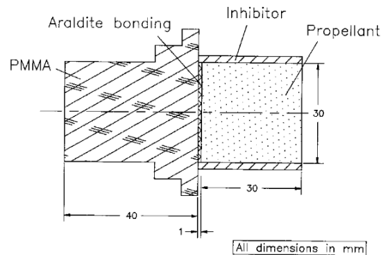
Figure 20 Propellant Sample Used in Closed Bomb Tests [15]
