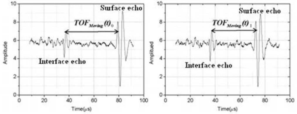
Figure 11 Moving gate method modified from [35]
