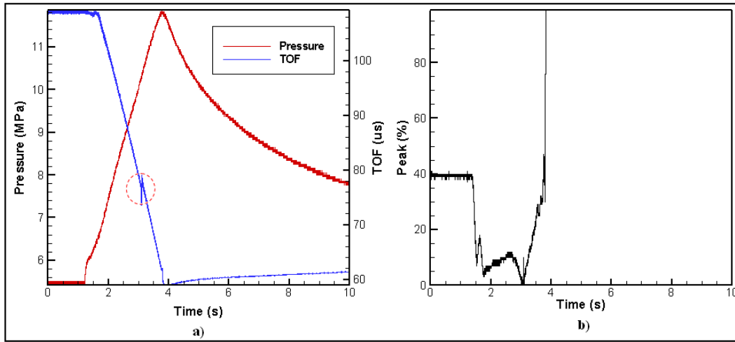
Figure 46 a) Measured pressure and time of flight versus time for Test 3 b) Peak data versus time for Test 3
