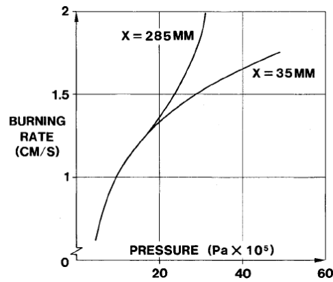
Figure 19 Test results for the two-dimensional test setup [1]
