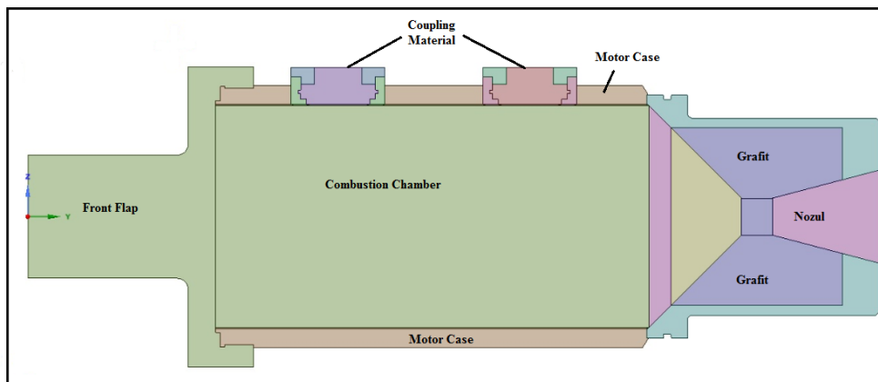
Figure 93 Subscale Test Motor
