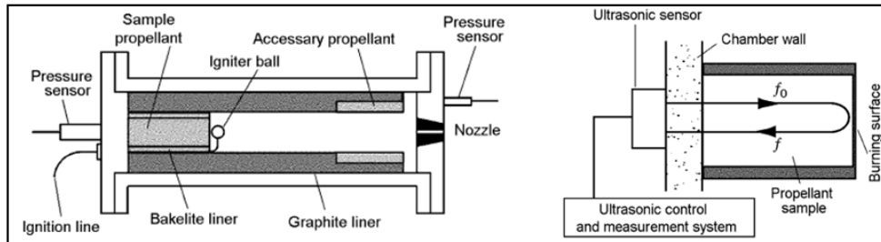
Figure 15 A sketch of combustion chamber and principle of the Doppler method [23]
