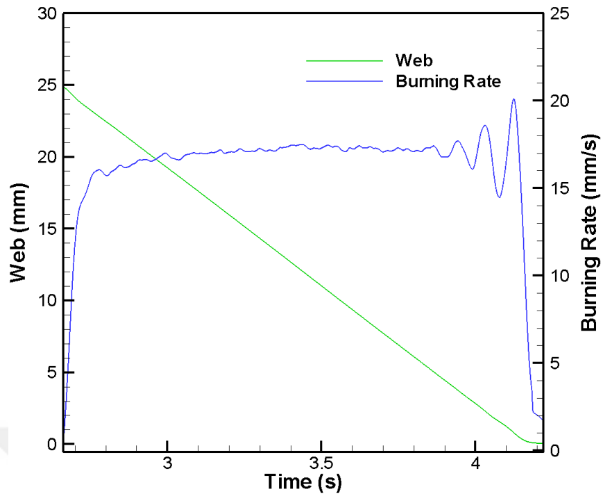
Figure 79 Burning rate and web thickness with respect to time for test 1
