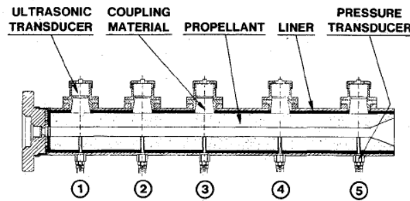
Figure 17 Axisymmetric motor without nozzle that was used in [1]
