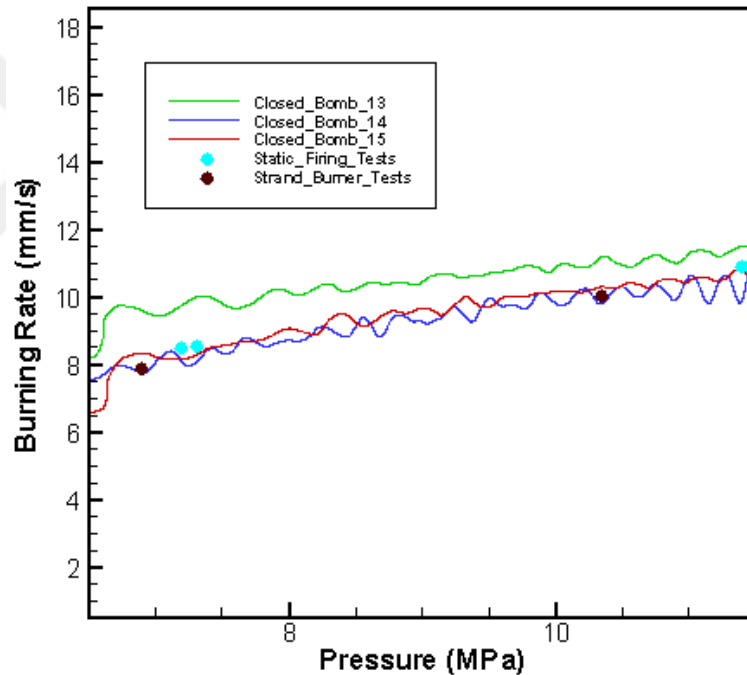
Figure 58 Burning Rate Value versus pressure that belongs to HSTYPE3
