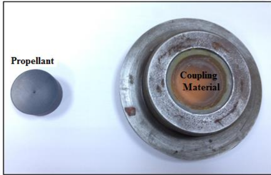
Figure 40 Propellant sample and propellant holder with coupling material
