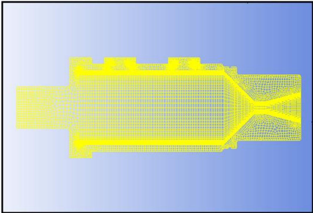
Figure 94 Mesh view of subscale test motor
