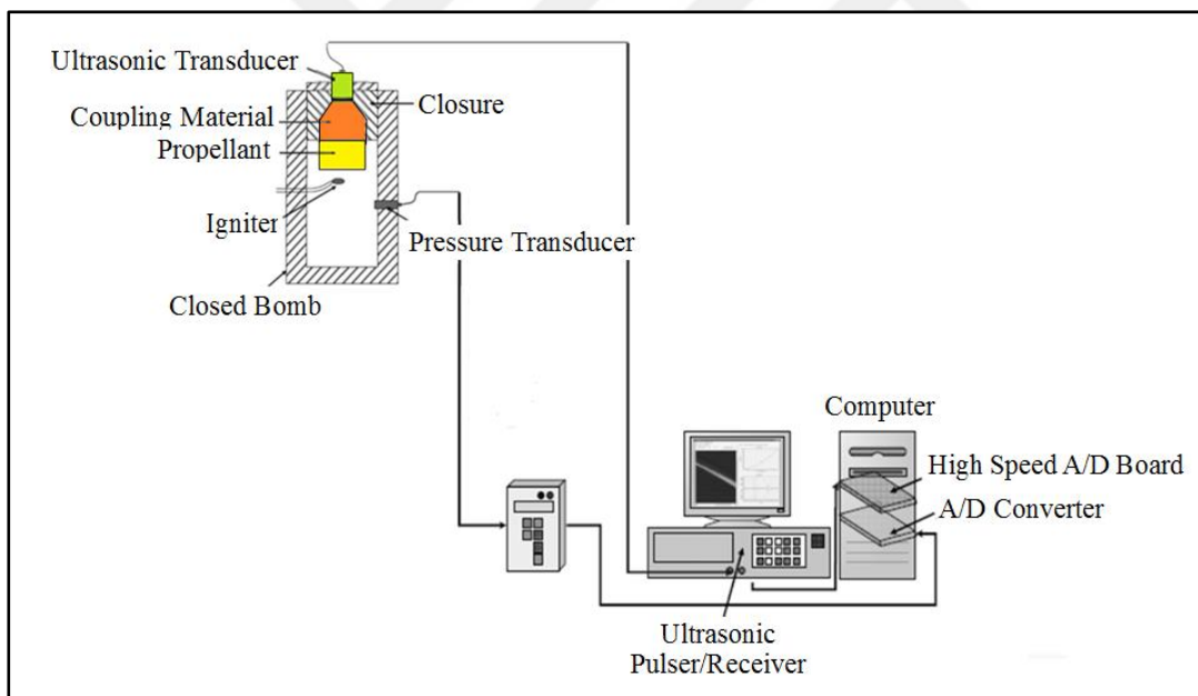
Figure 28 Schematic figure of the test setup components modified from [27]
