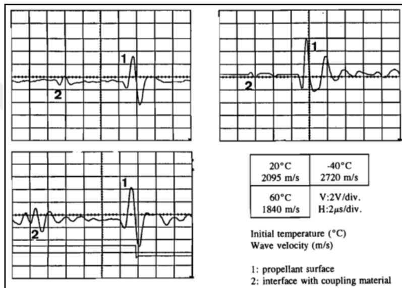
Figure 12 Ultrasonic echoes for various material temperatures belong to homogeneous propellant[14]
