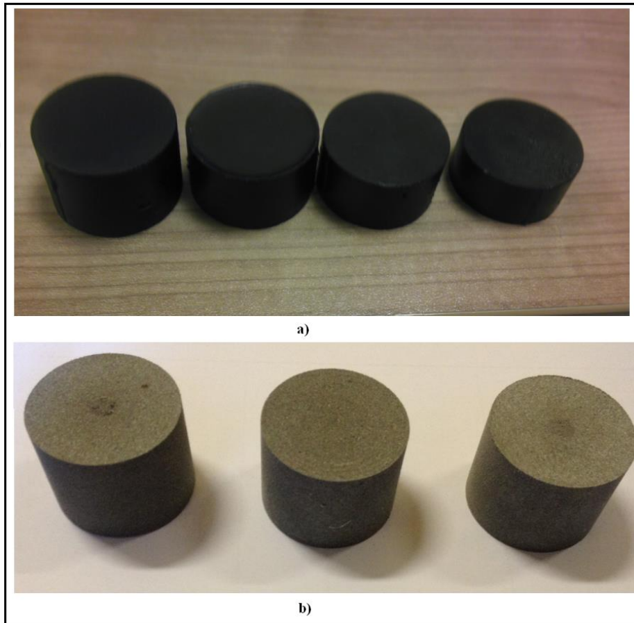
Figure 35 Propellant samples which have (a) different lengths b) same lengths
