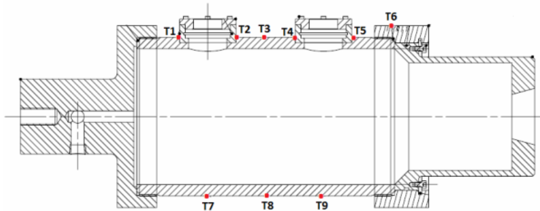
Figure 97 Termocouples places belong to test 3
