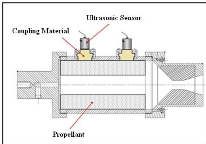
Figure 73 Technical Drawing of Test Motor
