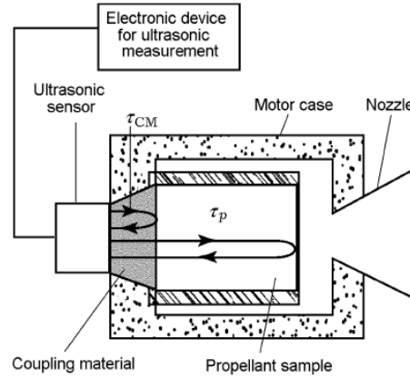
Figure 14 Ultrasonic demonstration for round trip method [23]
