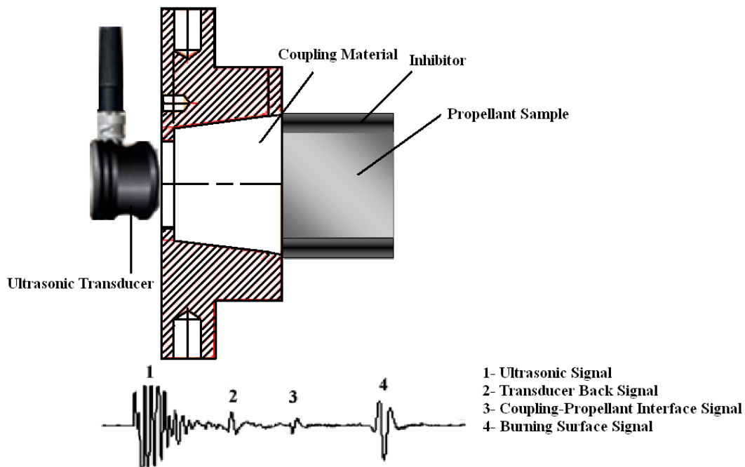
Figure 9 Schematic representation of ultrasonic measurement and example of a waveform
