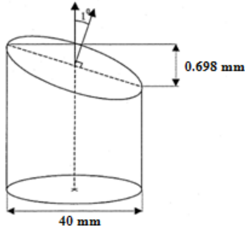
Figure 121 Non-perpendicularity of the propellant sample
