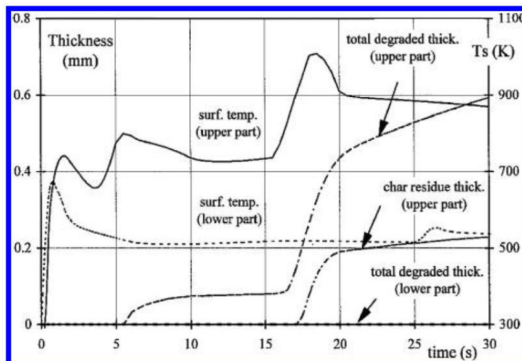
Figure 25 Measured surface temperature and Degraded thickness with respect to time [30]
