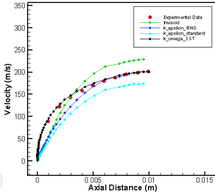
Figure 91 Velocity profile at location 0.401 m
