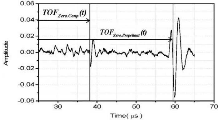
Figure 10 Zero Crossing Method [35]
