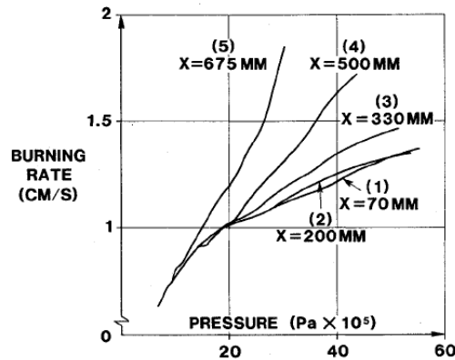
Figure 18 Test results for the axisymmetric motor test [1]
