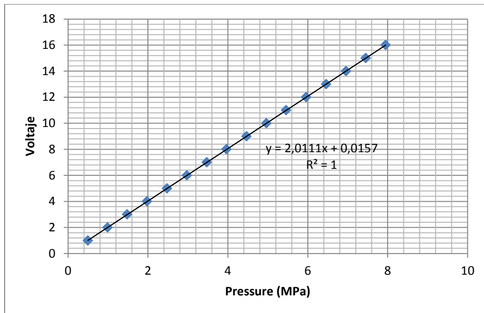
Figure 122 Calibration curve of pressure sensor
