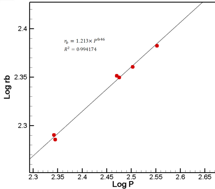
Figure 2 Example of evaluation of pressure exponent
