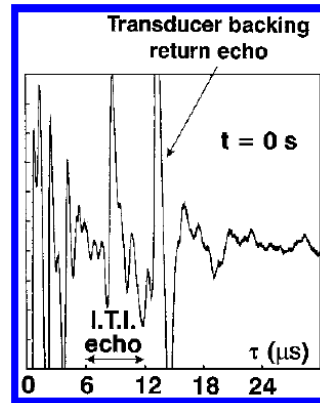
Figure 24 Ultrasound wave which reflects from insulation degradation surface [30]
