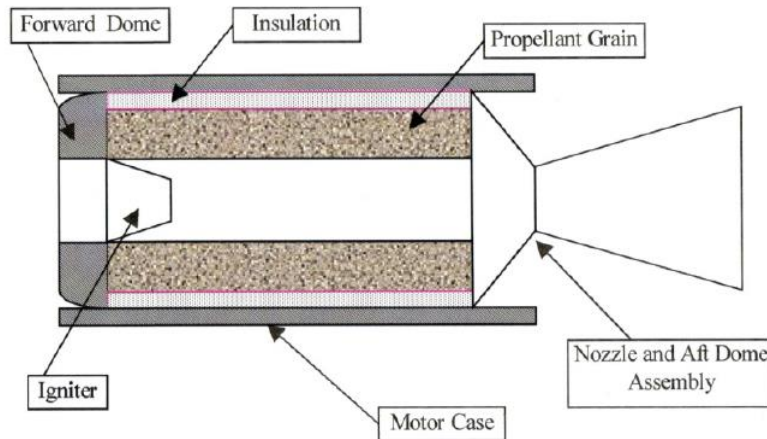
Figure 1 Basic representation of a rocket motor [12]
