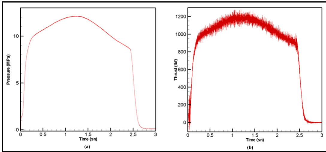
Figure 6 a) Pressure and b) Thrust curves gathered by a static firing test in Roketsan
