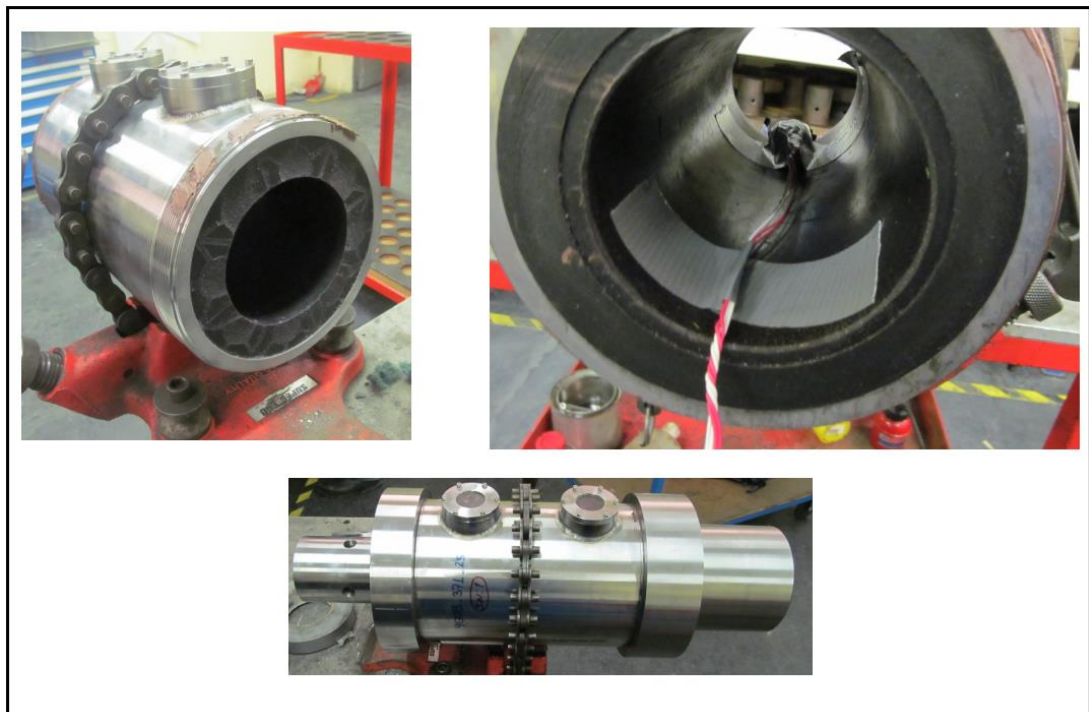
Figure 75 Assembly process of the test motor
