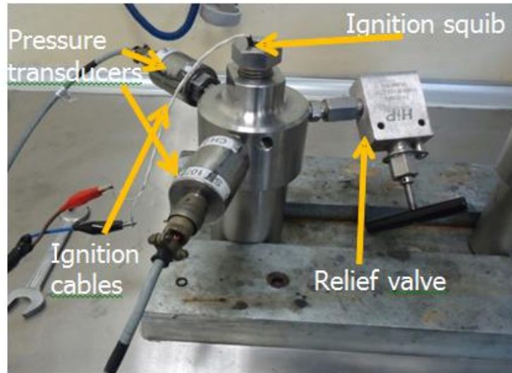
Figure 7 Closed Bomb that is used in Roketsan
