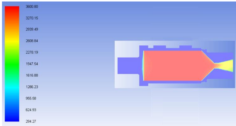
Figure 99 Temperature (Kelvin) distribution on test motor obtained from numerical analysis
