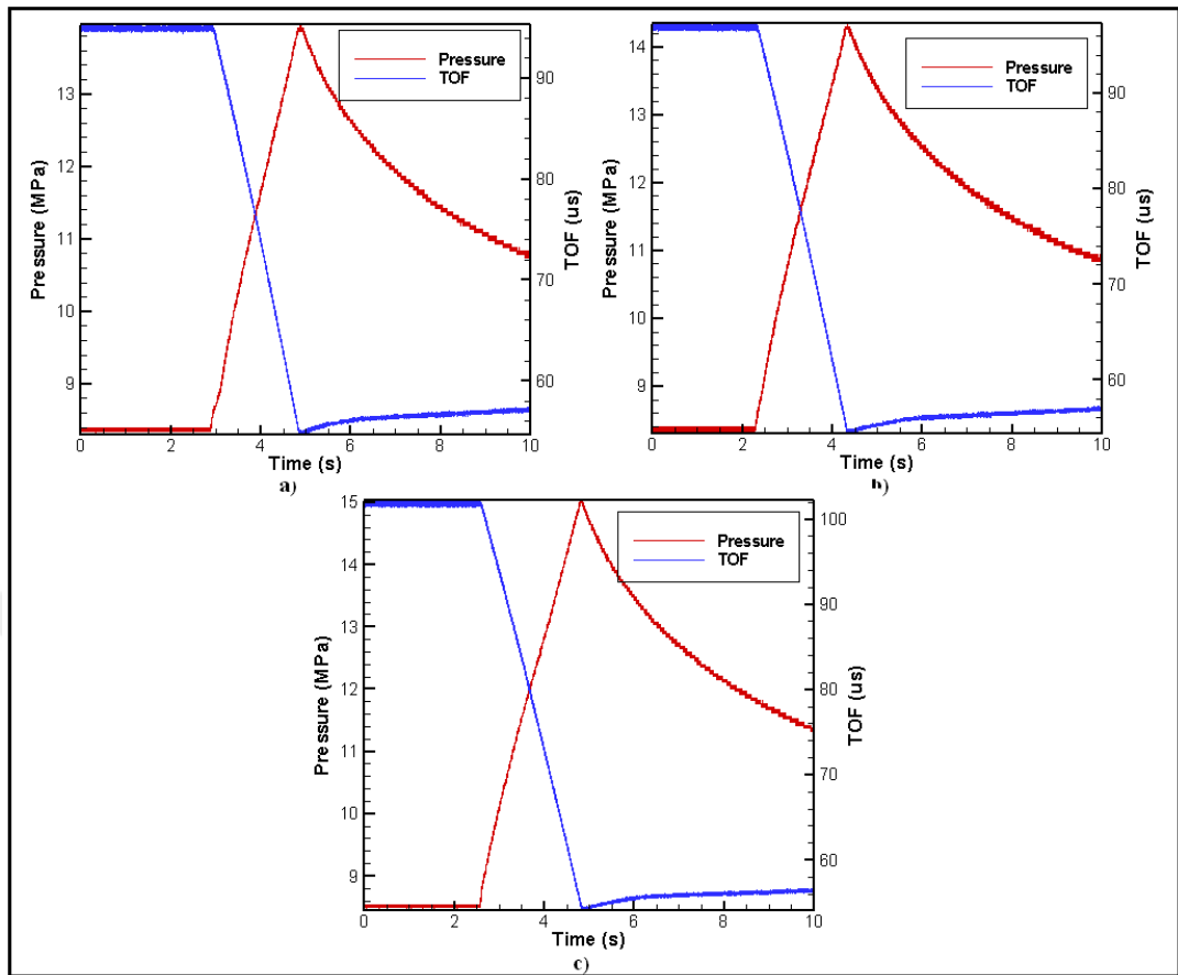
Figure 65 Measured pressure and time of flight versus time for a) Test 25 b) Test 26 c) Test 27
