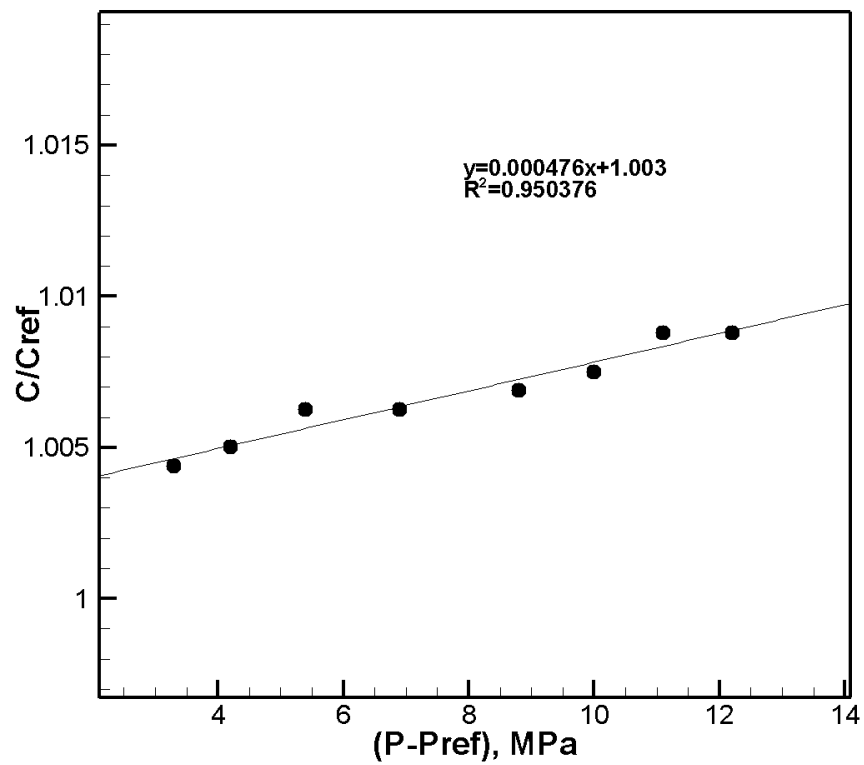
Figure 112 Wave velocity variation with pressure for coupling material
