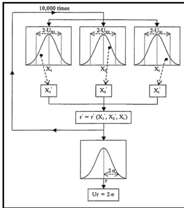
Figure 101 Direct Monte Carlo Simulation Diagram used in uncertainty Measurement [33]
