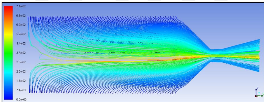
Figure 100 Alumina particles distribution in test motor
