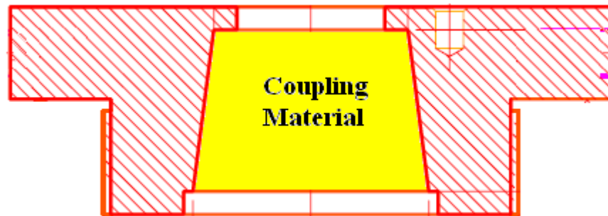
Figure 34 (a) Schematic view of the coupling material placed in propellant sample holder
