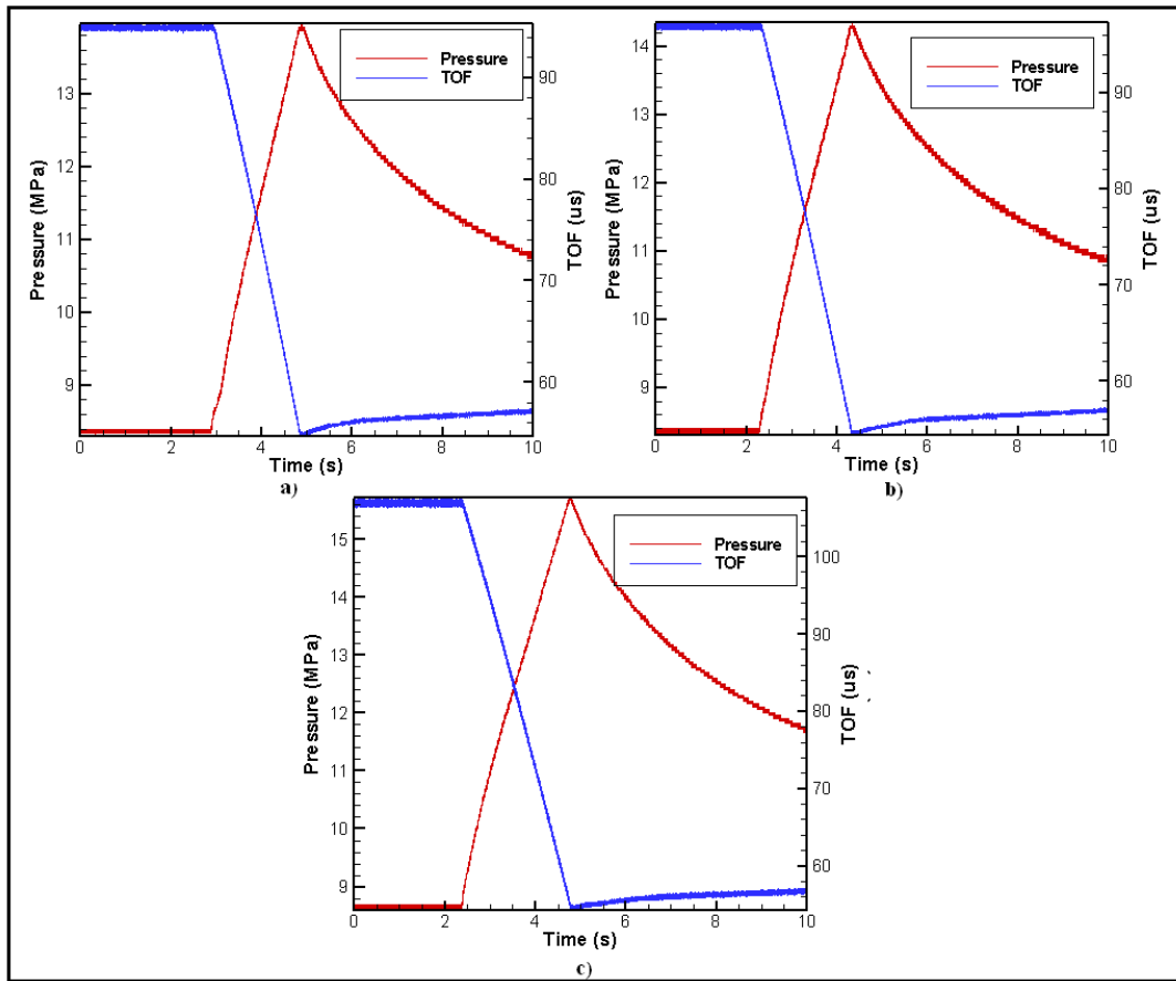
Figure 66 Measured pressure and time of flight versus time for a) Test 28 b) Test 29 c) Test 30
