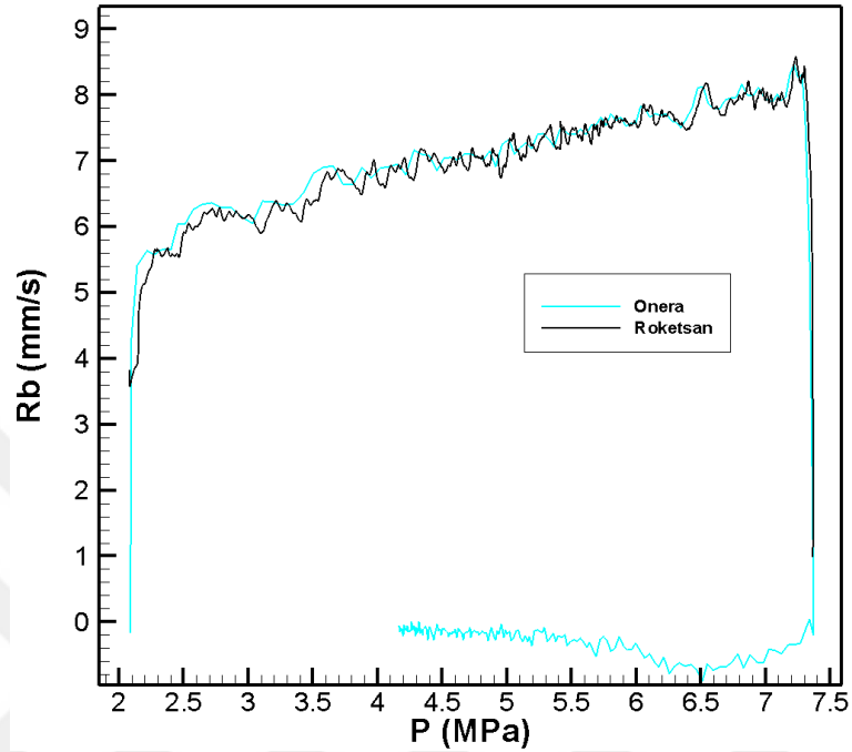
Figure 107 Burning rate results of test case 3
