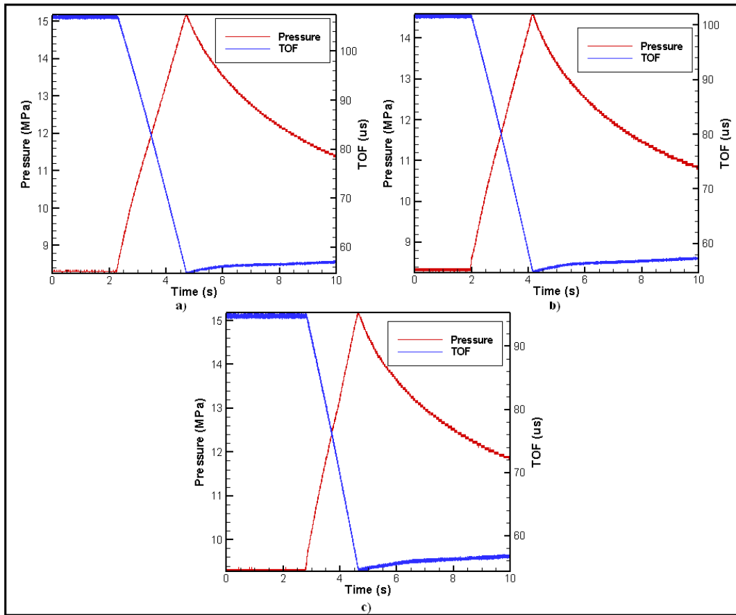
Figure 64 Measured pressure and time of flight for a) Test 22 b) Test 23 c) Test 24
