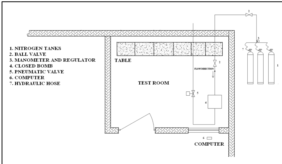
Figure 27 Layout of the Test Setup
