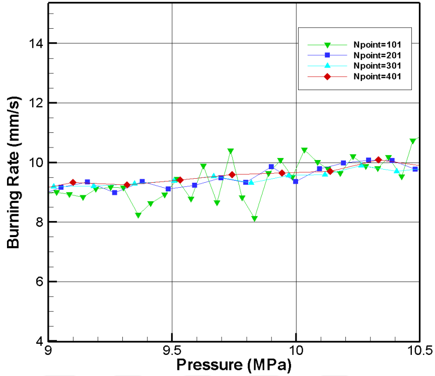
Figure 67 Effect of Npoint on burning rate evaluation
