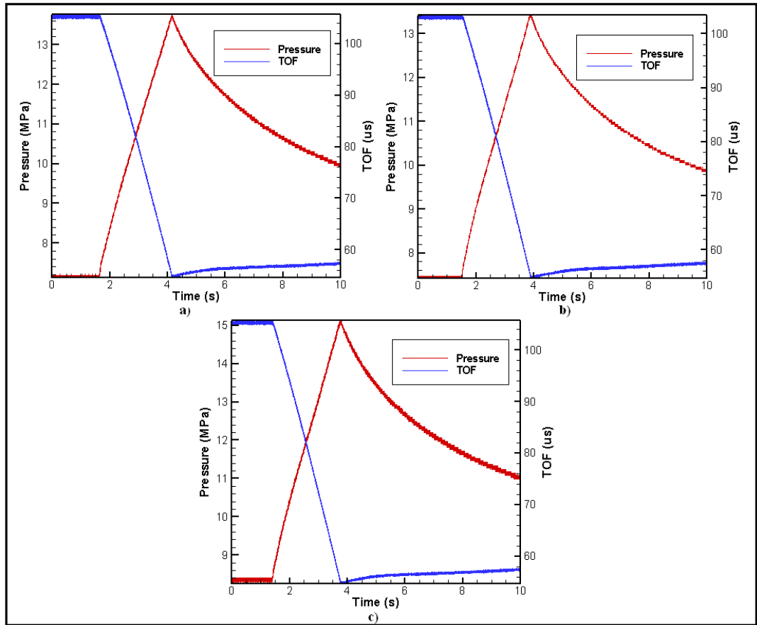
Figure 63 Measured pressure and time of flight versus time for a) Test 19 b) Test 20 c) Test 21
