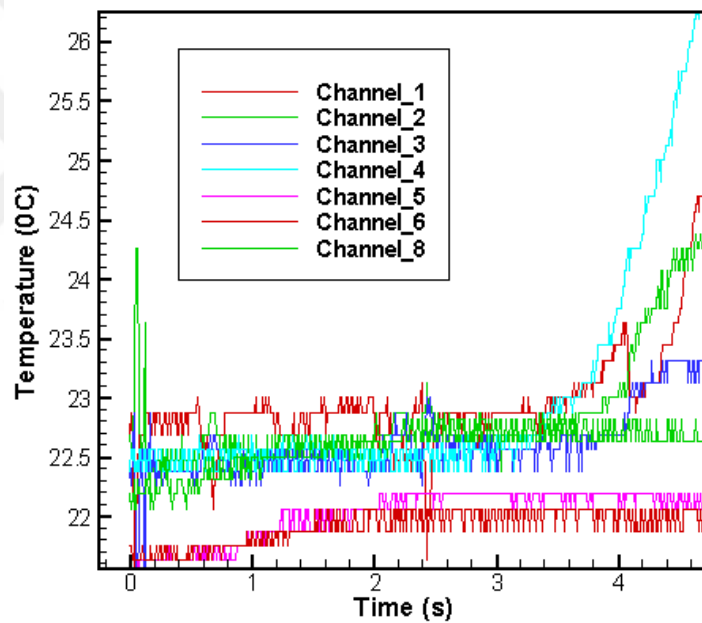
Figure 98 Temperature distribution on test motor obtained by thermocouples
