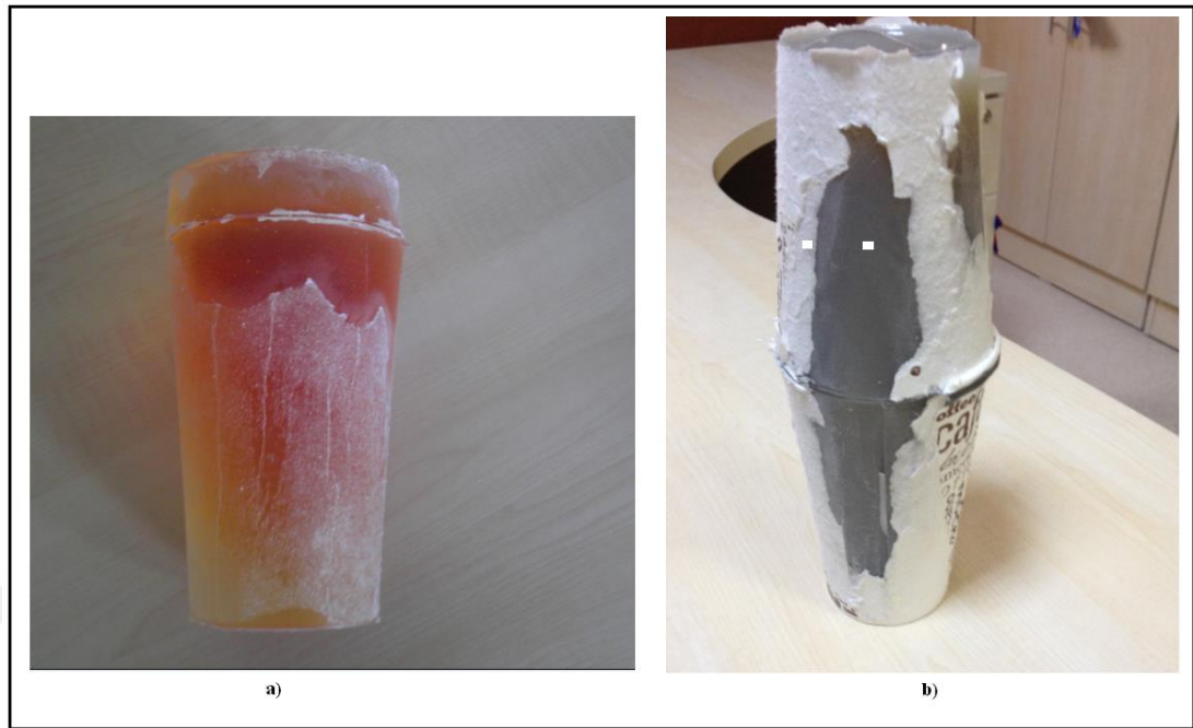
Figure 33 (a) a whole coupling material used for non-aluminized propellants (b) a whole coupling material used for aluminized propellants
