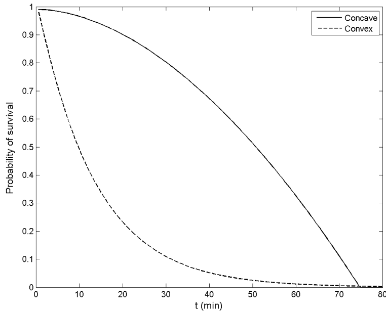
Figure 6.3: Survival Functions
