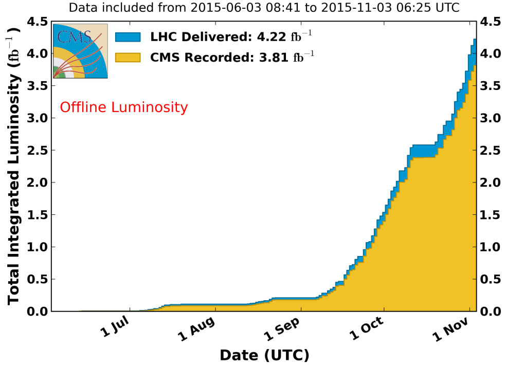
Figure 5.12 : CMS integrated luminosity between June 2015 and November 2015. Before June 2015 there is no beam [29].
