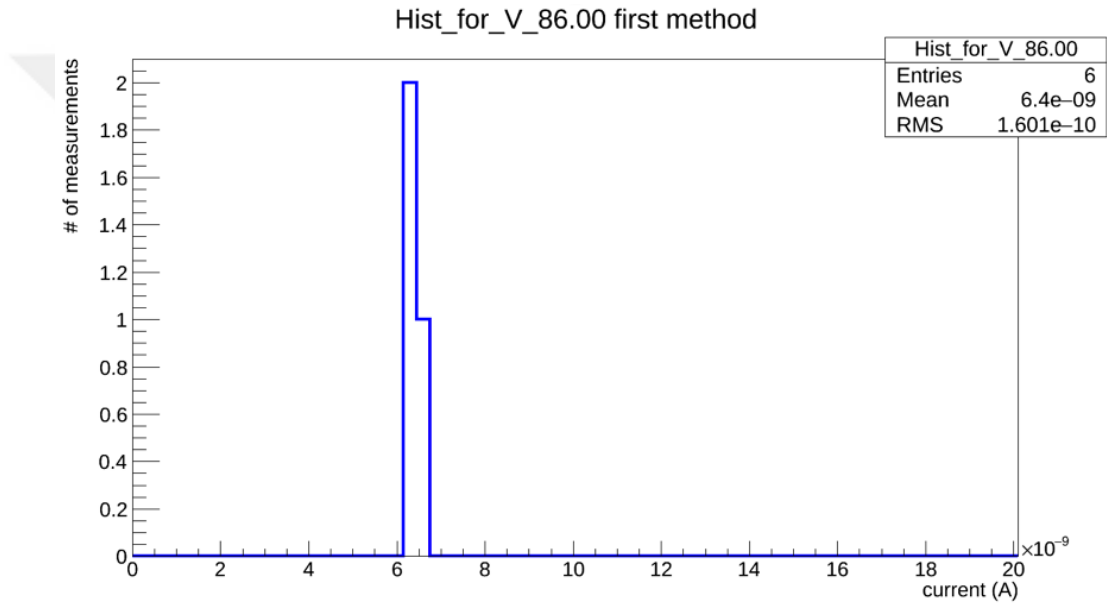
Figure 5.10 : Histogram for V = 86V with first method. There are only six entries since there is only six measurements.
