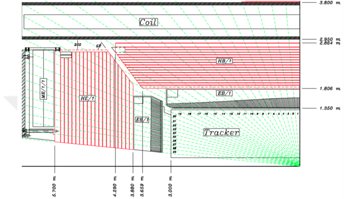
Figure 4.2 : Quarter view of the barrel and endcap hadron calorimeters, showing the intrinsic longitudinal segmentation capabilities. The front-end readout electronics, the readout boxes or “RBX”, are located directly behind tower 15 in the barrel and directly behind tower 18 in the endcap [26].
