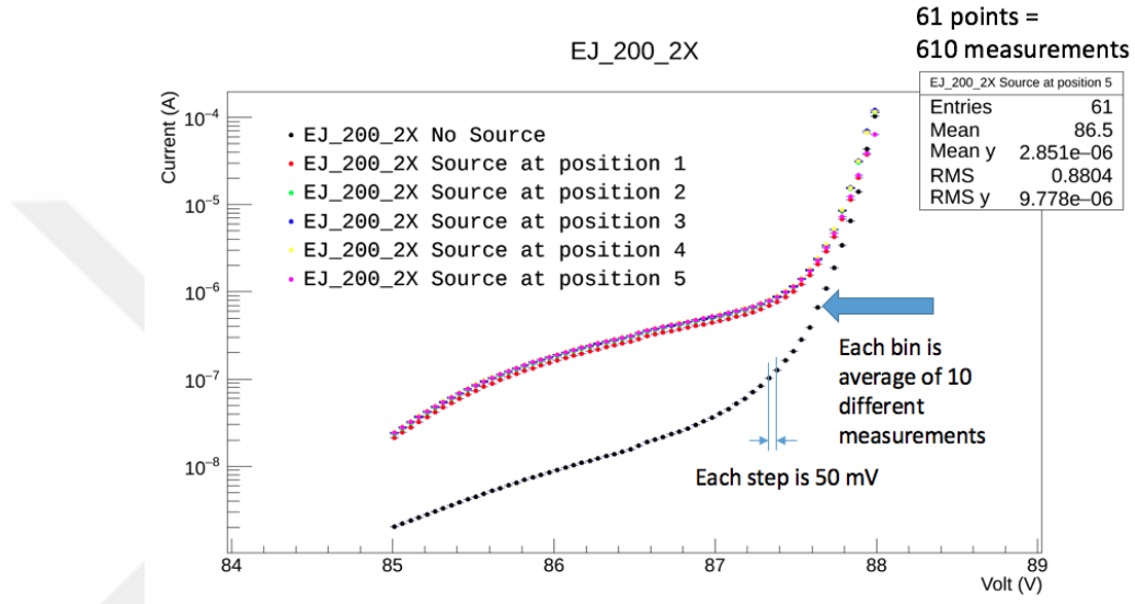
Figure 5.6 : An I - V of a measurement of EJ_200_2X scintillator with 5 different source and a background measurements. Measurement step is 50mV and each point is the mean of 10 different measurements.
