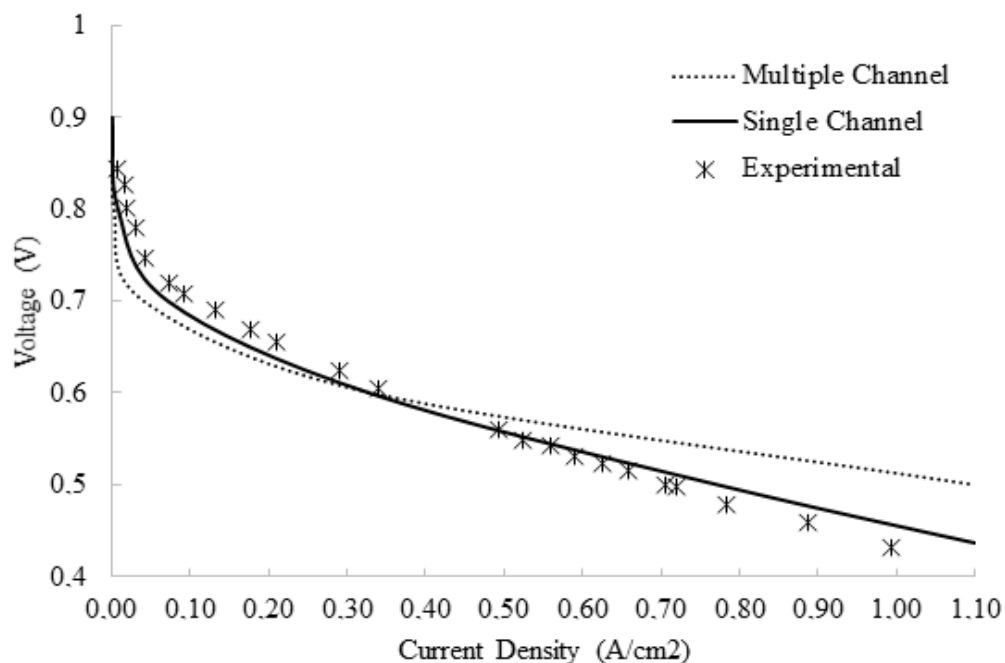
Figure 4.3 Comparison of single flow channel and triple mixed serpentine flow channel models with experimental data at 160 °C
