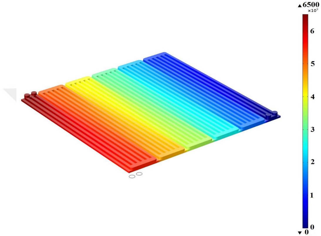
Figure 6.4 Pressure drop along the cathode flow channels with inlet reactant temperature of 165 °C and 0.6 V (Pa)
