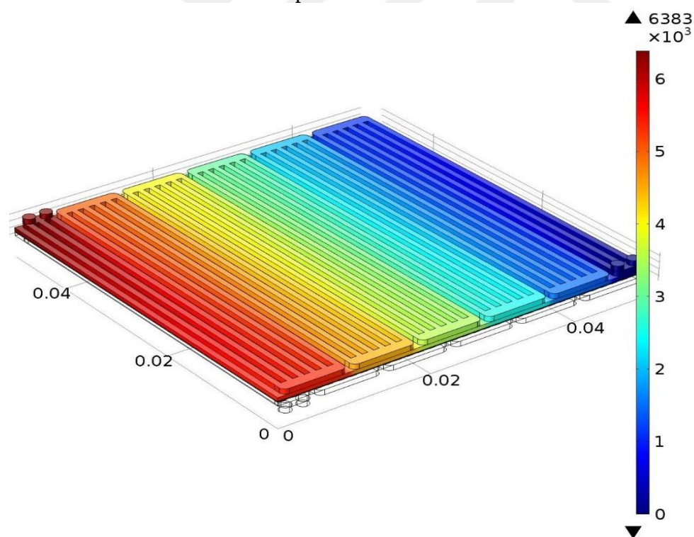
Figure 5.5 Pressure profile along cathode flow channels at V=0.6 V and 1.2 bar backpressure at 165 °C
