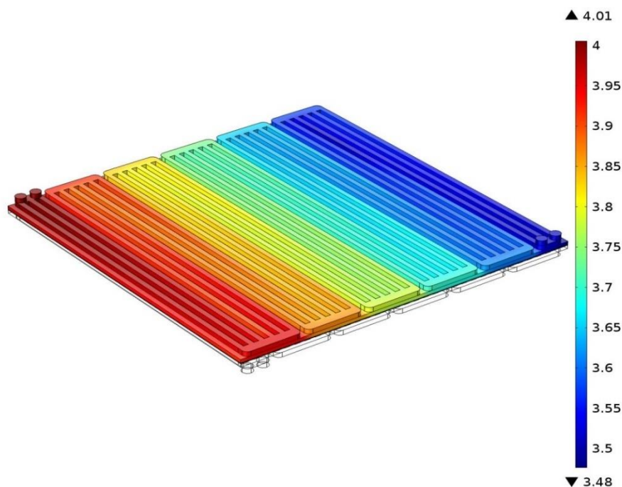
Figure 5.13 Oxygen concentration along cathode flow channels at 0.8 V and 1.2 bar backpressure ( \text{mol m}^{-3} )
