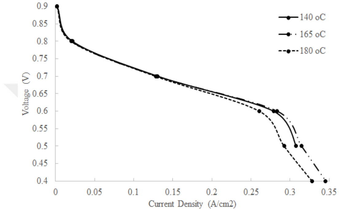
Figure 5.3 Polarization curve of models obtained for different operation temperatures for triple mixed serpentine models at 1.2 bar
