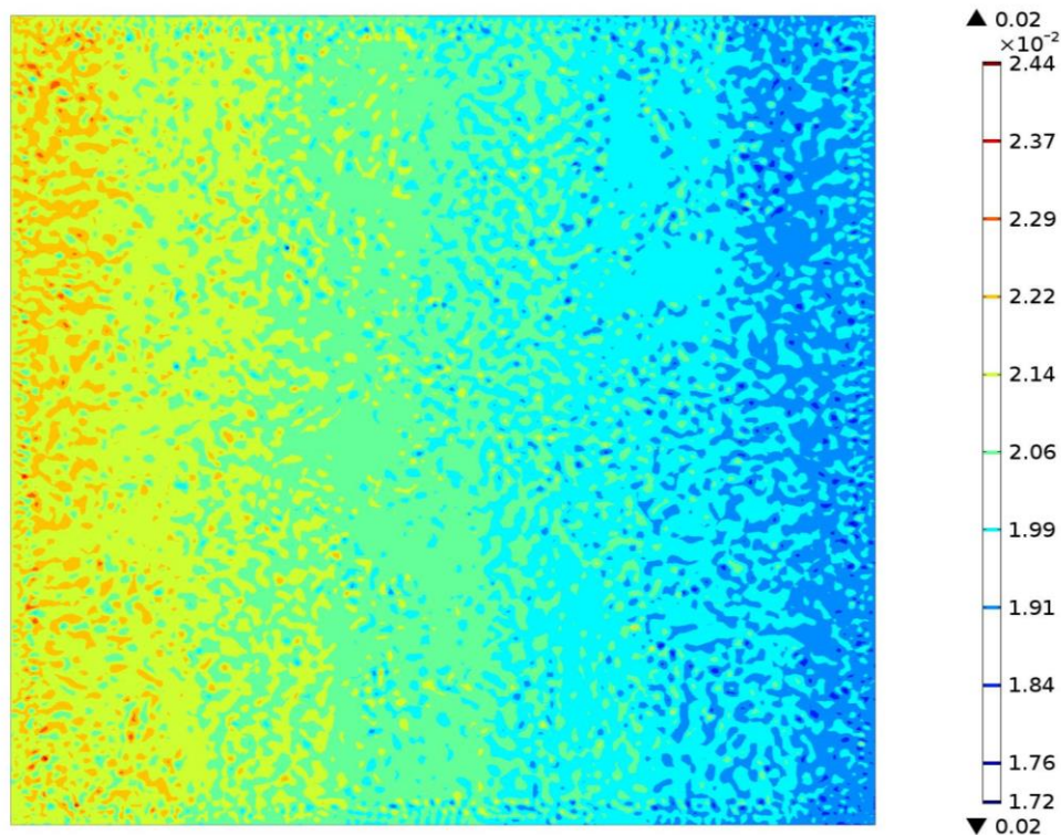
Figure 5.16 Membrane current density distribution at 165 °C, 1.2 bar and 0.8 V ( \text{A cm}^{-2} )
