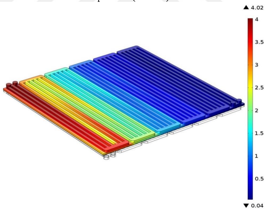
Figure 5.12 Oxygen concentration along cathode flow channels at 0.6 V and 1.2 bar backpressure ( \text{mol m}^{-3} )
