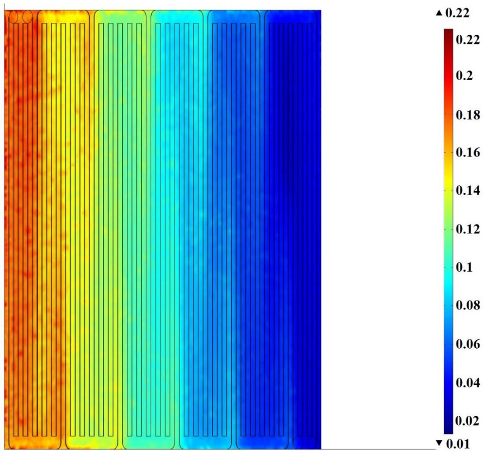
Figure 6.5 Membrane current density distribution at 0.6 V with inlet reactant temperature of 165 °C (A cm -2 )
