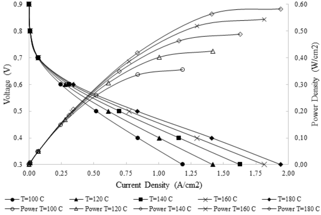
Figure 4.2 Simulated polarization curve of a single HTPeMFC obtained at different operating temperatures from single flow channel.
