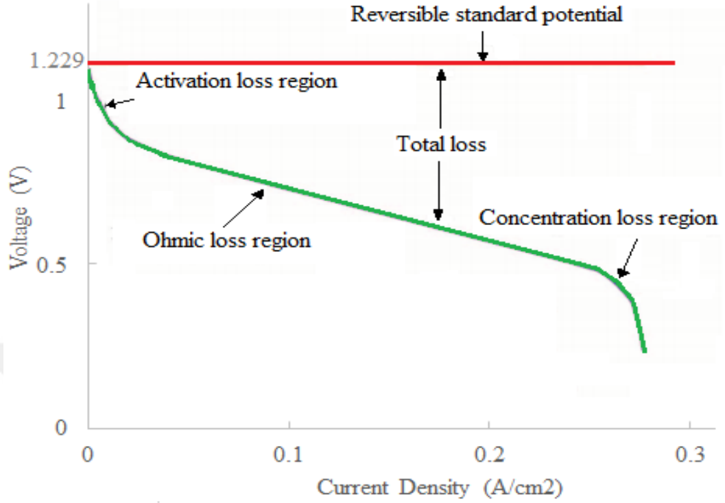
Figure 2.2 Polarization curve of a HT-PEMFC with various losses
