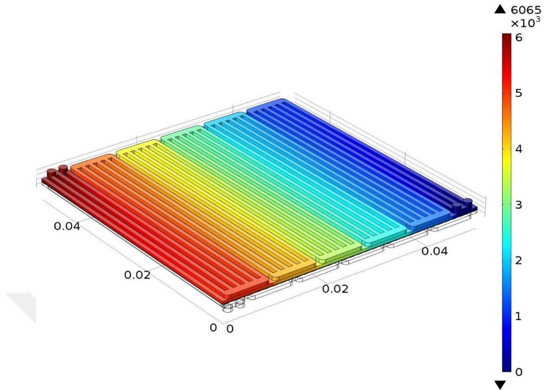
Figure 5.6 Pressure profile along cathode flow channels at V=0.6 V and 1.2 bar backpressure at 180 °C
