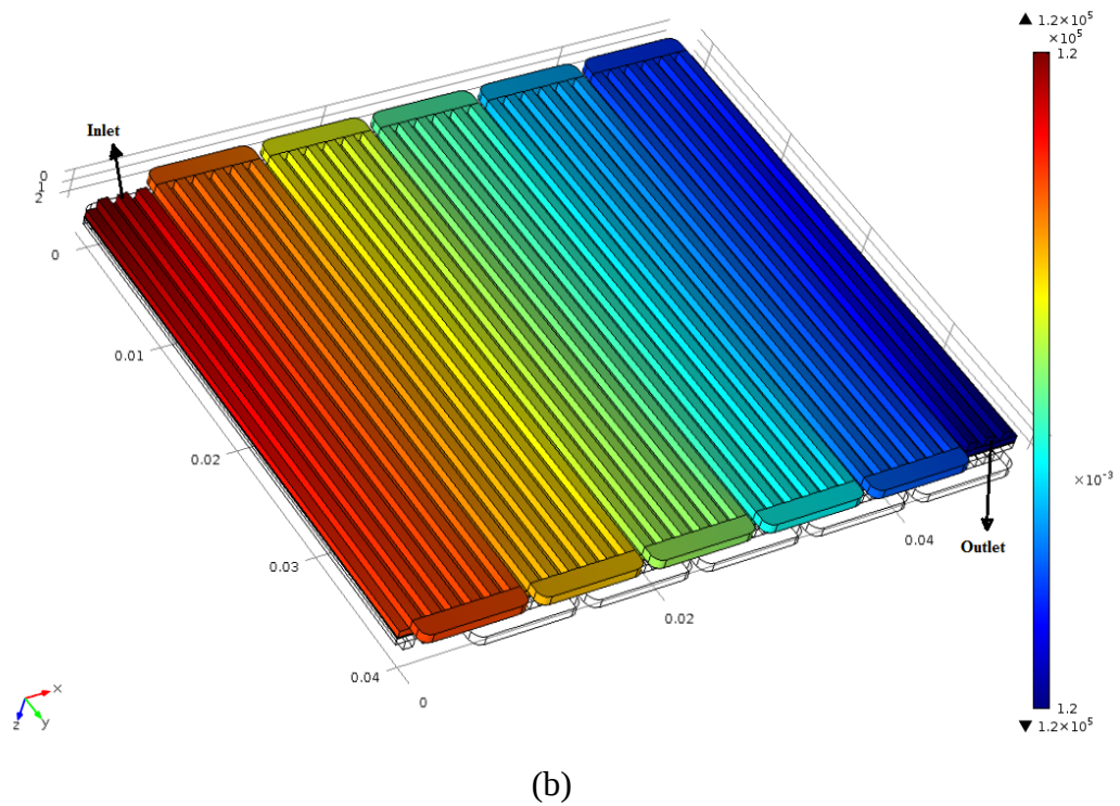
Figure 4.5 Pressure distribution at the flow channels at 160 °C and operating voltage of 0.6 V (a) cathode (1950 Pa pressure drop), (b) anode (100 Pa pressure drop)
