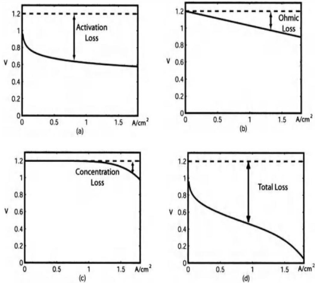
Figure 2.3 Voltage drops caused by different types of losses in fuel cell: (a) activation losses only; (b) ohmic losses only; (c) concentration losses only; (d) total losses[3]
