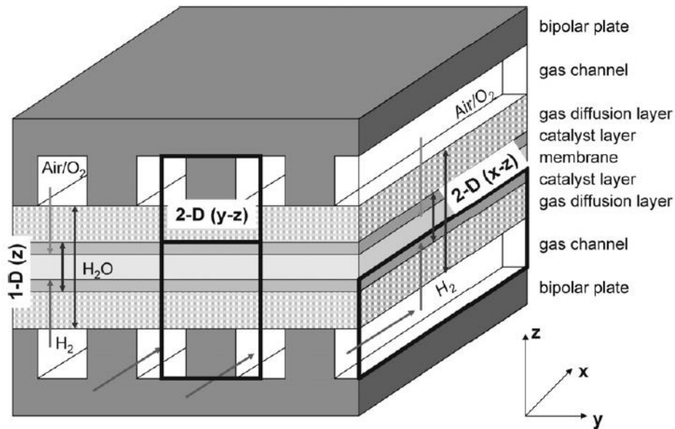
Figure 2.7 Model domains used in 1D and 2D models of HT-PEMFC [2]
