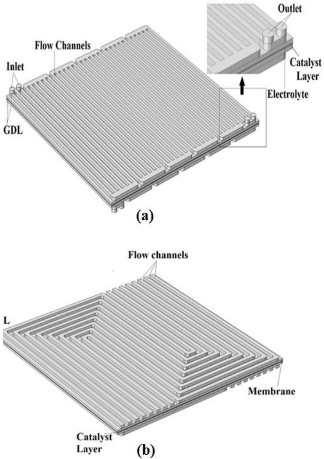
Figure 3.1 Isothermal model domains (a) triple mixed serpentine (b) serpentine
