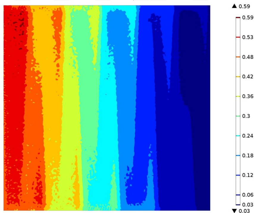
Figure 5.15 Membrane current density distribution at 165 °C, 1.2 bar and 0.6 V ( \text{A cm}^{-2} )
