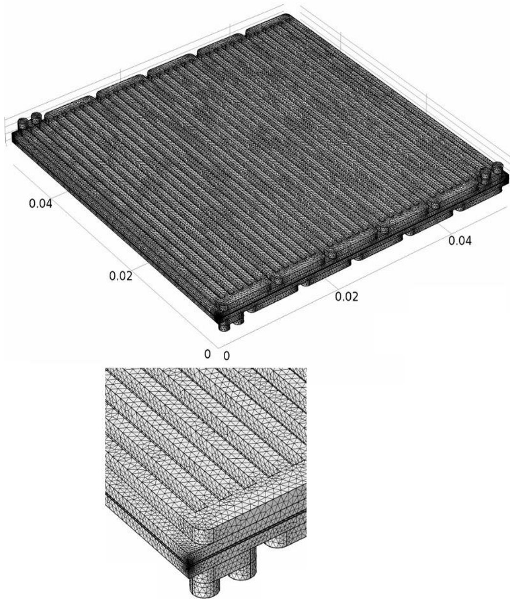
Figure D.1 Meshed computational domain for triple mixed serpentine model
