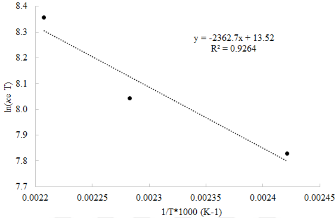
Figure 5.1 Temperature dependence of proton conductivity
