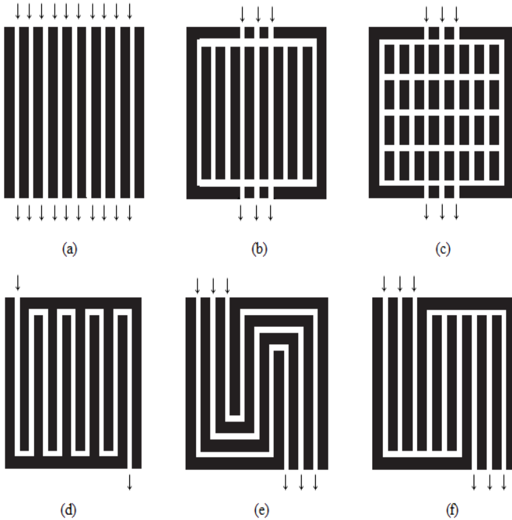
Figure 2.4 Flow Field Configurations used in Fuel Cells (a, b) Straight, (c) criss-cross, (d) single channel serpentine, (e) multichannel serpentine, (f) mixed serpentine [2]
