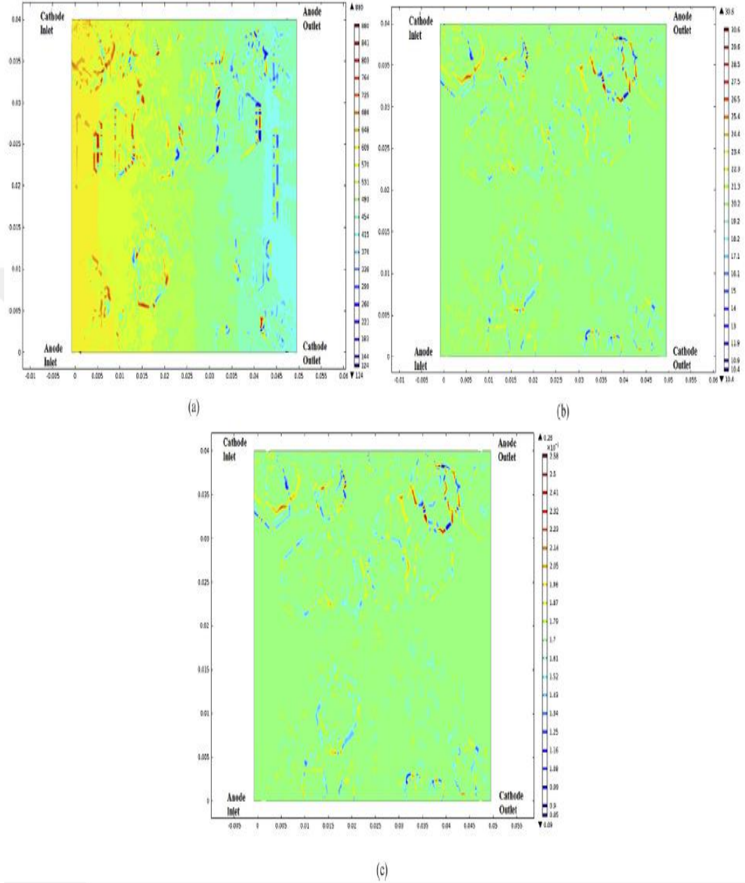
Figure 4.8 Predicted current density distribution at 160 °C operating temperature (a) V=0.5 V (b) V=0.7 V (c) V=0.9 V
