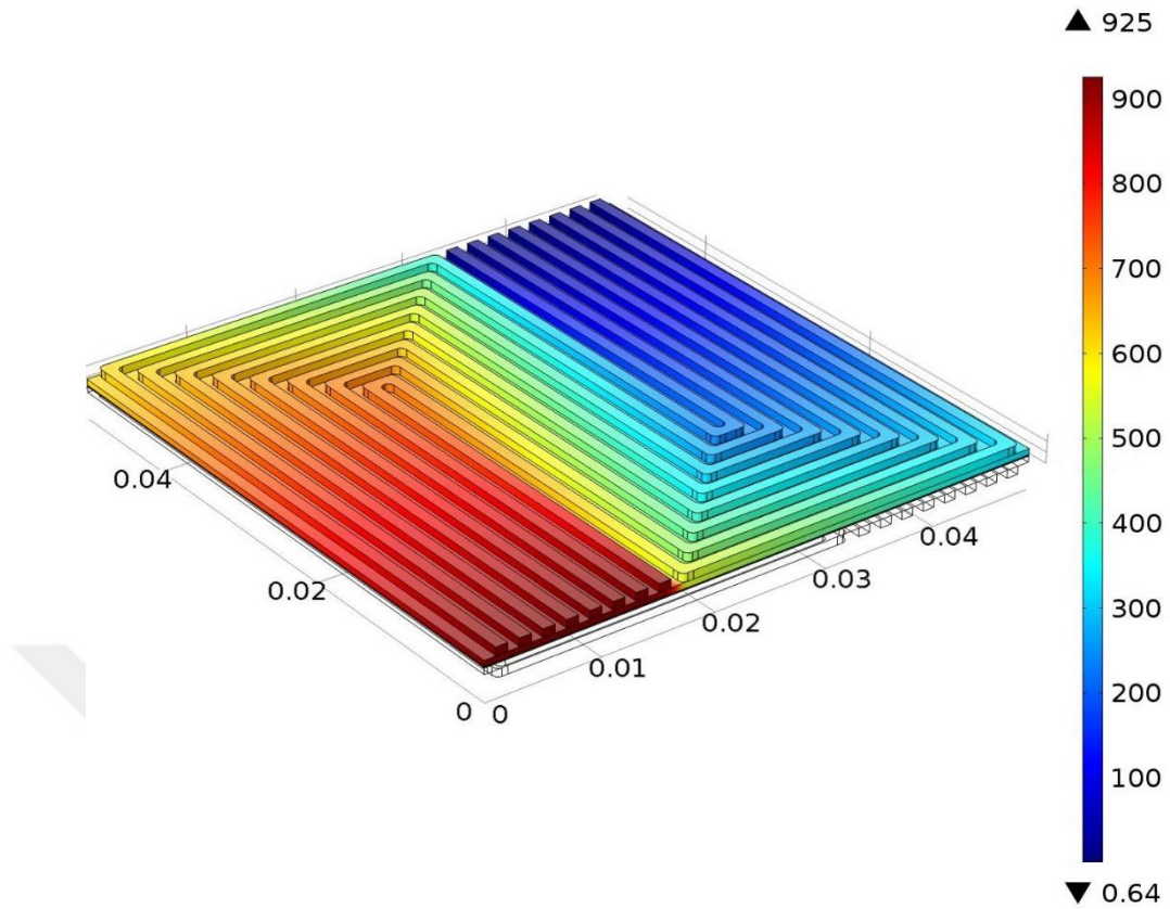
Figure 5.19 Pressure profile along cathode flow channel at 0.6 V and 165 °C for serpentine flow channel geometry (Pa)
