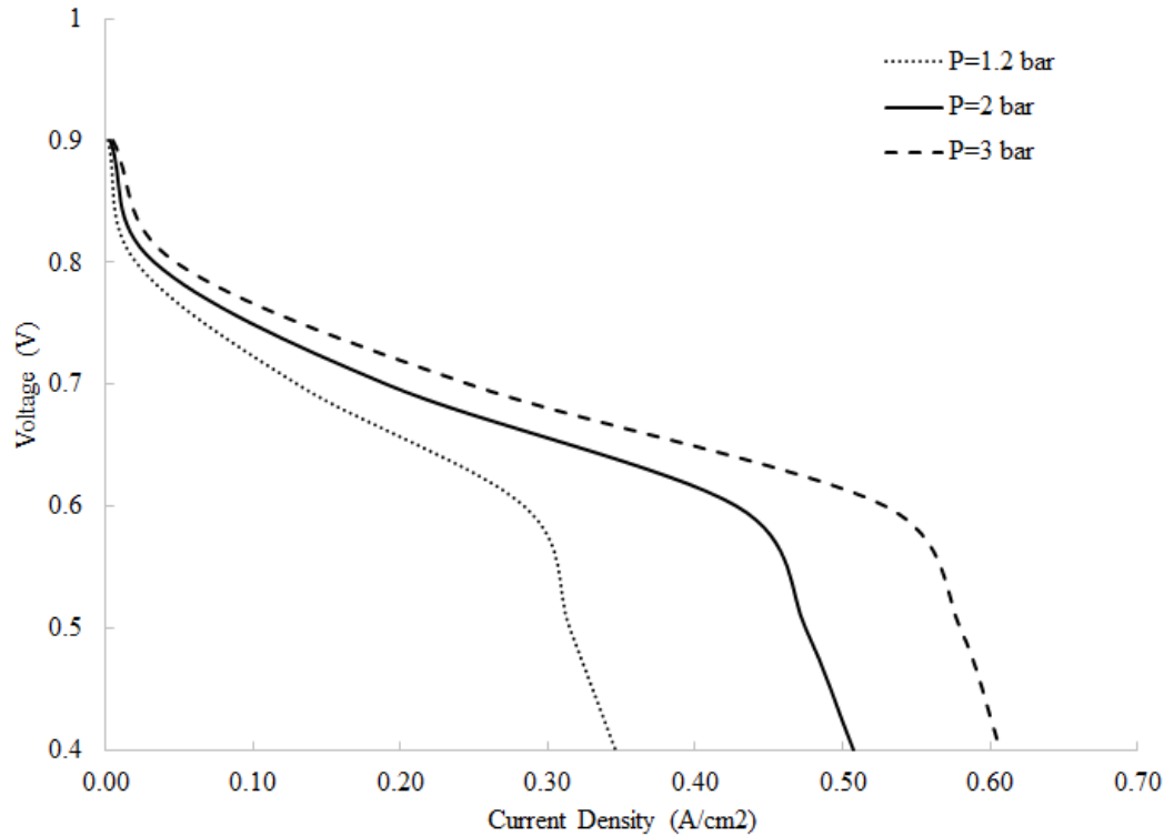
Figure 5.7 Polarization curve obtained at different operation pressures at 165 °C
