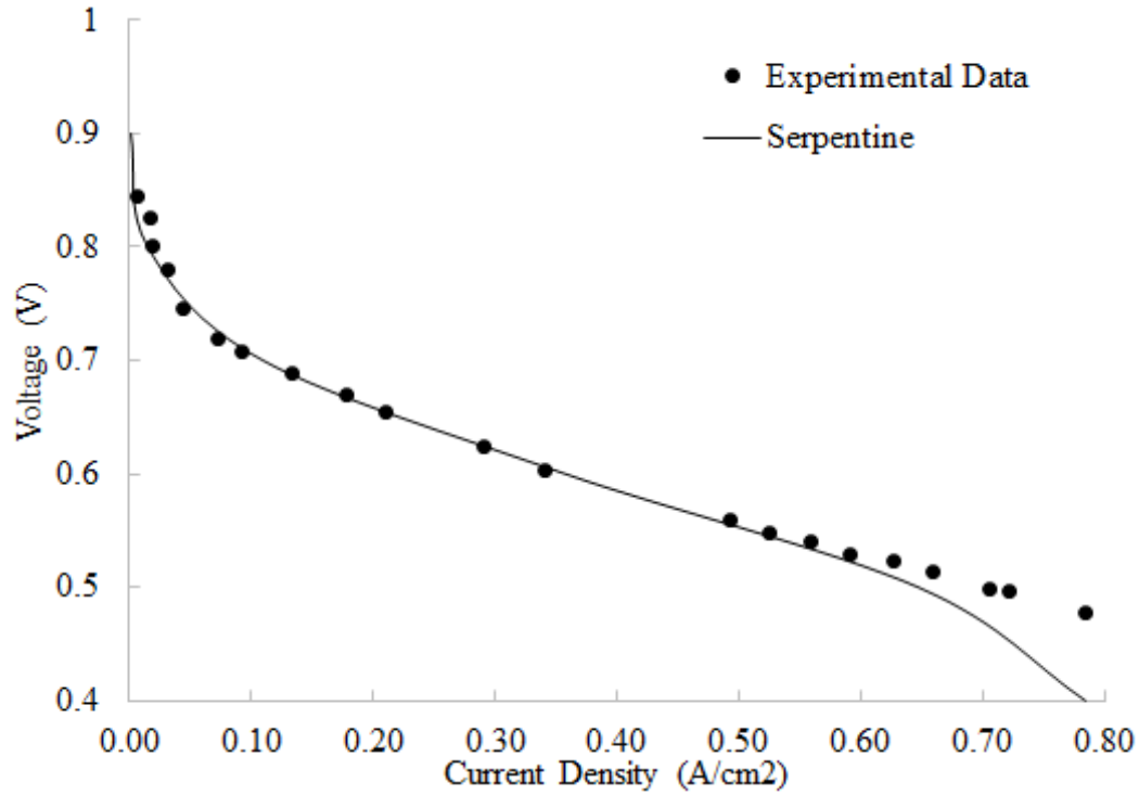
Figure 5.18 Comparison of serpentine model results with experimental data at 165 °C
