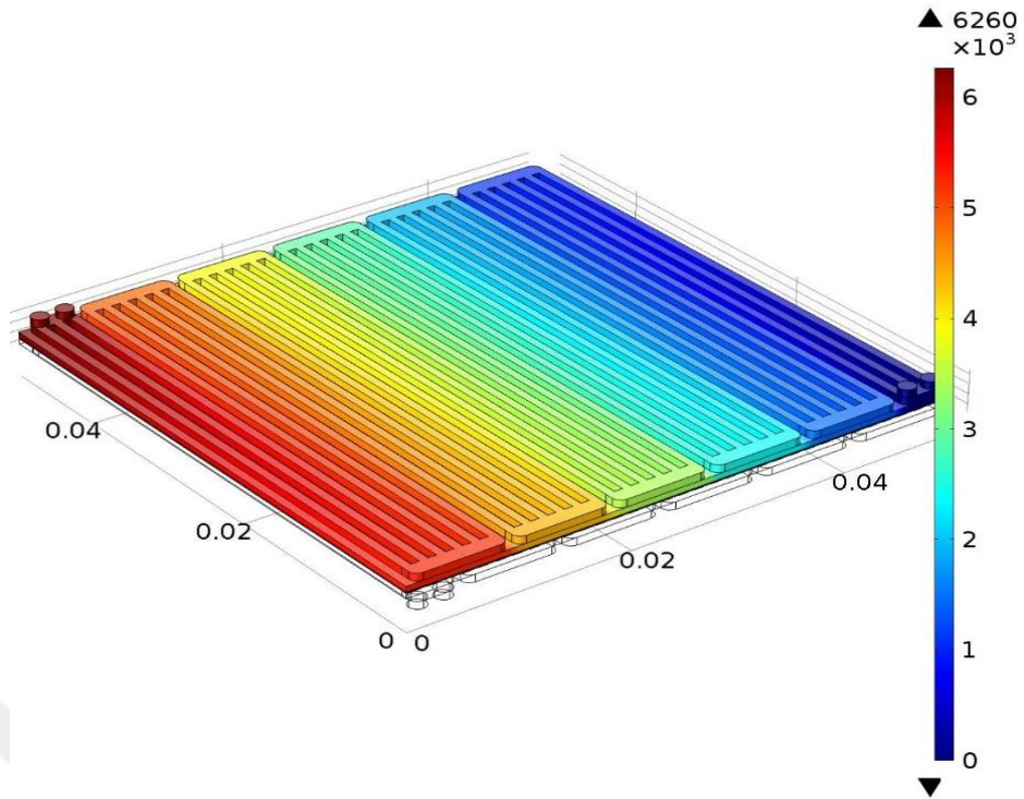
Figure 5.8 Pressure profile along the cathode flow channels at 165 °C, 0.8 V and 1.2 bar (absolute, Pa)
