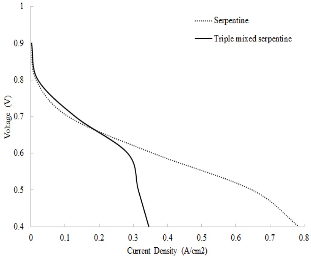
Figure 5.17 Polarization curve for triple mixed serpentine and serpentine models at 1.2 bar and 165 °C
