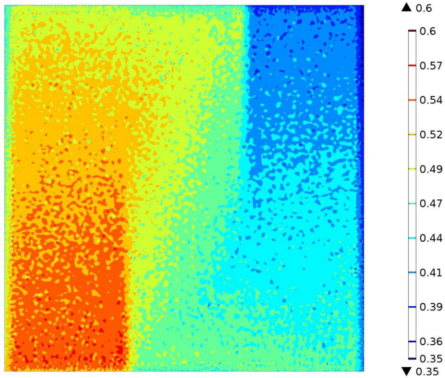
Figure 5.21 Membrane current density distribution at 165 °C and 0.6 V for serpentine flow channel geometry ( \text{A cm}^{-2} )
