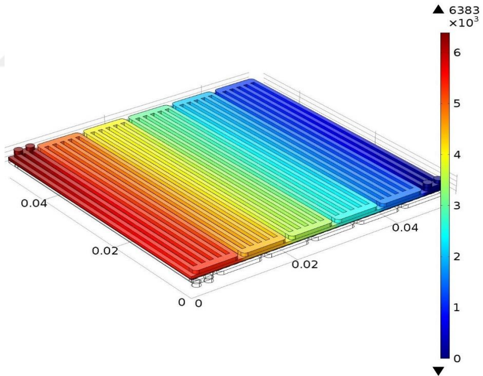
Figure 5.9 Pressure profile along the cathode flow channels at 165 °C, 0.6 V and 1.2 bar (absolute, Pa)
