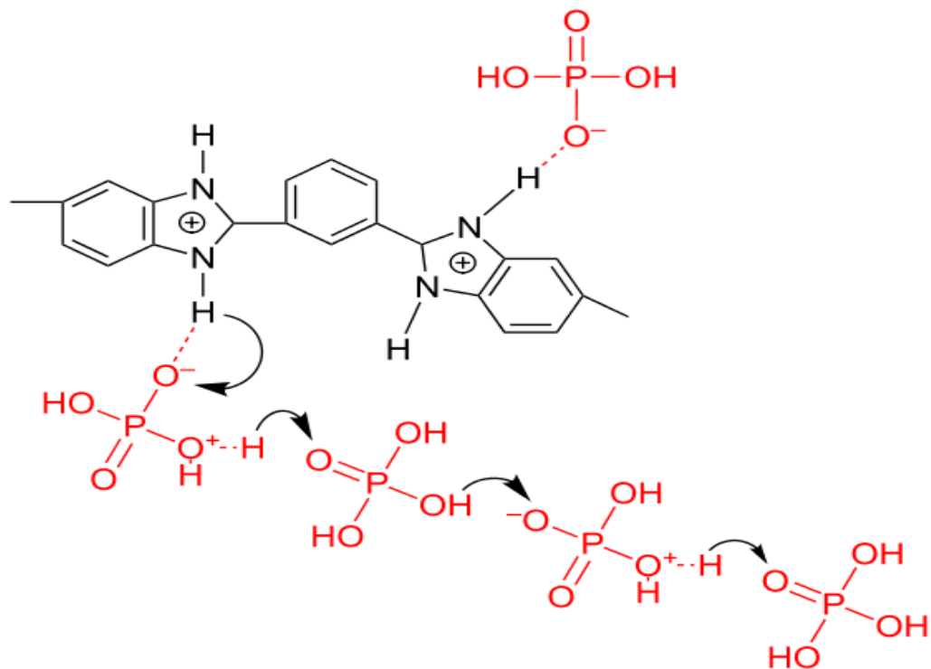
Figure 2.6 Interaction between phosphoric acid and PBI membrane for proton transfer [17]
