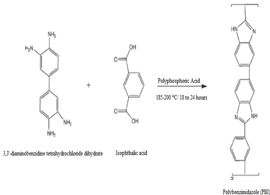
Figure 2.5 Synthesis of PBI membrane [7]
