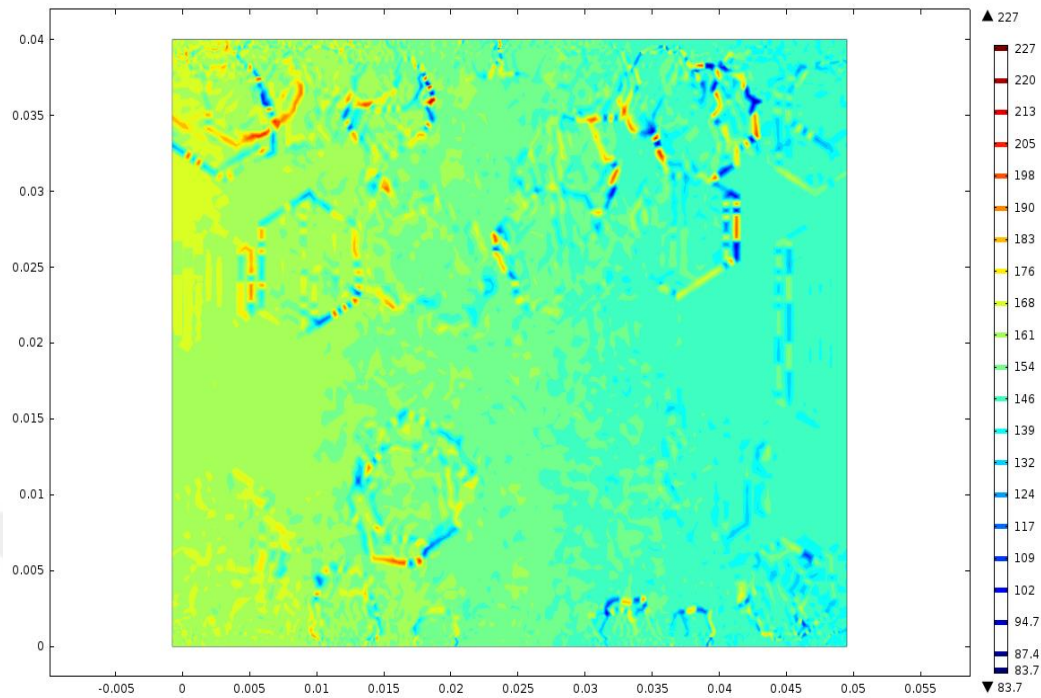
Figure 4.4 Predicted current density distribution at 160 °C and operating voltage of 0.6 V for triple mixed serpentine flow channel model
