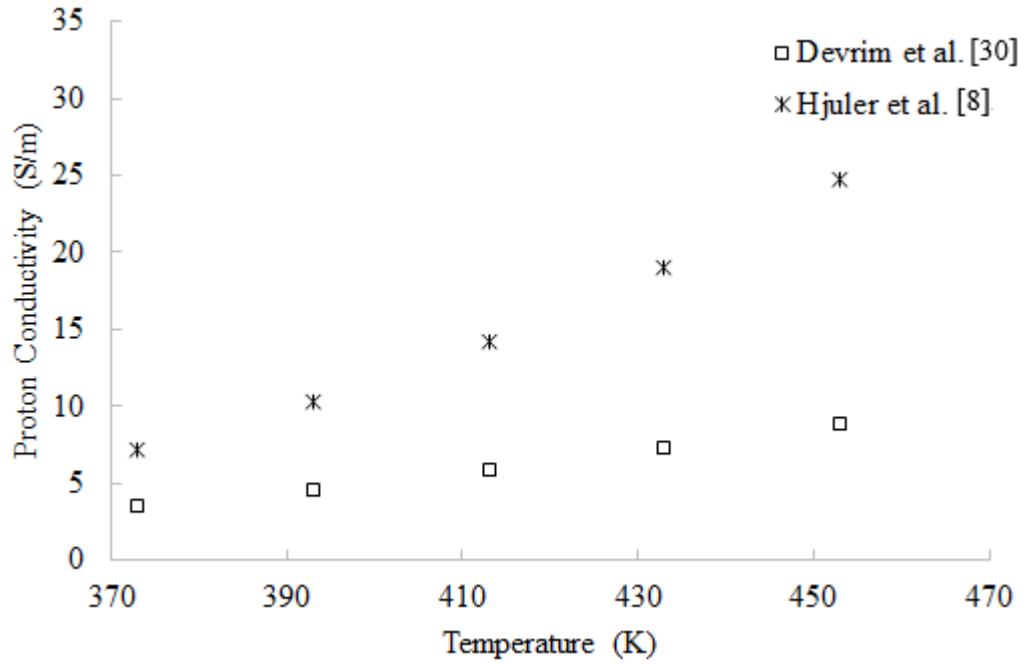
Figure 5.2 Proton conductivity of commercial and developing PBI membranes
