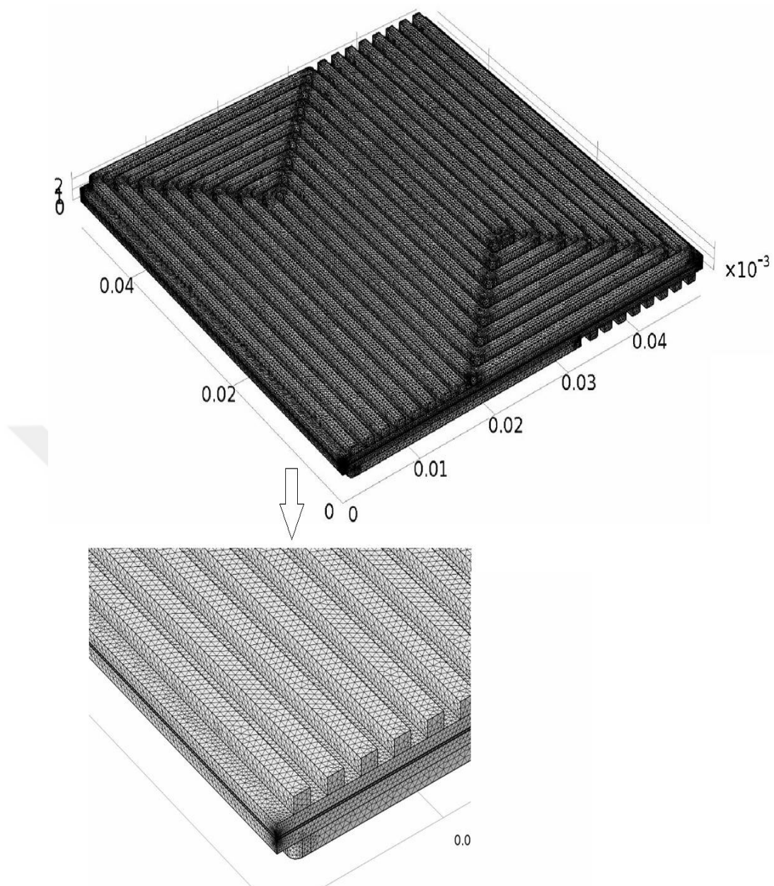
Figure D.2 Meshed computational domain for serpentine model
