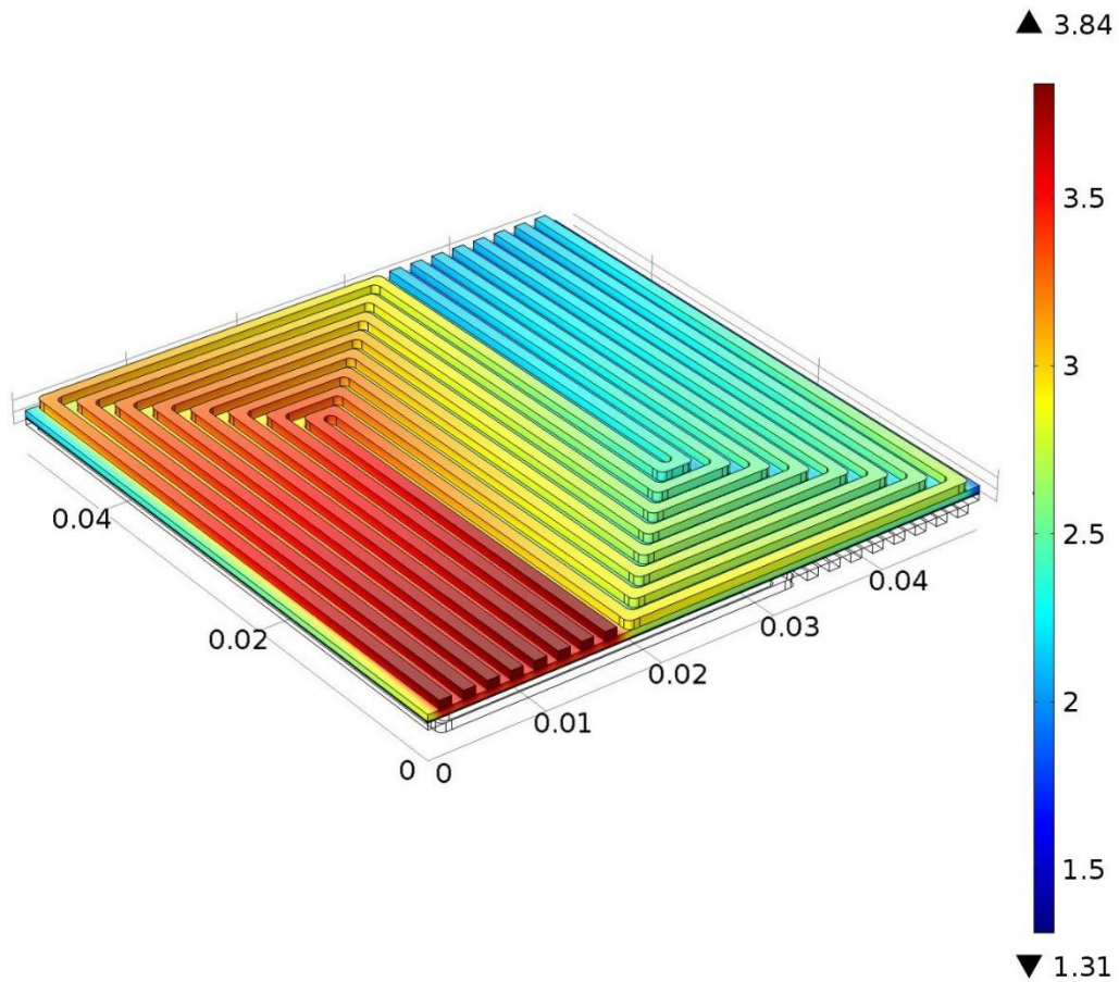
Figure 5.20 Concentration profile of oxygen at 165 °C and 0.6 V for serpentine flow channel geometry ( \text{mol m}^{-3} )
