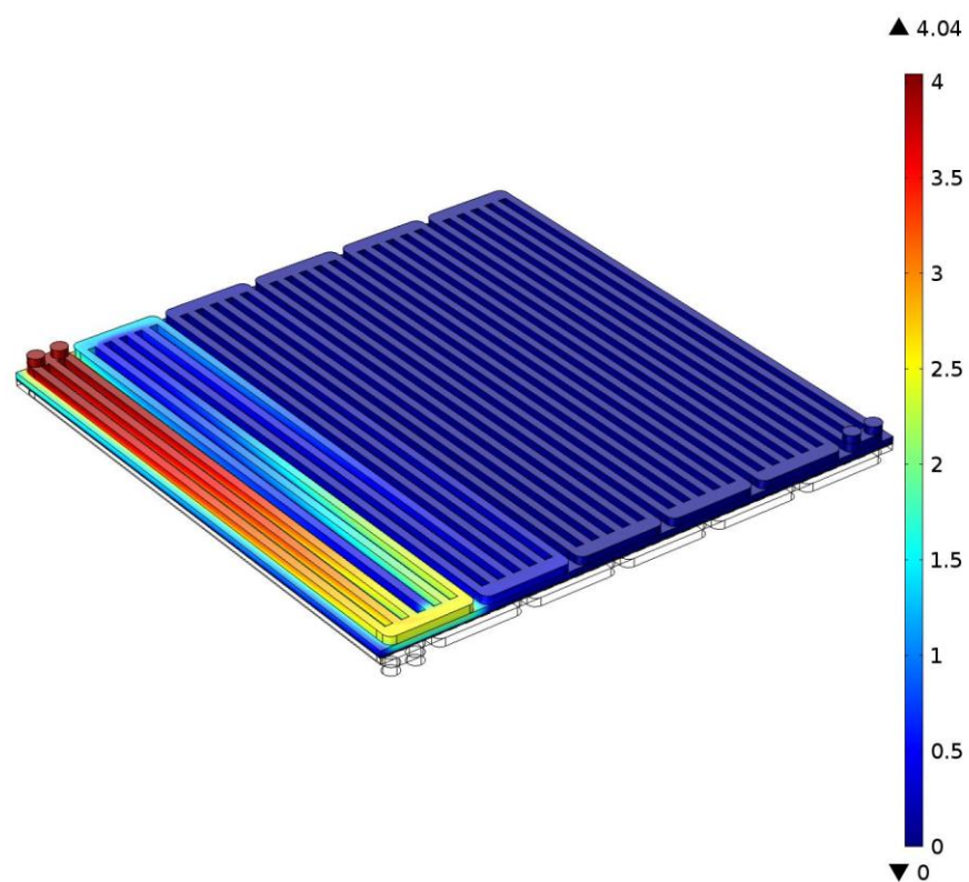
Figure 5.11 Oxygen concentration along cathode flow channels 0.4 V and 1.2 bar backpressure ( \text{mol m}^{-3} )
