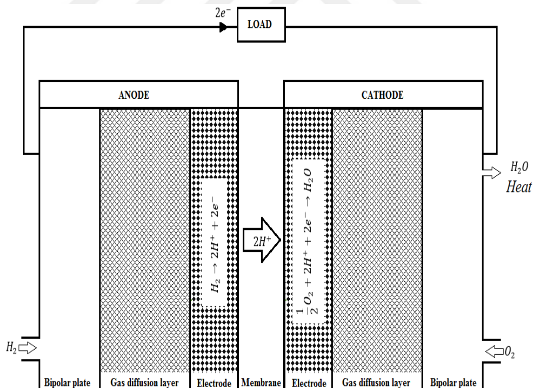
Figure 2.1 Representation of the PEM fuel cell
