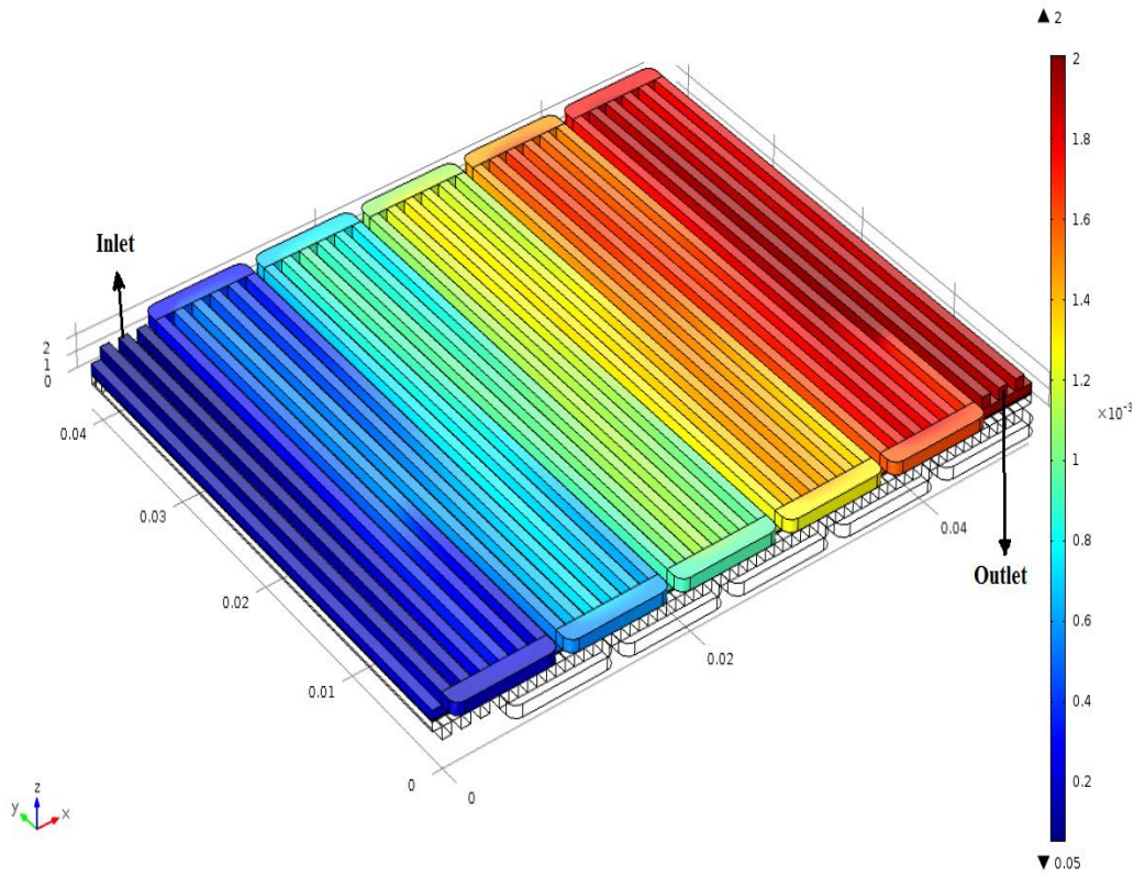
Figure 4.7 Concentration profile of the water along the cathode flow channel operating at 160 °C and 0.6 V ( \text{mol m}^{-3} )
