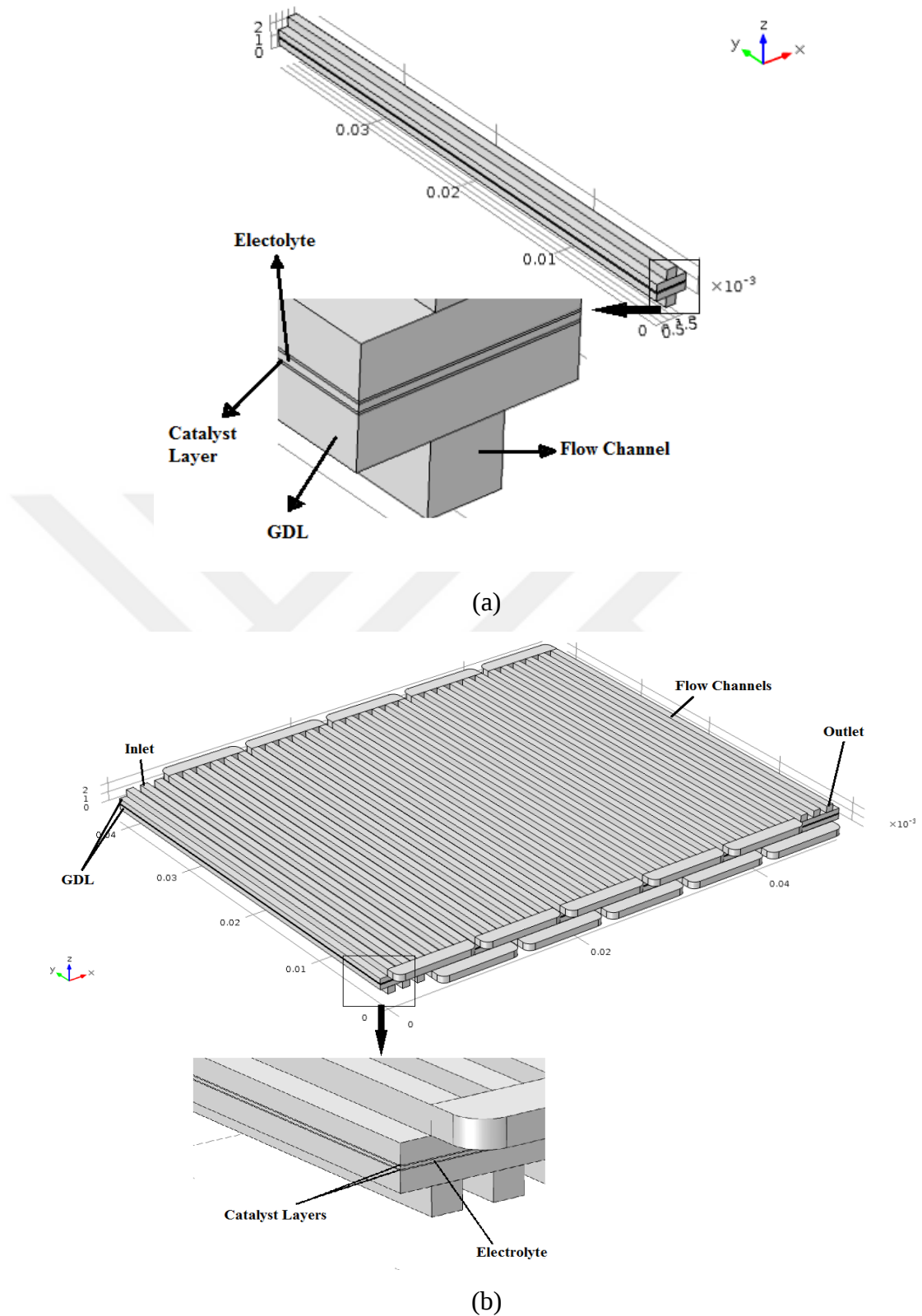
Figure 4.1 Components of the domain used in Comsol Multiphysics model (a) Single flow channel geometry (b) Triple mixed serpentine flow channel geometry
