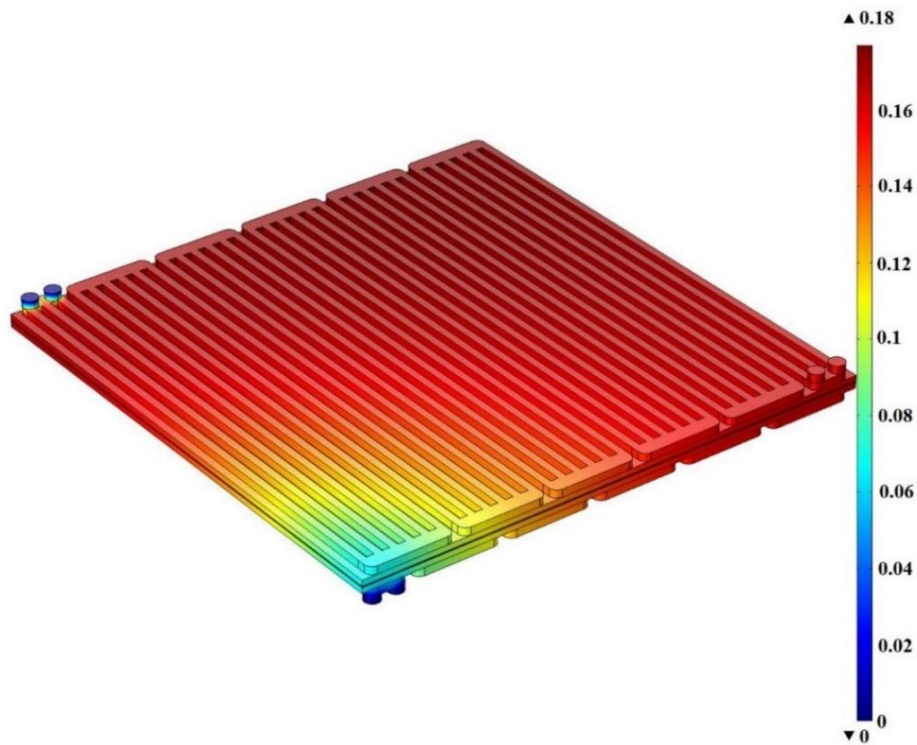
Figure 6.1 Temperature difference in a single cell, inlet reactant temperature is at 165 °C for V=0.60 V (K)
