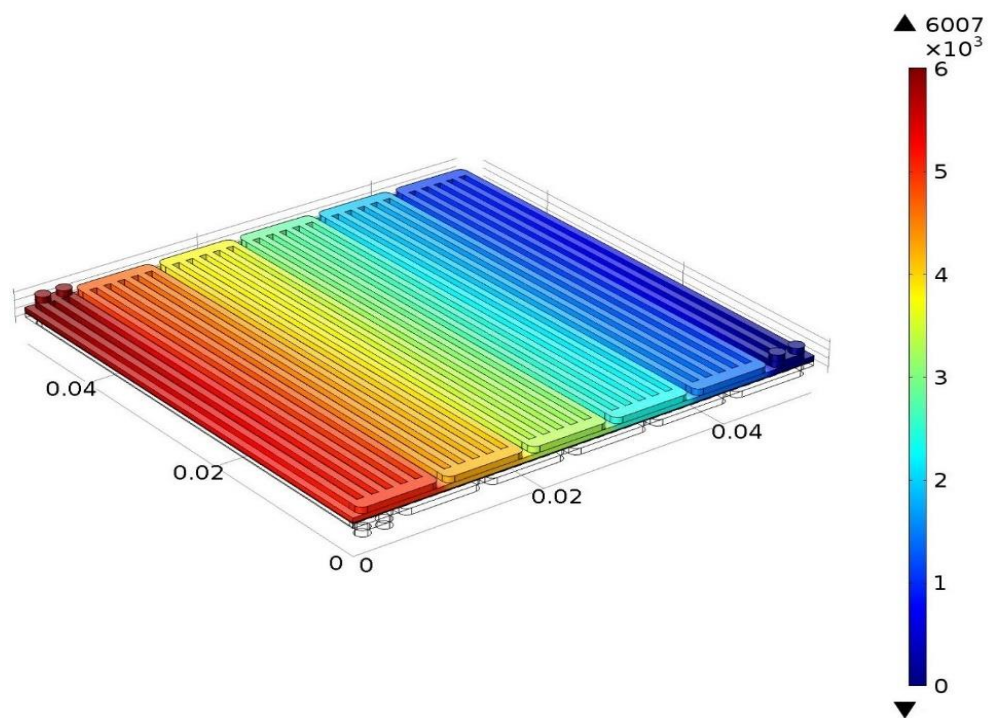
Figure 5.4 Pressure profile along cathode flow channels at V=0.6 V and 1.2 bar backpressure at 140 °C
