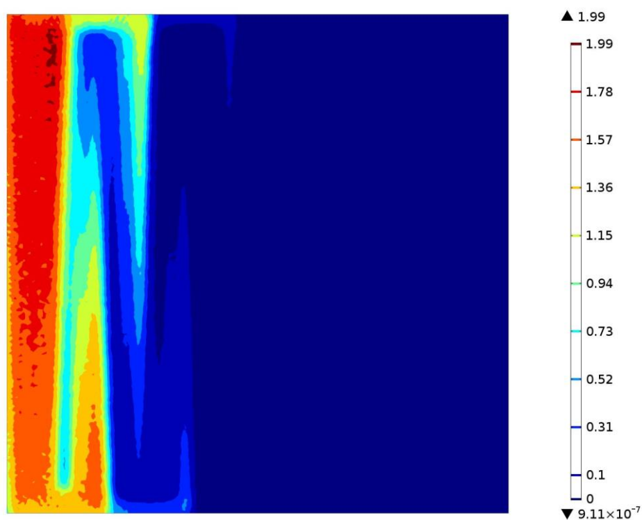
Figure 5.14 Membrane current density distribution at 165 °C, 1.2 bar and 0.4 V ( \text{A cm}^{-2} )
