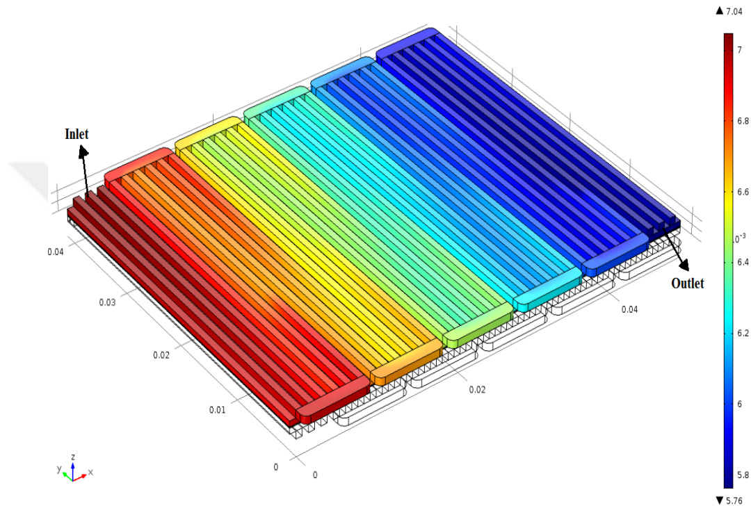
Figure 4.6 Concentration profile of the oxygen along the cathode flow channel operating at 160 °C and 0.6 V (mol m -3 )
