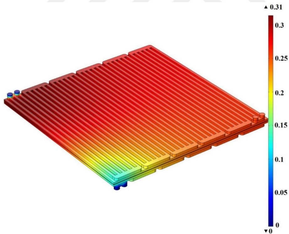
Figure 6.2 Temperature difference in a single cell, inlet reactant temperature is at 165 °C for V=0.45 V (K)
