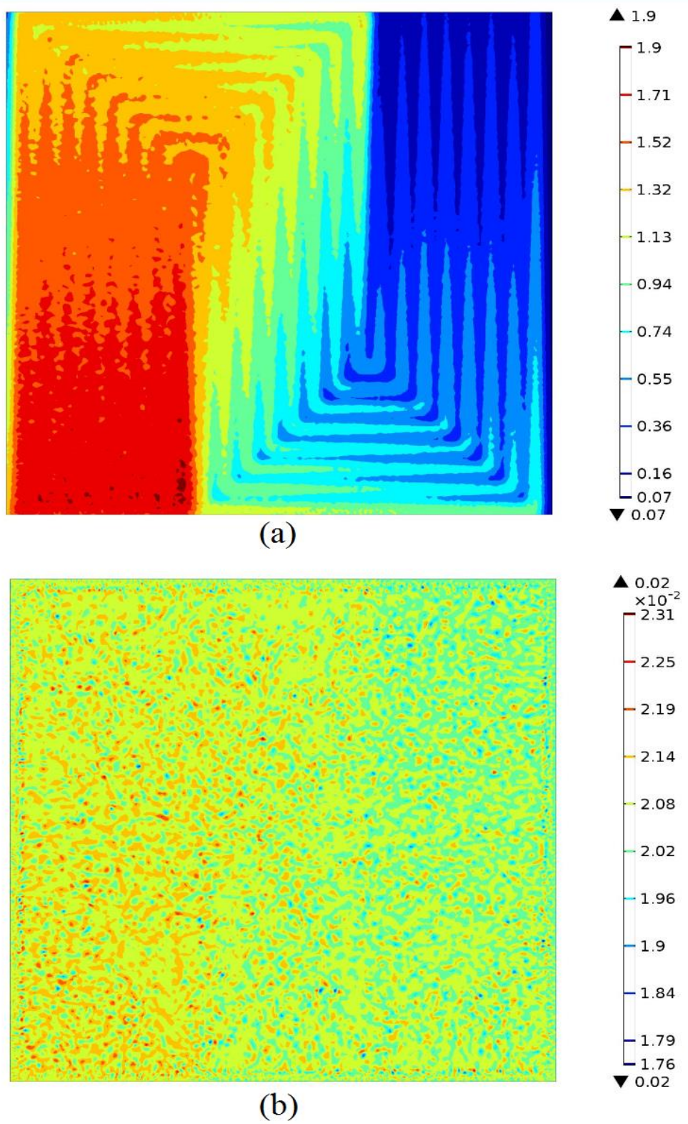
Figure 5.22 Membrane current density distribution at 165 °C for serpentine flow channel geometry (a) 0.4 V, (b) 0.8 V ( \text{A cm}^{-2} )
