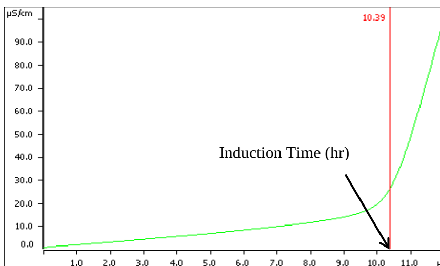
Figure 3.1. Rancimat oxidative stability curve
