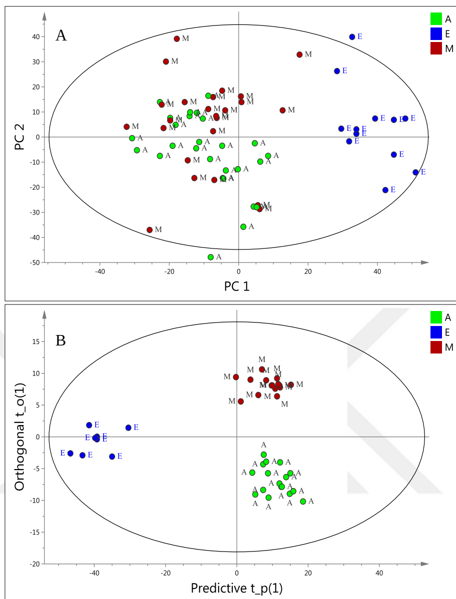
Figure 6.15. PCA (A) and OPLS-DA calibration model (B) Score plots of SNV+2der treated NIR spectra
