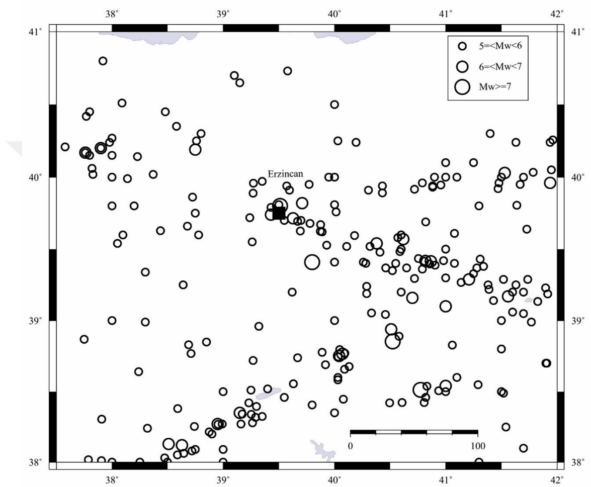
Figure 4.3 Spatial distribution of all earthquakes with M_w \geq 5.0 around Erzincan city center
