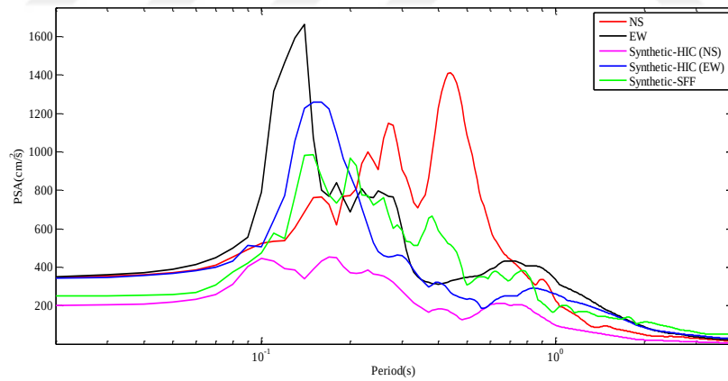
Figure 5.33 Station AQA; (a) Observed and simulated accelerograms (b) Fourier amplitude spectra (c) Response spectra with 5% damping obtained for observed (NS and EW) and simulated horizontal components (Synthetic-SFF and Synthetic-HIC)
