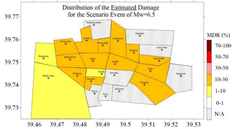
Figure 4.43 Spatial distribution of the estimated (a) PGA (b) PGV (c) MDR in the Erzincan region for scenario event of Mw=6.5
