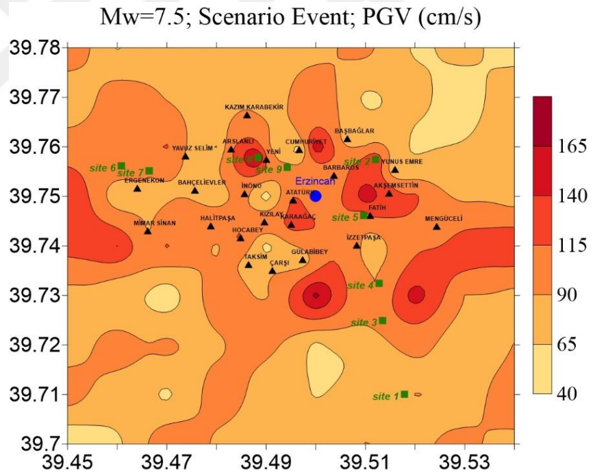
Figure 4.16 Spatial distribution of the simulated (a) PGA (b) PGV values of the scenario earthquake with Mw=7.5 in Erzincan region
