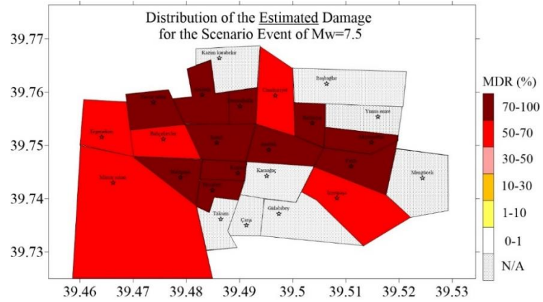
Figure 4.45 Spatial distribution of the estimated (a) PGA (b) PGV (c) MDR in the Erzincan region for scenario event of Mw=7.5
