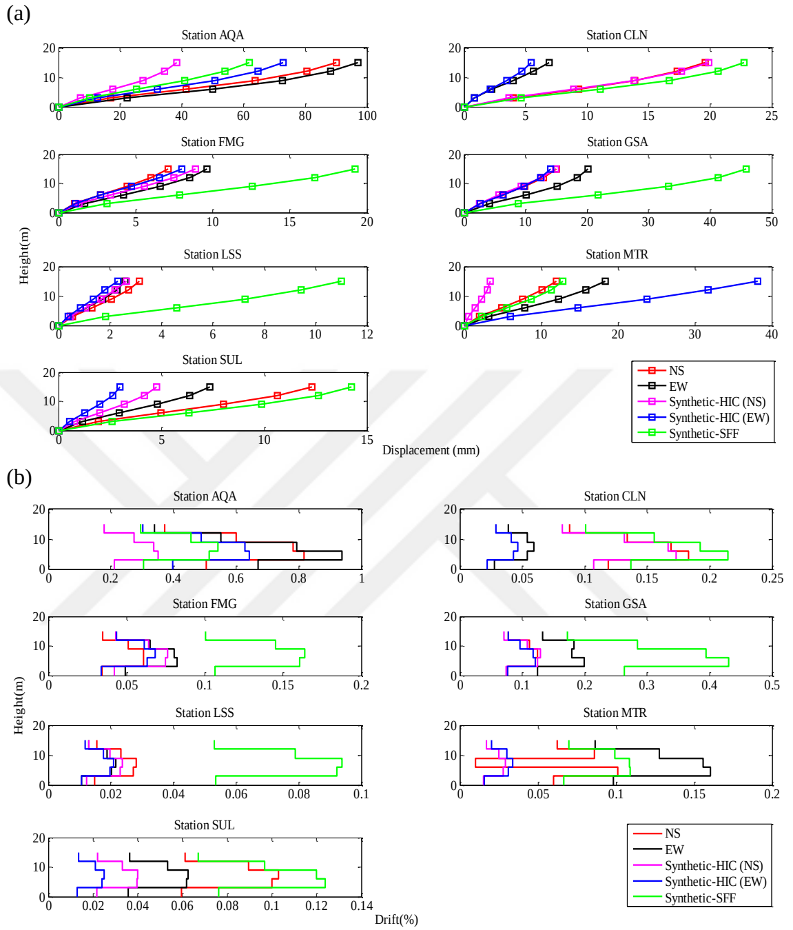
Figure 5.45 Distribution of (a): maximum story displacements and (b): maximum drift ratios due to the real and simulated records of L'Aquila Earthquake – F6-5S2B
