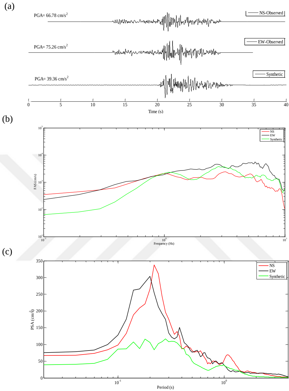
Figure 5.6 Station REF; (a) Observed and simulated accelerograms (b) Fourier Amplitude Spectra (c) Response Spectra with 5% damping obtained for observed (NS and EW) and simulated horizontal component (Synthetic)
