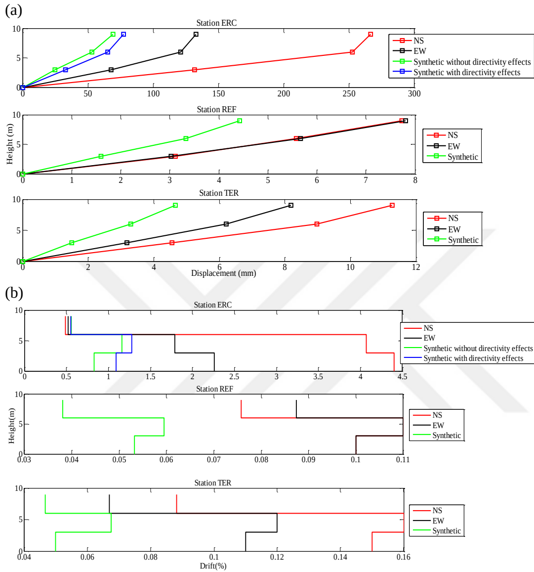
Figure 5.10 Distribution of (a) maximum story displacements and (b) maximum drift ratios due to the real and simulated records of Erzincan Earthquake – F3-3S3B
