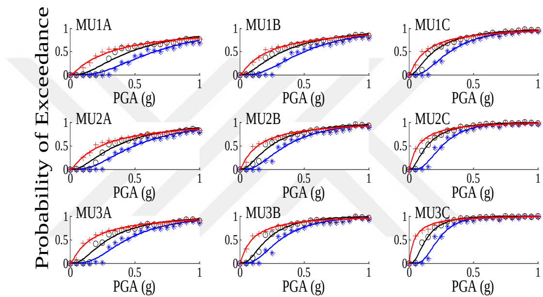
Figure B.4 Fragility curves developed for all masonry sub-classes with respect to PGA using new approach
