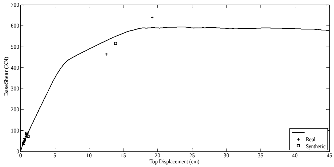
Figure E.11 Capacity Curve and Dynamic Responses of Düzce Earthquake for F2-3S2B
