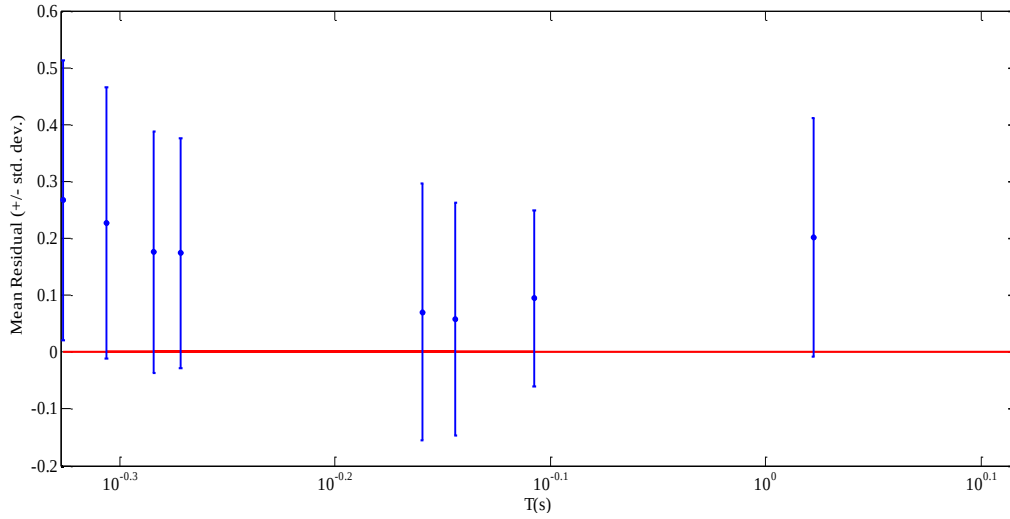
Figure F.6 Average of residuals over all simulated Düzce records versus period of frames, where residual = \log(\text{Predicted NR}) - \log(\text{Observed NR}) . Standard deviation of residuals is depicted by error bars.
