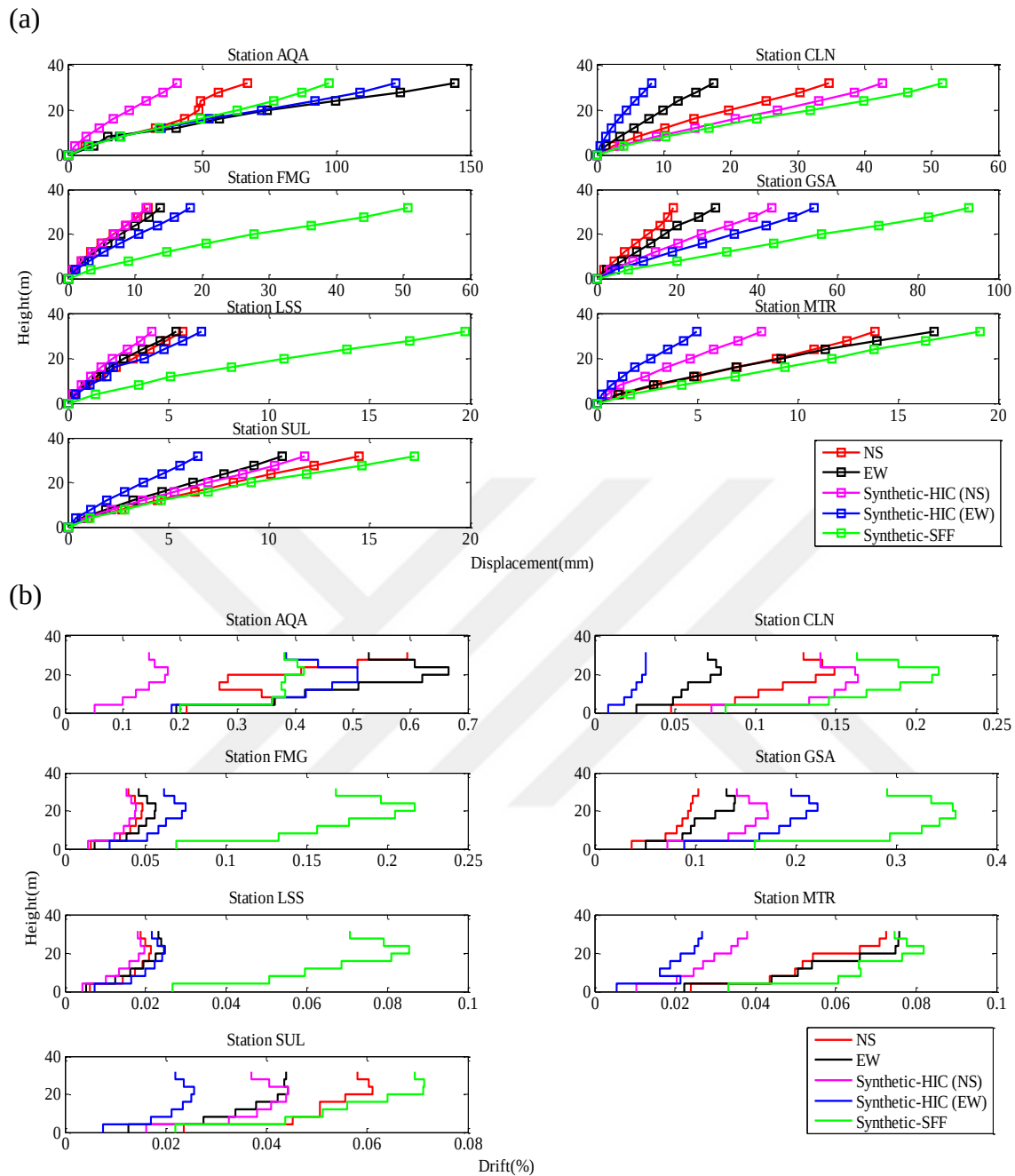
Figure 5.48 Distribution of (a): maximum story displacements and (b): maximum drift ratios due to the real and simulated records of L'Aquila Earthquake – F9-8S3B
