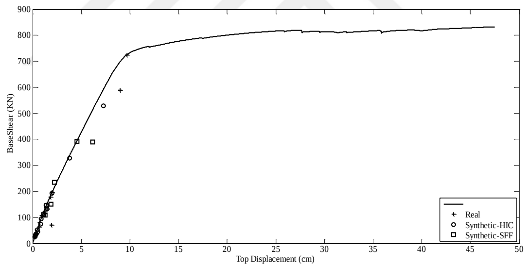
Figure E.24 Capacity Curve and Dynamic Responses of L'Aquila Earthquake for F6-5S2B
