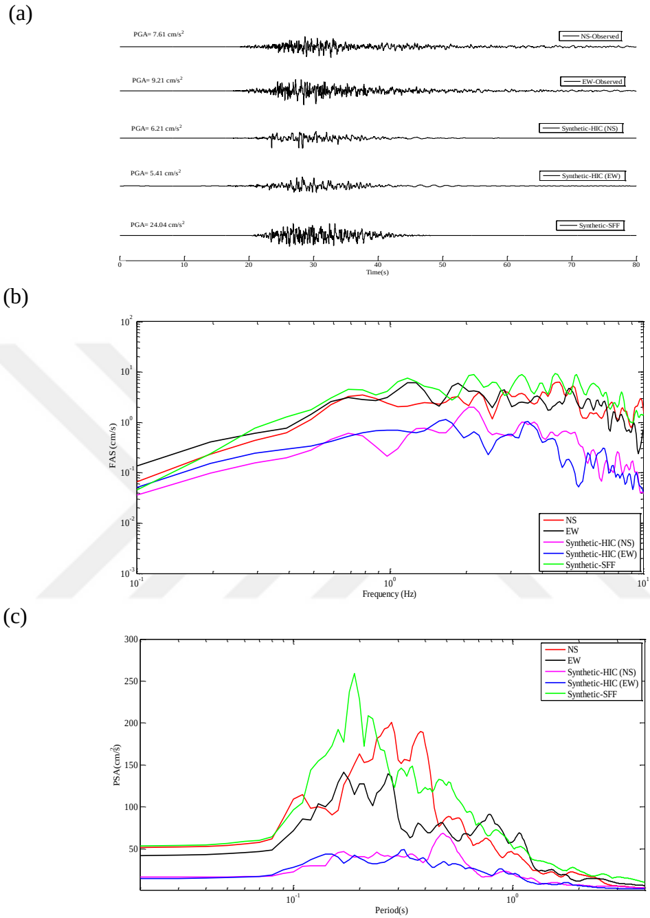
Figure 5.38 Station MTR; (a) Observed and simulated accelerograms (b) Fourier amplitude spectra (c) Response spectra with 5% damping obtained for observed (NS and EW) and simulated horizontal components (Synthetic-SFF and Synthetic-HIC)
