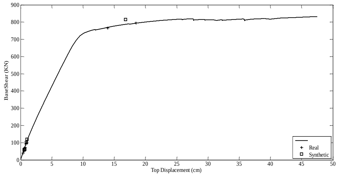
Figure E.15 Capacity Curve and Dynamic Responses of Düzce Earthquake for F6-5S2B
