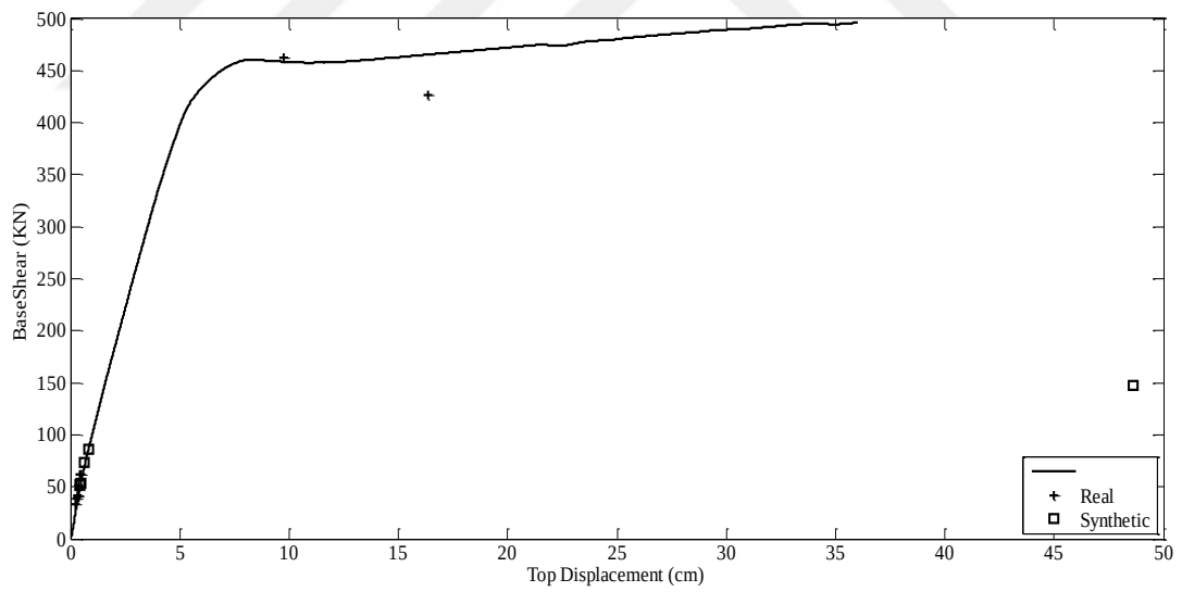
Figure E.12 Capacity Curve and Dynamic Responses of Düzce Earthquake for F3-3S3B
