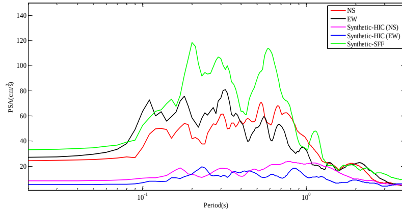
Figure 5.39 Station SUL; (a) Observed and simulated accelerograms (b) Fourier amplitude spectra (c) Response spectra with 5% damping obtained for observed (NS and EW) and simulated horizontal components (Synthetic-SFF and Synthetic-HIC)
