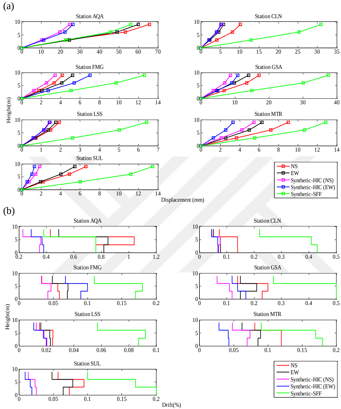
Figure 5.42 Distribution of (a): maximum story displacements and (b): maximum drift ratios due to the real and simulated records of L'Aquila Earthquake – F3-3S3B
