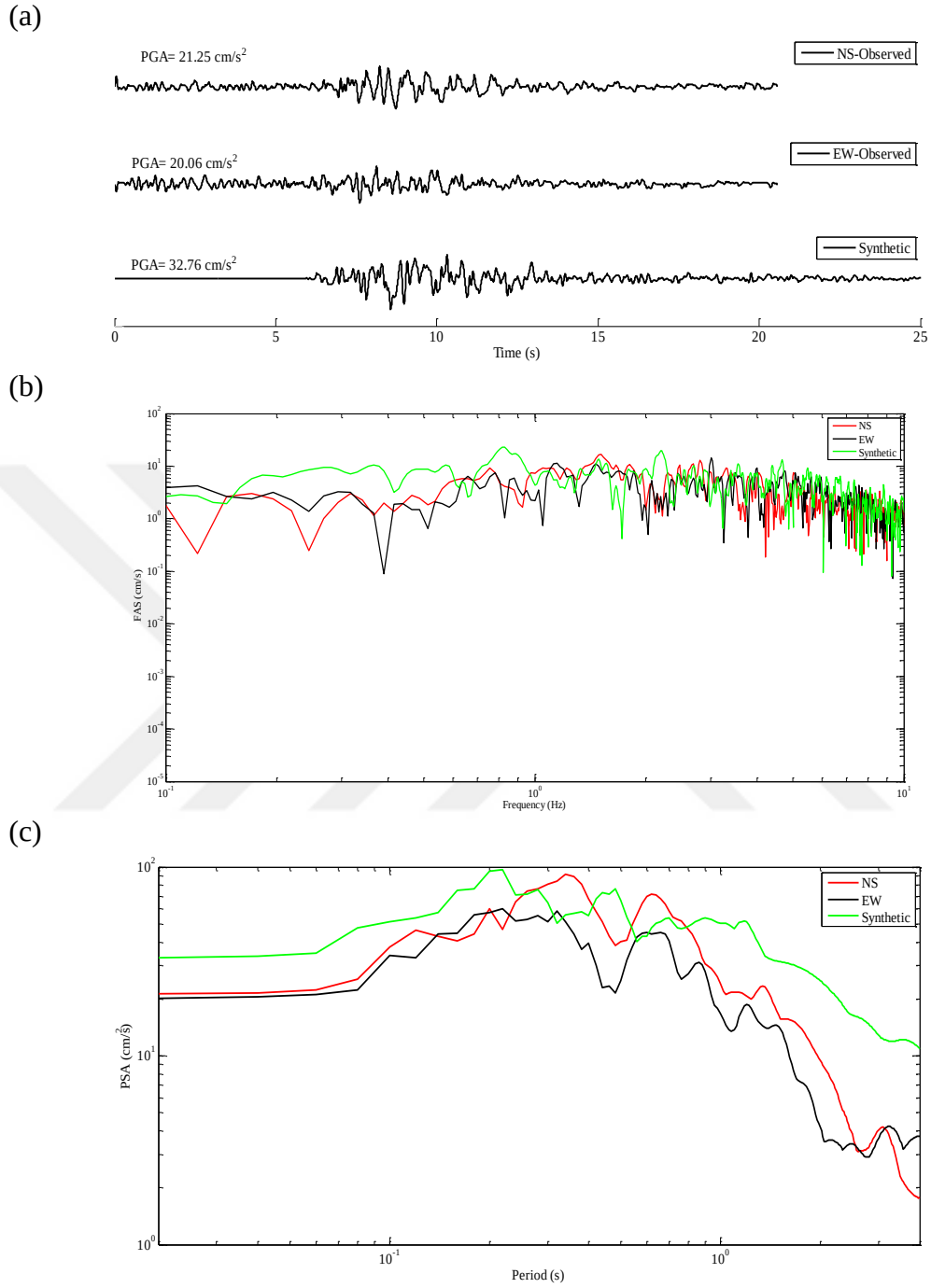
Figure 5.20 Station IZN; (a) Observed and simulated accelerograms (b) Fourier amplitude spectra (c) Response spectra with 5% damping obtained for observed (NS and EW) and simulated horizontal component (Synthetic)
