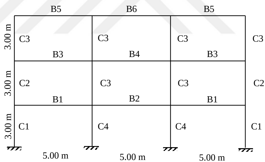
Figure D.3 Frame F3-3S3B
