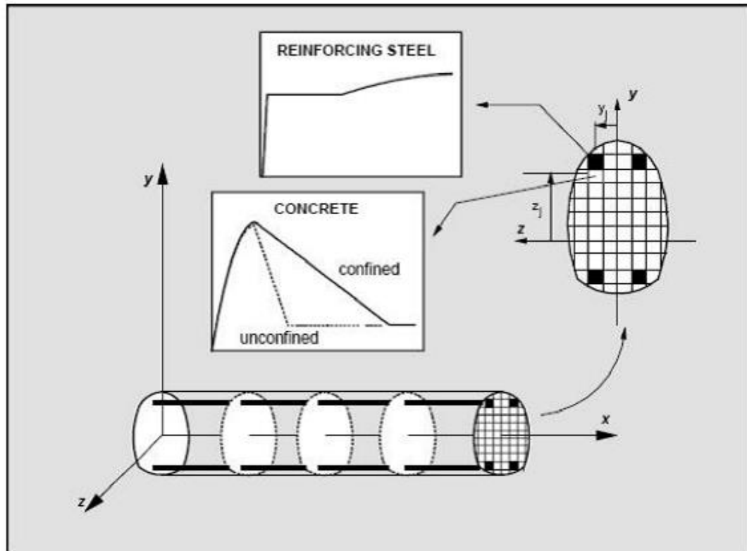
Figure 5.2 Graphical representation of a fiber element (Adopted from Taucer et al. , 1991)
