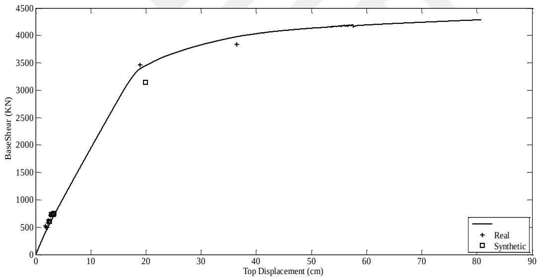
Figure E.18 Capacity Curve and Dynamic Responses of Düzce Earthquake for F9-8S3B
