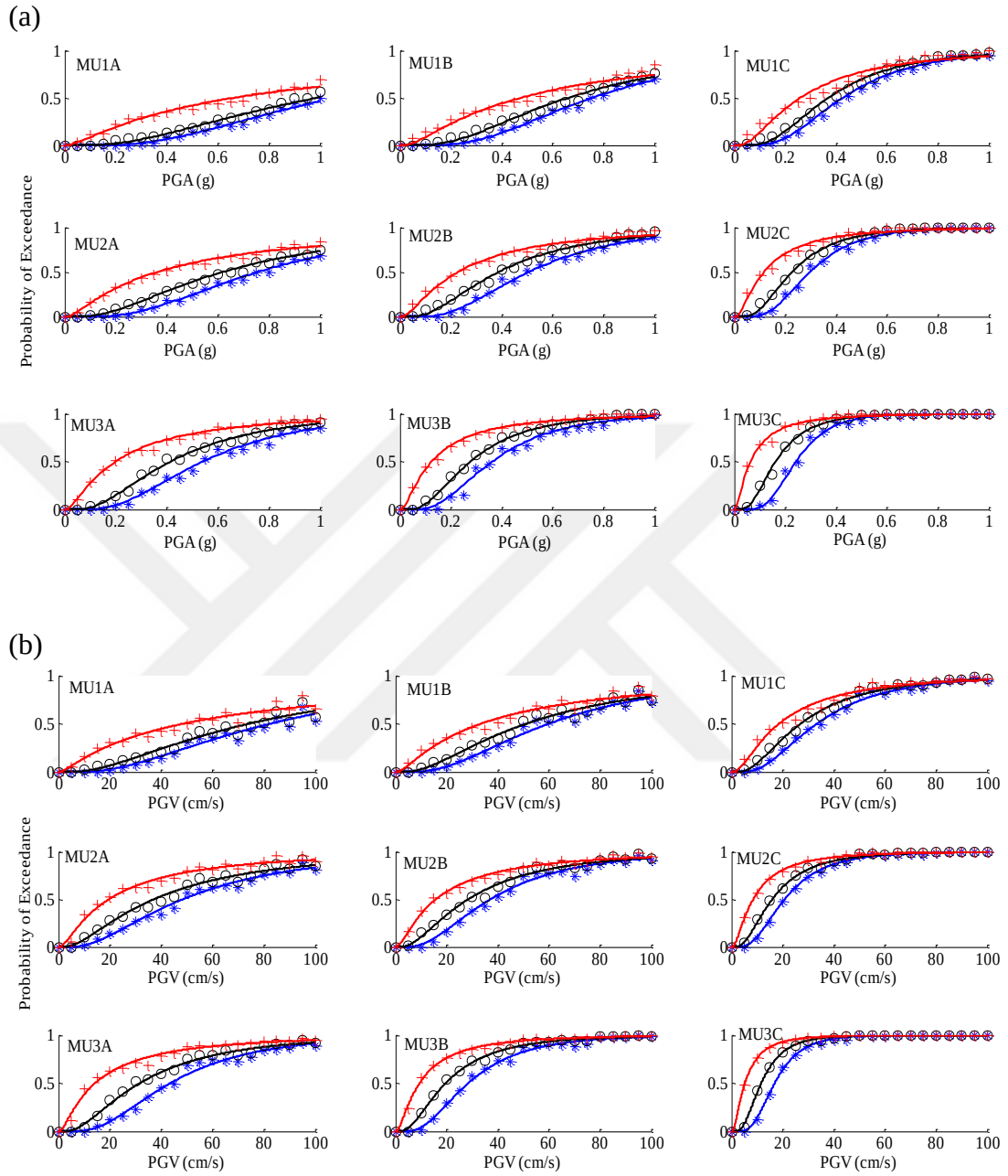
Figure 4.28 Fragility curves for masonry sub-classes using records categorized based on (a) PGA and (b) PGV where the red lines correspond to LS_1 , the black lines to LS_2 , and the blue lines to LS_3
