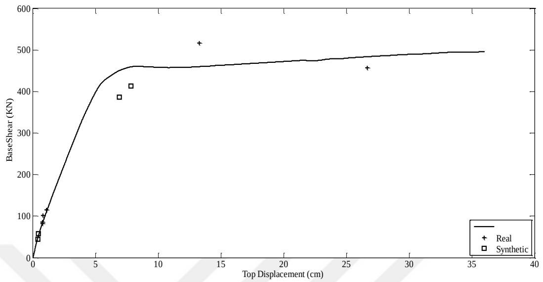
Figure E.3 Capacity Curve and Dynamic Responses of Erzincan Earthquake for F3-3S3B
