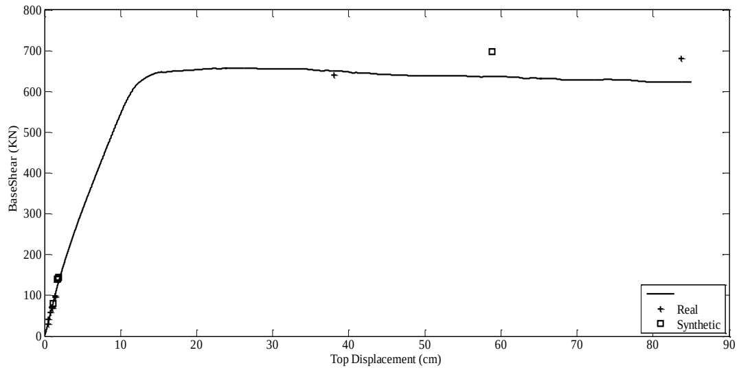
Figure E.17 Capacity Curve and Dynamic Responses of Düzce Earthquake for F8-7S4B
