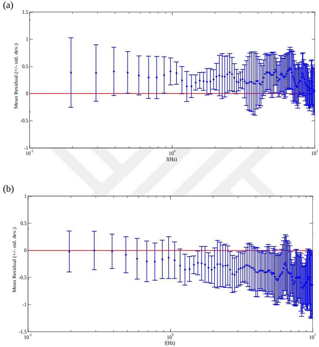
Figure F.7 Average of residuals using (a) Synthetic-SFF and (b) Synthetic-HIC methods over all simulated L'Aquila records versus frequency, where residual = \log(\text{Predicted FAS}) - \log(\text{Observed FAS}) . Standard deviation of residuals is depicted by error bars.
