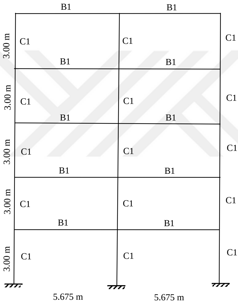
Figure D.6 Frame F6-5S2B
