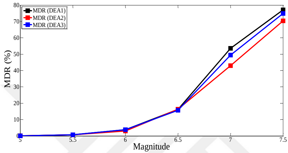
Figure C.1 Comparison of the average MDRs for Erzincan presented for three approaches: DEA1, DEA2, and DEA3
