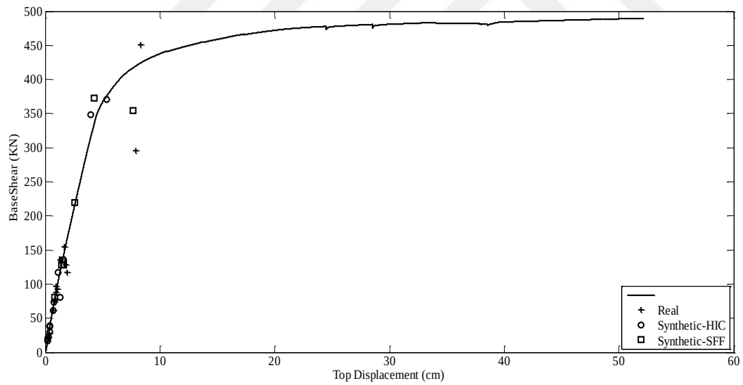
Figure E.22 Capacity Curve and Dynamic Responses of L'Aquila Earthquake for F4-4S3B
