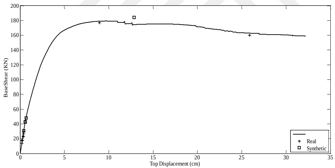
Figure E.14 Capacity Curve and Dynamic Responses of Düzce Earthquake for F5-4S3B
