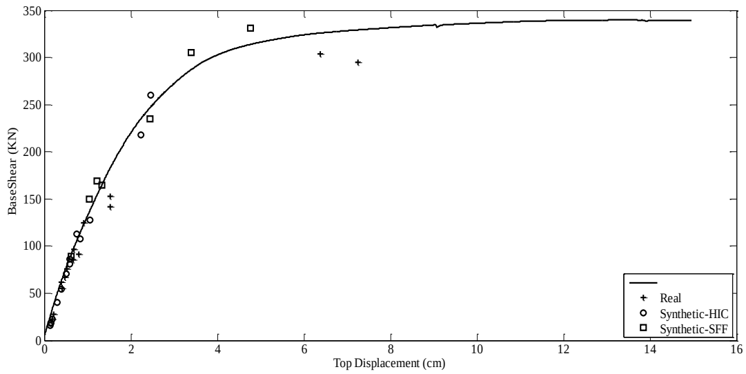
Figure E.25 Capacity Curve and Dynamic Responses of L'Aquila Earthquake for F7-5S4B
