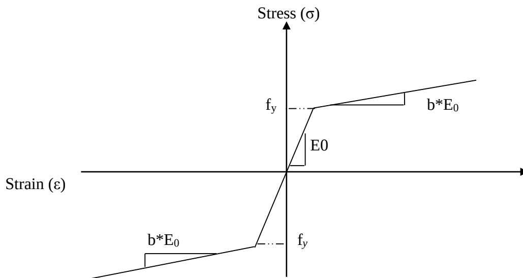
Figure 5.3 Material models for (a) steel and (b) concrete; (In this figure, f_y is the yield strength, E_0 is the initial elastic tangent, b is the strain-hardening ratio of the steel, f_c is the concrete compressive strength at 28 days, \epsilon_c is the concrete strain at maximum strength, f_u is the concrete crushing strength, \epsilon_u is the concrete strain at crushing strength)
