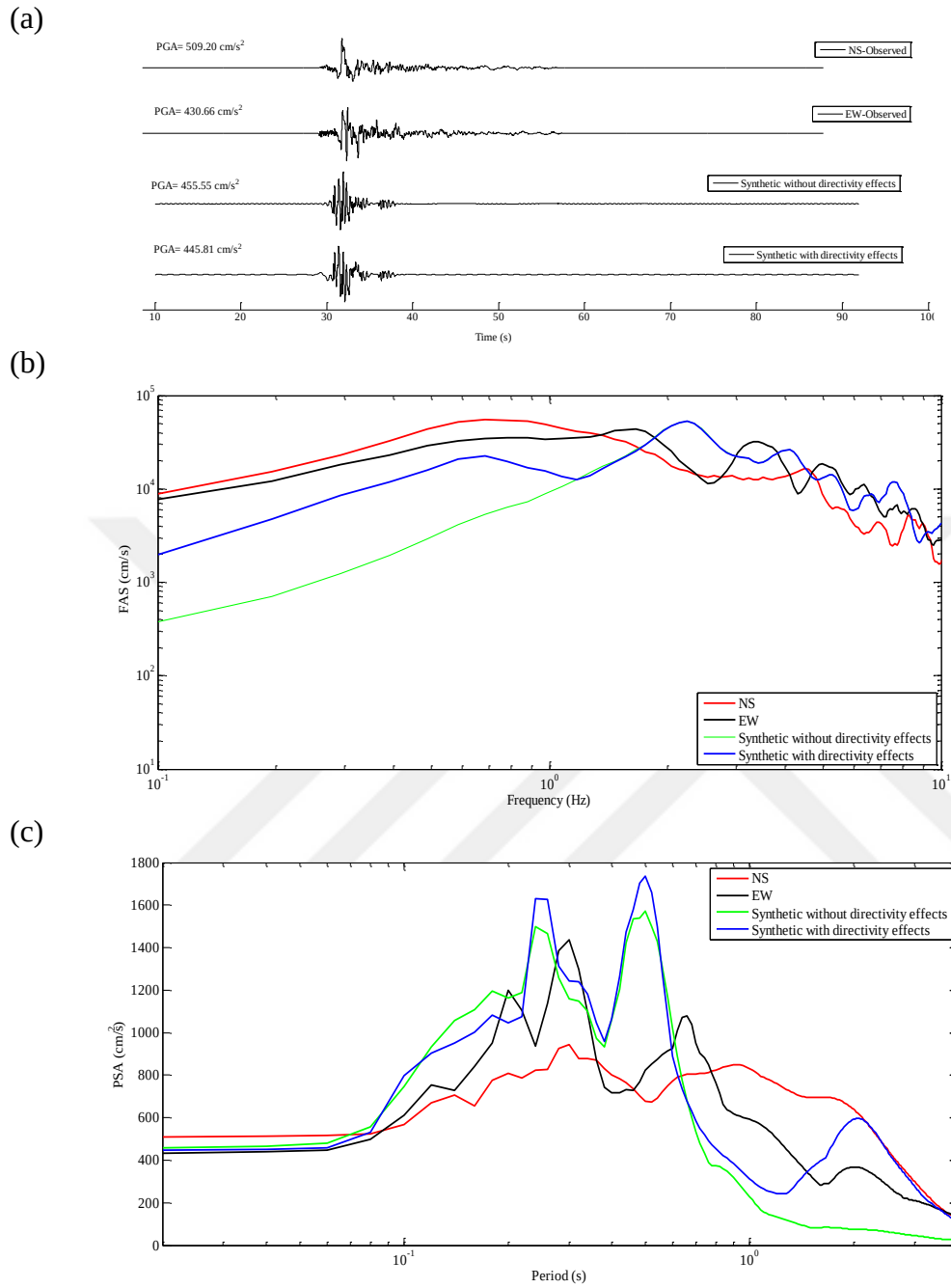
Figure 5.5 Station ERC; (a) Observed and simulated accelerograms (b) Fourier Amplitude Spectra (c) Response Spectra with 5% damping obtained for observed (NS and EW) and simulated horizontal component (Synthetic with and without directivity effects)
