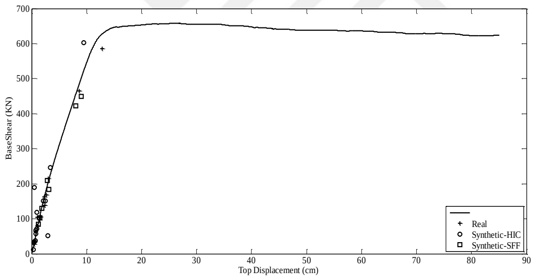
Figure E.26 Capacity Curve and Dynamic Responses of L'Aquila Earthquake for F8-7S3B
