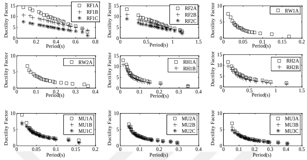
Figure 4.22 Period and ductility factor pairs generated by LHS technique for all sub-classes
