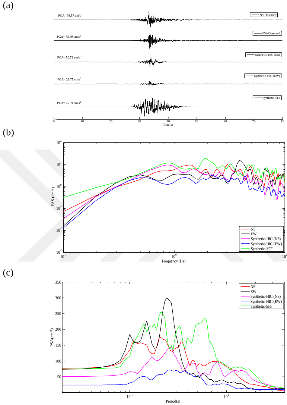
Figure 5.34 Station CLN; (a) Observed and simulated accelerograms (b) Fourier amplitude spectra (c) Response spectra with 5% damping obtained for observed (NS and EW) and simulated horizontal components (Synthetic-SFF and Synthetic-HIC)
