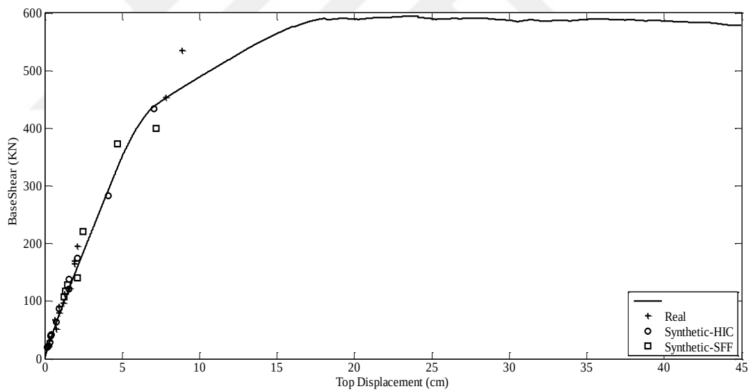
Figure E.20 Capacity Curve and Dynamic Responses of L'Aquila Earthquake for F2-3S2B
