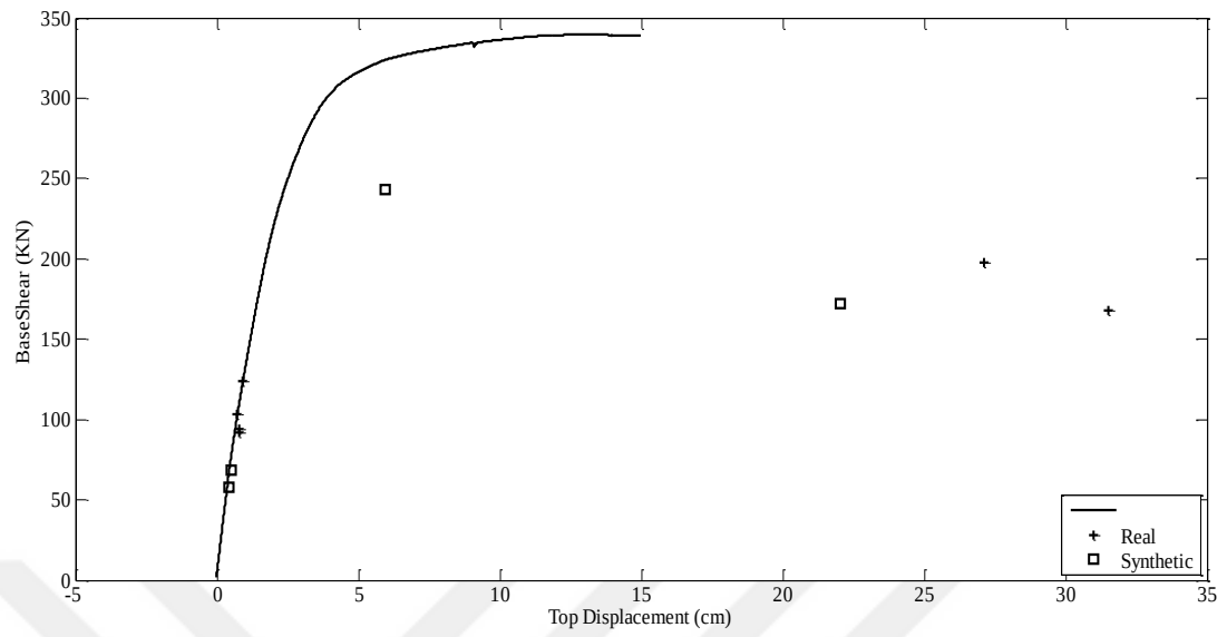
Figure E.7 Capacity Curve and Dynamic Responses of Erzincan Earthquake for F7-5S4B
