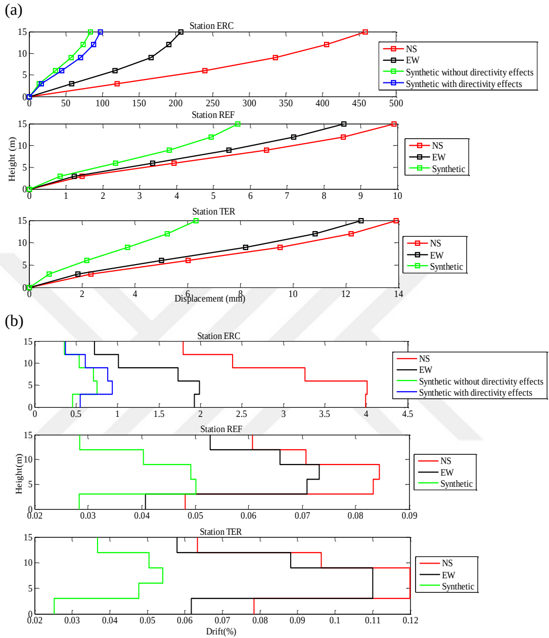
Figure 5.13 Distribution of (a) maximum story displacements and (b) maximum drift ratios due to the real and simulated records of Erzincan Earthquake – F6-5S2B
