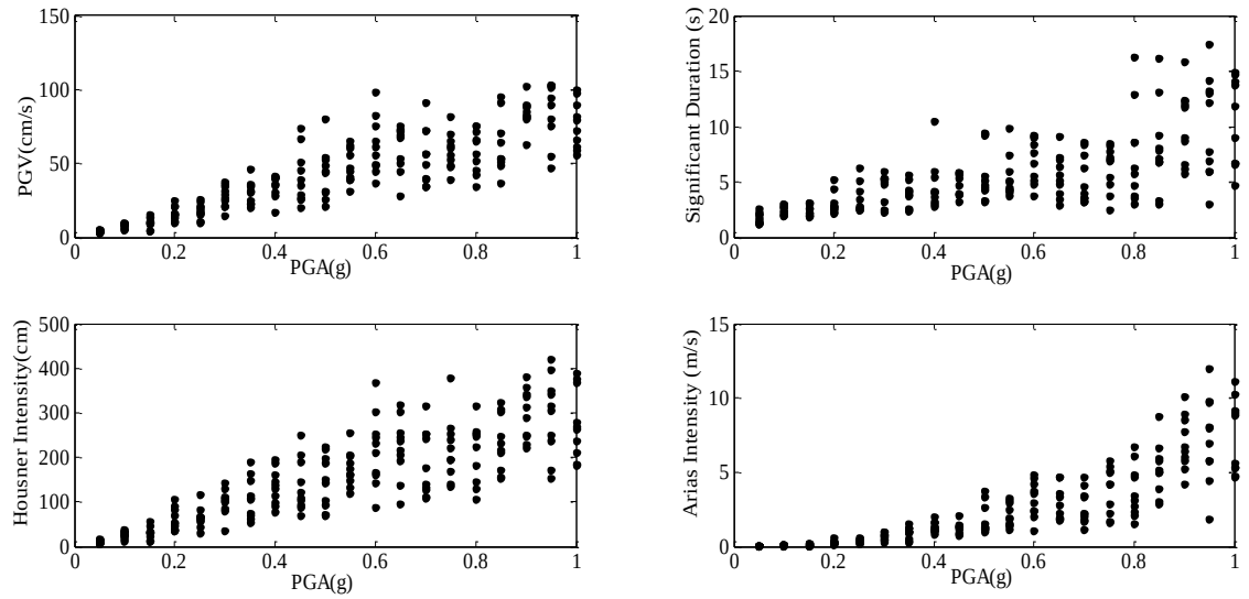
Figure 4.20 Distribution of the ground motion parameters for the second set of motions
