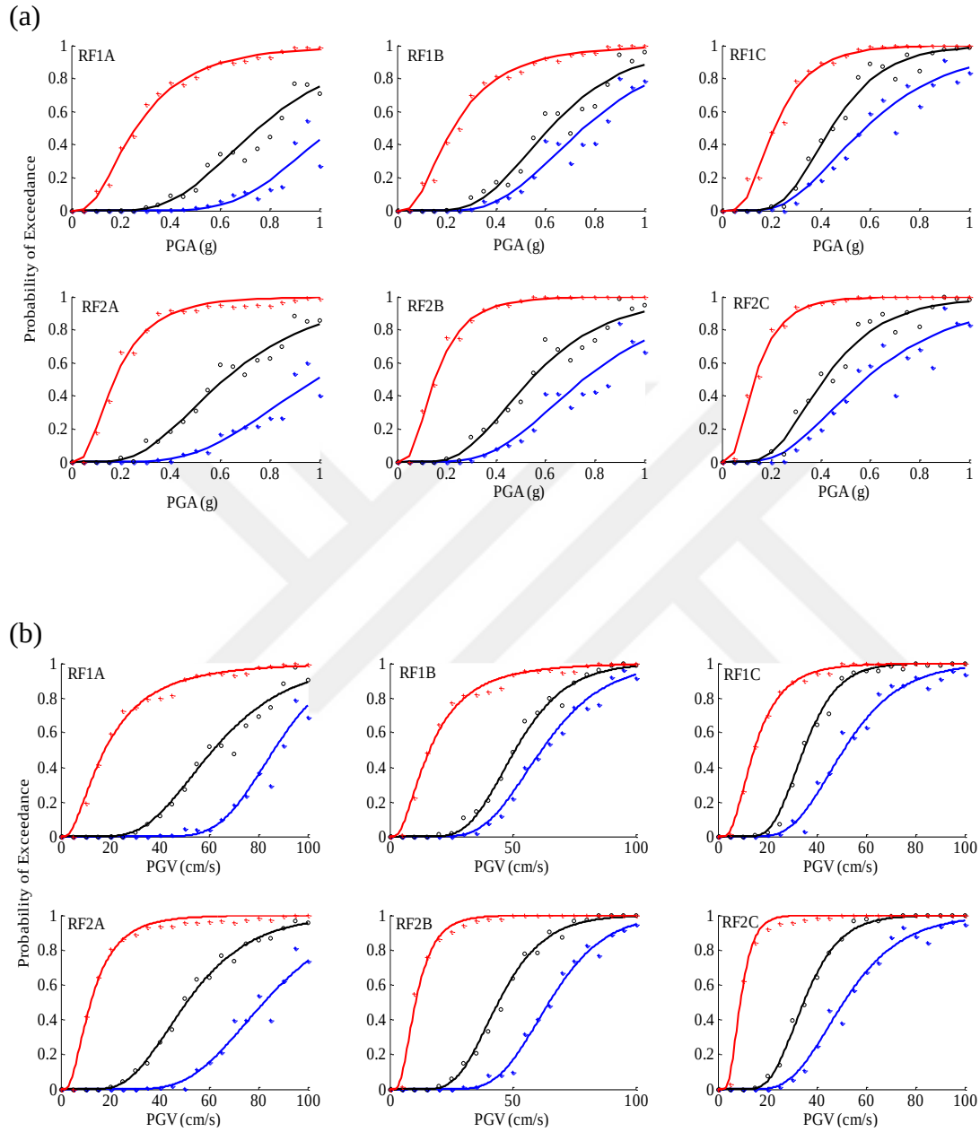
Figure 4.25 Fragility curves for RF sub-classes using records categorized based on (a) PGA and (b) PGV where the red lines correspond to LS_1 , the black lines to LS_2 , and the blue lines to LS_3
