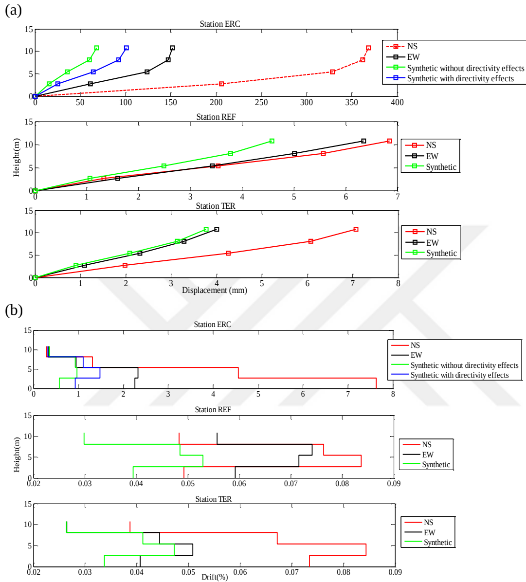
Figure 5.12 Distribution of (a) maximum story displacements and (b) maximum drift ratios due to the real and simulated records of Erzincan Earthquake – F5-4S3B
