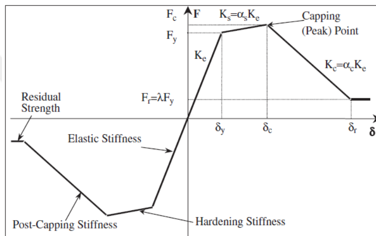
Figure 4.17 Backbone curve for hysteresis model (Adapted from Ibarra et al. , 2005)
