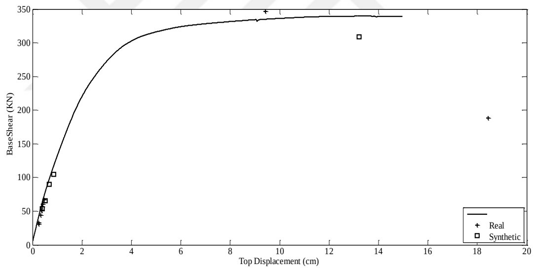
Figure E.16 Capacity Curve and Dynamic Responses of Düzce Earthquake for F7-5S4B
