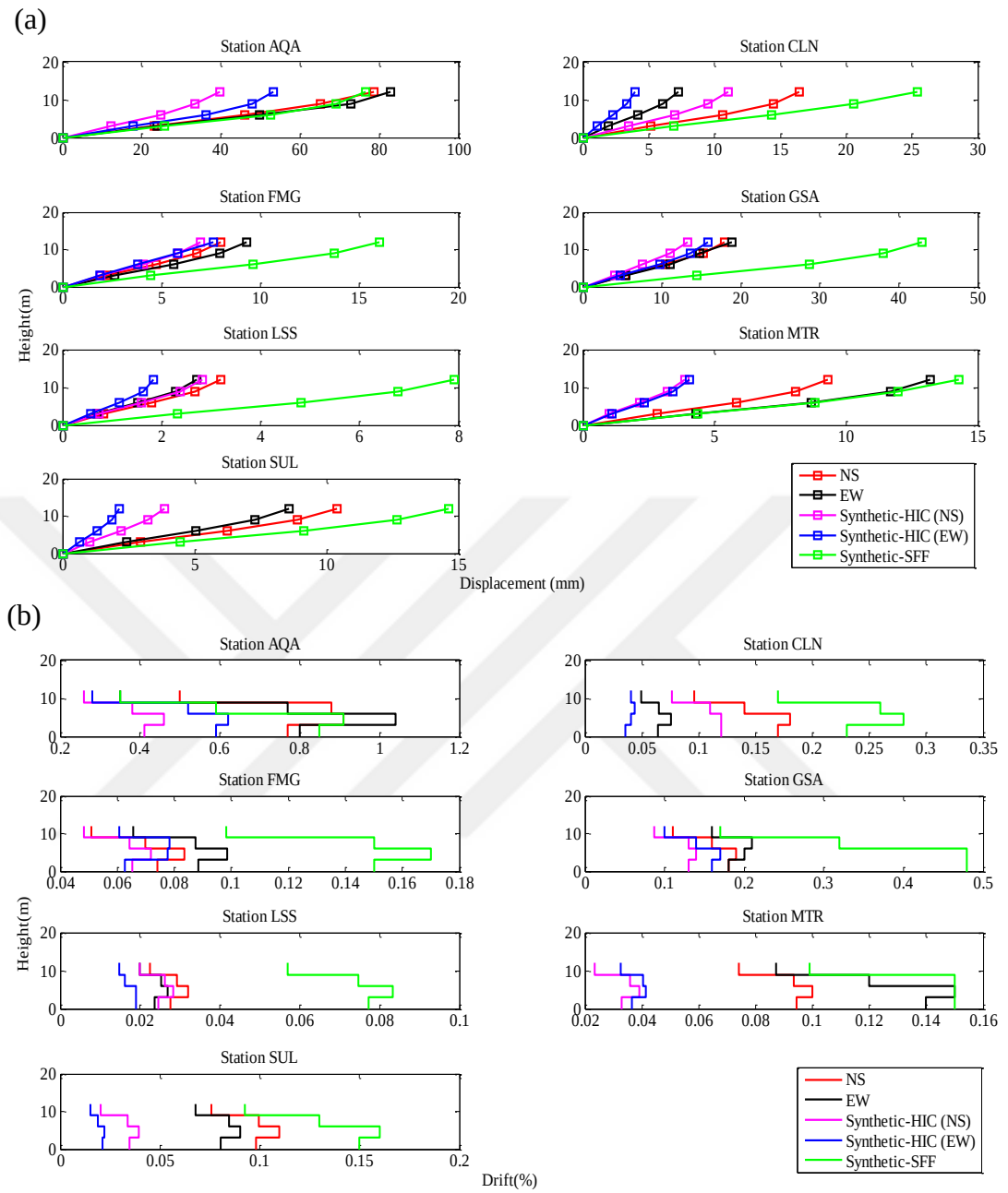
Figure 5.43 Distribution of (a): maximum story displacements and (b): maximum drift ratios due to the real and simulated records of L'Aquila Earthquake – F4-4S3B
