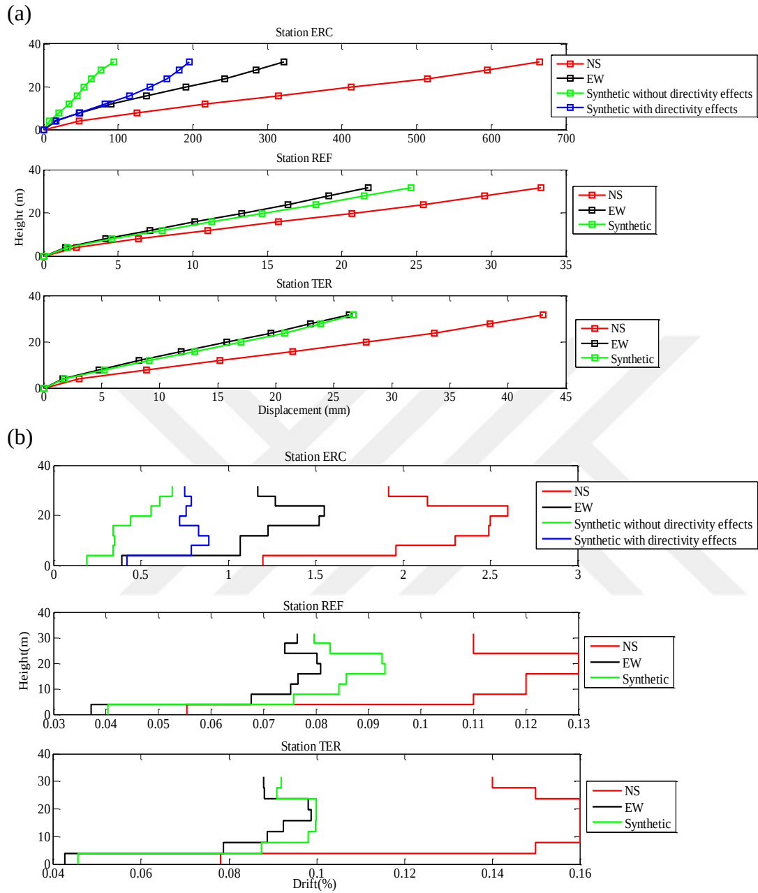
Figure 5.16 Distribution of (a) maximum story displacements and (b) maximum drift ratios due to the real and simulated records of Erzincan Earthquake – F9-8S3B
