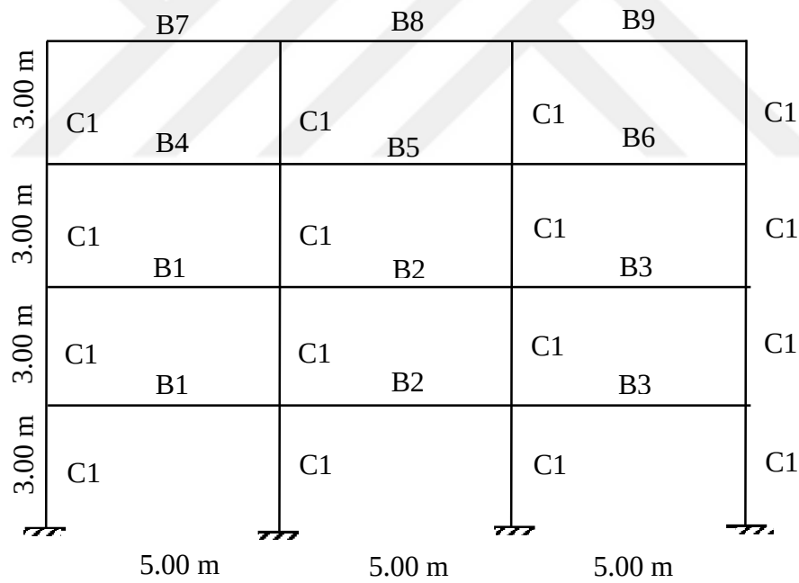
Figure D.4 Frame F4-4S3B
