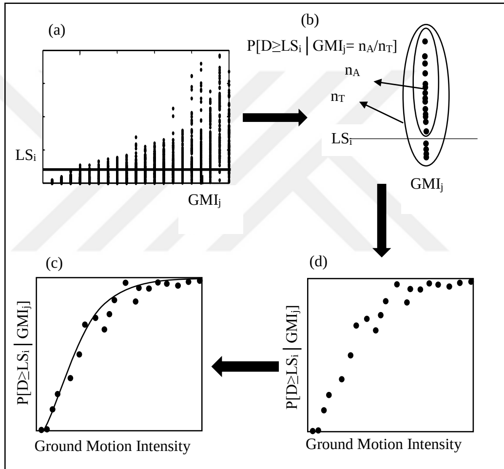
Figure 4.24 Schematic representation of the fragility curve generation procedure
