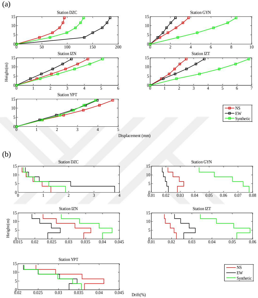
Figure 5.29 Distribution of (a): maximum story displacements and (b): maximum drift ratios due to the real and simulated records of Düzce Earthquake – F7-5S4B
