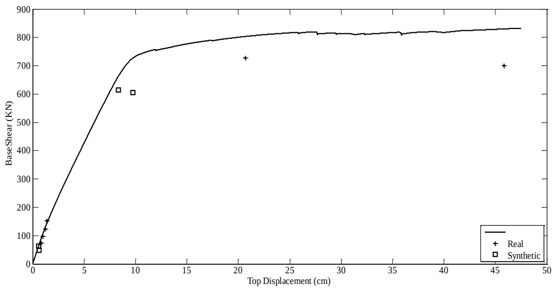
Figure E.6 Capacity Curve and Dynamic Responses of Erzincan Earthquake for F6-5S2B
