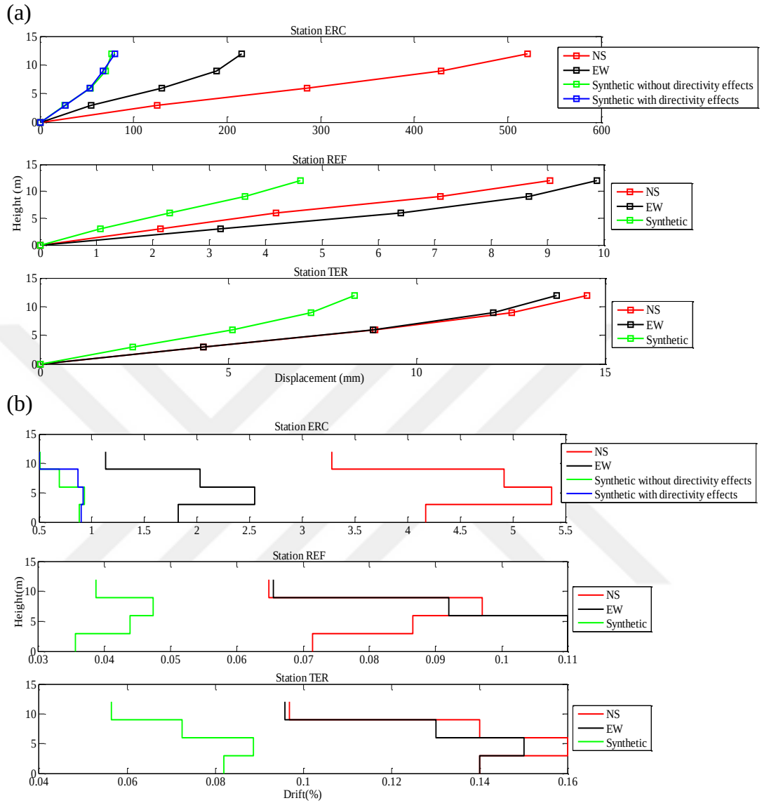
Figure 5.11 Distribution of (a) maximum story displacements and (b) maximum drift ratios due to the real and simulated records of Erzincan Earthquake – F4-4S3B
