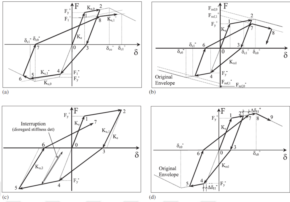
Figure 4.18 Individual deterioration modes of Ibarra peak-oriented model: (a) basic strength deterioration; (b) post-capping strength deterioration; (c) unloading stiffness deterioration; and (d) accelerated reloading stiffness deterioration (Adopted from Ibarra et al. , 2005)
