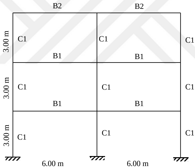
Figure D.2 Frame F2-3S2B
