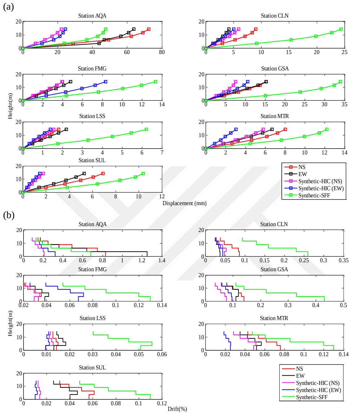
Figure 5.46 Distribution of (a): maximum story displacements and (b): maximum drift ratios due to the real and simulated records of L'Aquila Earthquake – F7-5S4B
