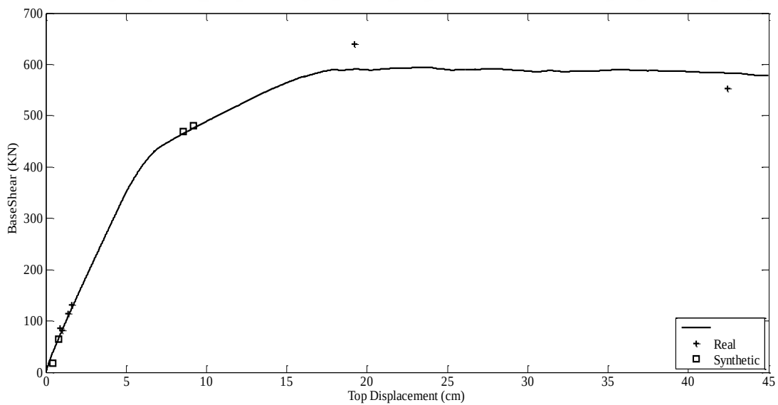
Figure E.2 Capacity Curve and Dynamic Responses of Erzincan Earthquake for F2-3S2B
