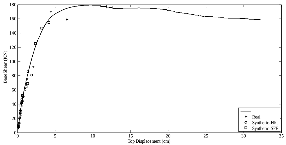
Figure E.23 Capacity Curve and Dynamic Responses of L'Aquila Earthquake for F5-4S3B
