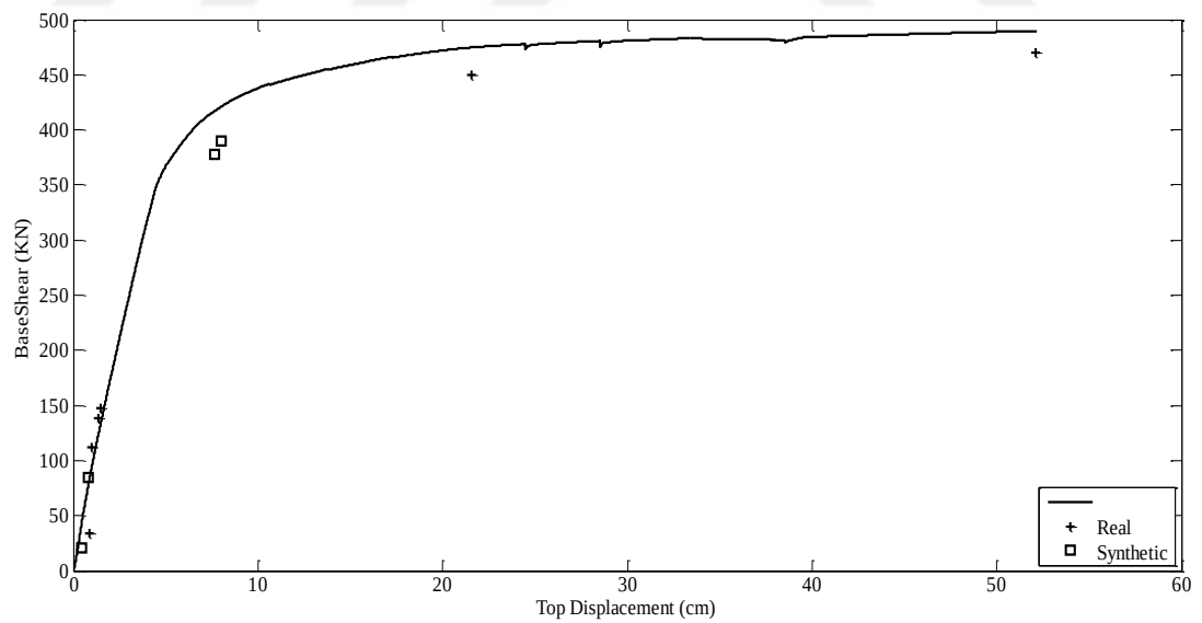
Figure E.4 Capacity Curve and Dynamic Responses of Erzincan Earthquake for F4-4S3B
