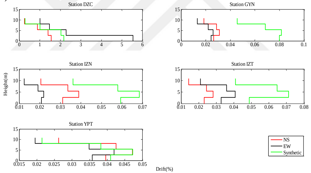
Figure 5.27 Distribution of (a): maximum story displacements and (b): maximum drift ratios due to the real and simulated records of Düzce Earthquake – F5-4S3B
