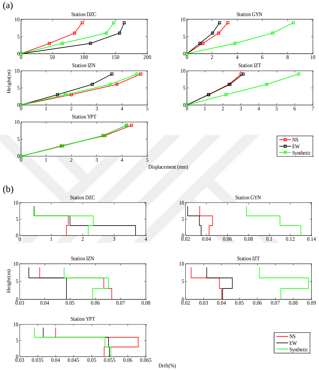
Figure 5.25 Distribution of (a): maximum story displacements and (b): maximum drift ratios due to the real and simulated records of Düzce Earthquake – F3-3S3B
