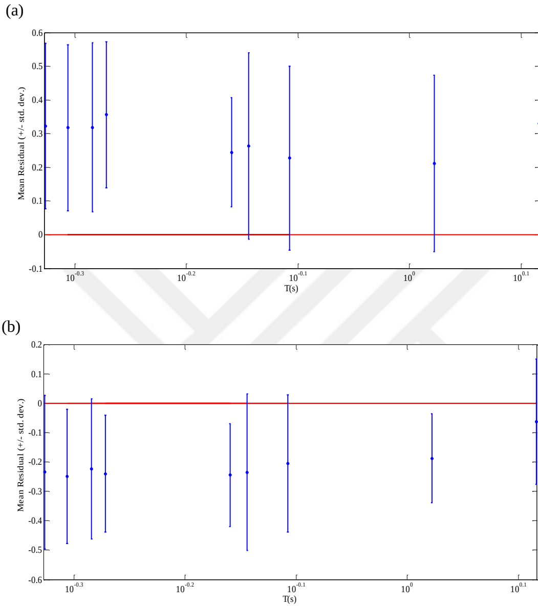
Figure F.9 Average of residuals using (a) Synthetic-SFF and (b) Synthetic-HIC methods over all simulated L'Aquila records versus period of frames, where residual = \log(\text{Predicted NR}) - \log(\text{Observed NR}) . Standard deviation of residuals is depicted by error bars.
