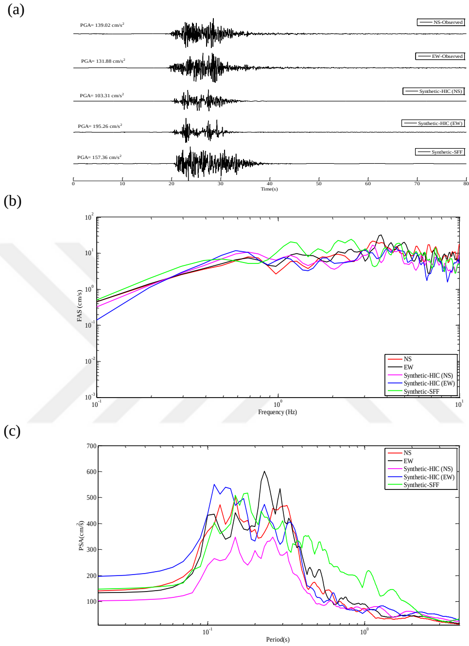
Figure 5.36 Station GSA; (a) Observed and simulated accelerograms (b) Fourier amplitude spectra (c) Response spectra with 5% damping obtained for observed (NS and EW) and simulated horizontal components (Synthetic-SFF and Synthetic-HIC)
