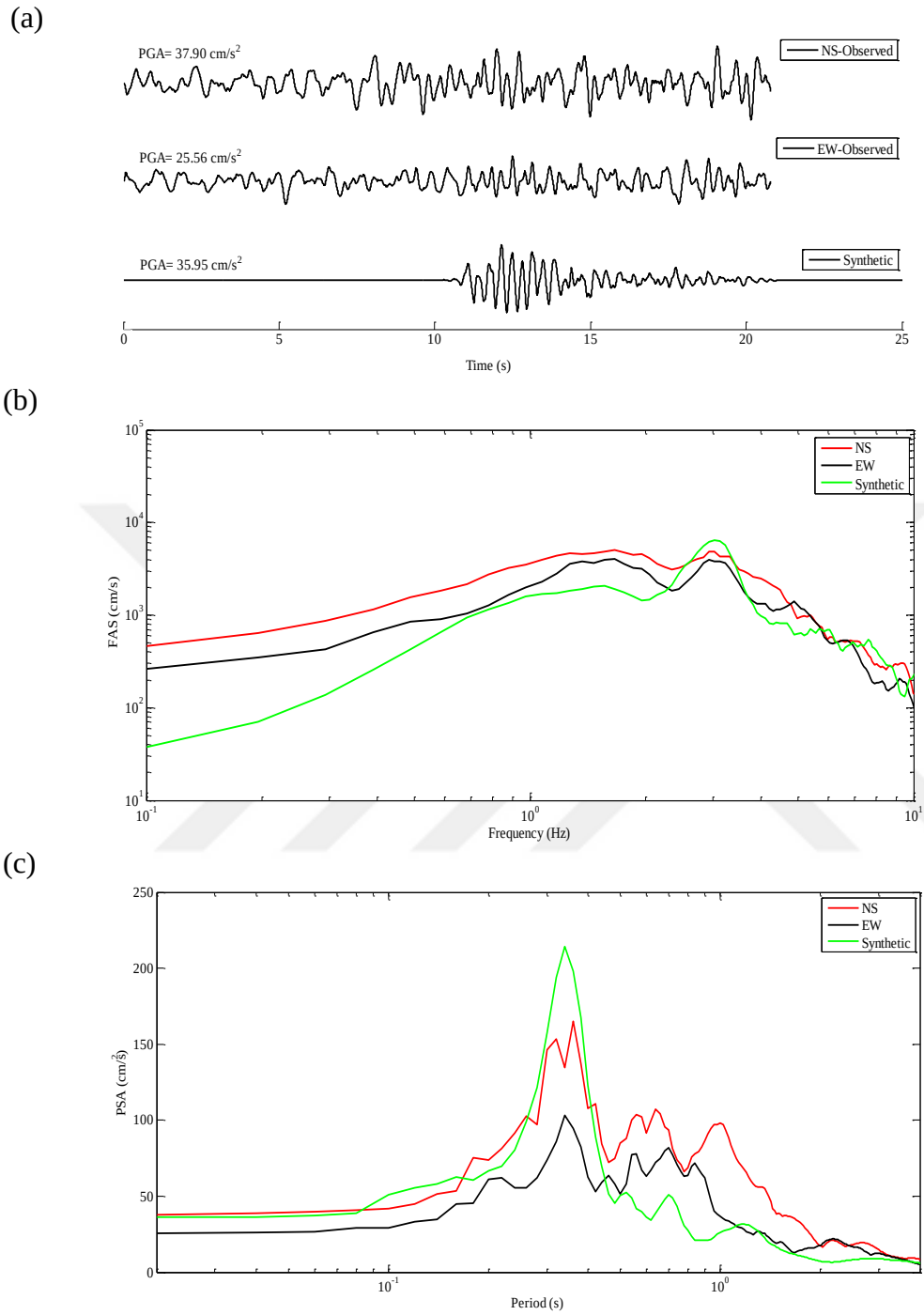
Figure 5.7 Station TER; (a) Observed and simulated accelerograms (b) Fourier Amplitude Spectra (c) Response Spectra with 5% damping obtained for observed (NS and EW) and simulated horizontal component (Synthetic)
