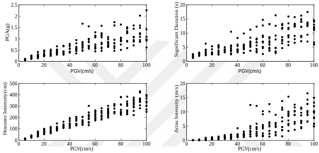
Figure 4.19 Distribution of the ground motion parameters for the first set of motions
