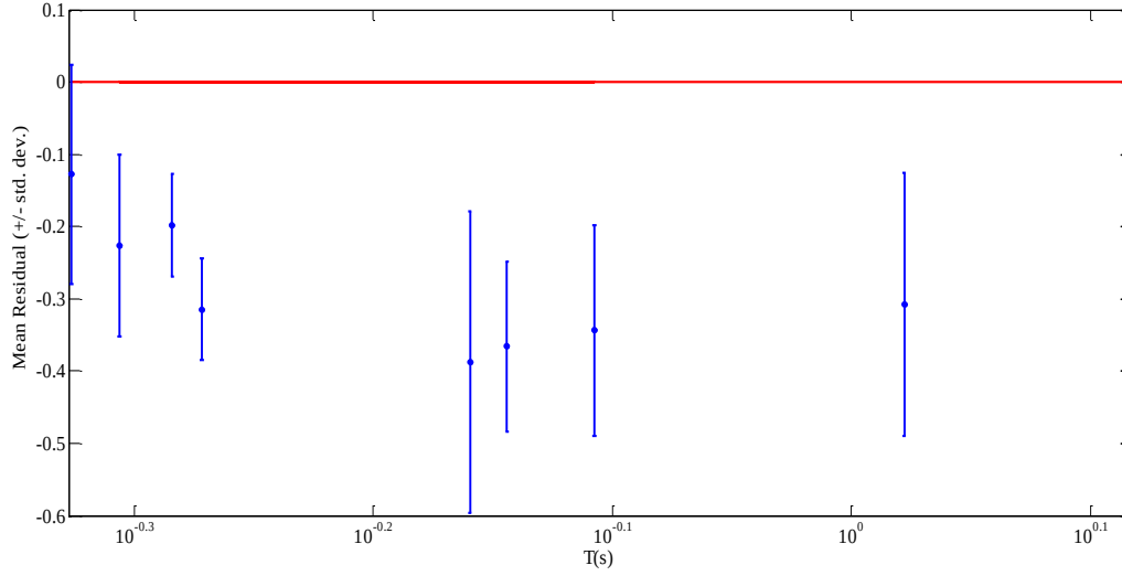
Figure F.3 Average of residuals over all simulated Erzincan records versus period of frames, where residual = \log(\text{Predicted NR}) - \log(\text{Observed NR}) . Standard deviation of residuals is depicted by error bars.
