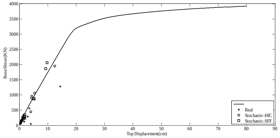
Figure E.27 Capacity Curve and Dynamic Responses of L'Aquila Earthquake for F9-8S3B
