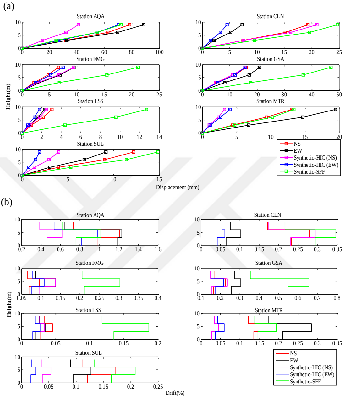
Figure 5.41 Distribution of (a): maximum story displacements and (b): maximum drift ratios due to the real and simulated records of L'Aquila Earthquake – F2-3S2B
