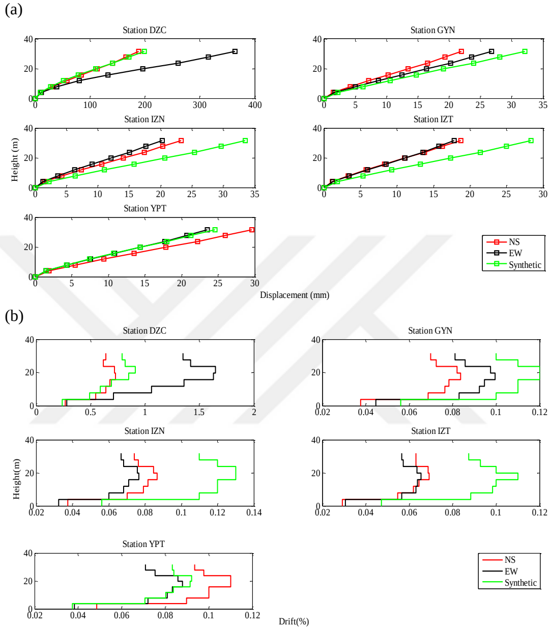
Figure 5.31 Distribution of (a): maximum story displacements and (b): maximum drift ratios due to the real and simulated records of Düzce Earthquake – F9-8S3B
