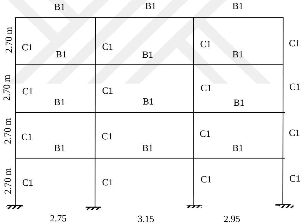
Figure D.5 Frame F5-4S
