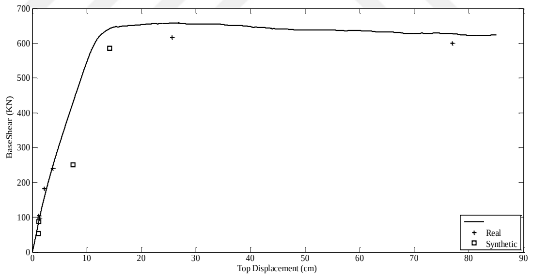
Figure E.8 Capacity Curve and Dynamic Responses of Erzincan Earthquake for F8-7S3B
