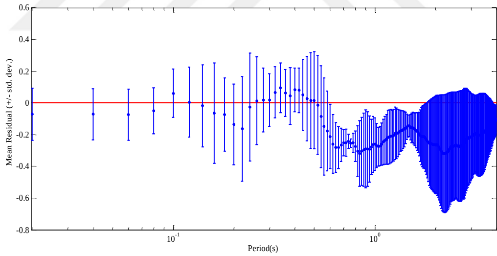
Figure F.2 Average of residuals over all simulated Erzincan records versus period, where residual = \log(\text{Predicted RS}) - \log(\text{Observed RS}) . Standard deviation of residuals is depicted by error bars.
