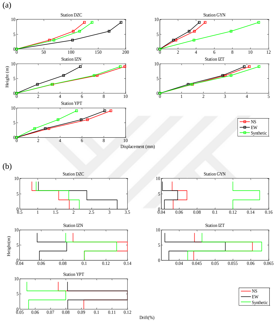
Figure 5.24 Distribution of (a): maximum story displacements and (b): maximum drift ratios due to the real and simulated records of Düzce Earthquake – F2-3S2B
