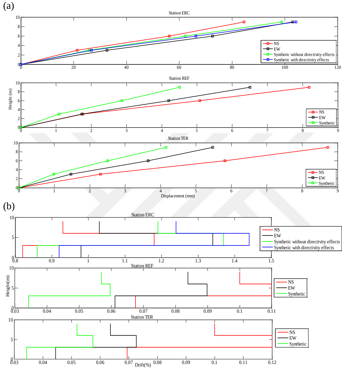
Figure 5.8 Distribution of (a) maximum story displacements and (b) maximum drift ratios due to the real and simulated records of Erzincan Earthquake – F1-3S2B
