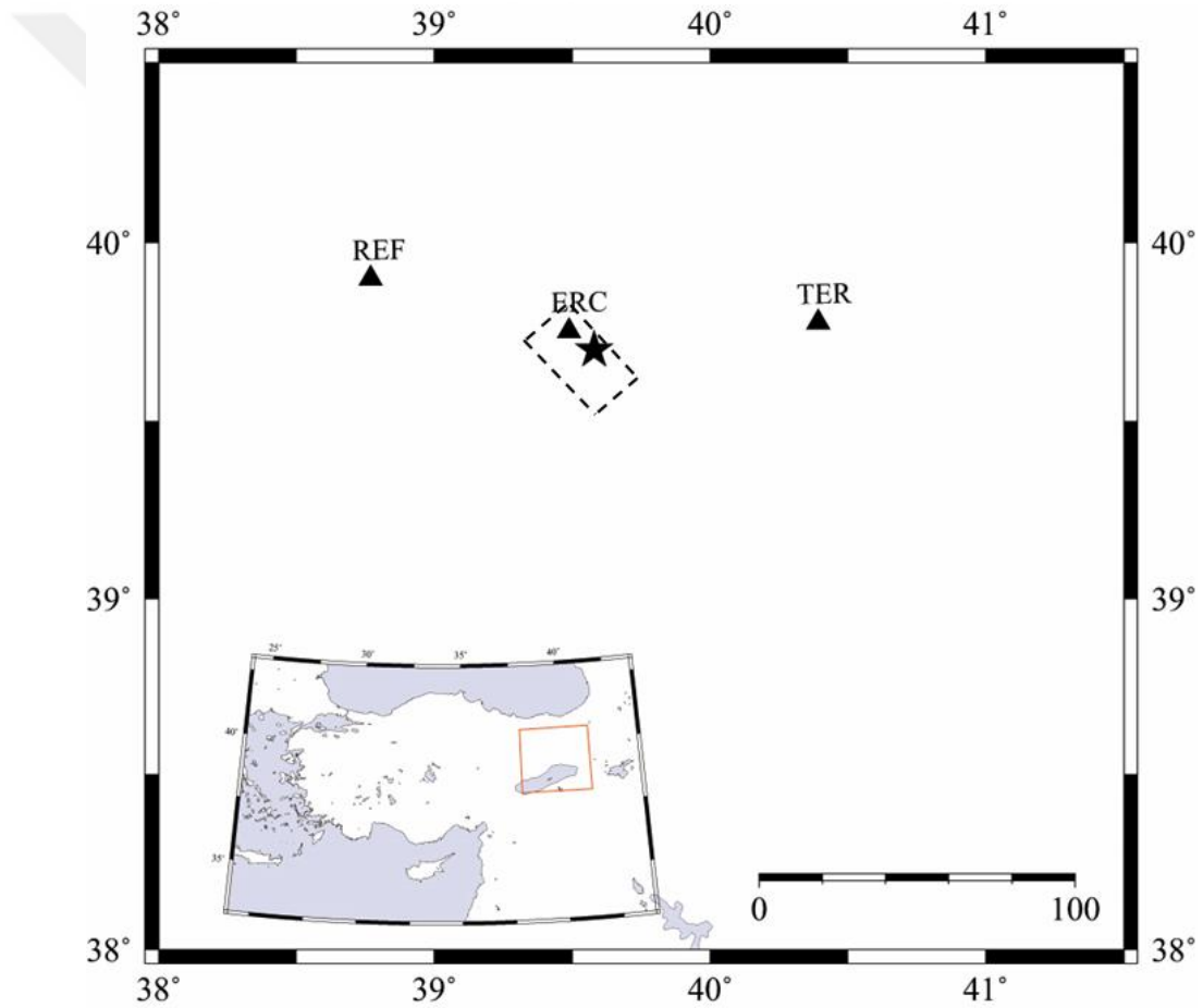
Figure 5.4 Map showing the fault plane and epicenter of the 1992 Erzincan earthquake with the locations of the stations
