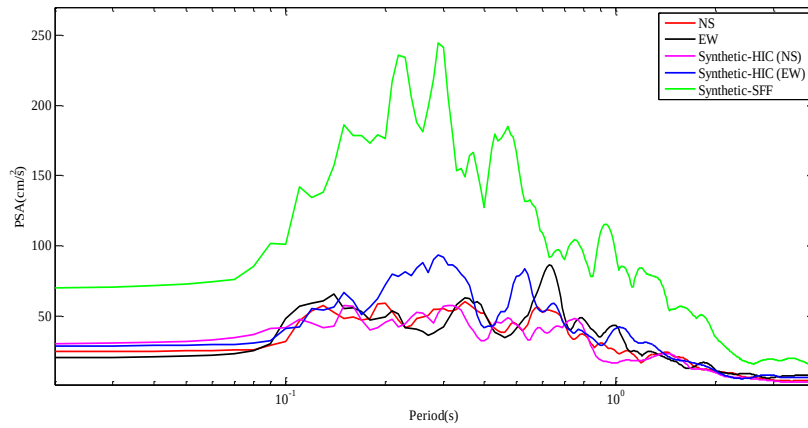
Figure 5.35 Station FMG; (a) Observed and simulated accelerograms (b) Fourier amplitude spectra (c) Response spectra with 5% damping obtained for observed (NS and EW) and simulated horizontal components (Synthetic-SFF and Synthetic-HIC)
