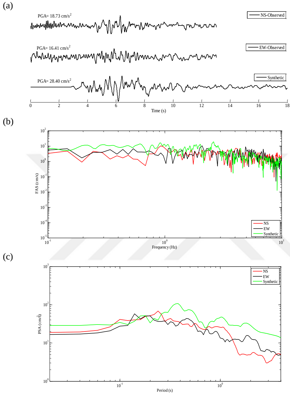
Figure 5.21 Station IZT; (a) Observed and simulated accelerograms (b) Fourier amplitude spectra (c) Response spectra with 5% damping obtained for observed (NS and EW) and simulated horizontal component (Synthetic)
