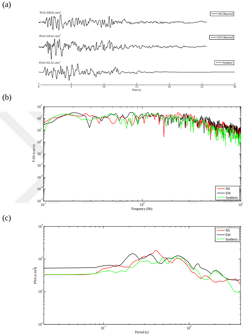
Figure 5.18 Station DZC; (a) Observed and simulated accelerograms (b) Fourier amplitude spectra (c) Response spectra with 5% damping obtained for observed (NS and EW) and simulated horizontal component (Synthetic)
