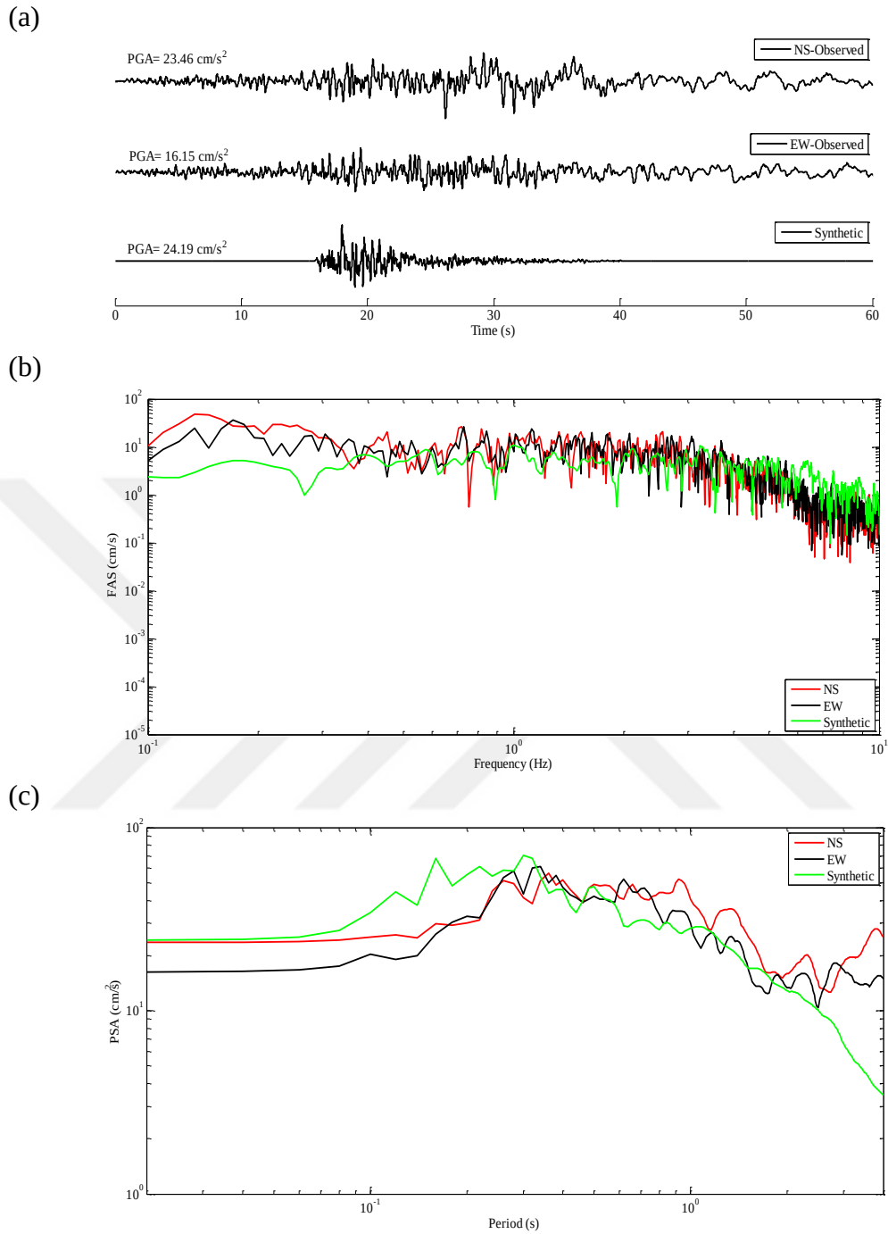
Figure 5.22 Station YPT; (a) Observed and simulated accelerograms (b) Fourier amplitude spectra (c) Response spectra with 5% damping obtained for observed (NS and EW) and simulated horizontal component (Synthetic)
