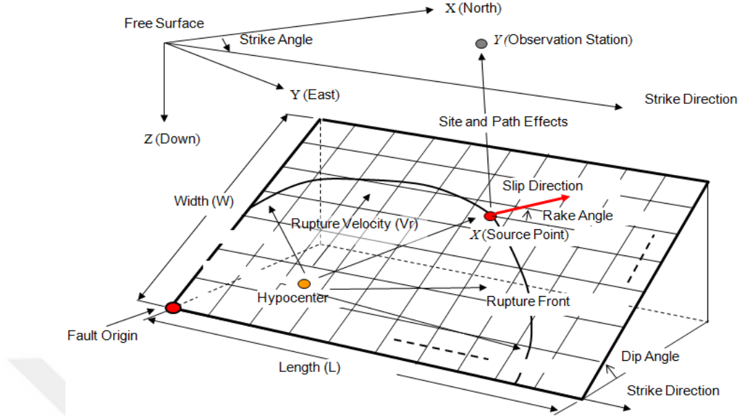
Figure 2.2 Wave propagation on a rectangular finite-fault model (Adapted from Hisada, 2008)
