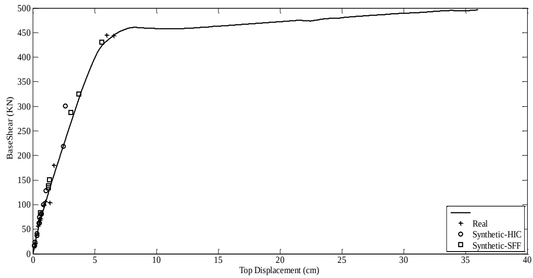
Figure E.21 Capacity Curve and Dynamic Responses of L'Aquila Earthquake for F3-3S3B
