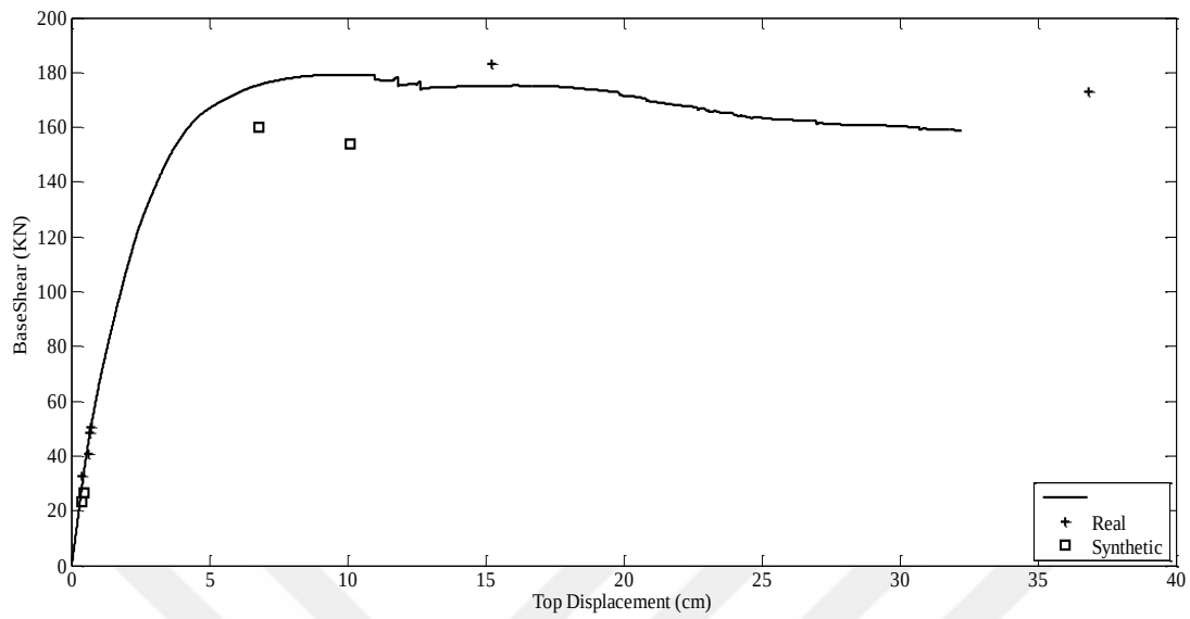
Figure E.5 Capacity Curve and Dynamic Responses of Erzincan Earthquake for F5-4S3B
