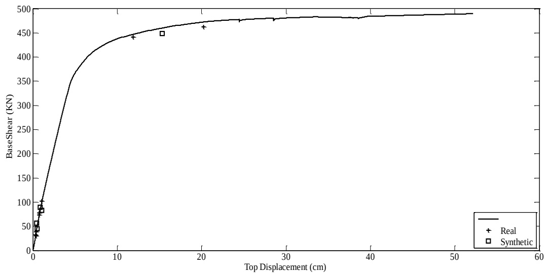
Figure E.13 Capacity Curve and Dynamic Responses of Düzce Earthquake for F4-4S3B
