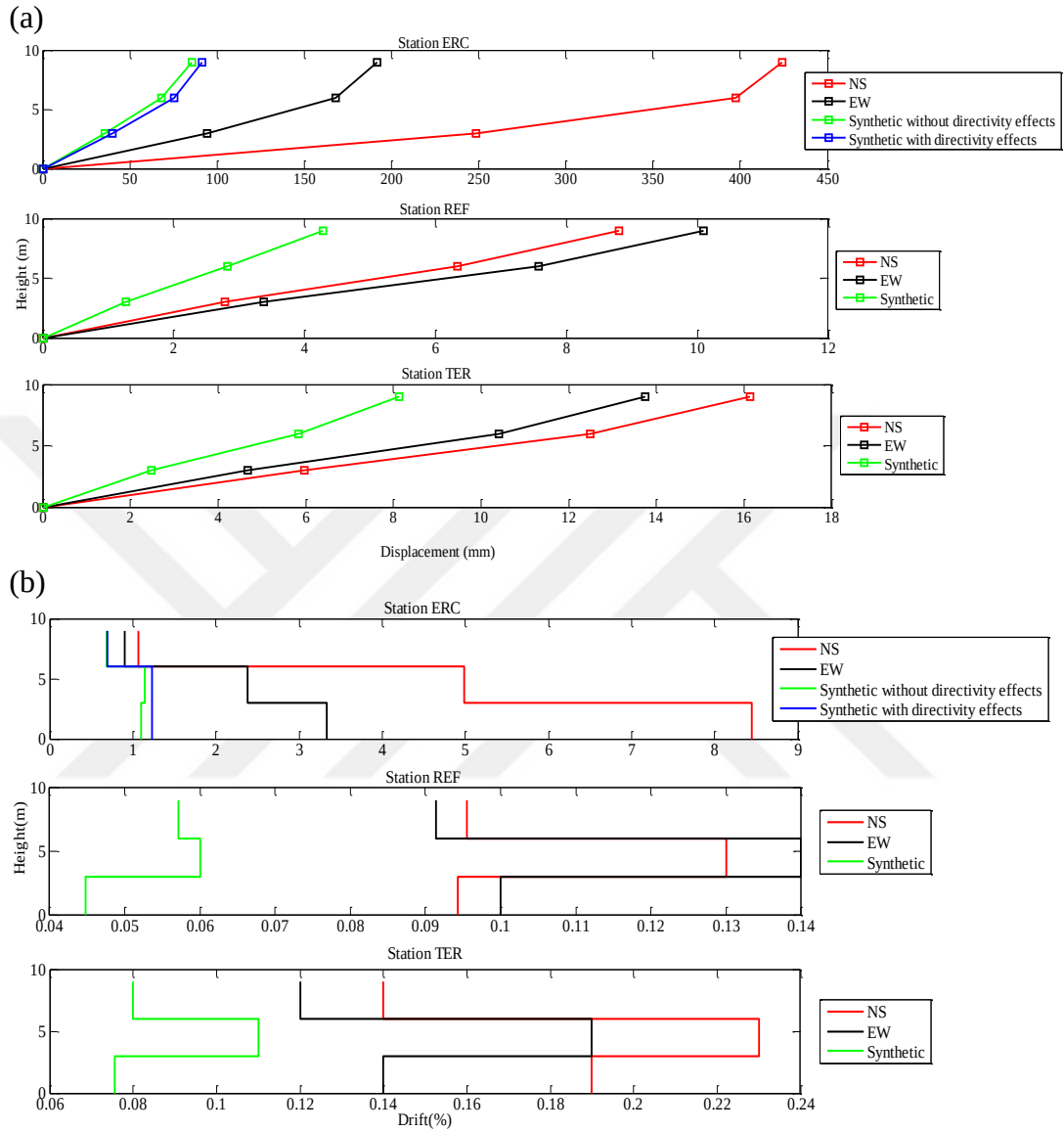
Figure 5.9 Distribution of (a) maximum story displacements and (b) maximum drift ratios due to the real and simulated records of Erzincan Earthquake – F2-3S2B
