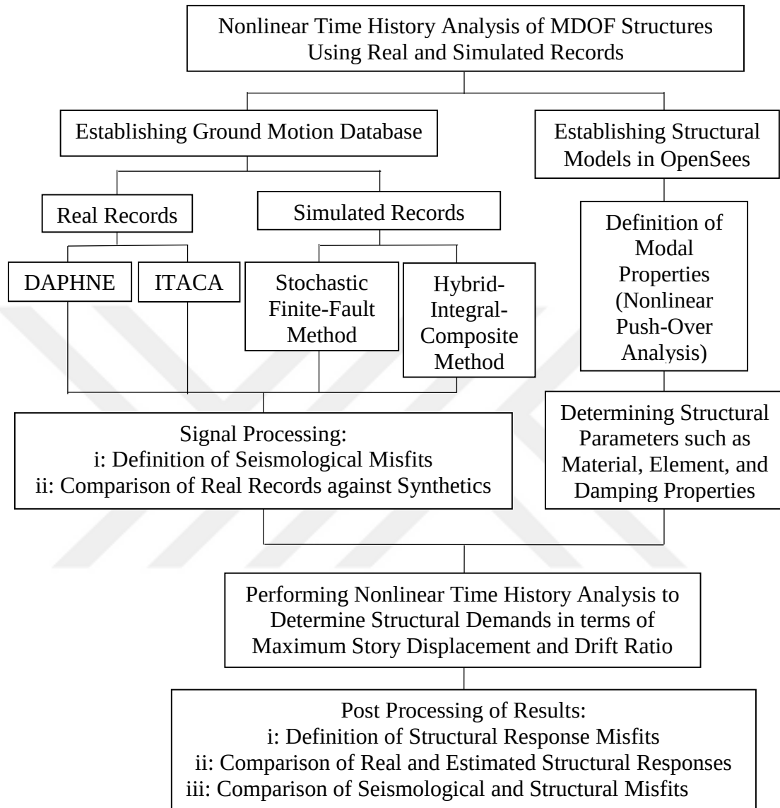
Figure 5.1 Main steps for NTHA of MDOF structures used in this study
