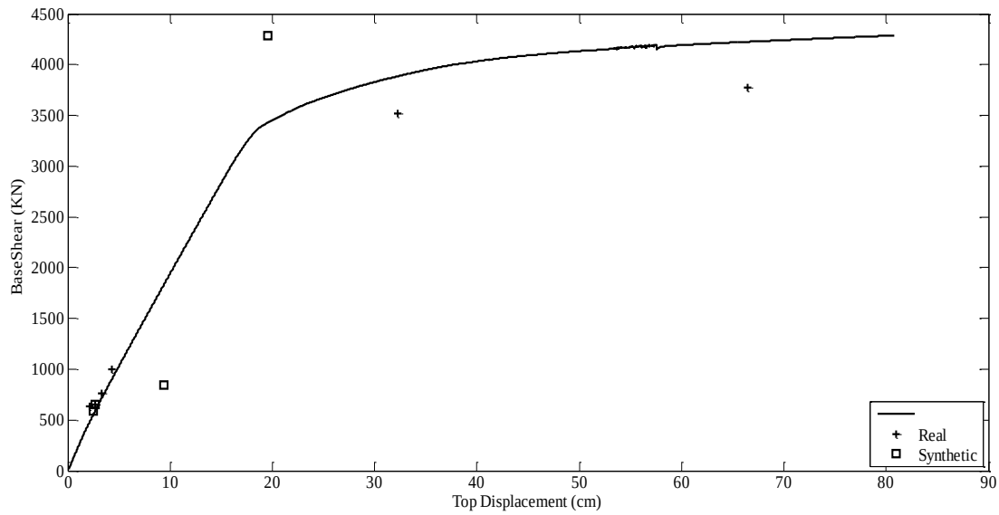
Figure E.9 Capacity Curve and Dynamic Responses of Erzincan Earthquake for F9-8S3B
