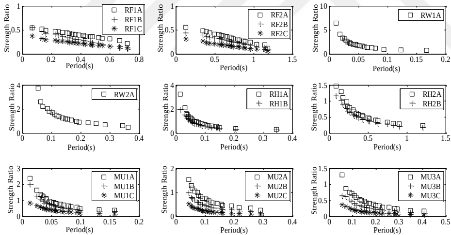
Figure 4.21 Period and strength ratio pairs generated by LHS technique for all sub-classes
