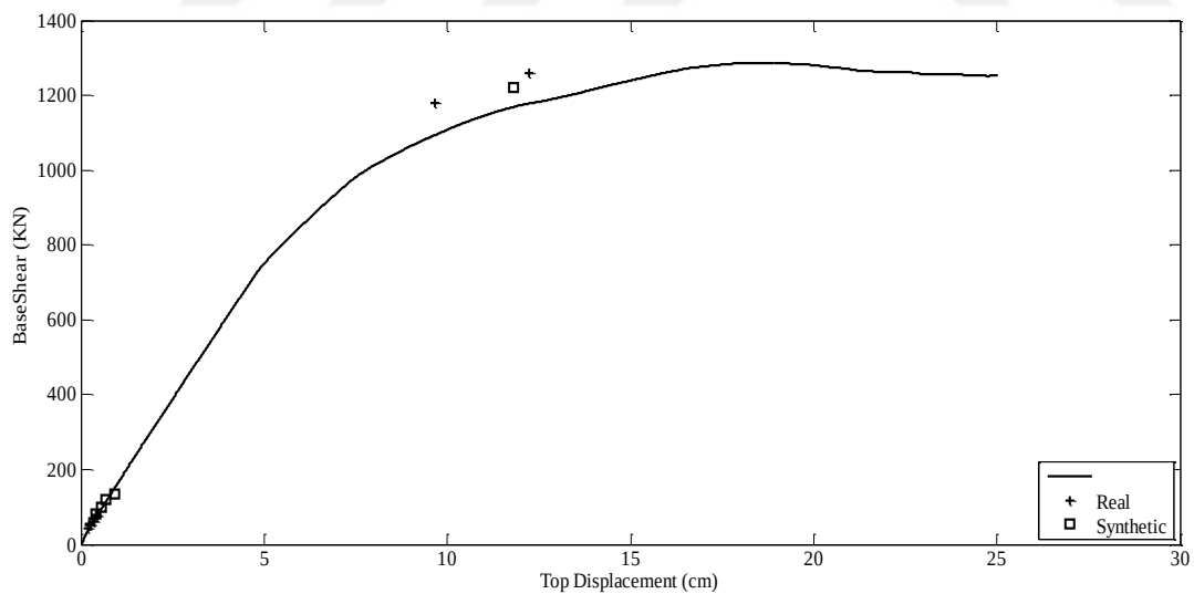
Figure E.10 Capacity Curve and Dynamic Responses of Düzce Earthquake for F1-3S2B
