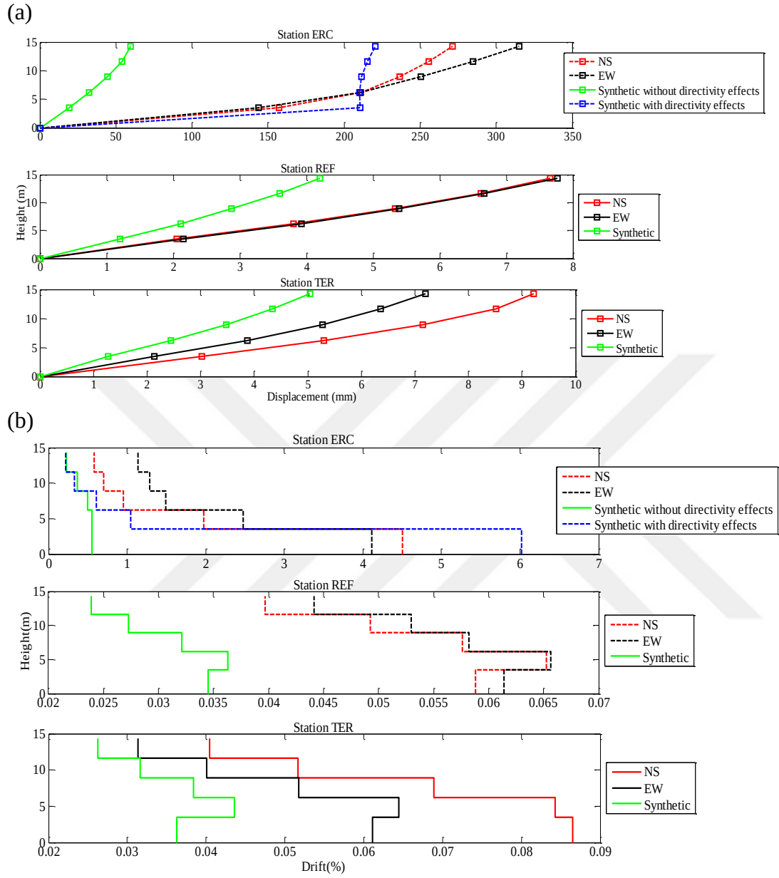
Figure 5.14 Distribution of (a) maximum story displacements and (b) maximum drift ratios due to the real and simulated records of Erzincan Earthquake – F7-5S4B
