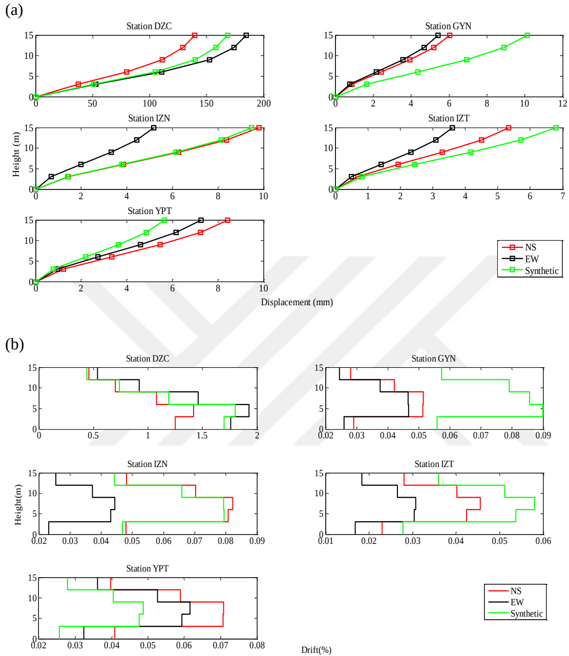
Figure 5.28 Distribution of (a): maximum story displacements and (b): maximum drift ratios due to the real and simulated records of Düzce Earthquake – F6-5S2B
