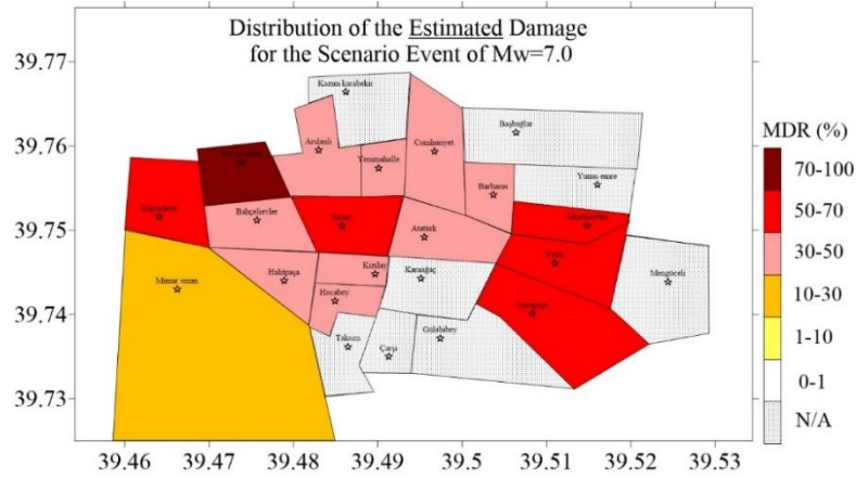
Figure 4.44 Spatial distribution of the estimated (a) PGA (b) PGV (c) MDR in the Erzincan region for scenario event of Mw=7.0
