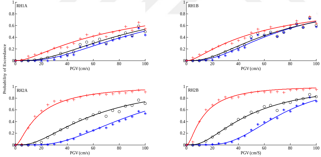
Figure 4.27 Fragility curves for RH sub-classes using records categorized based on (a) PGA and (b) PGV where the red lines correspond to LS_1 , the black lines to LS_2 , and the blue lines to LS_3
