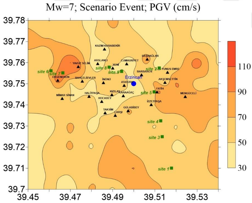
Figure 4.15 Spatial distribution of the simulated (a) PGA (b) PGV values of the scenario earthquake with Mw=7.0 in Erzincan region
