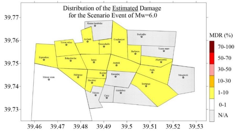
Figure 4.42 Spatial distribution of the estimated (a) PGA (b) PGV (c) MDR in the Erzincan region for scenario event of Mw=6.0
