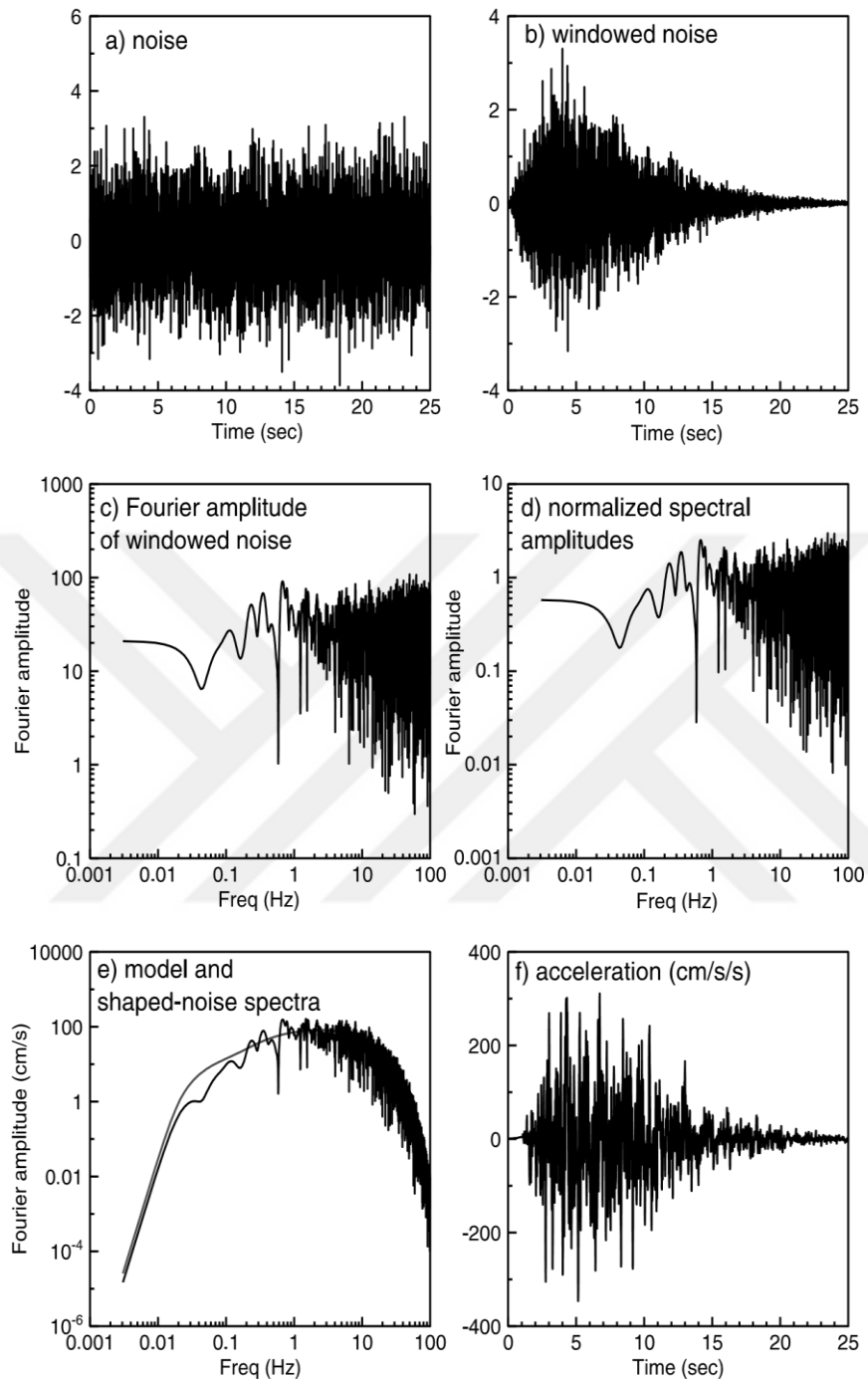
Figure 2.1 Step by step stochastic point-source modeling procedure (Adapted from Boore, 2003)
