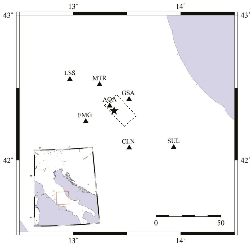
Figure 5.32 Map showing the fault plane and epicenter of 2009 L'Aquila earthquake with the locations of the selected stations
