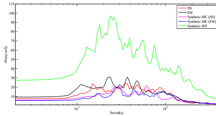
Figure 5.37 Station LSS; (a) Observed and simulated accelerograms (b) Fourier amplitude spectra (c) Response spectra with 5% damping obtained for observed (NS and EW) and simulated horizontal components (Synthetic-SFF and Synthetic-HIC)
