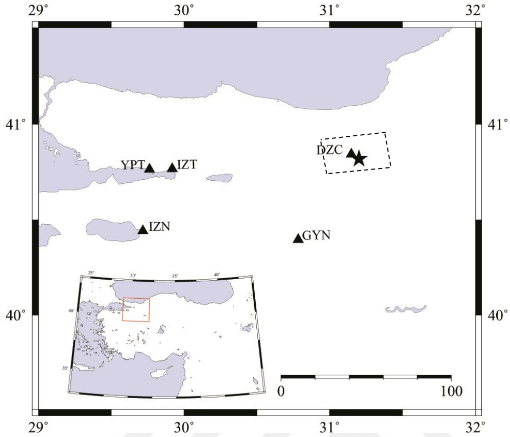
Figure 5.17 Map showing the fault plane and epicenter of the 1999 Düzce earthquake with the locations of the stations
