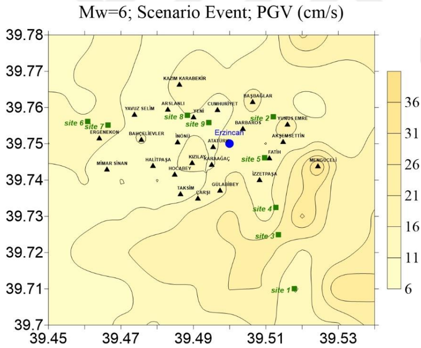
Figure 4.13 Spatial distribution of the simulated (a) PGA (b) PGV values of the scenario earthquake with Mw=6.0 in Erzincan region
