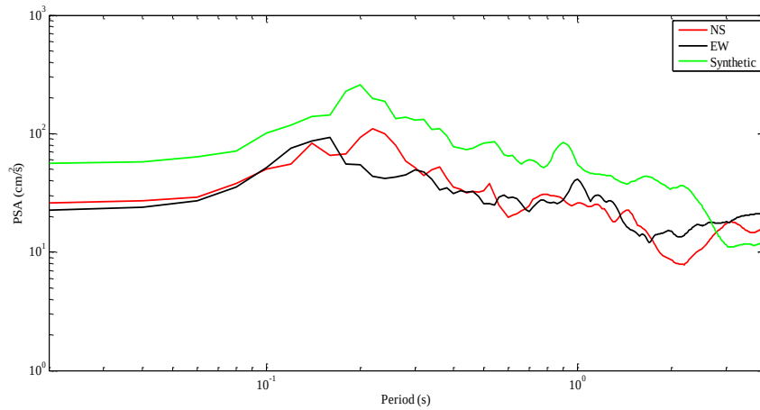
Figure 5.19 Station GYN; (a) Observed and simulated accelerograms (b) Fourier amplitude spectra (c) Response spectra with 5% damping obtained for observed (NS and EW) and simulated horizontal component (Synthetic)
