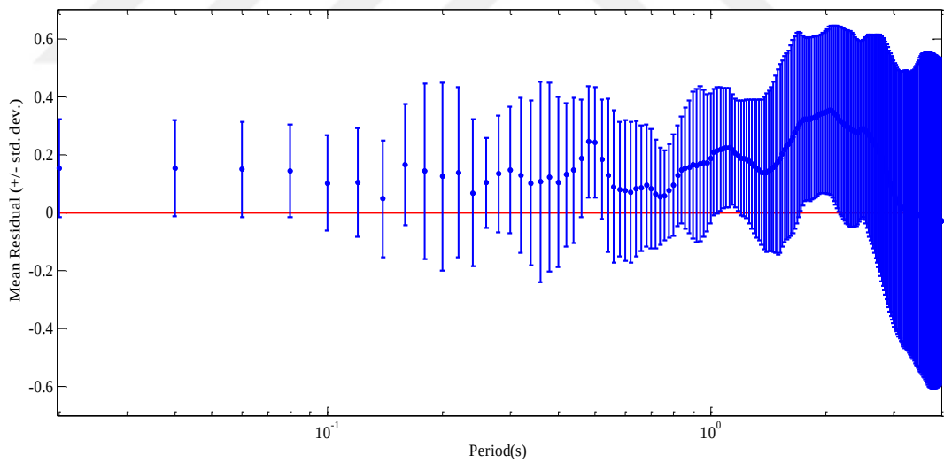
Figure F.5 Average of residuals over all simulated Düzce records versus period, where residual = \log(\text{Predicted RS}) - \log(\text{Observed RS}) . Standard deviation of residuals is depicted by error bars.
