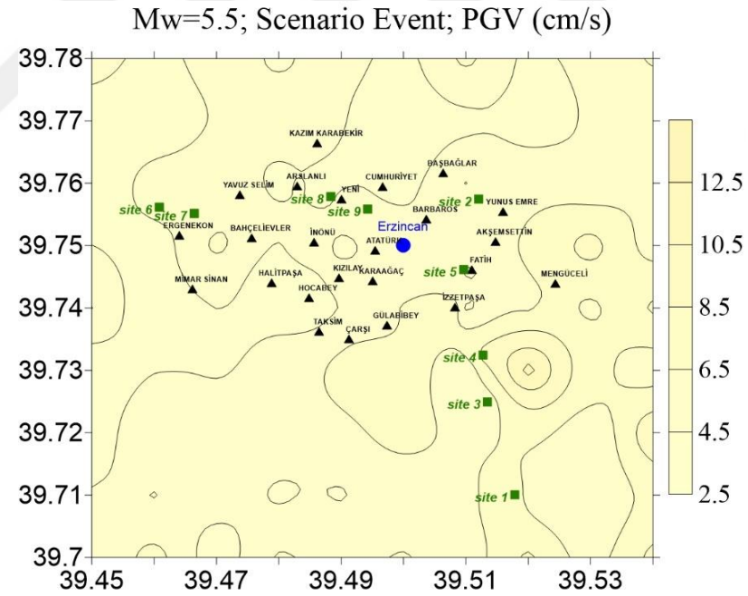
Figure 4.12 Spatial distribution of the simulated (a) PGA (b) PGV values of the scenario earthquake with Mw=5.5 in Erzincan region
