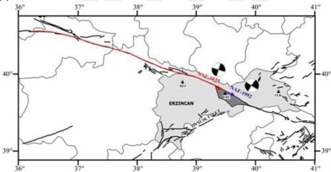
Figure 4.2 (a) Major tectonic structures around the Anatolian plate and large earthquakes on the North Anatolian Fault Zone in the last century (b) Seismotectonics in the Erzincan region with the fault systems and the epicenters of the 1939 and 1992 events (Figures 4.2.a and 4.2.b are adapted from Akyüz et. al. , 2002 and Askan et al. , 2013, respectively)
