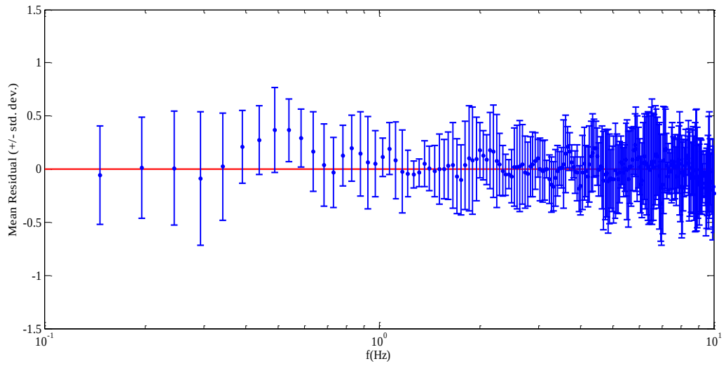
Figure F.4 Average of residuals over all simulated Düzce records versus frequency, where residual = \log(\text{Predicted FAS}) - \log(\text{Observed FAS}) . Standard deviation of residuals is depicted by error bars.
