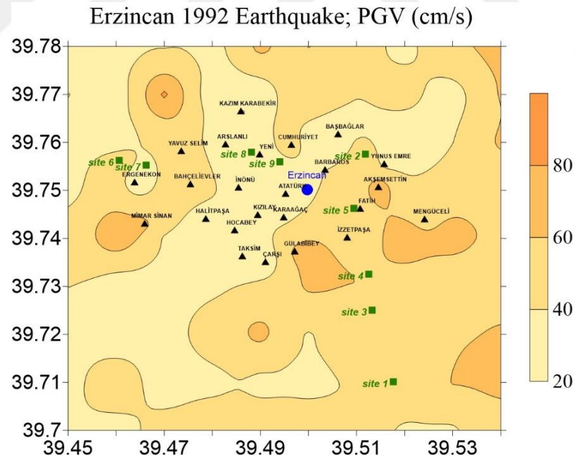
Figure 4.10 Spatial distribution of the simulated (a) PGA (b) PGV values of the 1992 Erzincan earthquake in Erzincan region
