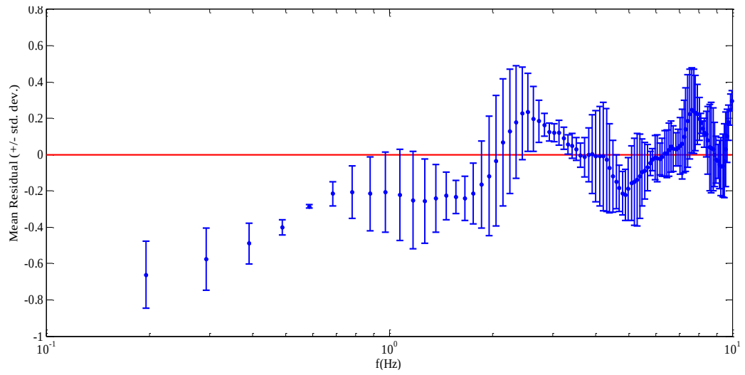
Figure F.1 Average of residuals over all simulated Erzincan records versus frequency, where residual = \log(\text{Predicted FAS}) - \log(\text{Observed FAS}) . Standard deviation of residuals is depicted by error bars.
