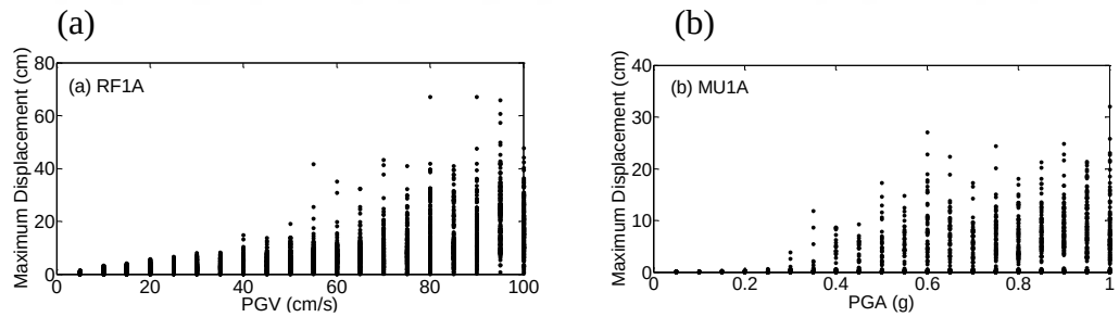
Figure 4.23 Distribution of the response parameter in terms of maximum displacement with respect to ground motion intensity parameter for (a) RF1A and (b) MU1A
