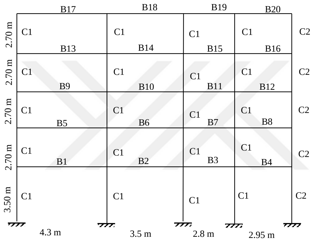
Figure D.7 Frame F7-5S4B
