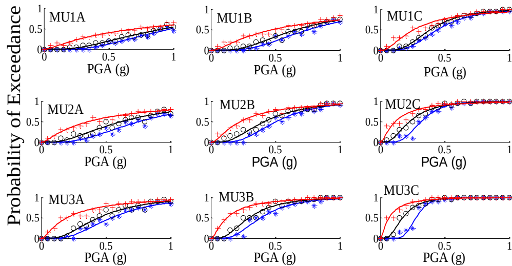
Figure B.2 Fragility curves developed for all masonry subclasses corresponding to records selected with respect to PGA without considering ground motion variability
