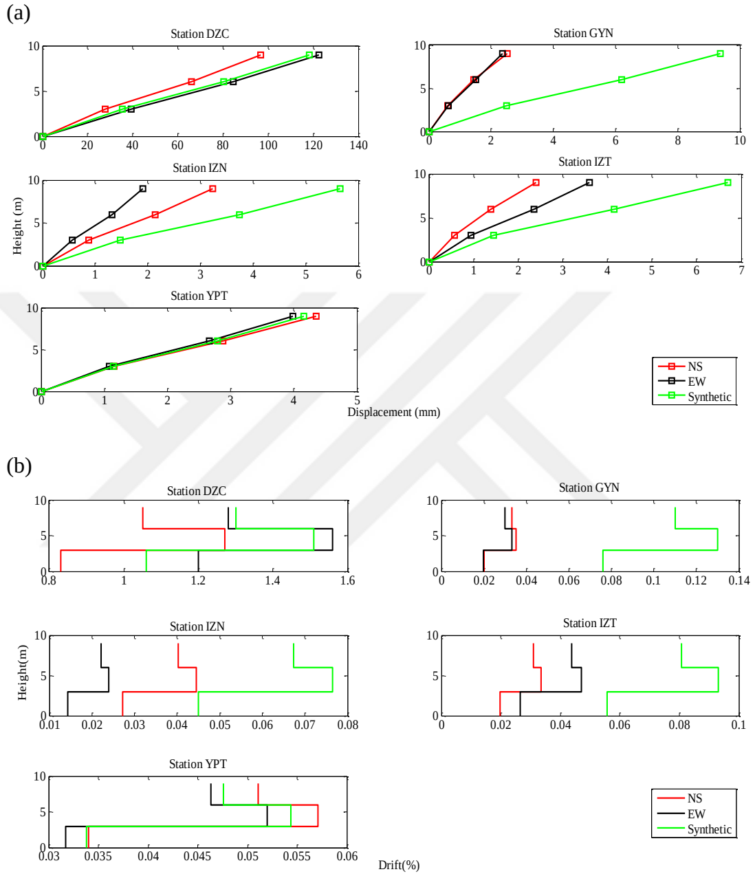
Figure 5.23 Distribution of (a): maximum story displacements and (b): maximum drift ratios due to the real and simulated records of Düzce Earthquake – F1-3S2B
