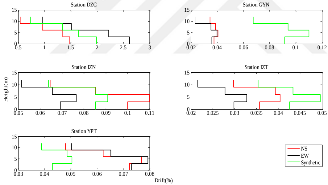
Figure 5.26 Distribution of (a): maximum story displacements and (b): maximum drift ratios due to the real and simulated records of Düzce Earthquake – F4-4S3B
