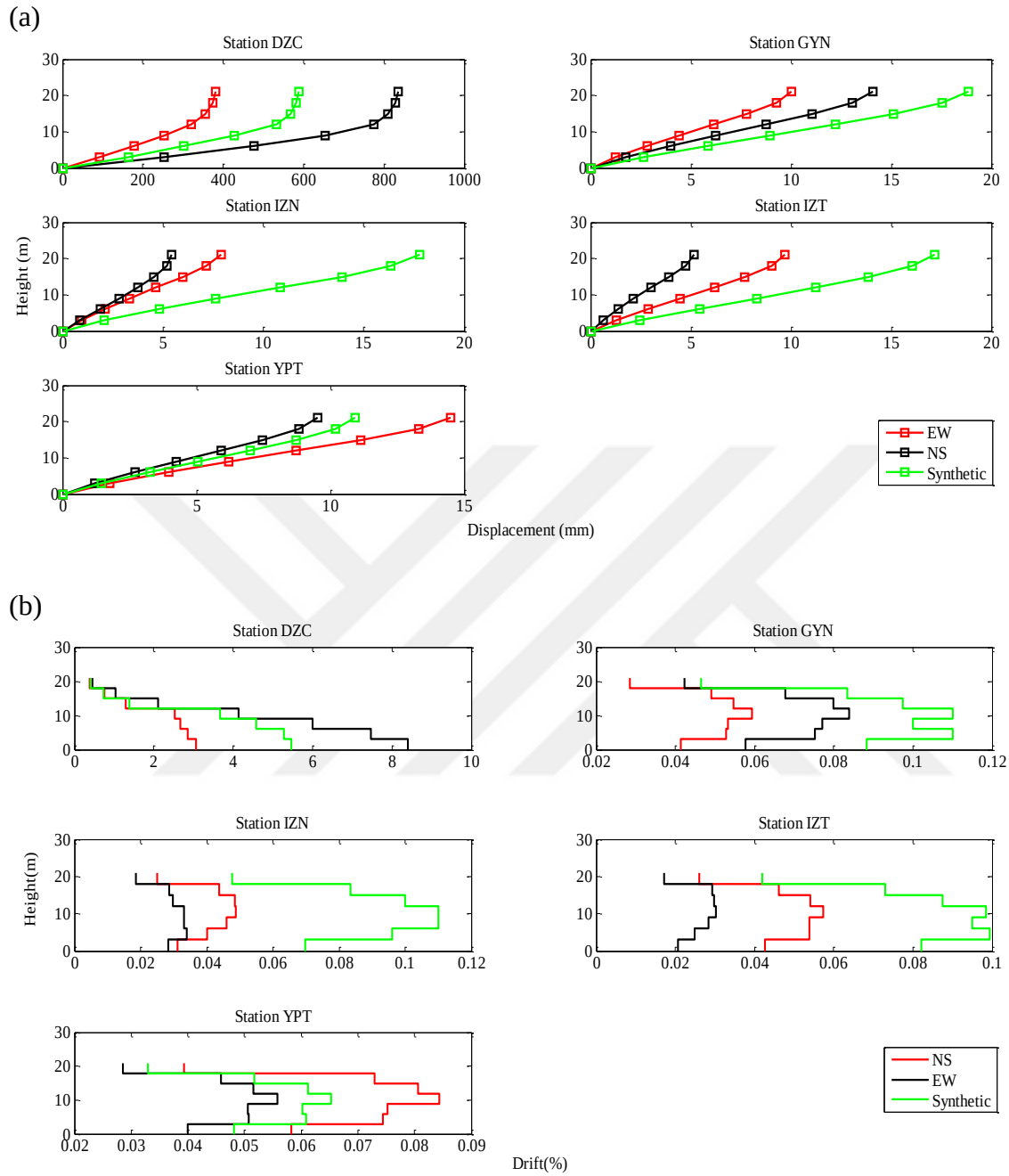
Figure 5.30 Distribution of (a): maximum story displacements and (b): maximum drift ratios due to the real and simulated records of Düzce Earthquake – F8-7S3B
