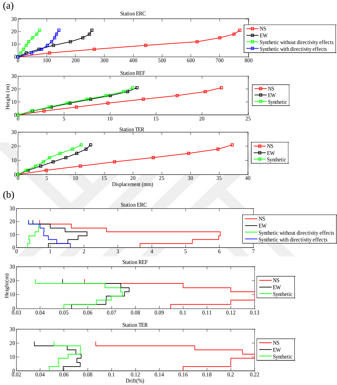
Figure 5.15 Distribution of (a) maximum story displacements and (b) maximum drift ratios due to the real and simulated records of Erzincan Earthquake – F8-7S3B
