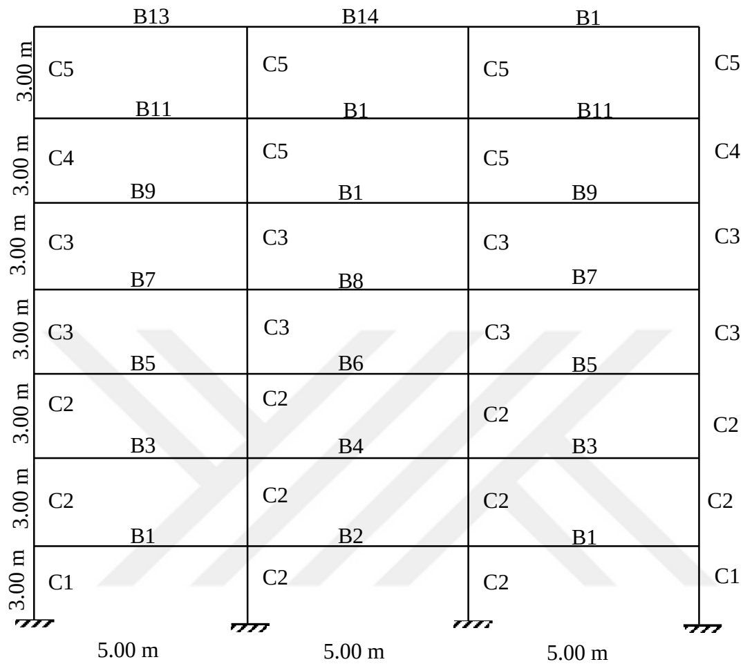
Figure D.8 Frame F8-7S3B
