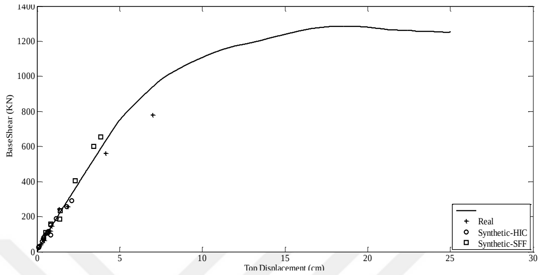
Figure E.19 Capacity Curve and Dynamic Responses of L'Aquila Earthquake for F1-3S2B
