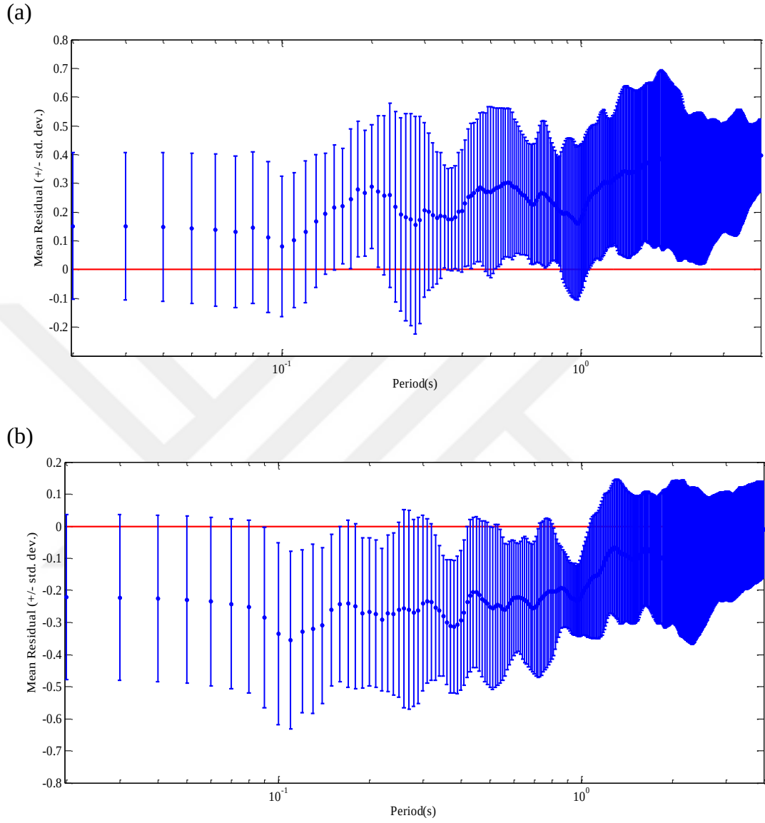
Figure F.8 Average of residuals using (a) Synthetic-SFF and (b) Synthetic-HIC methods over all simulated L'Aquila records versus period, where residual = \log(\text{Predicted RS}) - \log(\text{Observed RS}) . Standard deviation of residuals is depicted by error bars.
