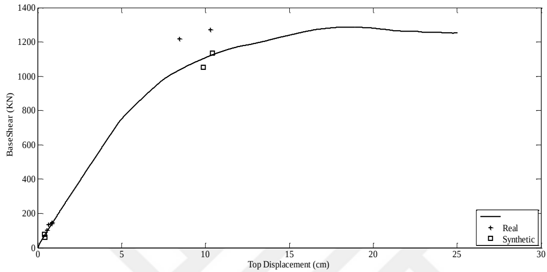
Figure E.1 Capacity Curve and Dynamic Responses of Erzincan Earthquake for F1-3S2B
