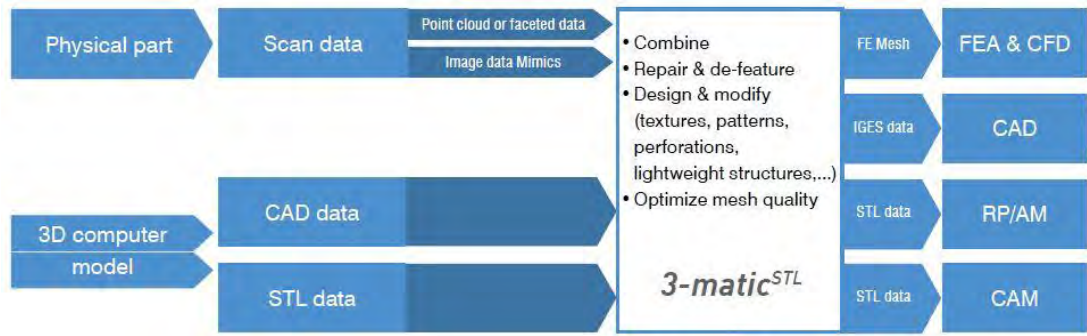
Figure 4.9 Workflow and Features of 3-matic STL (“3-matic STL | Software for Additive Manufacturing,” n.d.)
