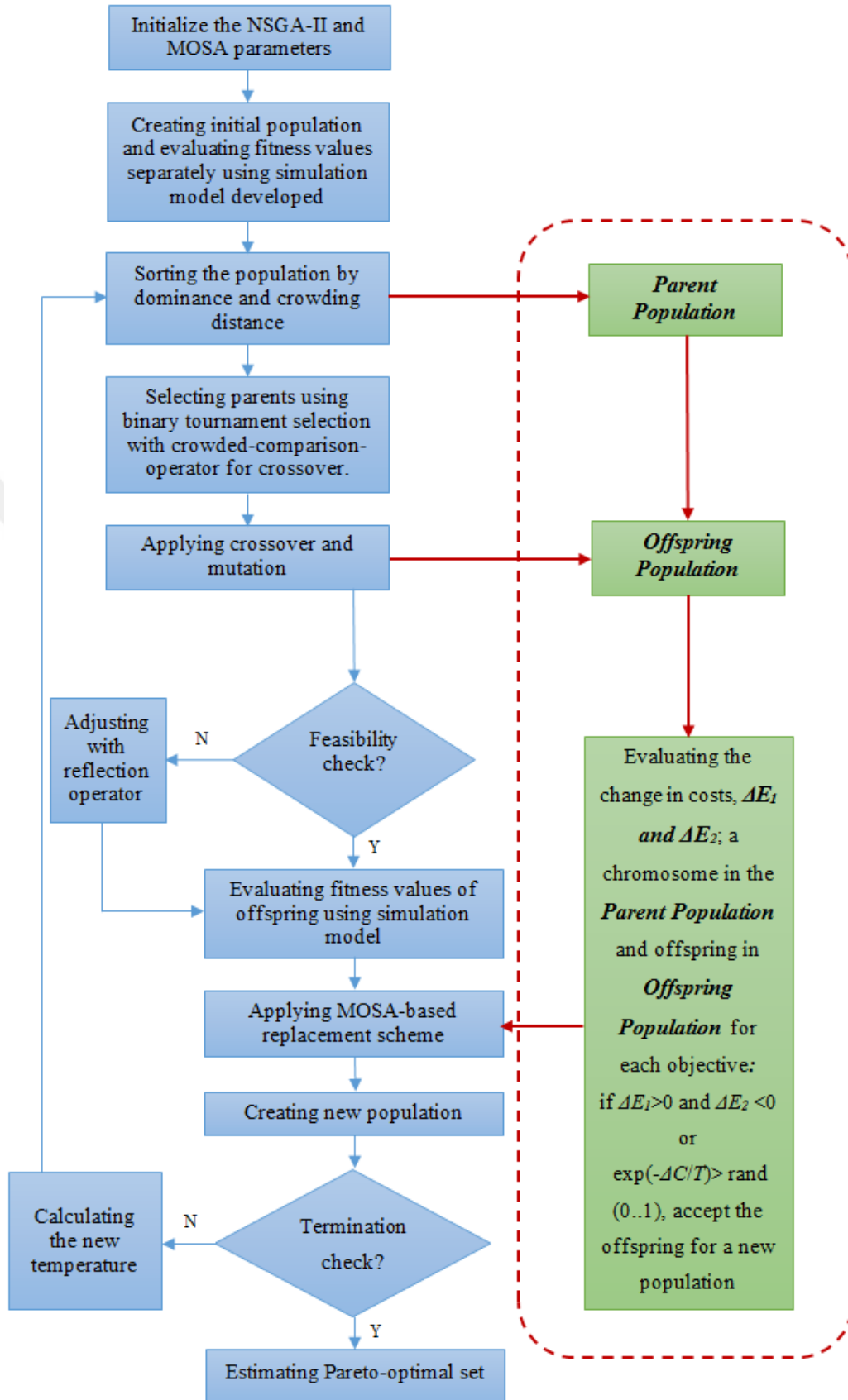
Figure 5.1 The control logic of the proposed MOHEA.
