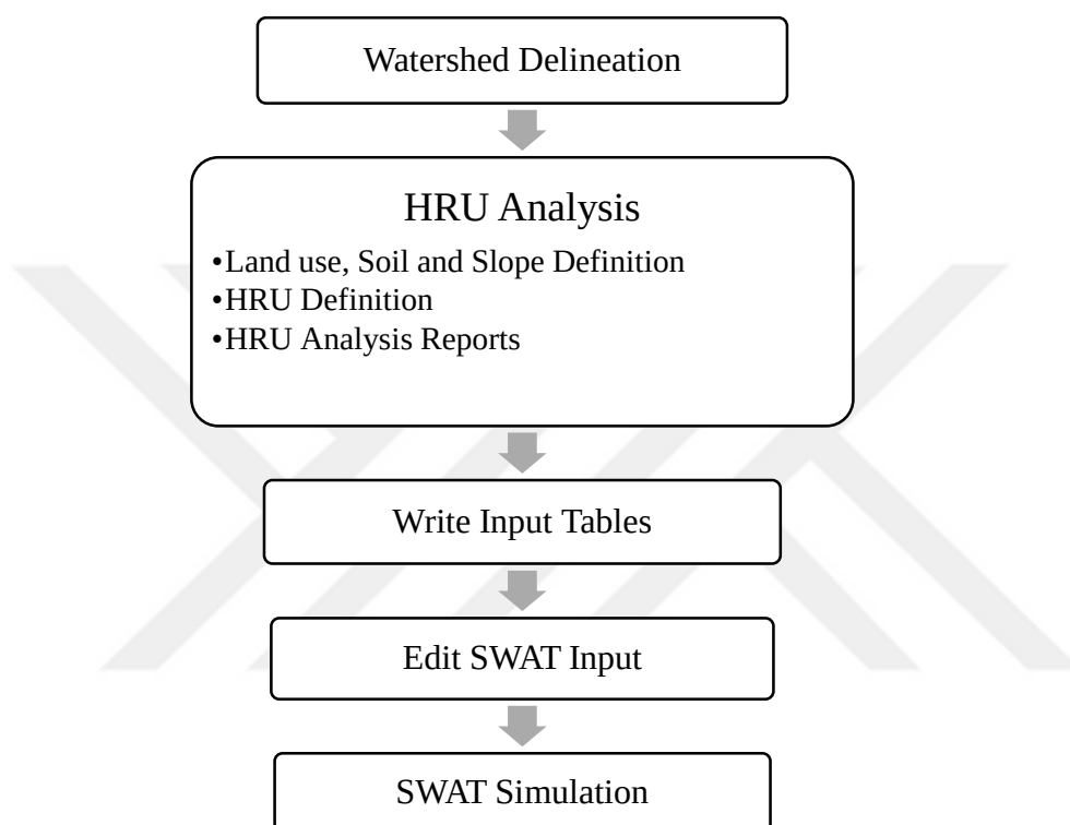
Figure 58. SWAT model construction steps: HRU Analysis
