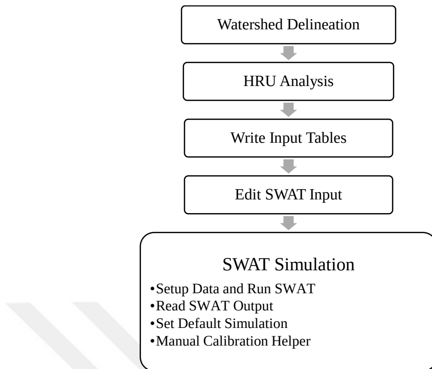
Figure 61. SWAT model construction steps: SWAT Simulation
