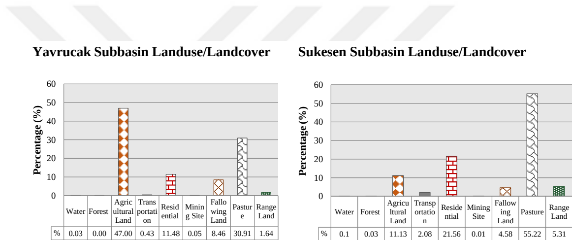
Figure 25. Sukesen and Yavrucak subbasins' landuse percentages
