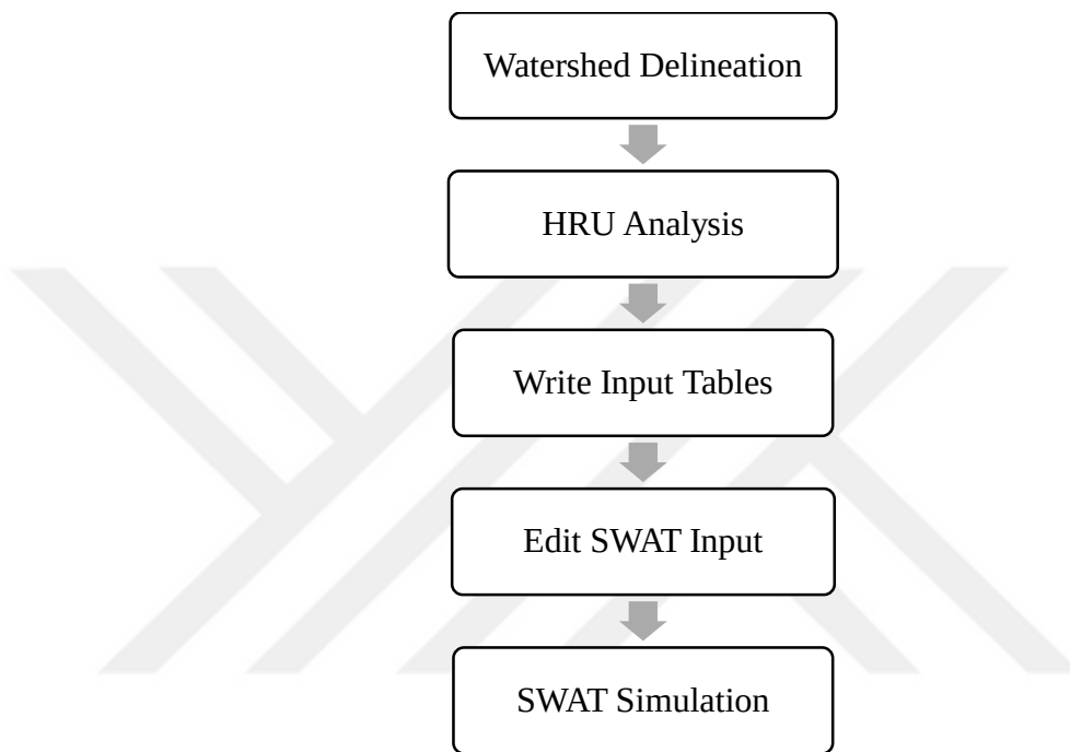
Figure 11. Steps to setup a SWAT model project
