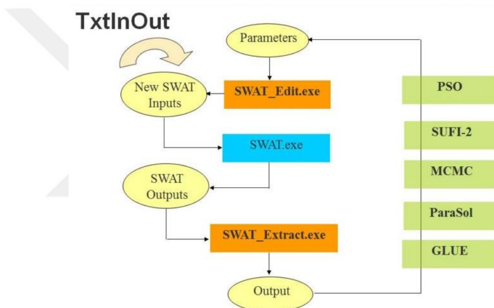
Figure 62. Schematic diagram of the linkage between SWAT-CUP and optimization procedures (Abbaspour, 2015)
