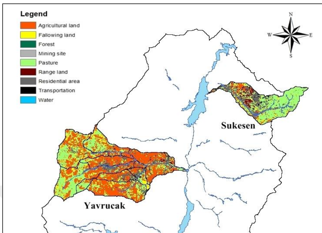
Figure 26. Land use map of Yavrucak and Sukesen subbasins
