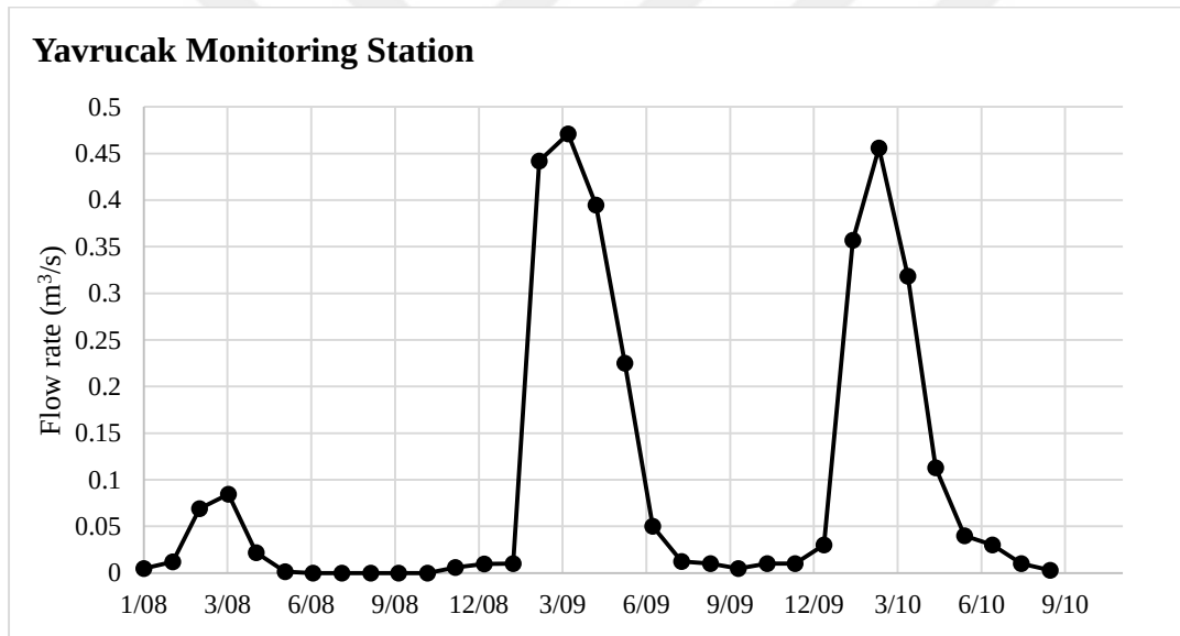
Figure 12. Observed streamflow values at Yavrucak monitoring station
