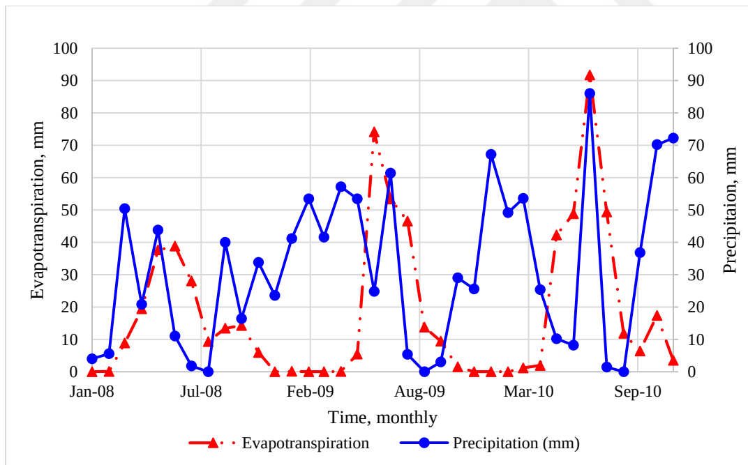
Figure 18. Comparison of precipitation and evapotranspiration in Yavrucak subbasin
