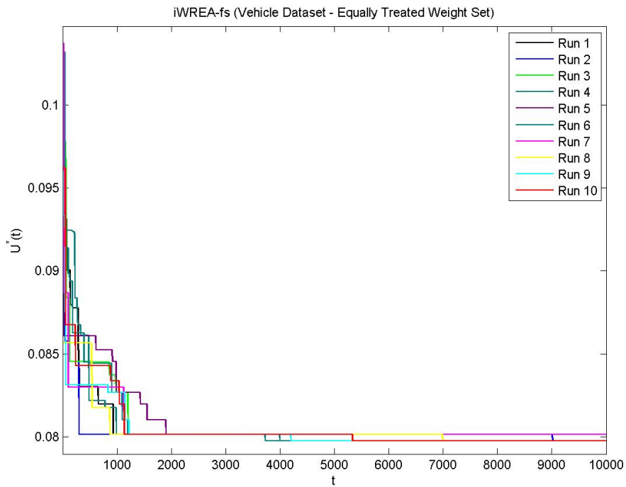
Figure B.17 Vehicle – Equally Treated – iWREA-fs
