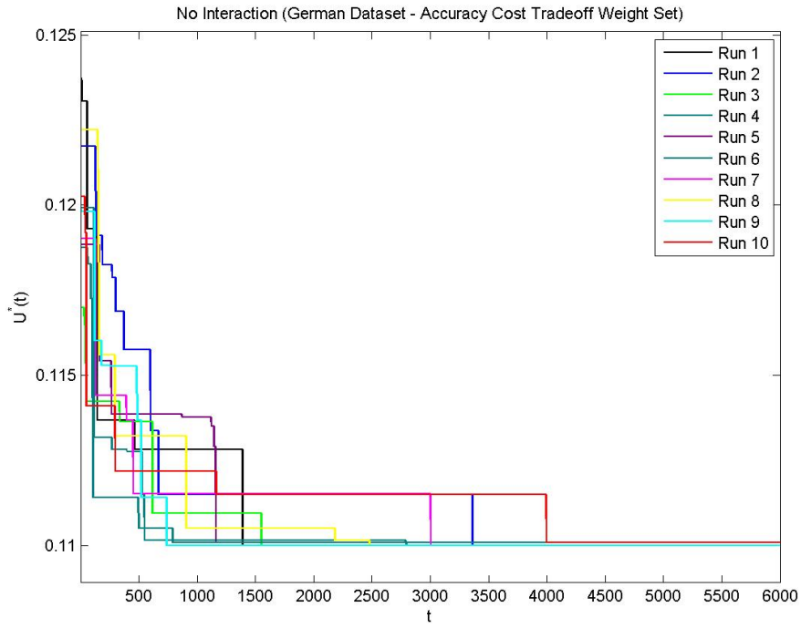
Figure B.24 German – Accuracy and Cost Tradeoff – No Interaction
