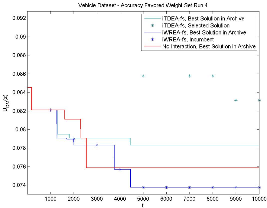
Figure 6.5 4 th replication of quadratic preference function experiments with Accuracy Favored weight set
