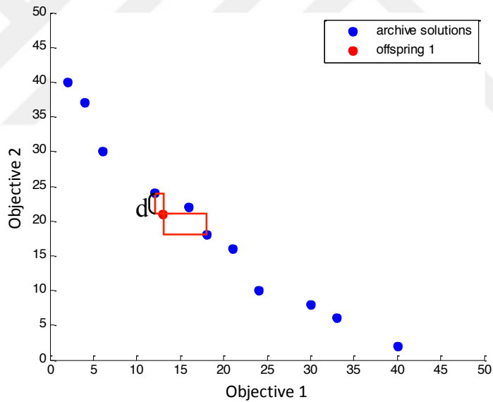
Figure 5.3 Archive update in iTDEA-fs: the offspring is accepted into archive if d \leq \tau .
