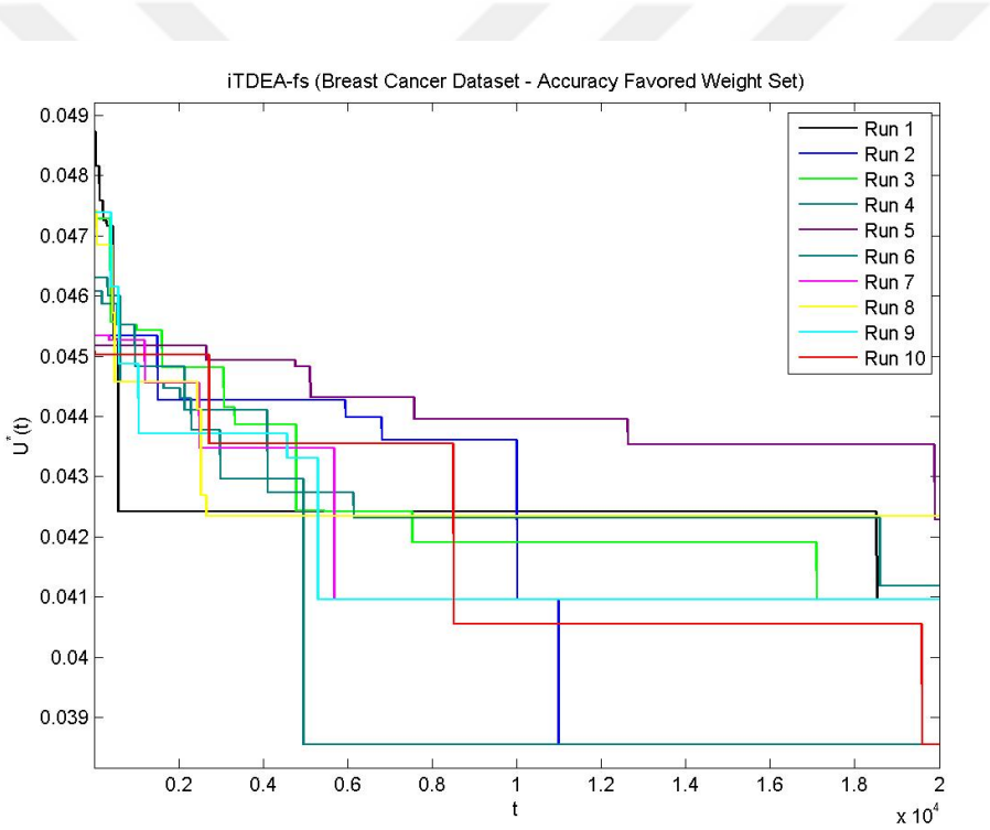
Figure 6.1 Archive progress of iTDEA-fs on Breast Cancer dataset experiments with Accuracy Favored weight set
