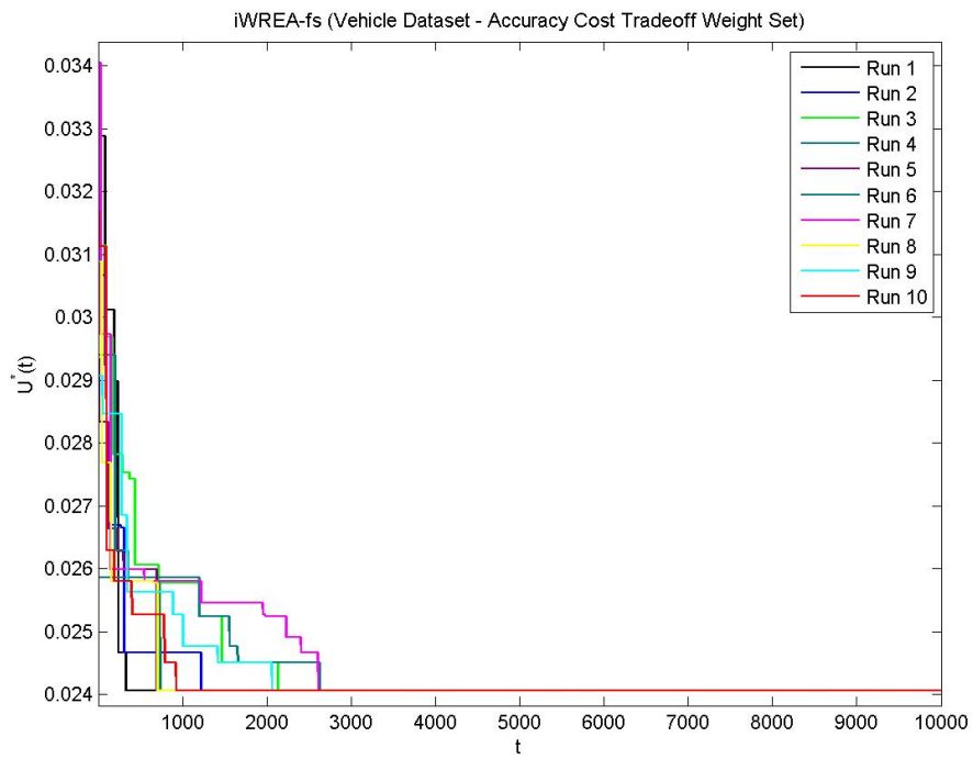
Figure D.5 Accuracy and Cost Tradeoff – iWREA-fs
