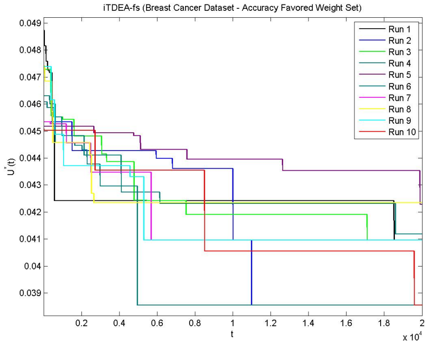
Figure B.28 Breast Cancer – Accuracy Favored – iTDEA-fs
