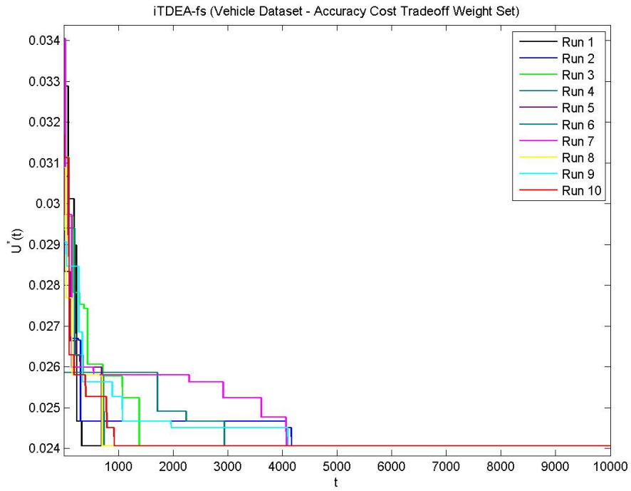
Figure D.4 Accuracy and Cost Tradeoff – iTDEA-fs
