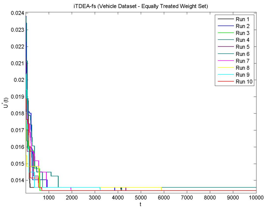
Figure D.7 Equally Treated – iTDEA-fs
