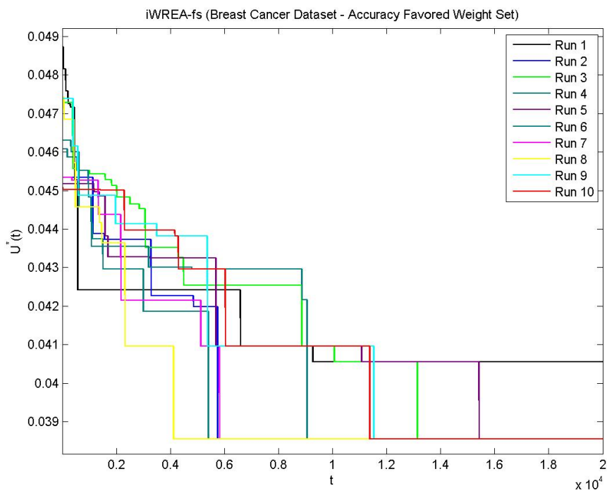
Figure B.29 Breast Cancer – Accuracy Favored – iWREA-fs
