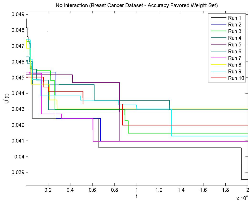
Figure 6.3 Archive progress of No Interaction on Breast Cancer dataset experiments with Accuracy Favored weight set t
