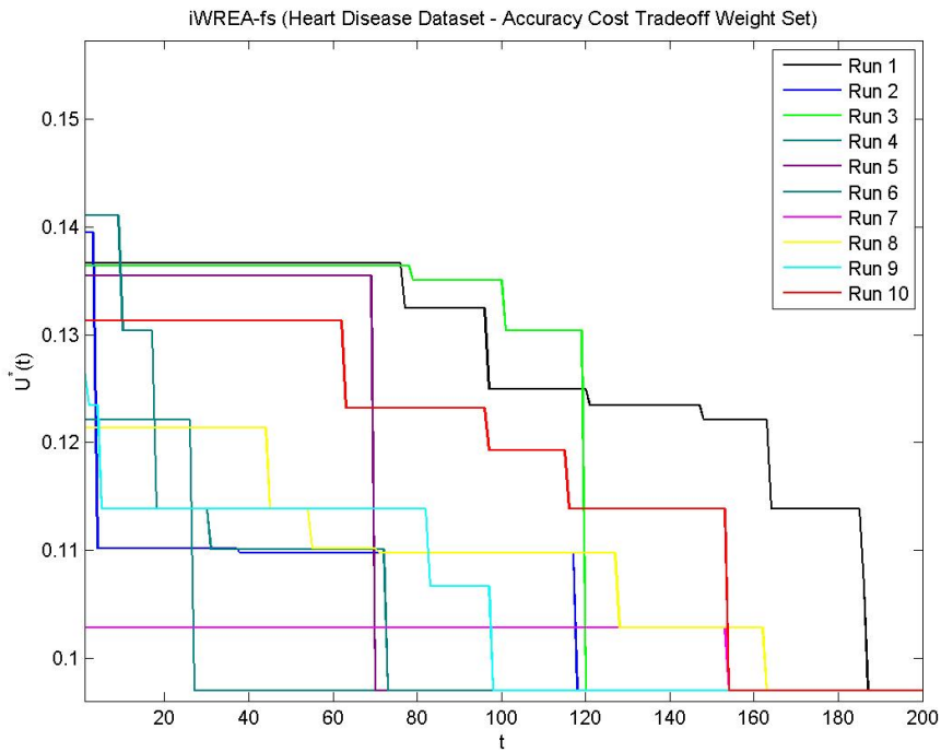
Figure B.5 Heart Disease – Accuracy and Cost Tradeoff – iWREA-fs
