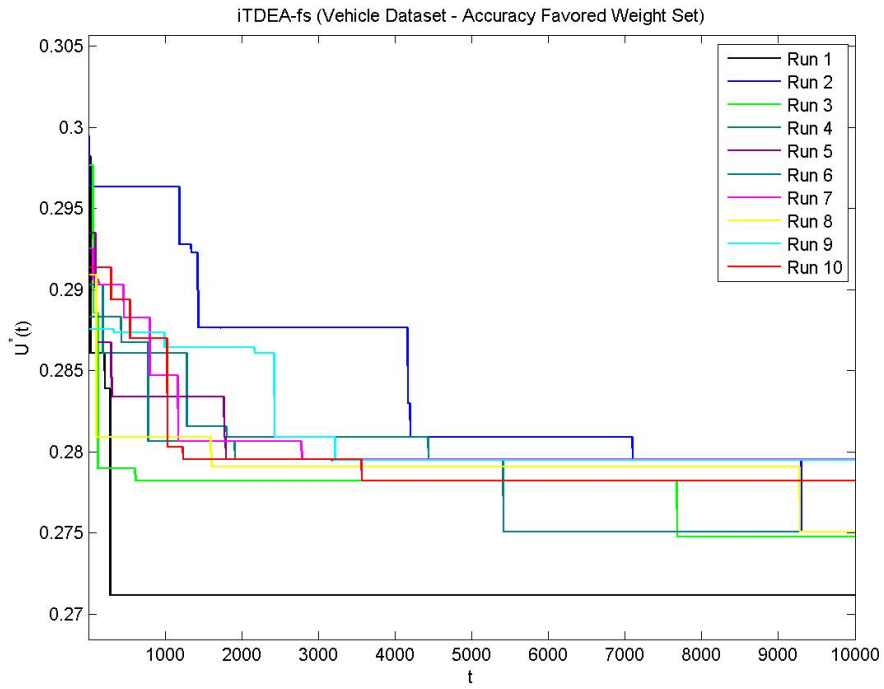
Figure B.10 Vehicle – Accuracy Favored – iTDEA-fs
