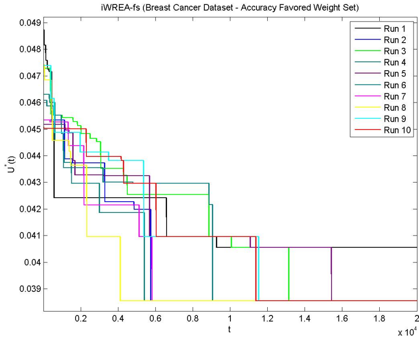
Figure 6.2 Archive progress of iWREA-fs on Breast Cancer dataset experiments with Accuracy Favored weight set
