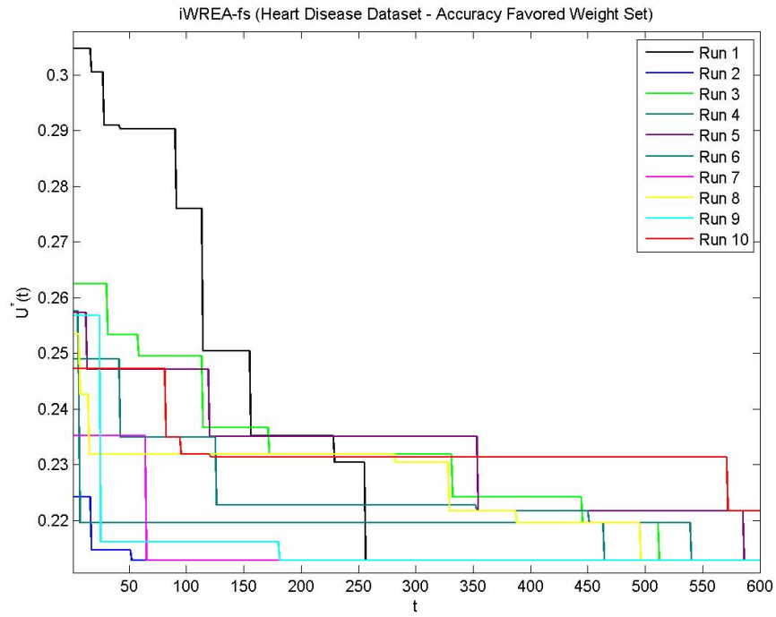
Figure B.2 Heart Disease – Accuracy Favored – iWREA-fs
