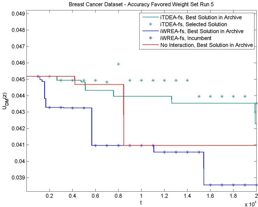
Figure 6.4 5 th replication on Breast Cancer dataset experiments with Accuracy Favored weight set
