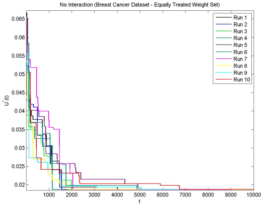
Figure B.36 Breast Cancer – Equally Treated – No Interaction
