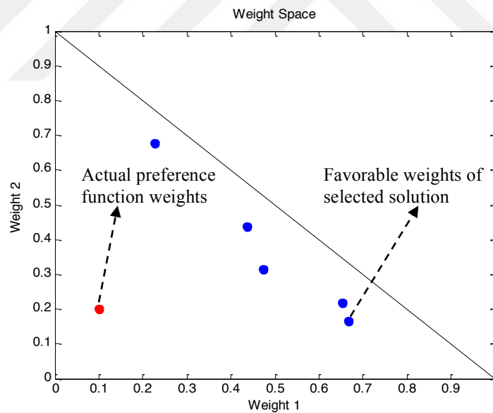
Figure 5.4 Favorable weights and actual weights in the example
