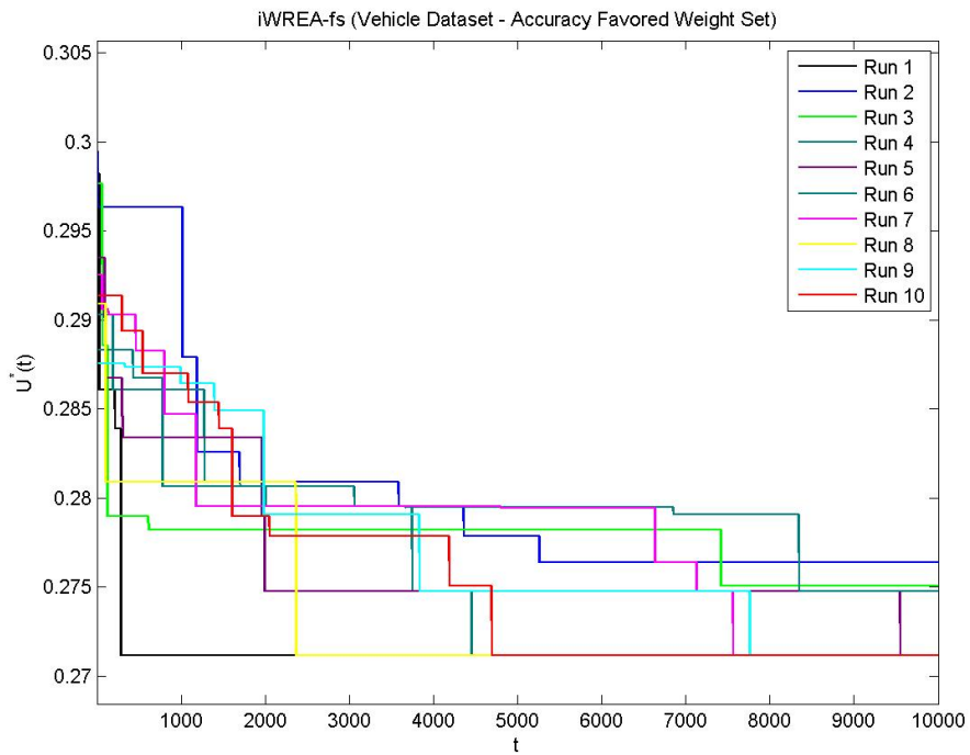
Figure B.11 Vehicle – Accuracy Favored – iWREA-fs
