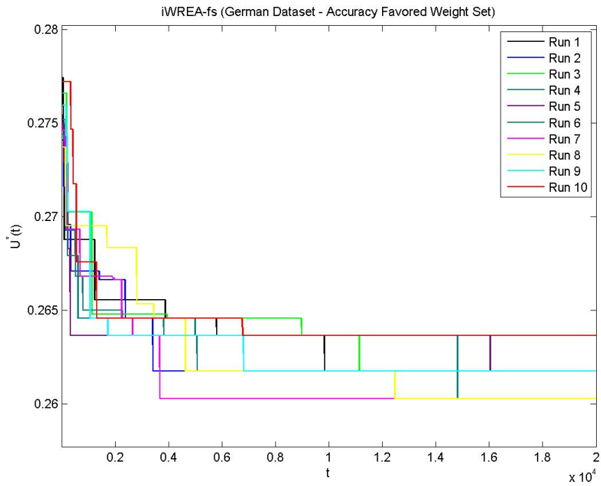
Figure B.20 German – Accuracy Favored – iWREA-fs
