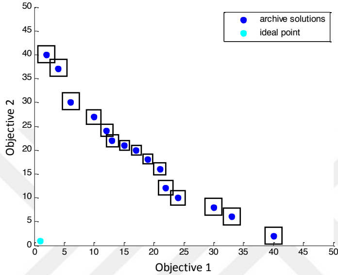
Figure 5.2 Smaller territory levels are assigned to the solutions in the preferred region in iTDEA-fs.
