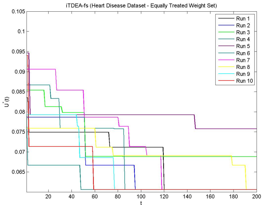
Figure B.7 Heart Disease – Equally Treated – iTDEA-fs
