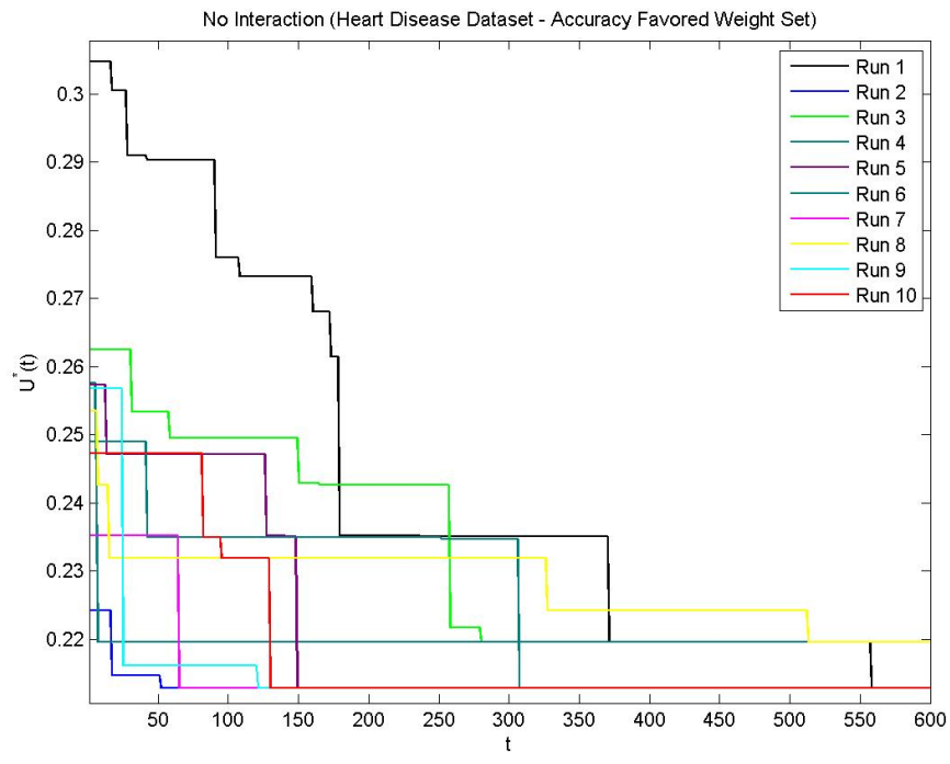
Figure B.3 Heart Disease – Accuracy Favored – No Interaction
