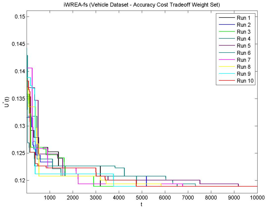
Figure B.14 Vehicle – Accuracy and Cost Tradeoff – iWREA-fs
