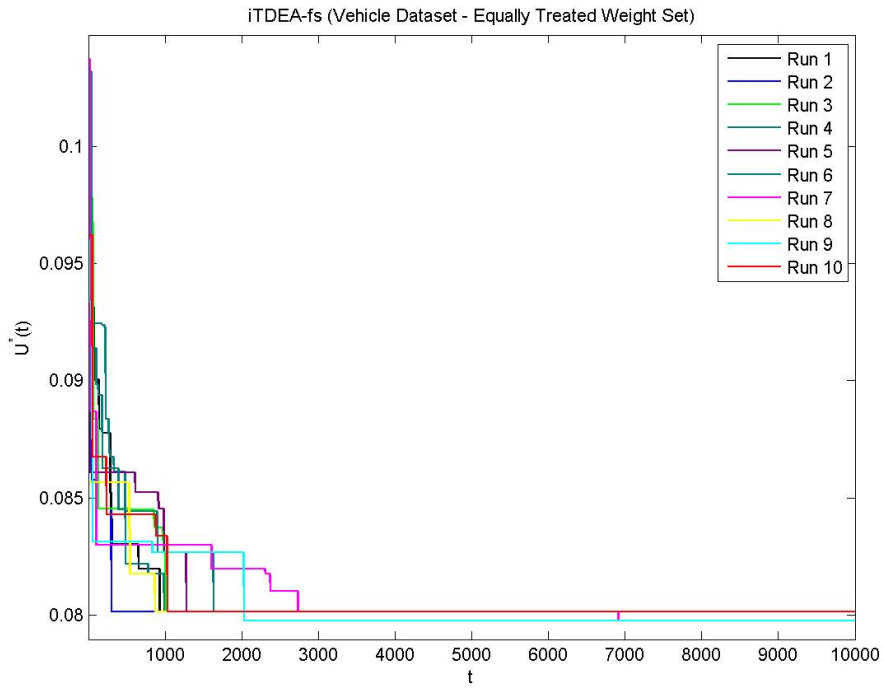
Figure B.16 Vehicle – Equally Treated – iTDEA-fs
