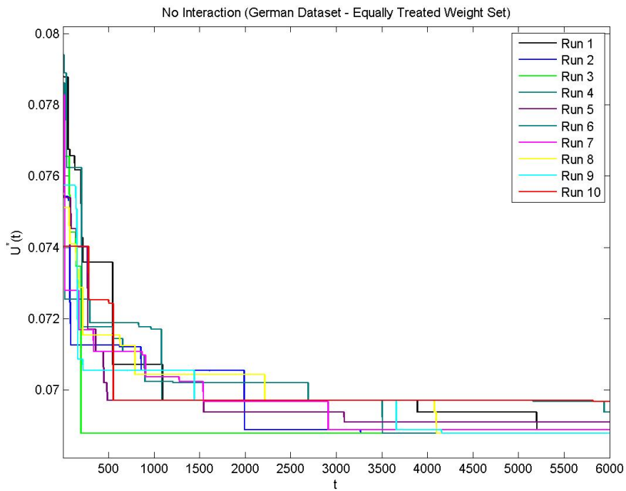
Figure B.27 German – Equally Treated – No Interaction
