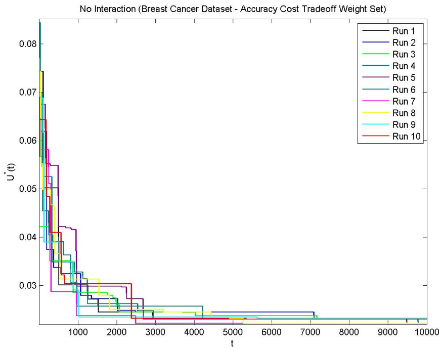
Figure B.33 Breast Cancer – Accuracy Cost Tradeoff – No Interaction
