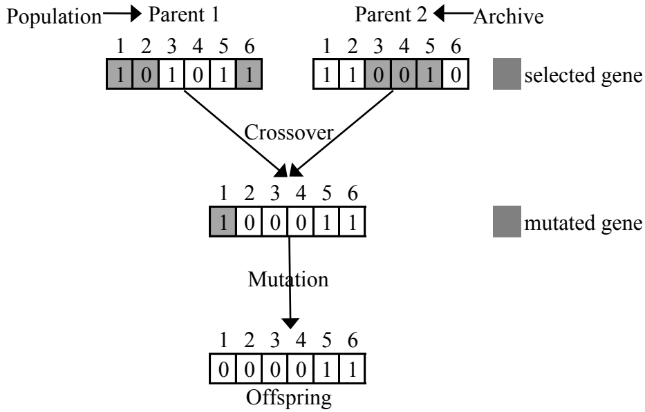
Figure 5.1 An example of crossover and mutation operations
