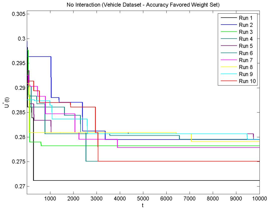
Figure B.12 Vehicle – Accuracy Favored – No Interaction
