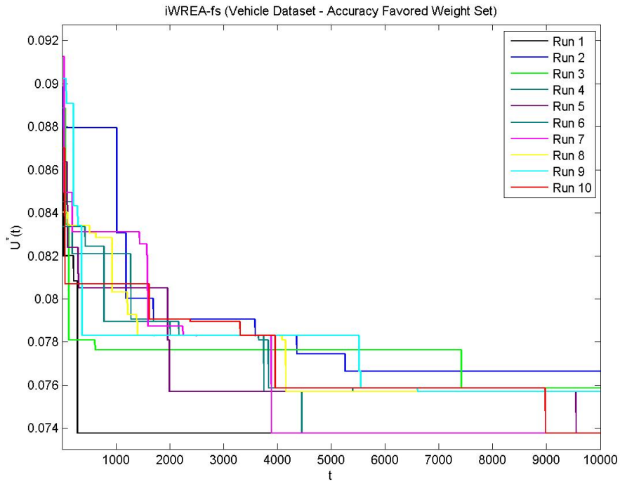
Figure D.2 Accuracy Favored – iWREA-fs
