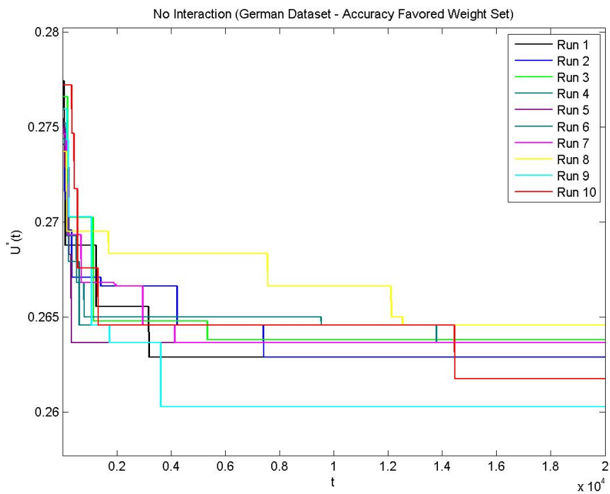
Figure B.21 German – Accuracy Favored – No Interaction
