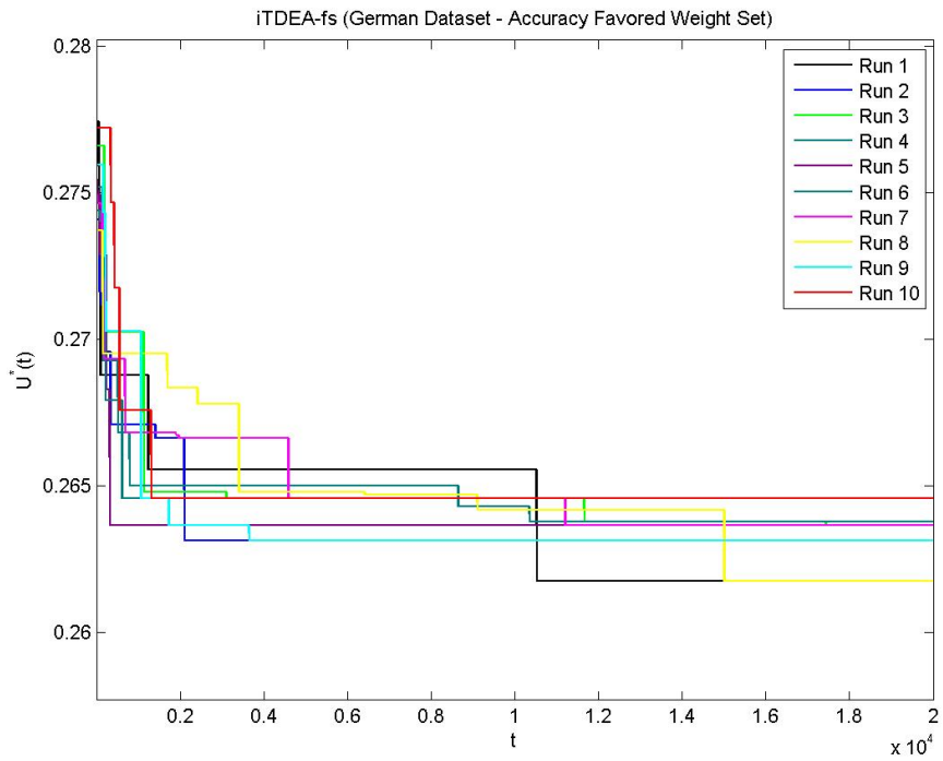
Figure B.19 German – Accuracy Favored – iTDEA-fs
