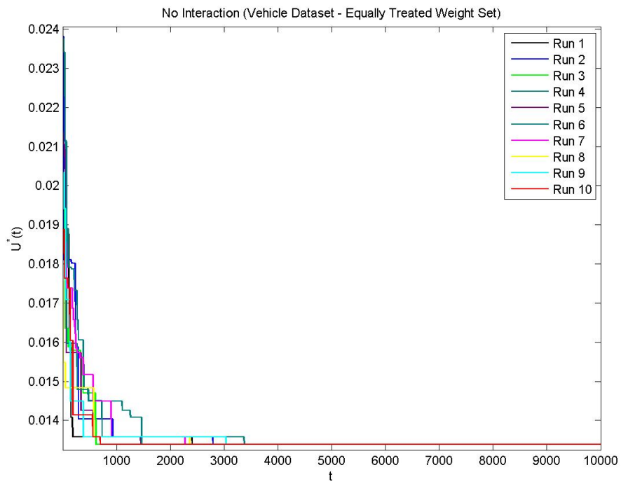
Figure D.9 Equally Treated – No Interaction
