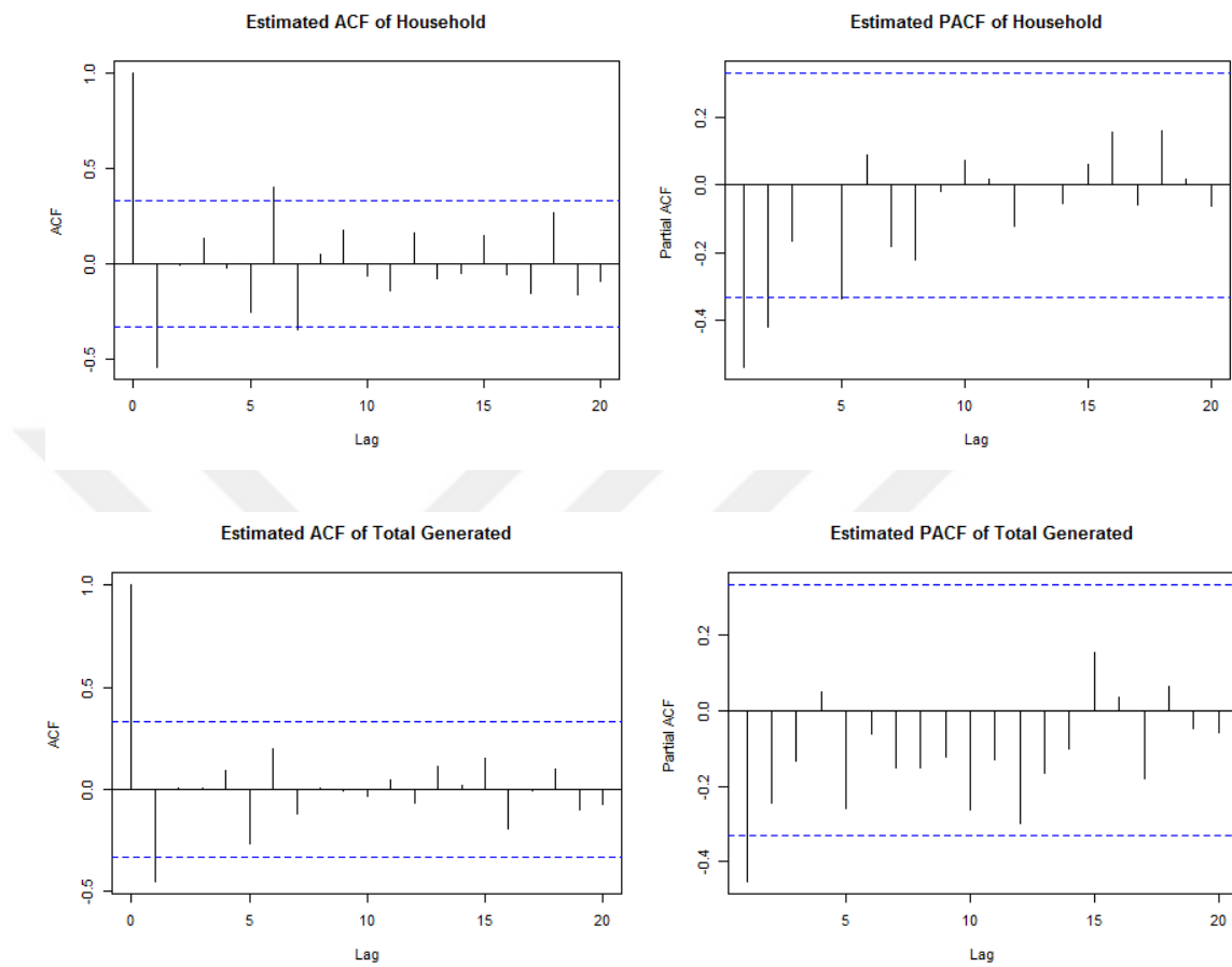
Figure Appendix 46: The estimated ACF and PACF correlogram of solid waste time series.
