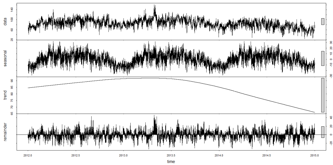
Figure Appendix 5: STL Plot of Teknecik for O 3 (Hourly)
