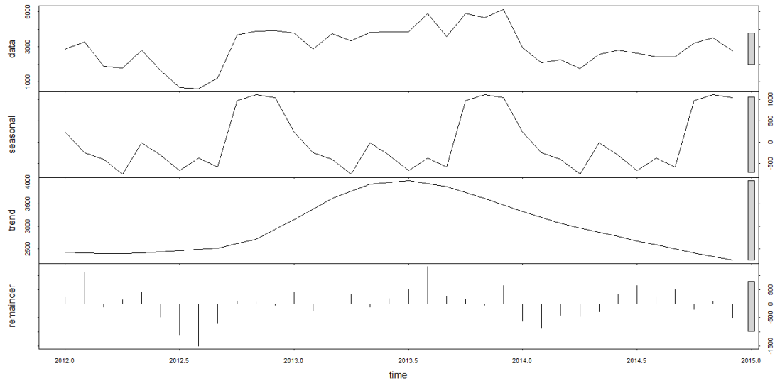
Figure Appendix 22: STL Decomposition of Teknecik NO 2 (Monthly)
