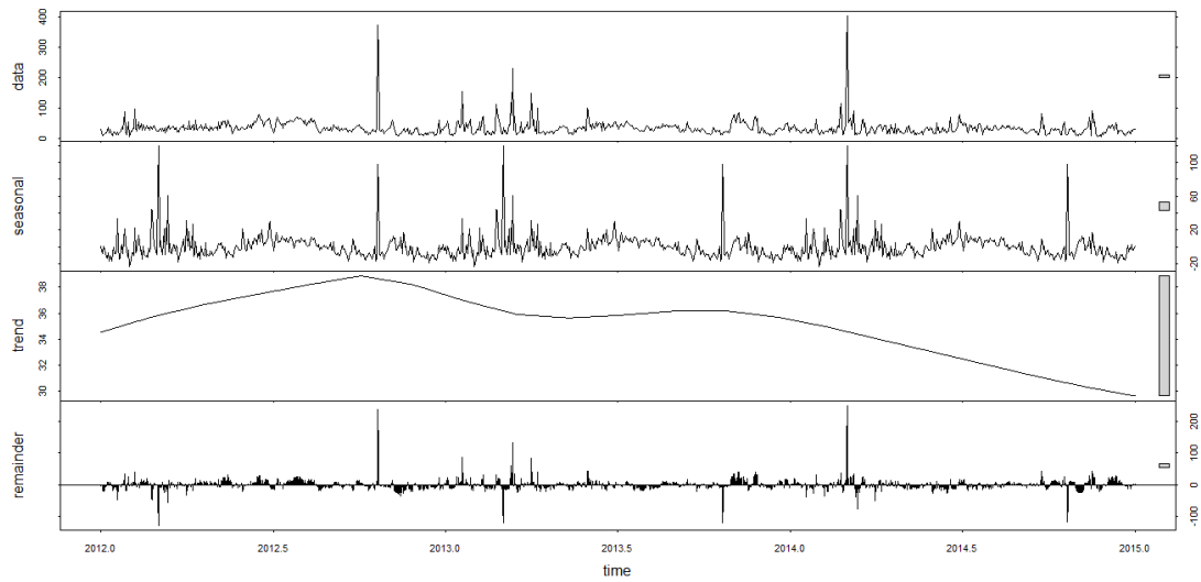
Figure Appendix 9: STL Plot of Kalecik for PM 10 (Daily)
