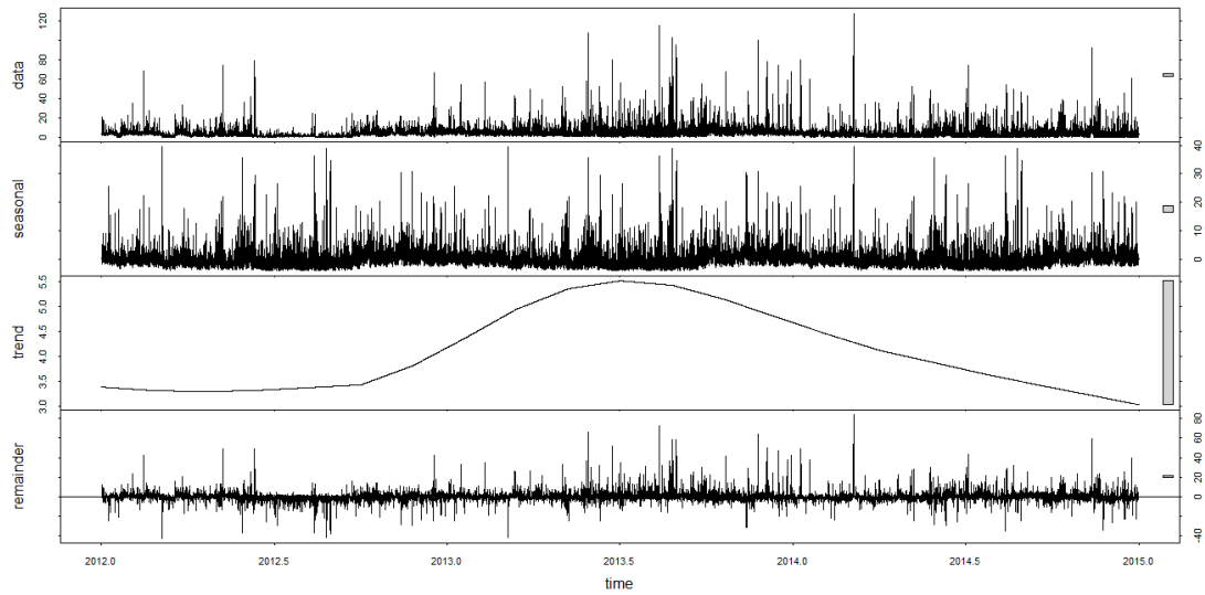
Figure Appendix 4: STL Plot of Teknecik for NO 2 (Hourly)
