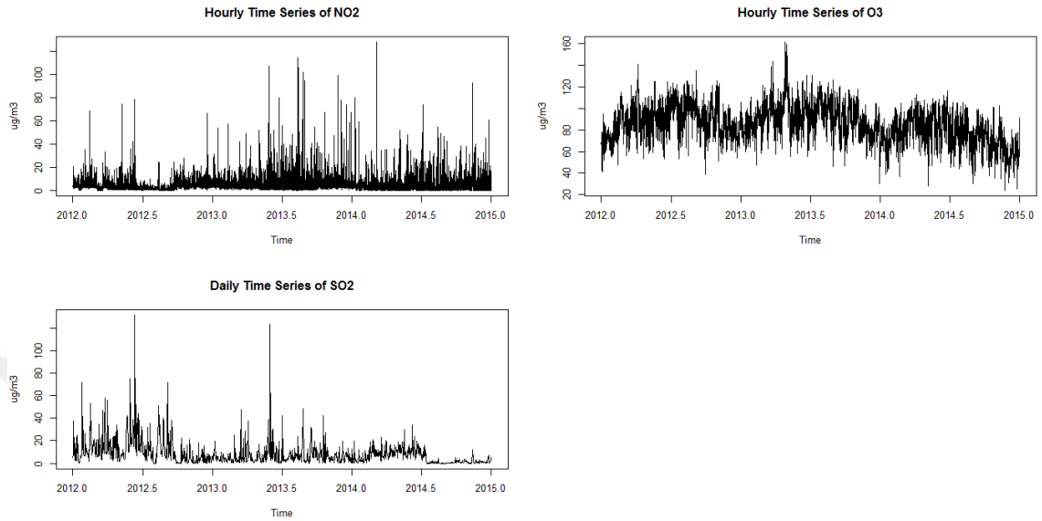
Figure 6: Time Series Plotting of Variables for Teknecik
