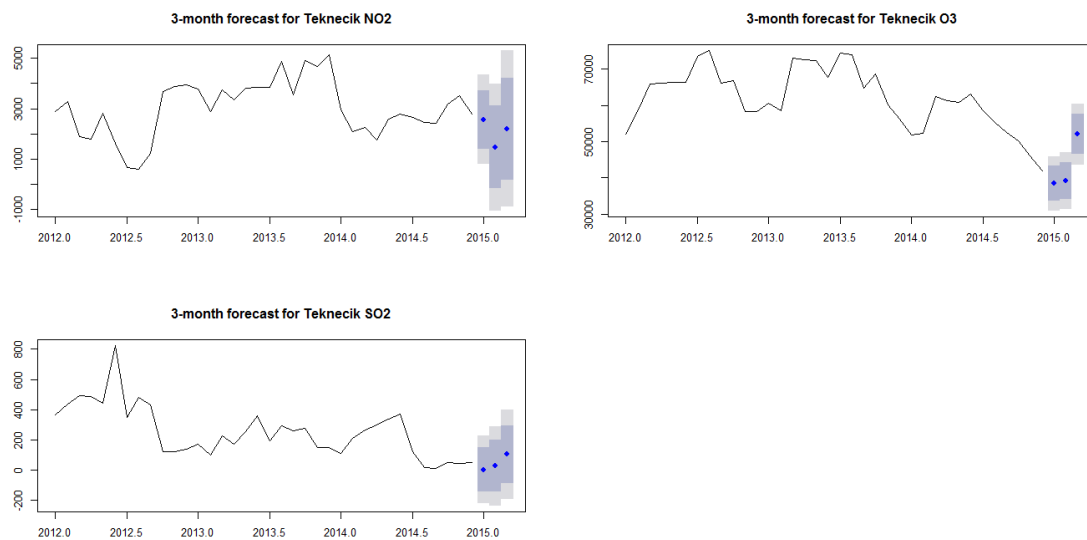
Figure 10: Holt-Winters Prediction of Teknecik
