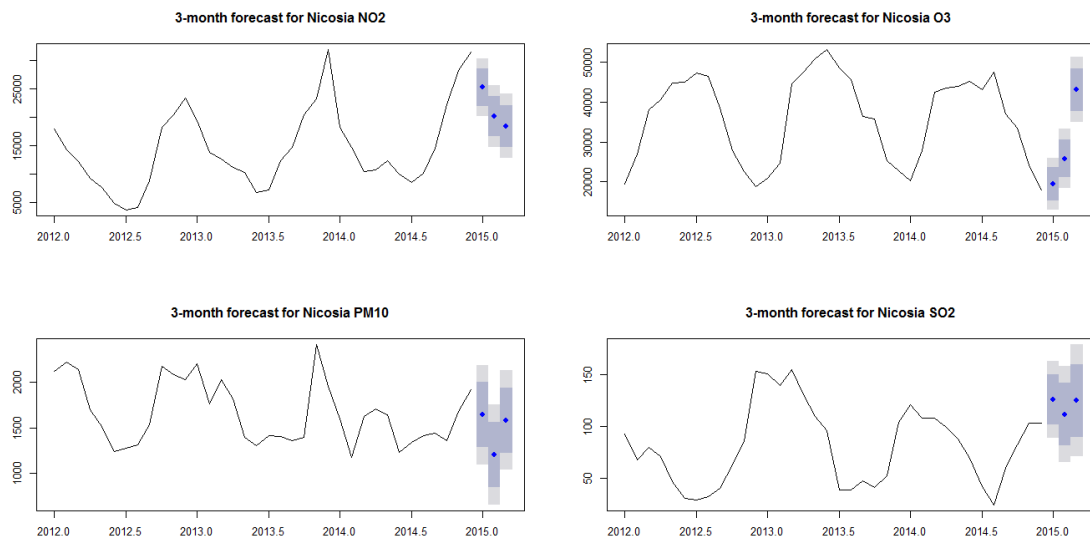
Figure 12: Holt-Winters Prediction of Nicosia
