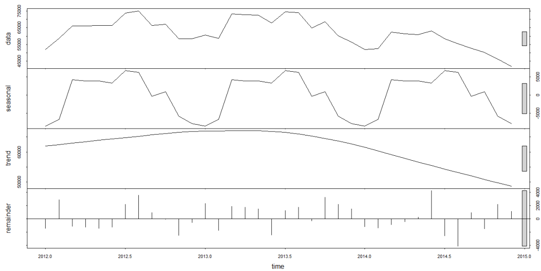
Figure Appendix 23: STL Decomposition of Teknecik O 3 (Monthly)
