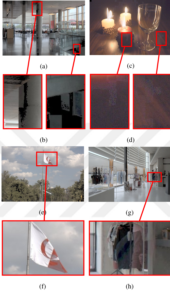
Figure 3.5: Outputs of Silk and Lang [121] for (a) Cafe, (c) Candles, (e) Flag, and (g) Shop2 scenes. In the outputs of the algorithm some of the regions become black, especially if the they have low pixel-intensity values in the input images. In (b), two such regions are shown. In (d), two regions are shown where the boundaries of super-pixels are visually noticeable. (e) and (f) shows the observed color artifacts after the blending operation. (h) shows a region in Shop2 scene where multiple sources are used to fill an underexposed region.
