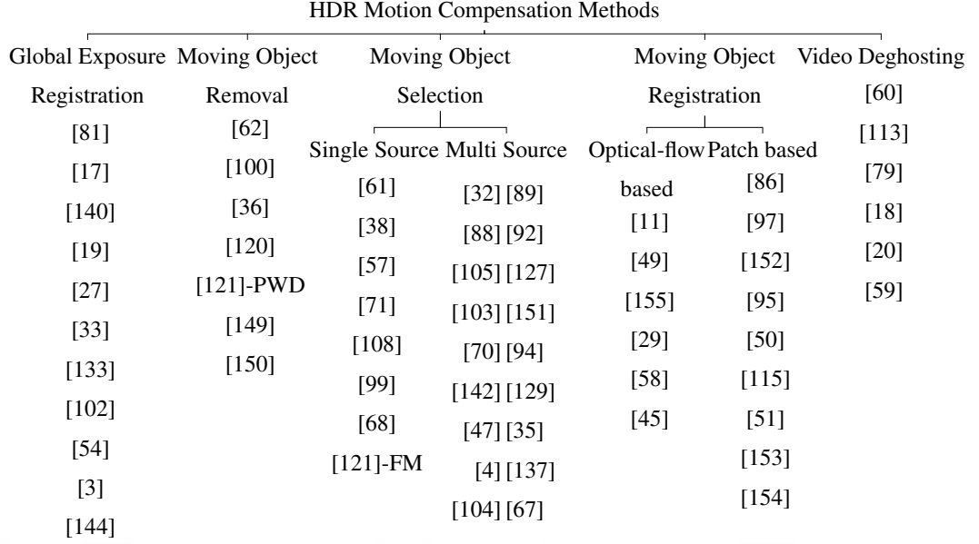
Figure 2.1: Taxonomy of HDR motion compensation methods
