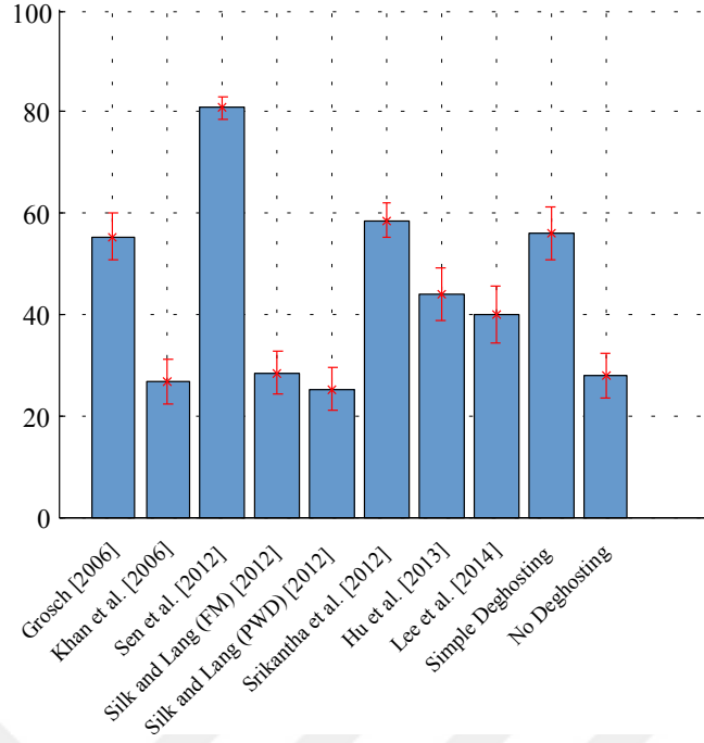
Figure 4.2: Average ratings of the compared algorithms in the subjective experiment. The red lines indicate the standard error.
