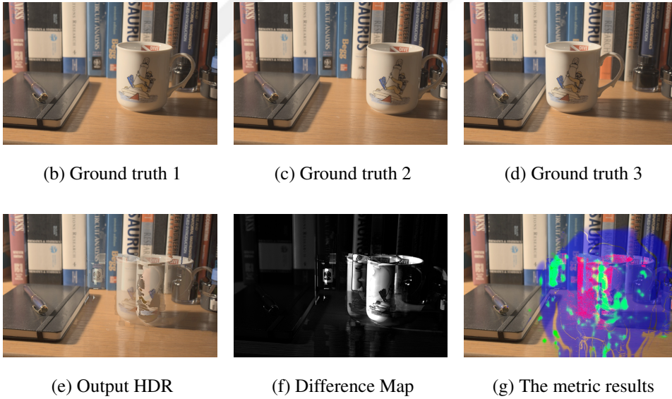
Figure 4.9: Comparison of the objective metric result (g) with the absolute difference (f) between the output of Silk and Lang [121] (e) and ground truth HDR (c). The input exposures with EV -1, 0 and +1 are shown in (a). For each position of the moving object, the ground truth HDR image obtained by using the input exposures is given in (b-d).
