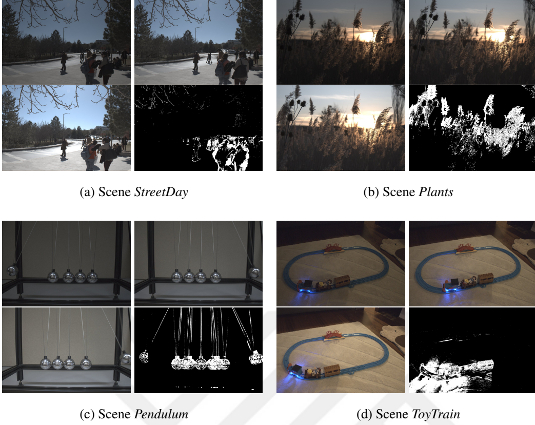
Figure 4.5: Dynamic region bitmaps detected by the heuristic described in the text. Note that the bitmaps successfully capture dynamic objects such as people, foliage, pendulum, and a toy train while generating only a few false positives.
