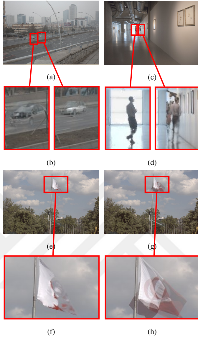
Figure 3.4: Outputs of Khan et al. [62] in (a) FastCars, (c) Gallery2 and (e) Flag scenes. The problematic regions are magnified in (b), (d), (f) and (h). In FastCars scene, the critical assumption of the algorithm does not hold. A vehicle in the scene takes the position of another vehicle from the previous frame; therefore, the majority of the exposures do not capture the background in these regions, which is required for a correct pixel-weighting operation. This situation results in even increased amount of weights where the pixels are affected by the motion in (b). Since there is not a semantic constraint in the pixel down-weighting operations, two copies of the same person appears in the Gallery2 (d) scene. (f) shows the output of Khan et al. in the presence of deformable body motion. The overlapping parts of the moving object are kept whereas other parts are cleared by the algorithm giving rise to a broken appearance. In (h), the same region is shown with no deghosting operation for reference.
