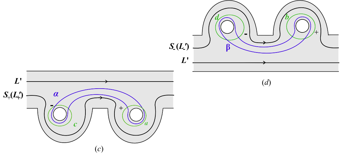
Figure 2.8: (c) Positive destabilization of L' , S_+(L'_+) = L' , (d) Negative destabilization of L' , S_-(L'_-) = L' .
