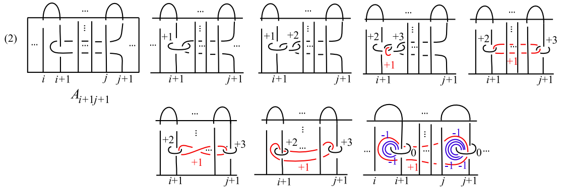
Figure 3.12: Case (2) A_{i+1j+1} .
