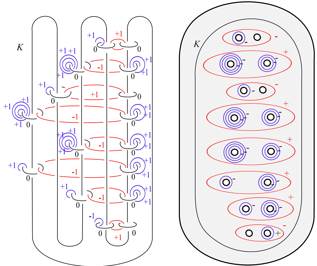
Figure 3.8: Page of a planar open book decomposition containing the figure eight knot, pages are disk with 16 punctures.
