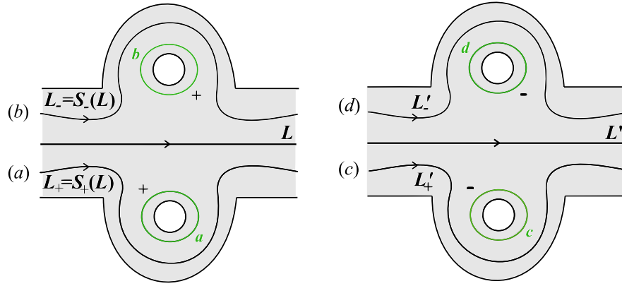
Figure 2.6: (a) Positive stabilization S_+(L) of L , (b) Negative stabilization S_-(L) of L , (c) Positive destabilization of L' , S_+(L'_+) = L' , (d) Negative destabilization of L' , S_-(L'_-) = L' .
