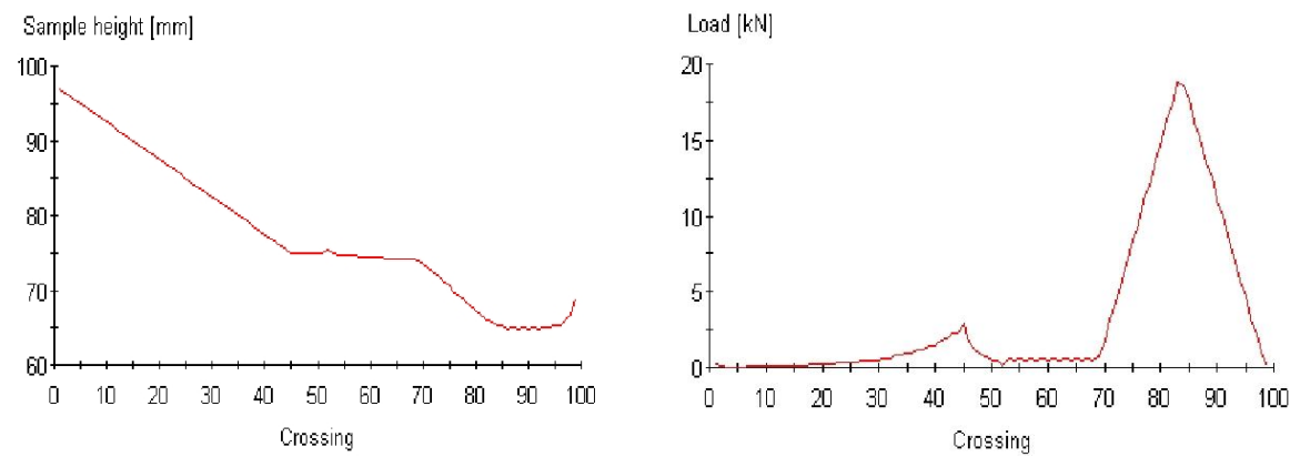
GGAC- C- Binder Course Compaction Result
