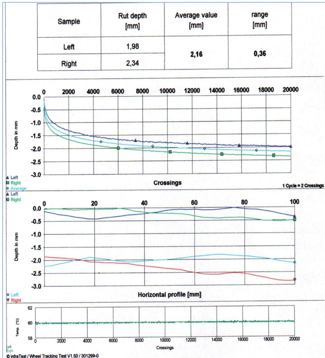
Figure 6.19. GGAC- 2 Specimen Rutting Test Result Plot
