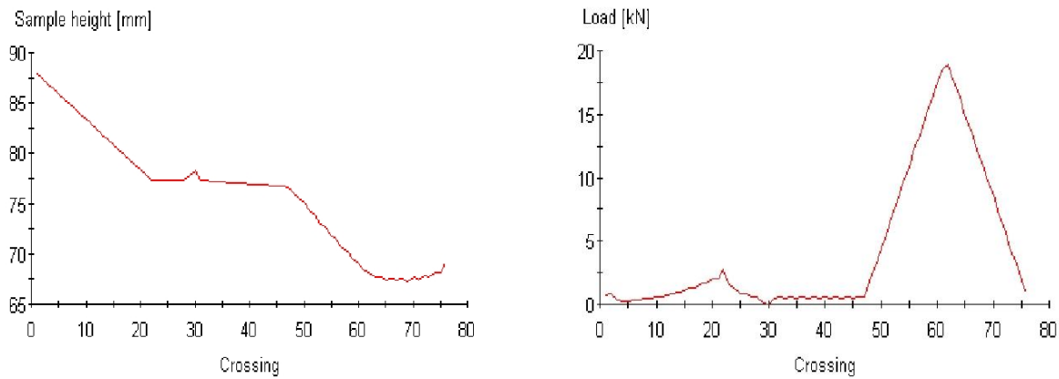
DGAC- 1- Binder Course Compaction Result
