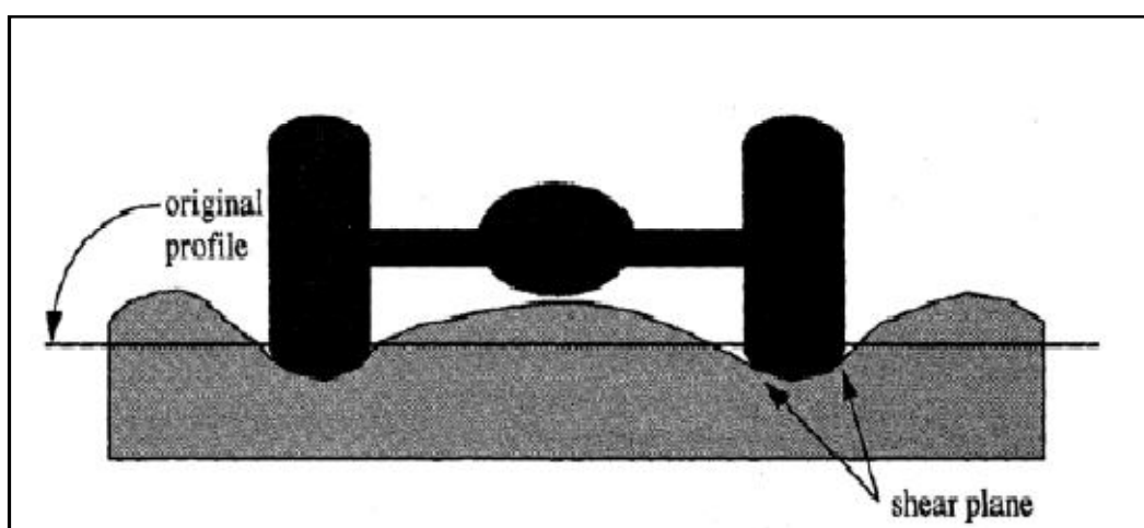
Figure 3.5. Mix rutting. (Huber 1999)
