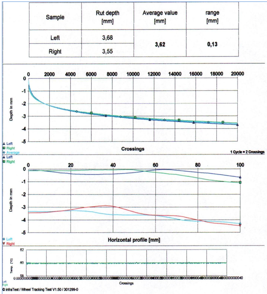
Figure 6.16. DGAC- 4 Specimen Rutting Test Result Plot
