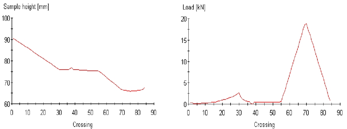
DGAC- 2- Binder Course Compaction Result
