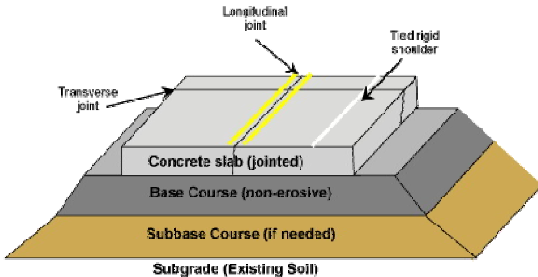
Figure 2.3. Typical section for a rigid pavement.
