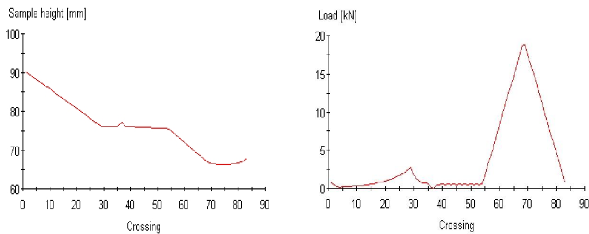
DGAC- 4- Binder Course Compaction Result
