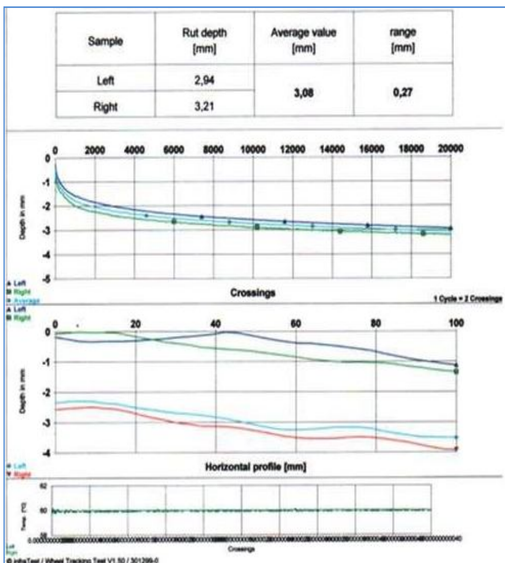
Figure 6.12. DGAC- C Specimen Rutting Test Result Plot
