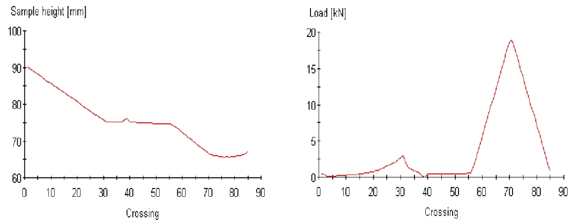
GGAC- C- Binder Course Compaction Result
