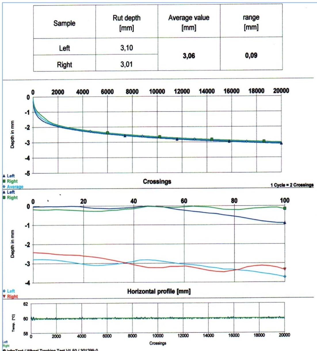
Figure 6.15. DGAC- 3 specimen rutting test result plot
