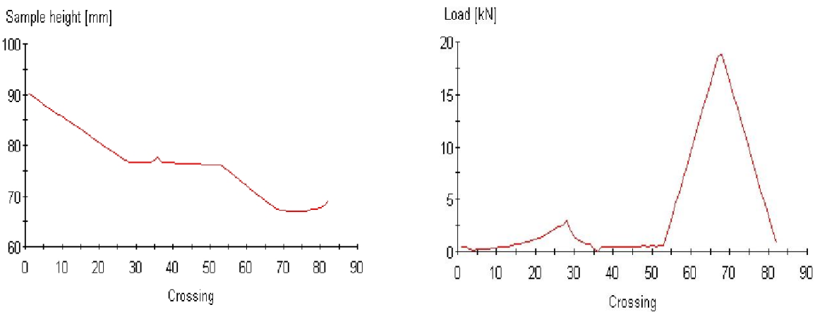
DGAC- 2- Binder Course Compaction Result
