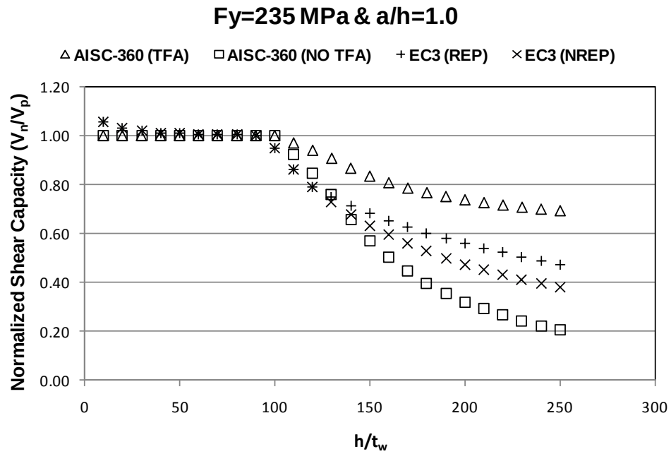
Fig. 6.5: Normalized Shear Capacity for a/h=1.0 and F_y=235 MPa
