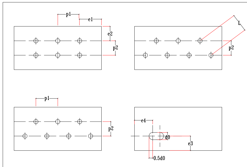
Fig. 7.3: Bolt Orientations
