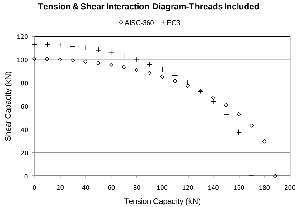
Fig. 7.5: Shear & Tension Interaction Diagram-Threads Included
