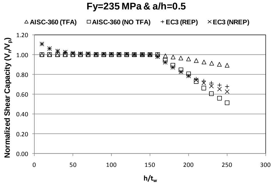
Fig. 6.4: Normalized Shear Capacity for a/h=0.5 and F_y=235 MPa
