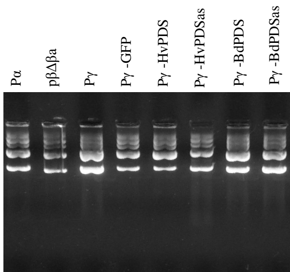
Figure 3.8. Isolated plasmids were separated on 1 % agarose gel. The bands at the bottom are the ones that we cut from the gel.
