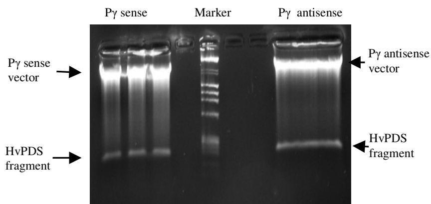
Figure 3.7. Excision of HvPDS from P \gamma sense and P \gamma antisense vectors. Both vectors were cut with Not I and Pac I restriction enzymes. Samples were separated on 1 % agarose gel by electrophoresis.
