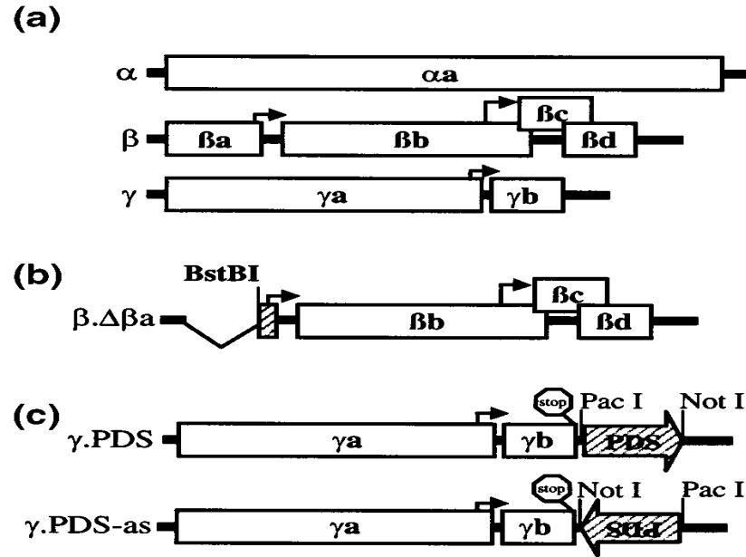
Figure 2.2. BSMV RNA derived vectors. (a) p\alpha , p\beta and p\gamma genomes of BSMV. (b) p\beta\Delta\beta a representing the deleted version of p\beta genome. (c) p\gamma.PDS s and p\gamma.PDSas orientations. The picture was taken from Holzberg et al. 2002.
