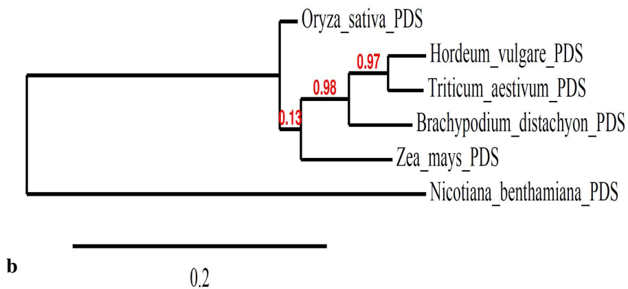
Figure 3.5(b). Phylogenetic tree of Brachypodium distachyon , Hordeum vulgare , Triticum aestivum , Nicotiana benthamiana , Oryza sativa , Zea mays . Phylogeny fr (Dereeper et al. 2007) was used to draw Phylogenetic tree.
