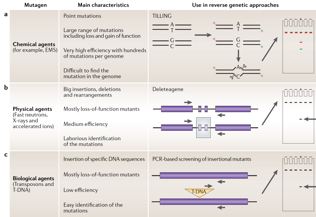
Figure 1.2. Reverse genetic approaches (a) Gene silencing by using chemical agents such as ethyl methanesulphonate (EMS). In this method point mutations are created among the genome and these mutations can be identified using targeting induced local lesions in genomes (TILLING) method. (b) Interfering with gene action using physical agents such as X-rays or accelerated ions. In this method deletion of part of gene of interest is verified by PCR using primers that flank the gene of interest after causing damage by physical agents (c) Disruption of gene by biological agents such as transferred DNA (T-DNA) or transposons. This method is based on insertional inactivation of gene of interest. (Alonso et al. 2006)
