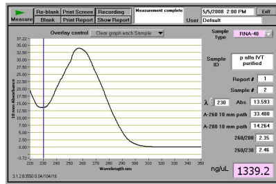
Pa transcript
