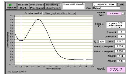
Pγ-GFP transcript
