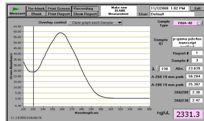
Pγ-HvPDSas transcript
