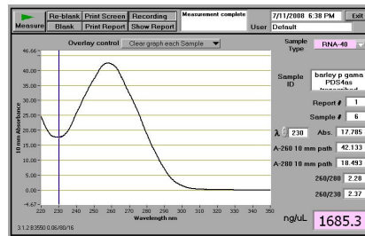
Pγ-BdPDSas transcript
