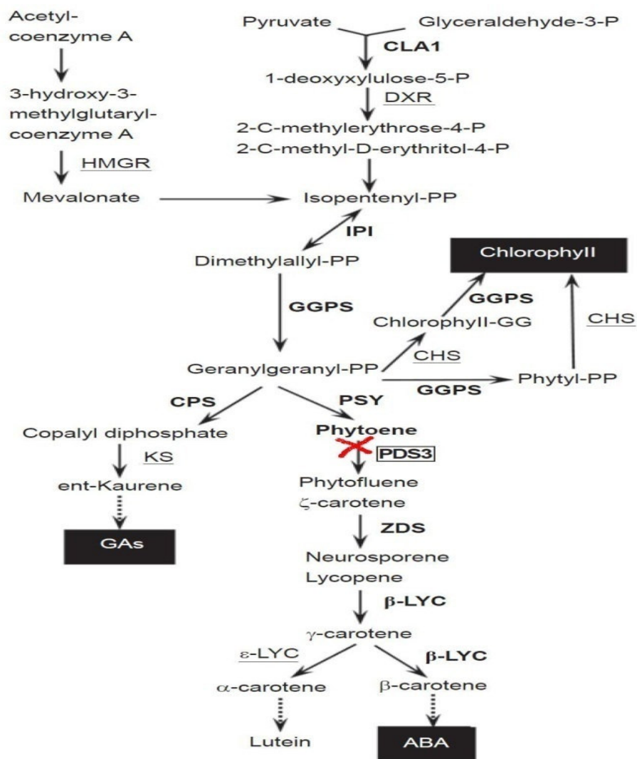
Figure 1.6. Carotenoid, chlorophyll and GA biosynthesis pathways. Inhibition of PDS enzyme caused phytoene accumulation and this interferes with production of \alpha and \beta carotene (Qin et al. 2007).
