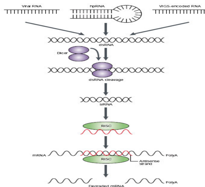
Figure 1.4 The RNA-mediated gene silencing model. Double stranded RNA (ds RNA) is generated from replicating viral RNA. In our case VIGS vectors (viral-vector-derived BSMV vectors) are used to produce viral ds RNA by in vitro transcription (Waterhouse and Helliwell, 2003).
