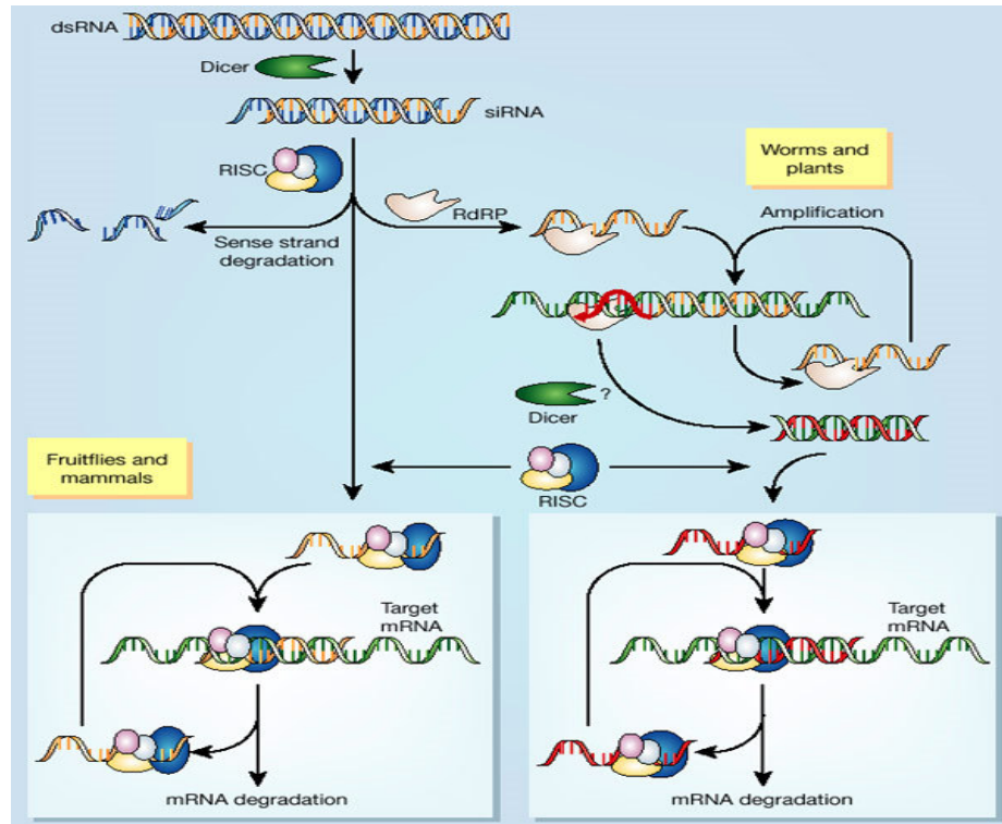
Figure 1.3. Short interfering RNAs— Post-Transcriptional Gene Silencing (PTGS). dsRNAs introduced into or expressed in cells are recognized by Dicer which converts long dsRNA precursor into small RNA duplexes (guide siRNA/ passenger siRNA). Guide siRNA is selected and loaded onto Argonaut protein. This activates RISC and target mRNA is either sliced (commonly in plants) or translationally repressed (commonly in mammals and fruit flies). In worms and plants there is also a distinct pathway to create secondary siRNAs by the action of RDRP (RNA-dependent RNA polymerase) which uses siRNA as primer and target sequence as template to generate and amplify siRNAs. Novina et al. (2004)
