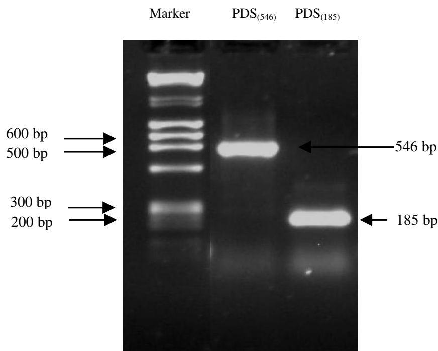
Figure 3.3. B. distachyon PDS fragments on the 1 % agarose gel. Marker used is 100 bp marker.
