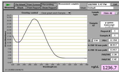
Pγ transcript
