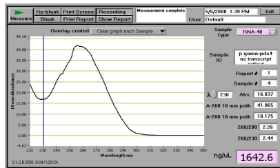
Pγ-HvPDS transcript
