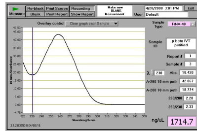
PβΔβa transcript
