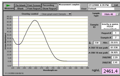
Pγ-BdPDS transcript
