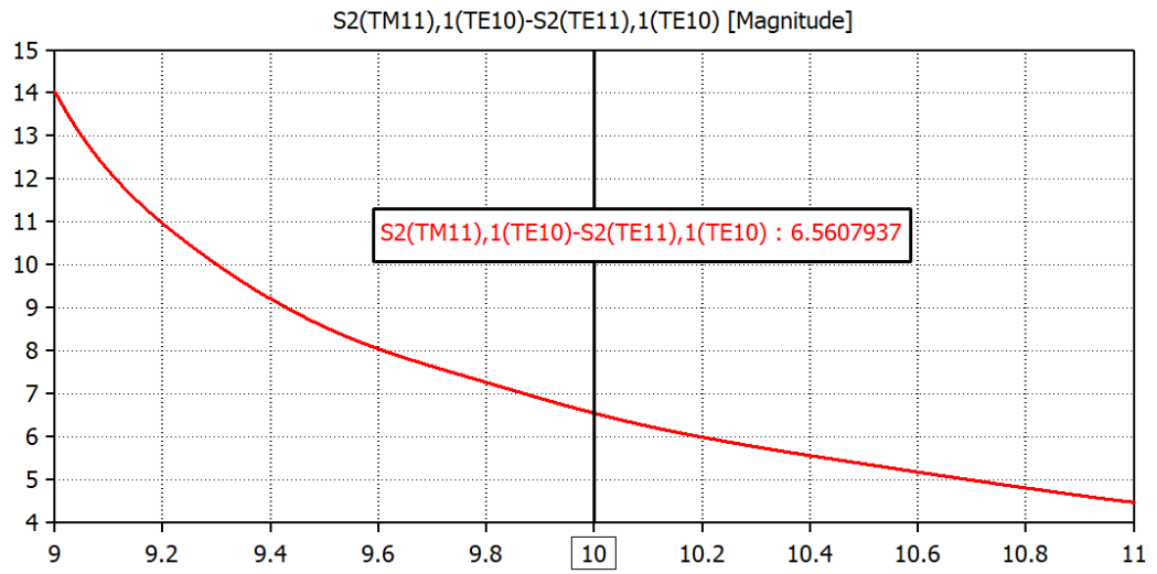
Figure 3.40: S_{2,1} difference of \text{TM}_{11} and \text{TE}_{11} modes
