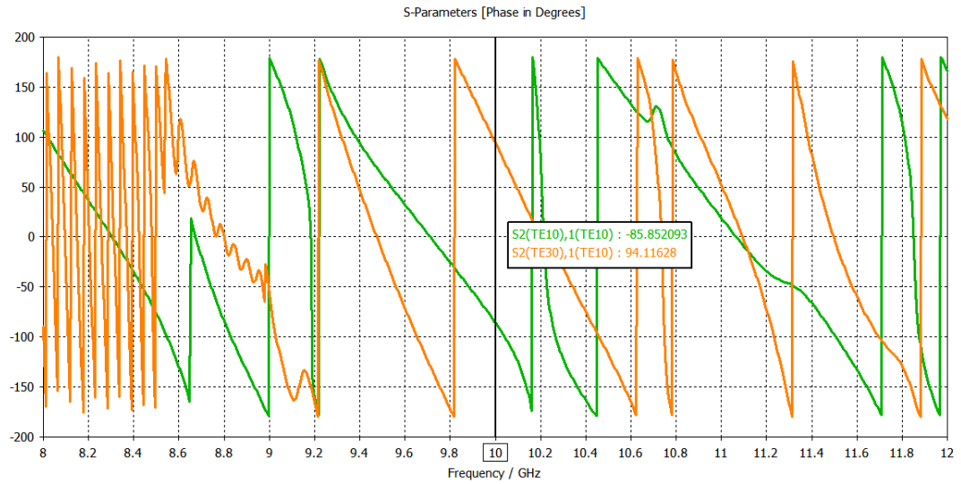
Figure 3.15: Phases of TE_{10} and TE_{30} modes at the output terminal
