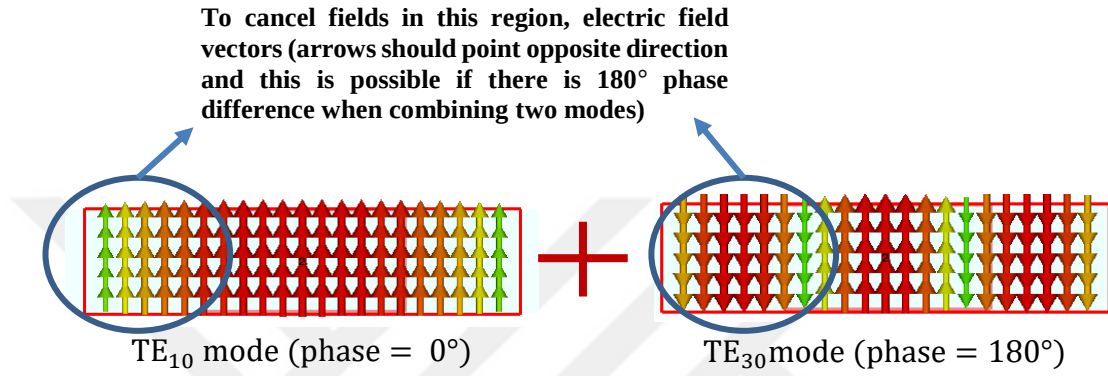
Figure 3.12: The reason for 180° phase difference when combining two modes
