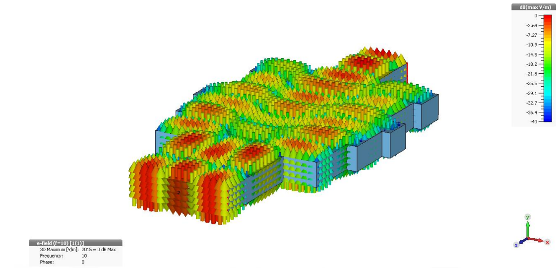
Figure 3.6: Electric field vectors inside designed 5 stepped TE_{10} to TE_{30} converter at 10 GHz
