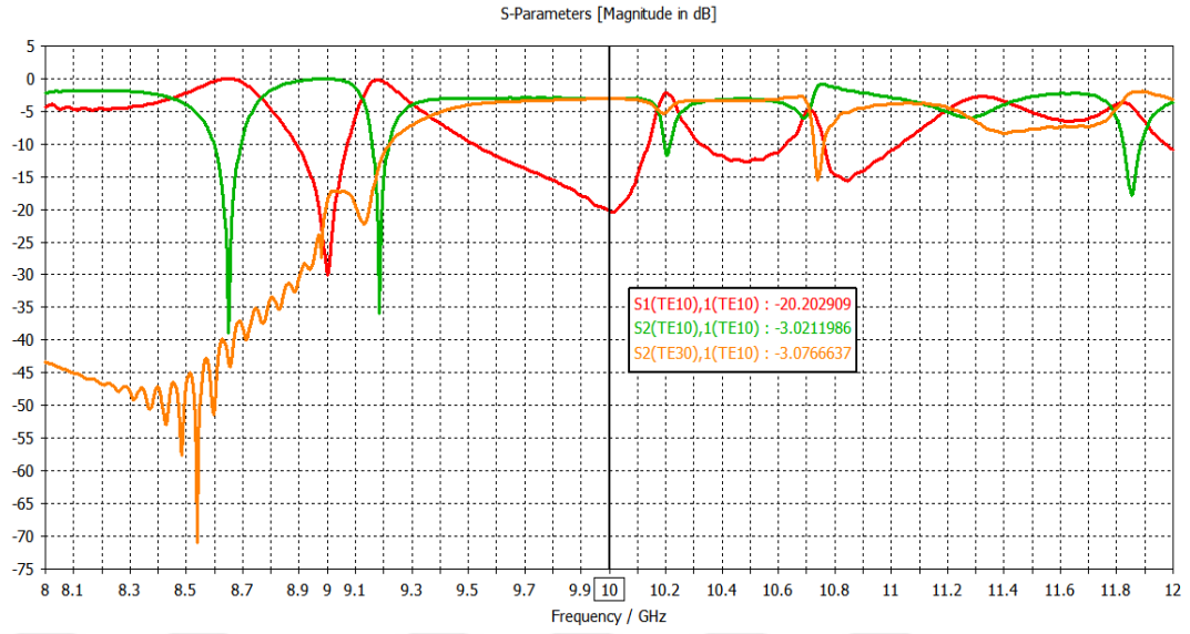
Figure 3.14: S parameter result of designed 5 stepped TE_{10} to TE_{10}+TE_{30} converter
