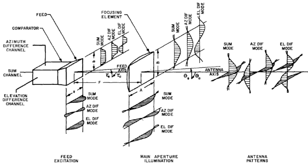
Figure 1.15: The summary of beam optimization problem in conventional monopulse feeds [25]
