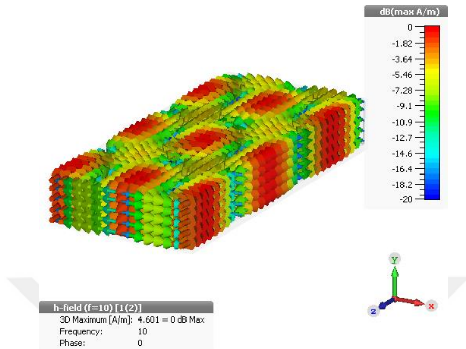
Figure 2.9: Magnetic field vectors of TE_{20} mode inside rectangular waveguide
