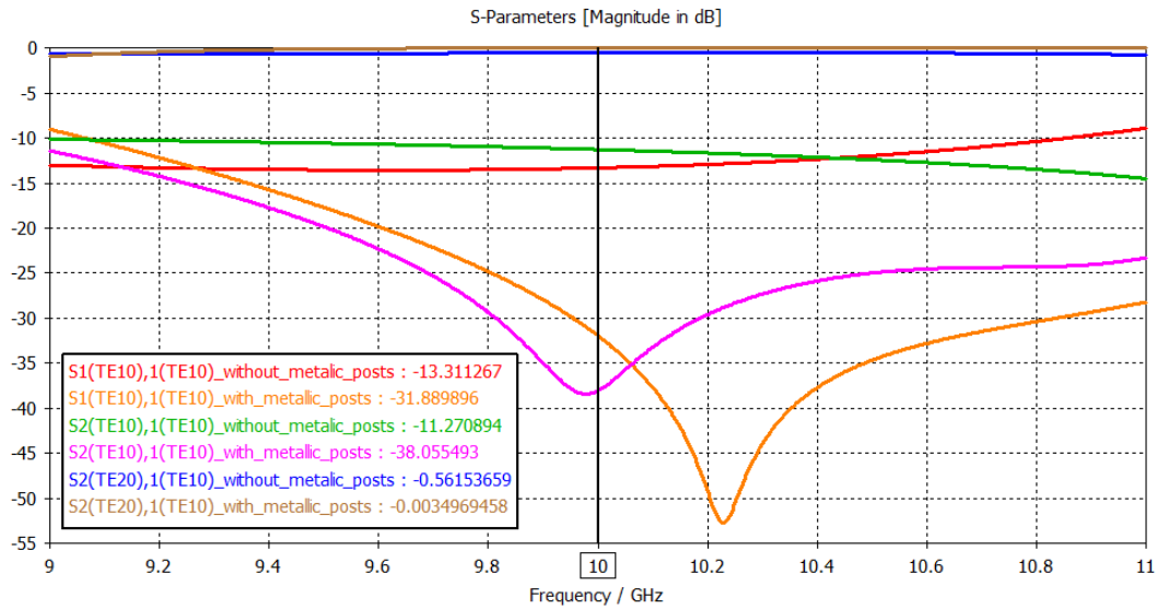
Figure 3.44: S parameters of H-plane corner \text{TE}_{10} - \text{TE}_{20} mode converter with and without metallic posts
