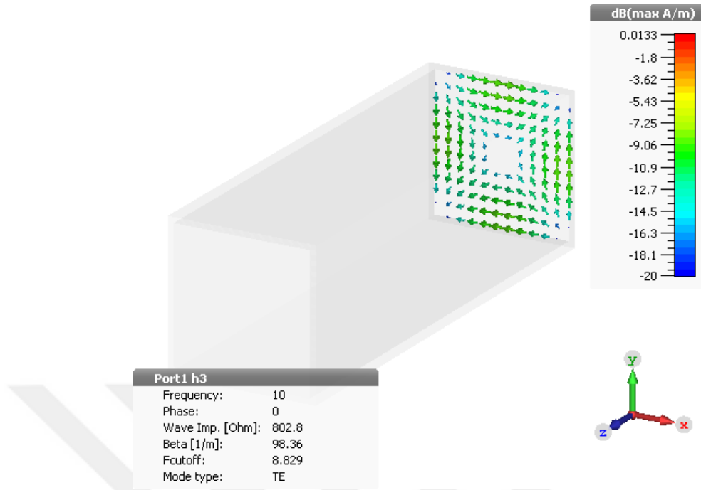
Figure 2.21: Cross sectional magnetic field vectors of TE 11 mode at the input
