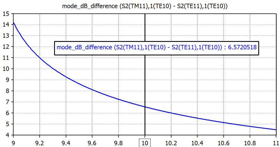
Figure 3.28: S_{2,1} difference of \text{TM}_{11} and \text{TE}_{11} modes
