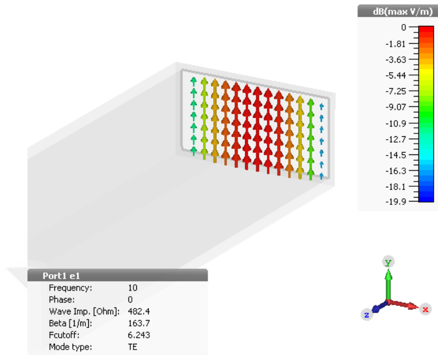
Figure 2.5: Magnetic field vectors of TE_{10} mode inside rectangular waveguide
