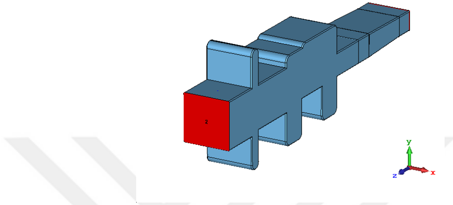
Figure 4.3: Addition of transition region
