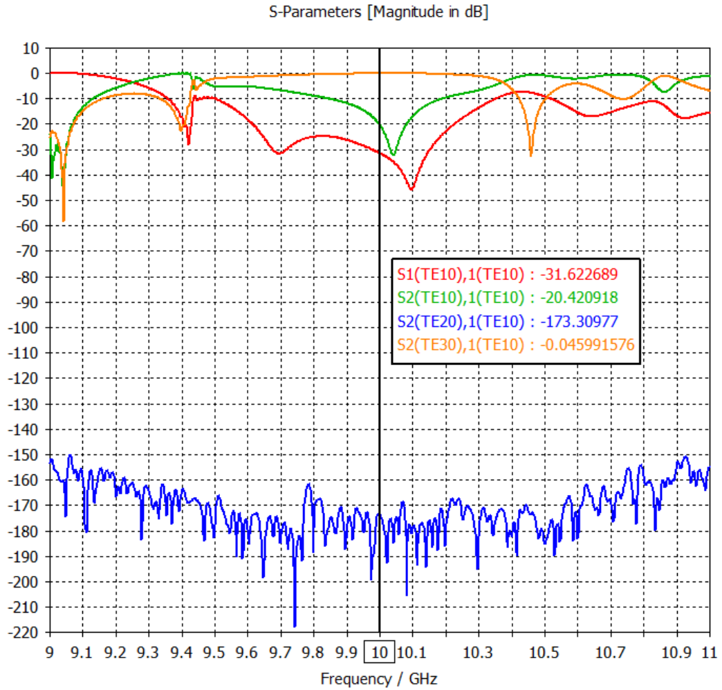
Figure 3.10: S parameter result of designed 20 stepped TE_{10} to TE_{30} converter
