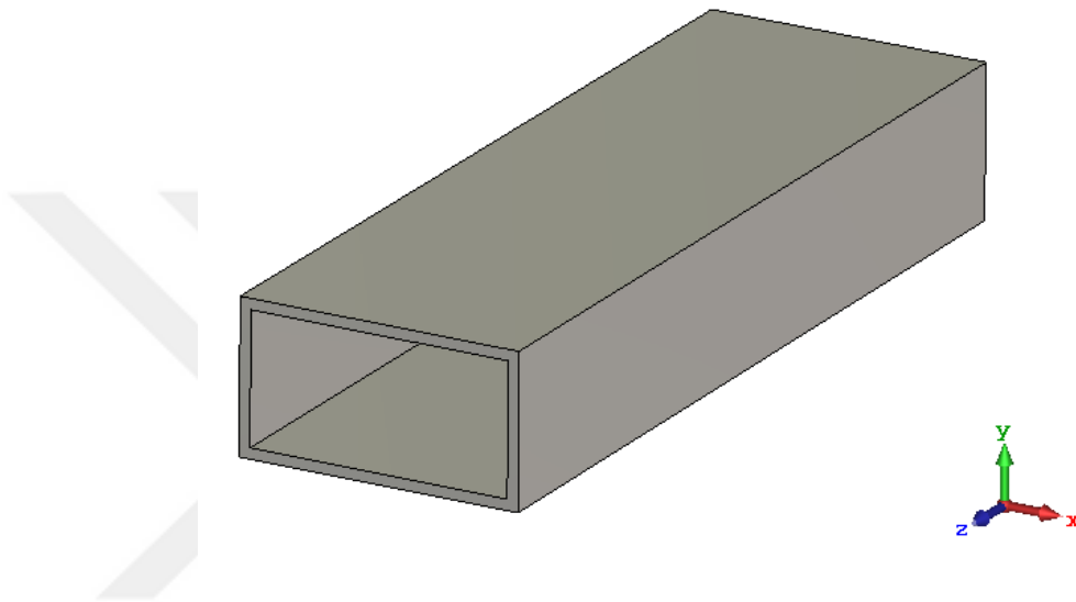
Figure 2.2: Rectangular waveguide with dimensions a = 24 mm, b = 12 mm & l = 80 mm
