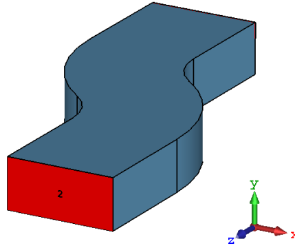
Figure 3.33: Designed TE_{10} - TE_{20} double H-plane bend mode converter
