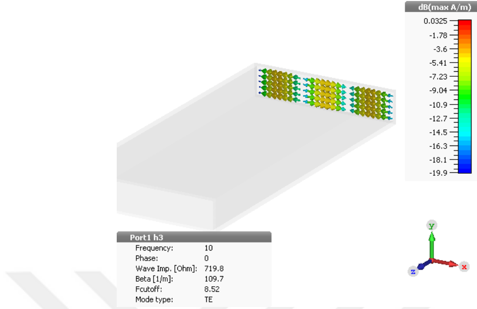
Figure 2.16: Cross sectional magnetic field vectors of TE 30 mode at the input
