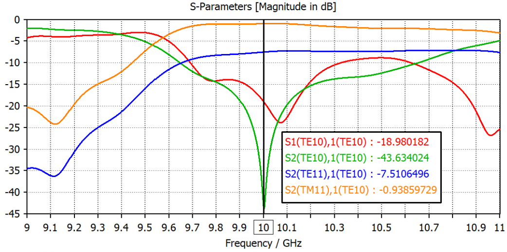
Figure 3.27: S parameter result of designed 5 stepped \text{TE}_{10} to \text{TE}_{11}+\text{TM}_{11} converter
