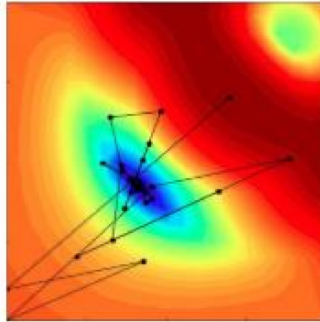
Figure A.5: Visualization of Nelder-Mead Simplex algorithm process
