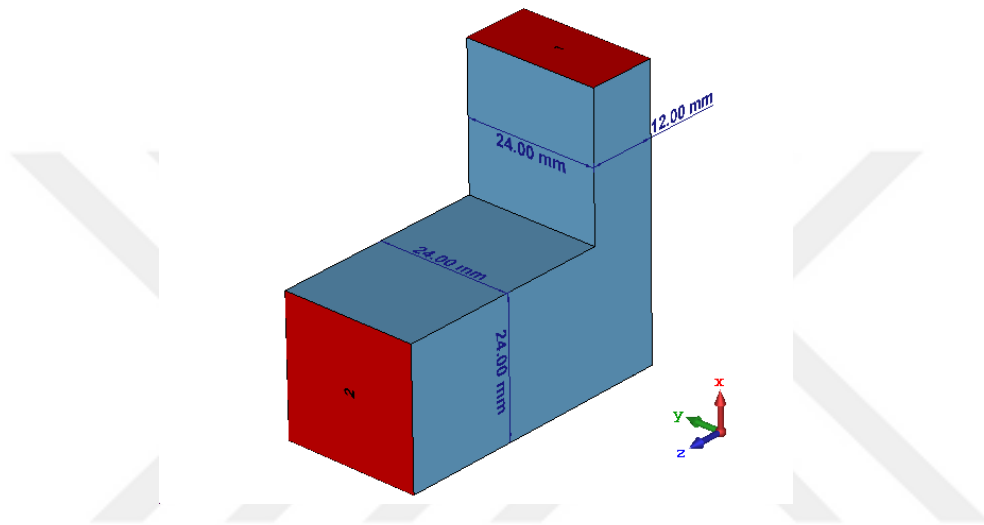
Figure 3.49: Initial E-Plane corner structure with its waveguide dimensions
