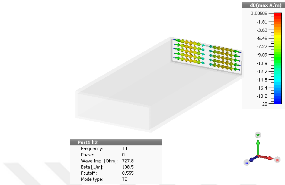
Figure 2.11: Cross sectional magnetic field vectors of TE 20 mode at the input
