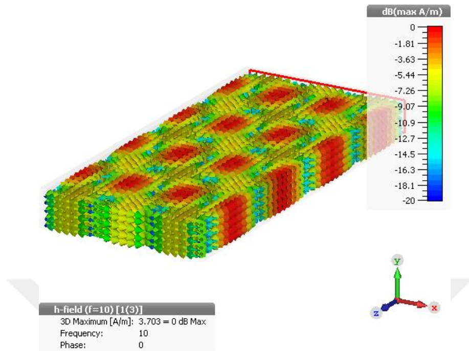
Figure 2.14: Magnetic field vectors of TE_{20} mode inside rectangular waveguide
