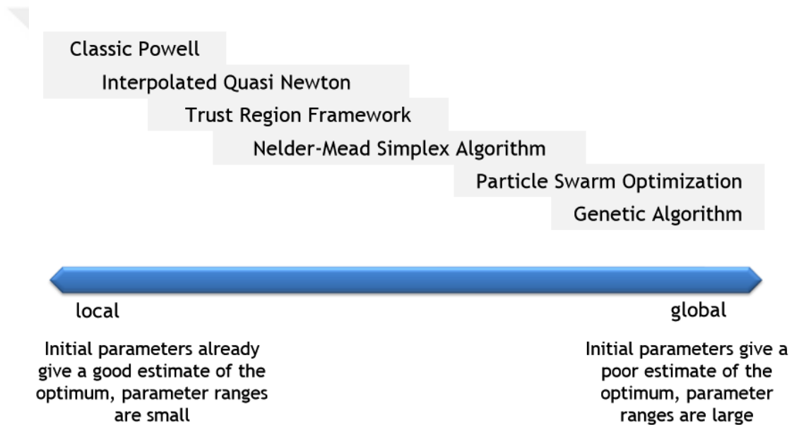
Figure A.1: Choice of optimization algorithm depending on initial parameters
