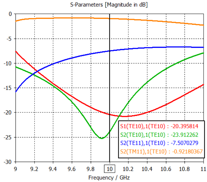
Figure 3.54: S parameter results of obtained E-plane corner TE_{10} to TE_{11}+TM_{11} mode converter with two metallic posts
