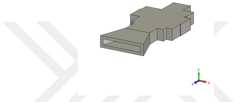
Figure 3.21: Horn antenna and designed 5 stepped TE_{10} to TE_{20} converter structure
