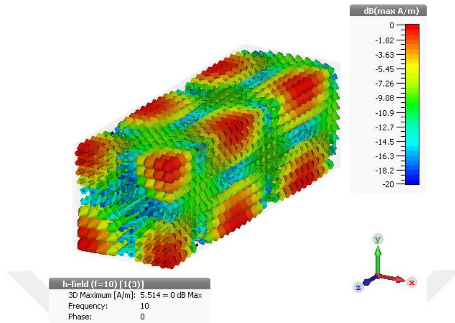
Figure 2.19: Magnetic field vectors of TE_{11} mode inside rectangular waveguide
