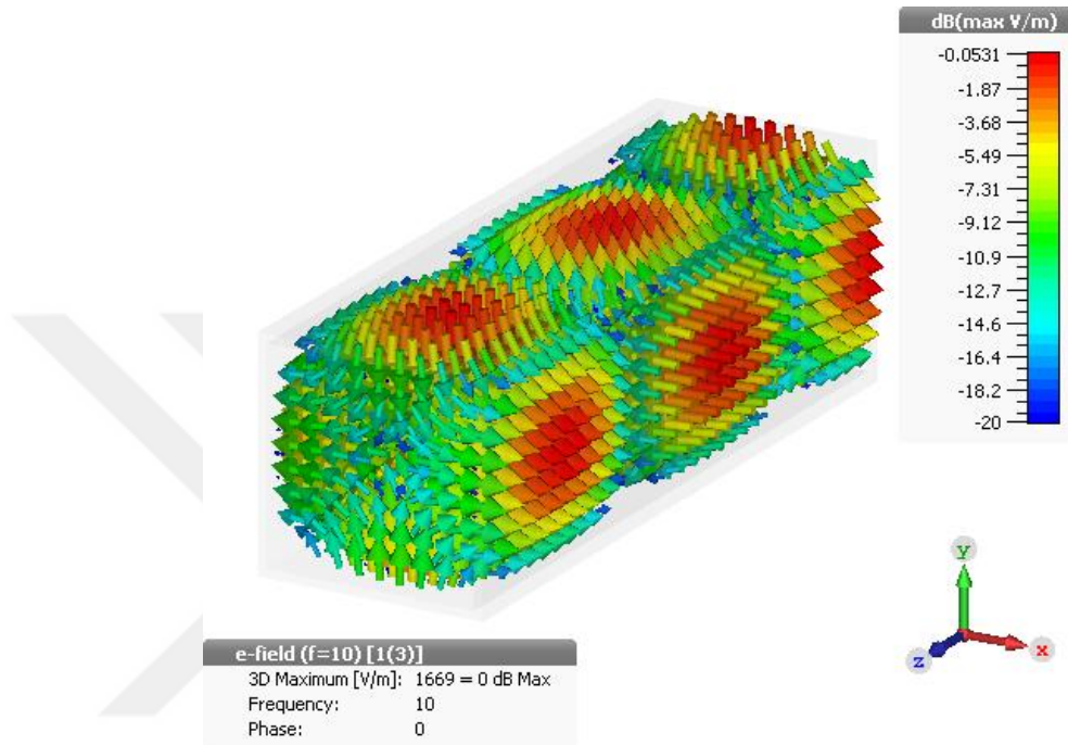
Figure 2.18: Electric field vectors of TE_{11} mode inside rectangular waveguide
