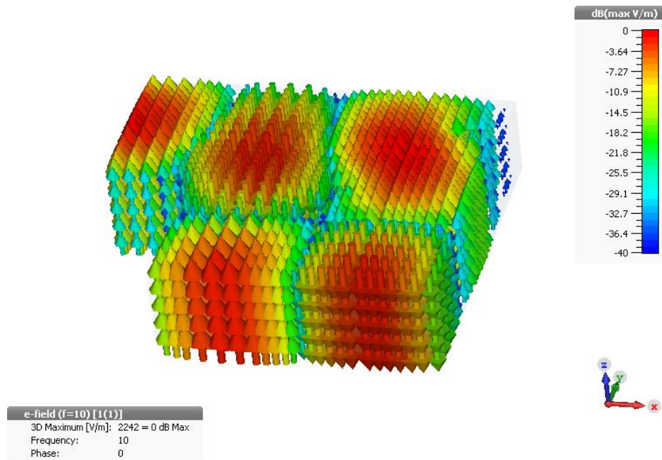
Figure 3.45: Electric field vectors inside investigated \text{TE}_{10} to \text{TE}_{20} converter at 10 GHz
