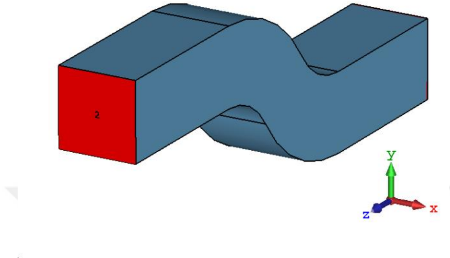
Figure 3.37: Designed TE_{10} to TE_{11}+TM_{11} double E-plane bend mode converter
