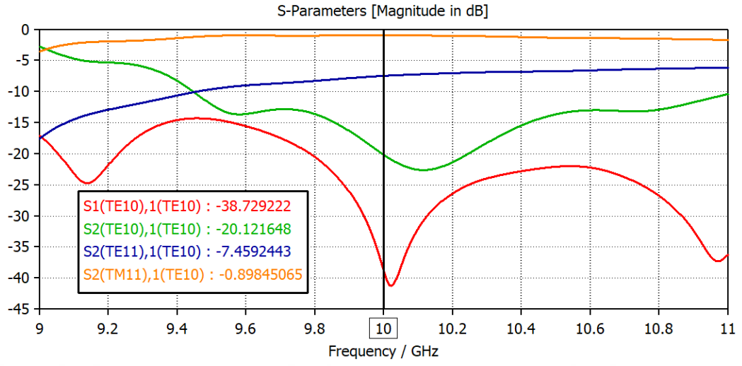
Figure 3.39: S parameter result of designed \text{TE}_{10} to \text{TE}_{11}+\text{TM}_{11} double E-plane bend mode converter
