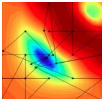
Figure A.3: Visualization of Interpolated Quasi Newton algorithm process
