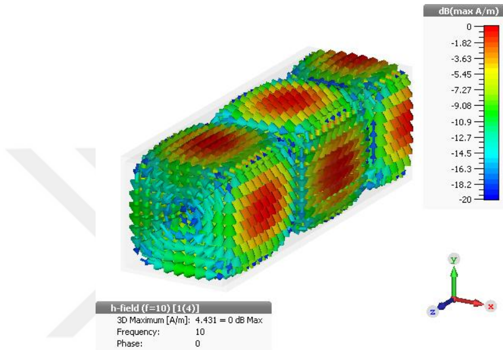
Figure 2.23: Magnetic field vectors of TM_{11} mode inside rectangular waveguide
