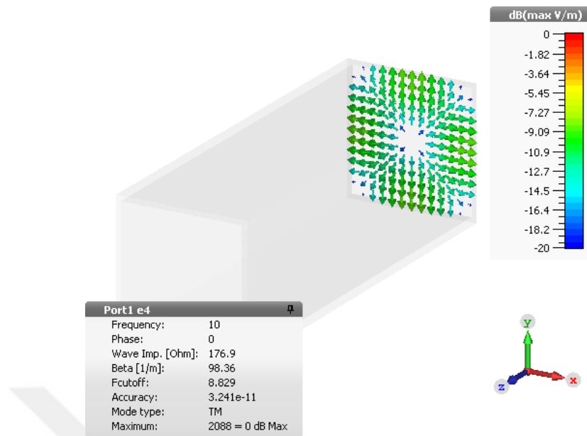
Figure 2.24: Cross sectional electric field vectors of TM_{11} mode at the input
