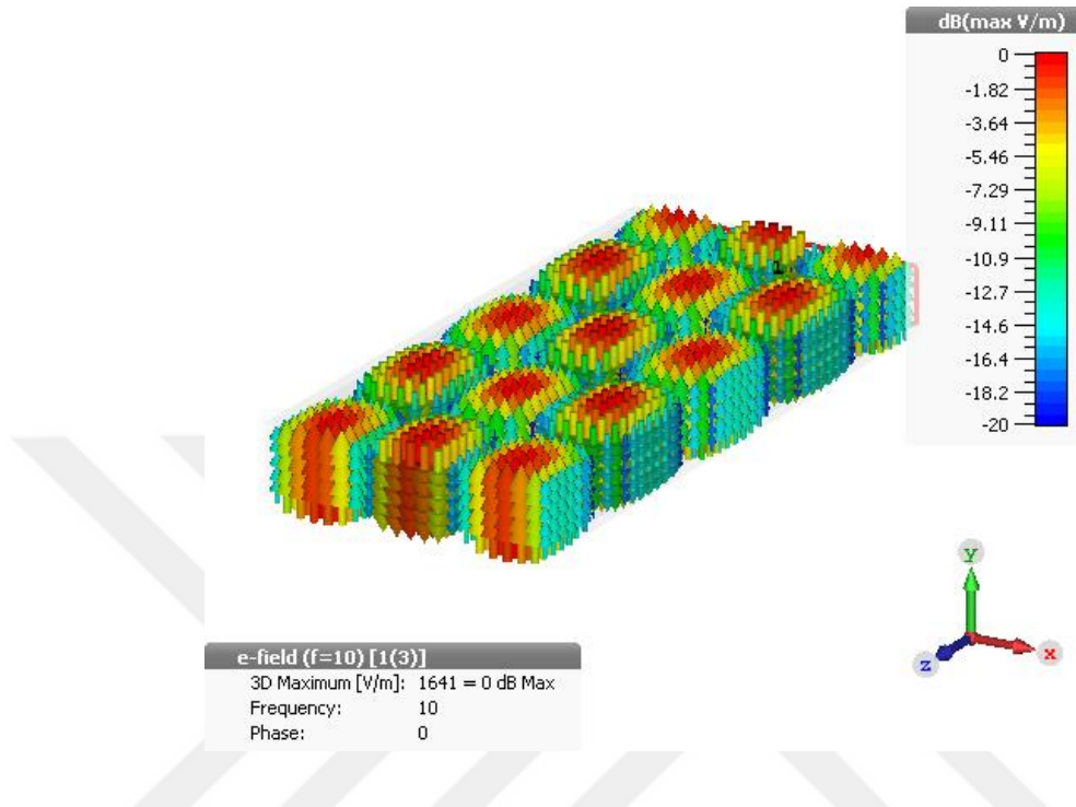
Figure 2.13: Electric field vectors of TE_{30} mode inside rectangular waveguide
