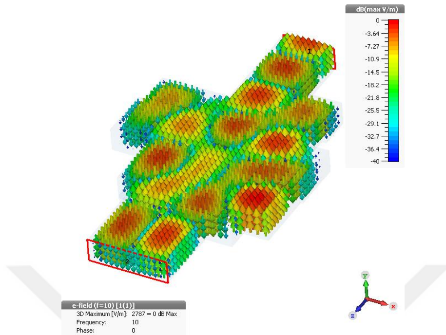
Figure 3.19: Electric field vectors inside designed 5 stepped TE_{10} to TE_{20} converter at 10 GHz
