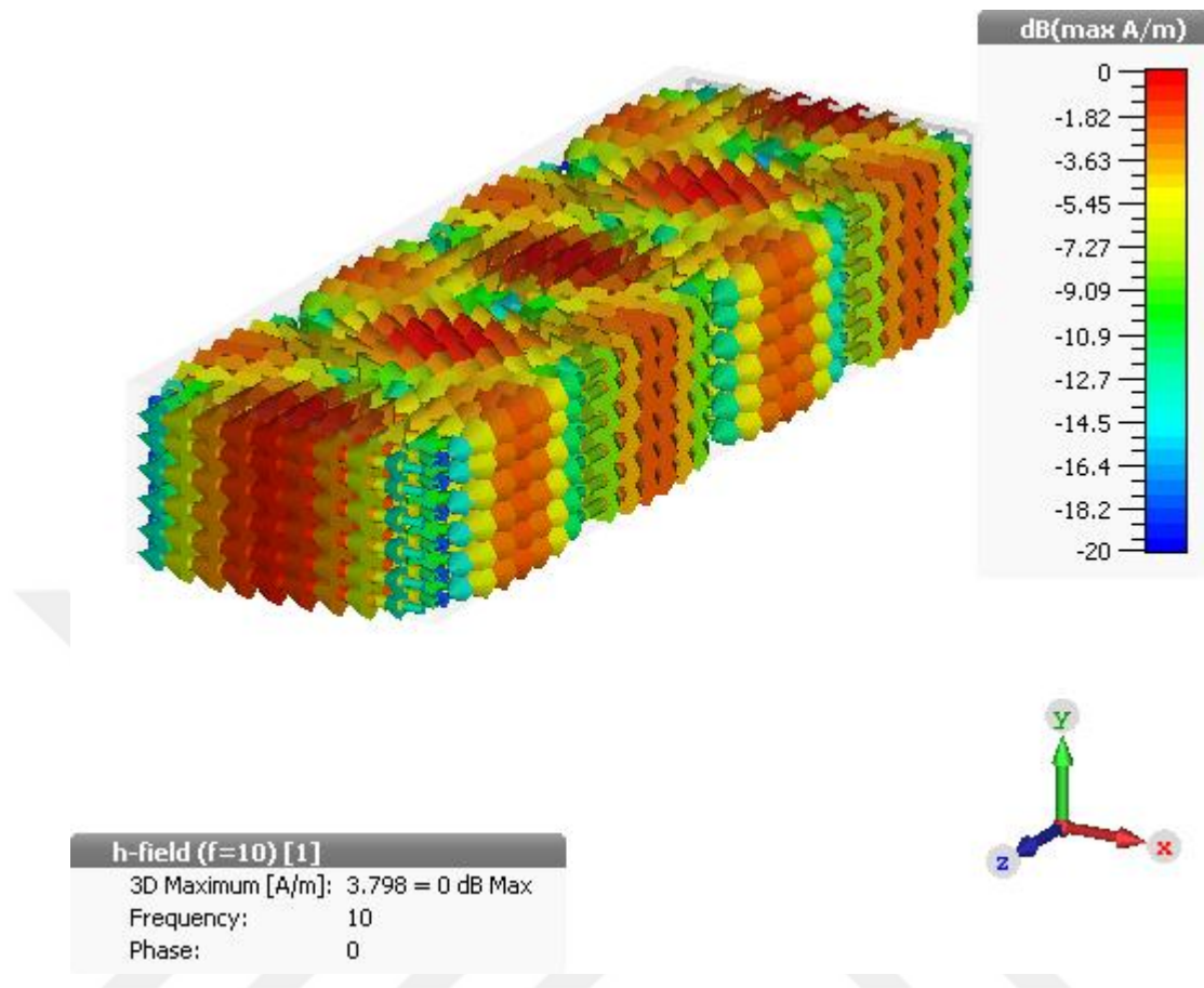
Figure 2.4: Magnetic field vectors of TE_{10} mode inside rectangular waveguide
