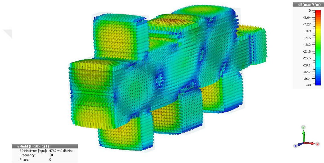
Figure 3.29: Electric field vectors inside designed 5 stepped TE_{10} to TE_{11}+TM_{11} converter at 10 GHz
