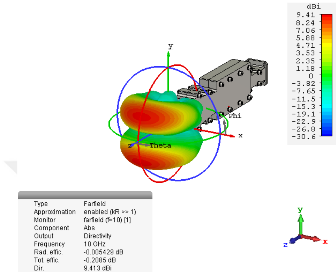
Figure 4.6: 3D radiation pattern of fabrication model
