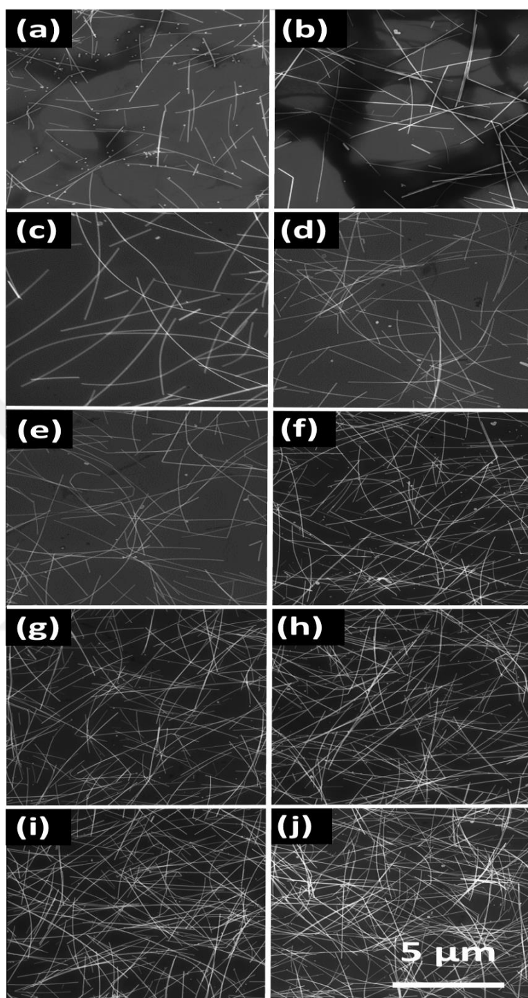
Figure 3.31 SEM images of Ag NWs networks with different densities of (a) 0.28, (b) 0.34, (c) 0.44, (d) 0.50, (e) 0.59, (f) 0.70, (g) 0.82, (h) 0.98, (i) 1.35 and (j) 1.62 NW/ \mu\text{m}^2 .
