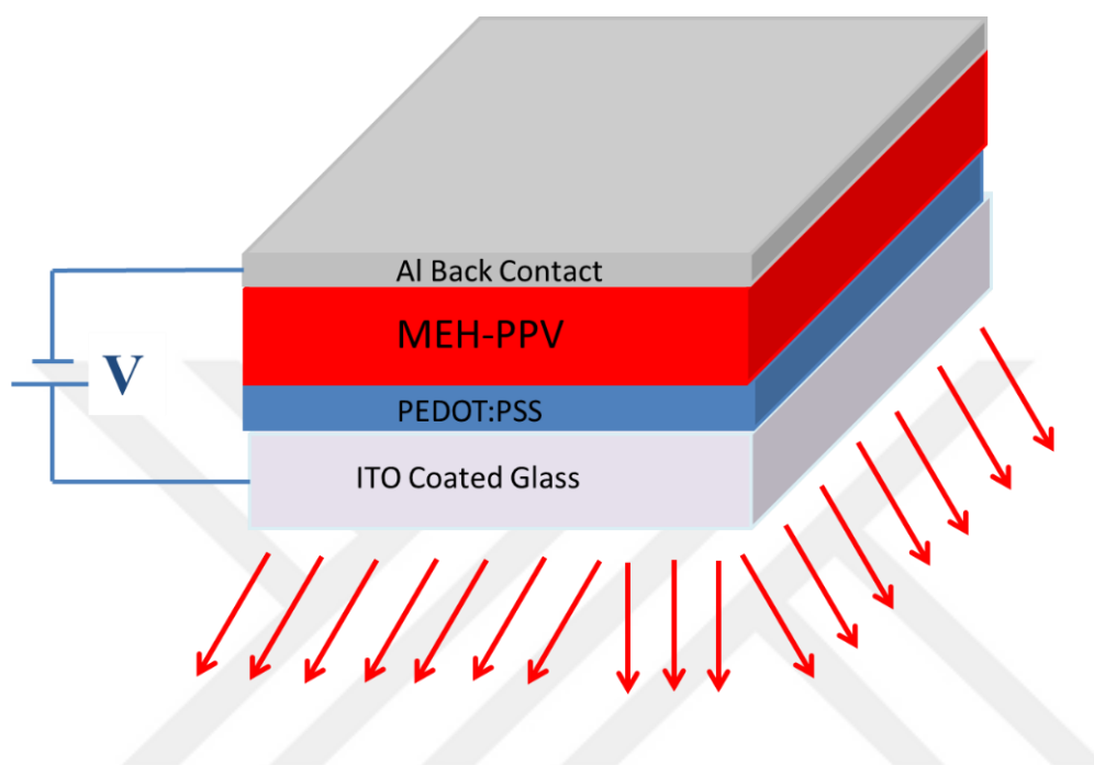
Figure 4.1 Schematic of a typical MEH-PPV based PLED.
