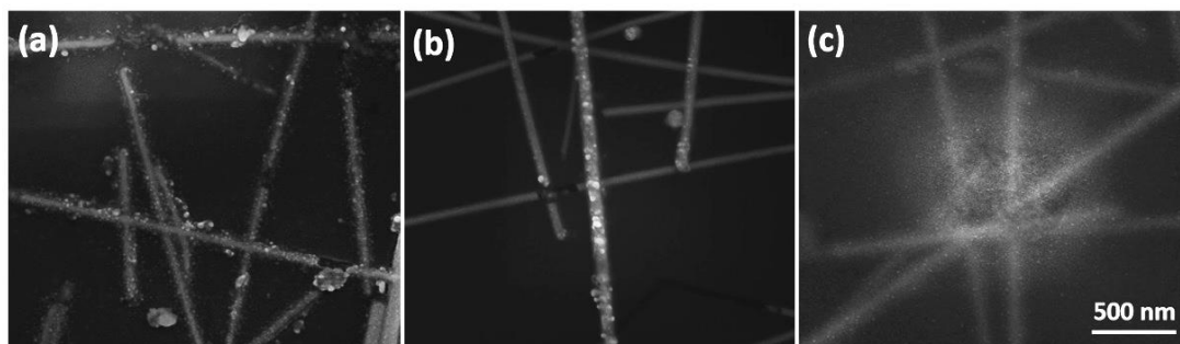
Figure 6. 13 SEM images of (a) 5, (b) 10 and (c) 15 times NiO deposited Ag NW networks after 4 months. Under ambient conditions. All scales are the same.
