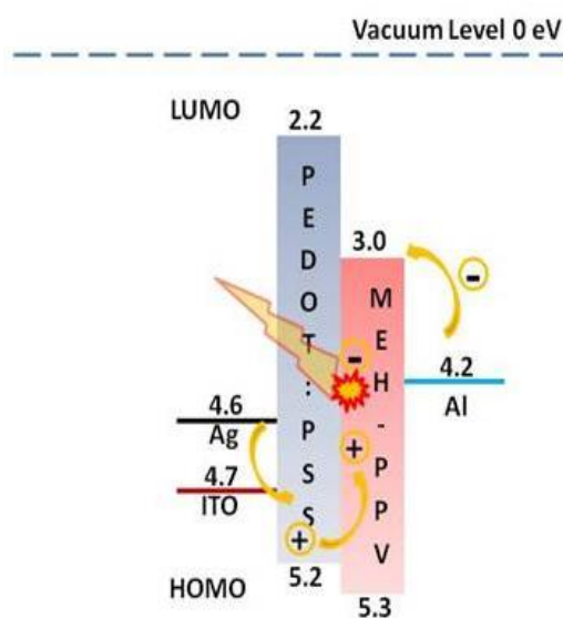
Figure 4.8 Corresponding band diagram of the fabricated PLED devices with both ITO and Ag NW network anodes.
