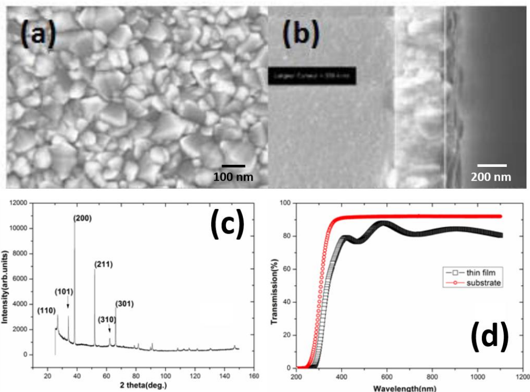
Figure 3.8 (a) Top and (b) cross-sectional FESEM images of FTO thin films. (c) XRD pattern and (d) UV-visible transmission spectra of FTO thin films deposited at 420°C [57].
