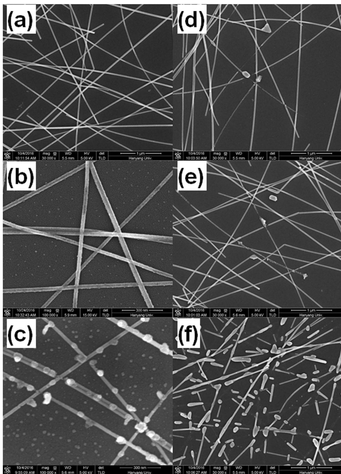
Figure 5.6 SEM images of the (a) pristine Ag NWs, (b) 30 minutes UV/O 3 -treated Ag NWs, (c) 60 minutes UV/O 3 -treated Ag NWs, and the Ag NWs thermally treated at (d) 160, (e) 190, and (f) 210 °C for 10 minutes [89].
