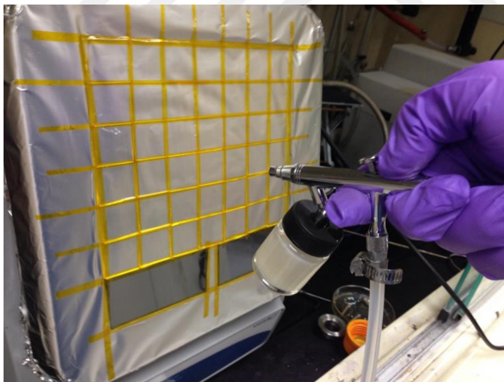
Figure 6.3 Image of spray deposition set-up for silver nanowire coating.
