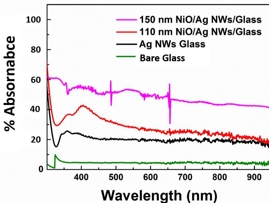
Figure 6.17 Percent absorbance of NiO / Ag NW nano composites.
