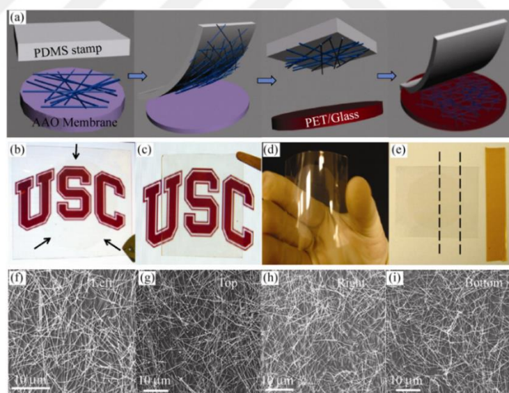
Figure 3.23 (a) Schematic representation of the transfer process. (b) Photograph of an Ag NW film transferred onto PET. (c) Photograph of a nanowire film on glass substrate. (d) Photograph of a nanowire film on PET showing the flexibility of film. (e) Photograph showing the results of adhesion tests. Nanowires remain adhered to the PET substrate when sticky tape was peeled off from the area shown by dotted
