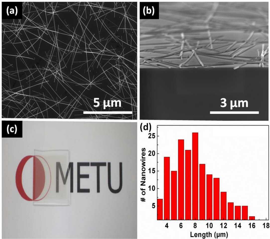
Figure 3.30 SEM images of top view (a) and 35° inclined view (b) of Ag NW networks fabricated in this work. (c) Photograph of Ag NW networks on a glass substrate. (d) Length distribution of Ag NWs used for the fabrication of networks [76].
