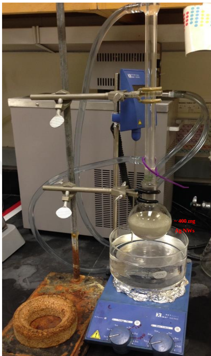
Figure 2.10 The experimental setup for Ag NW synthesis by modified polyol process.
