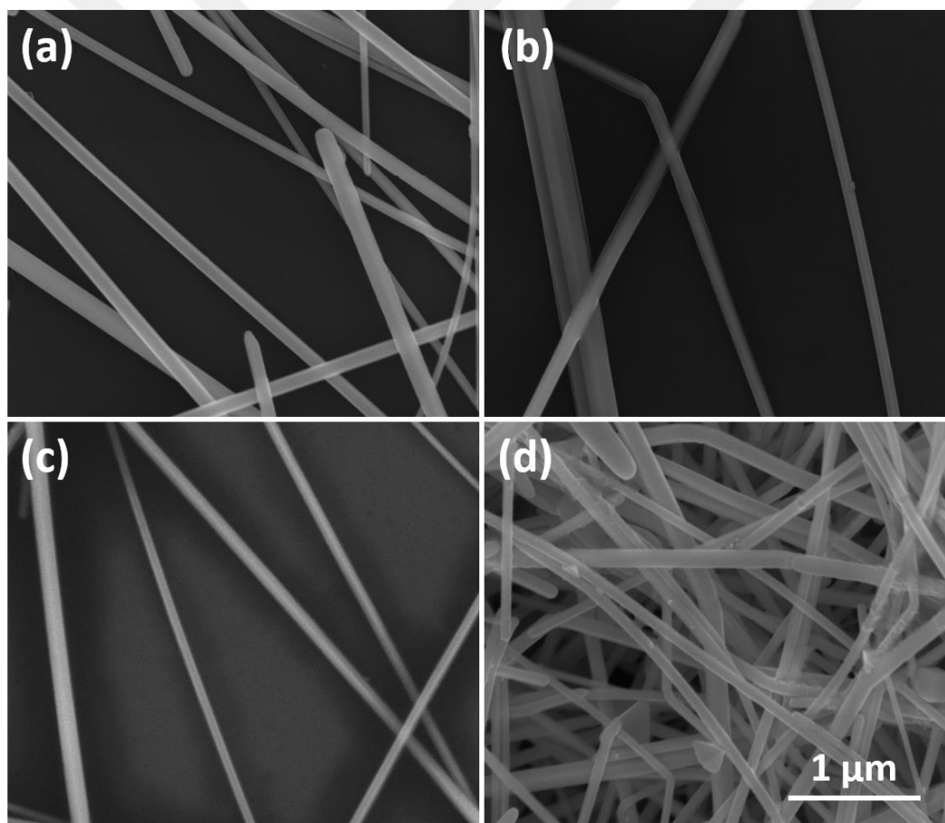
Figure 5.19 SEM images of Ag NWs kept in (a) DI water, (b) ethanol, (c) IPA and (d) chloroform at 4°C for 2 years. All scales are the same.
