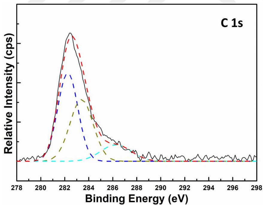
Figure 5.16 High-resolution XPS spectrum of C 1s.
