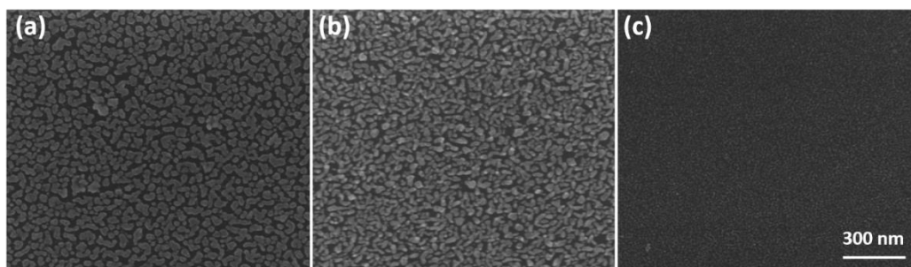
Figure 6.8 SEM images of NiO thin films on silicon substrates annealed at different temperatures of (a) 400, (b) 450 and (c) 500 °C [99].
