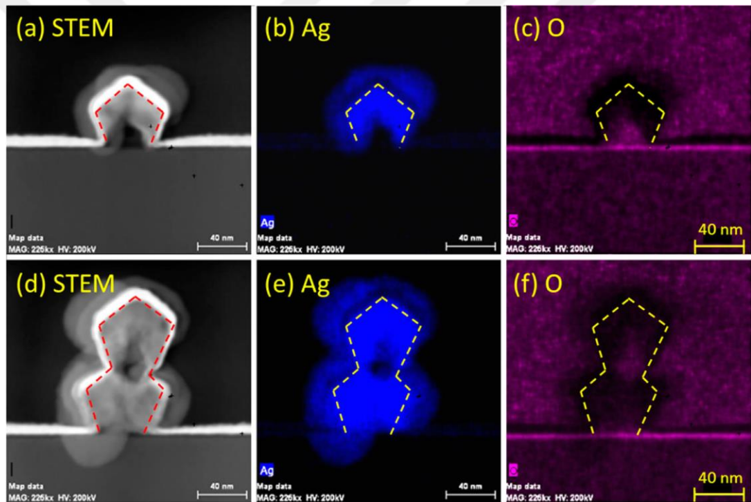
Figure 5.2 Cross-sectional STEM and EDS mapping images of oxidized sample. (a–d) STEM images of a single Ag NW and stacked Ag NWs. EDS mapping images in (b) and (e) correspond to Ag atoms and those in (c) and (f) for O atoms. Dashed lines are guides for the eyes of pentagonal Ag NWs [87].
