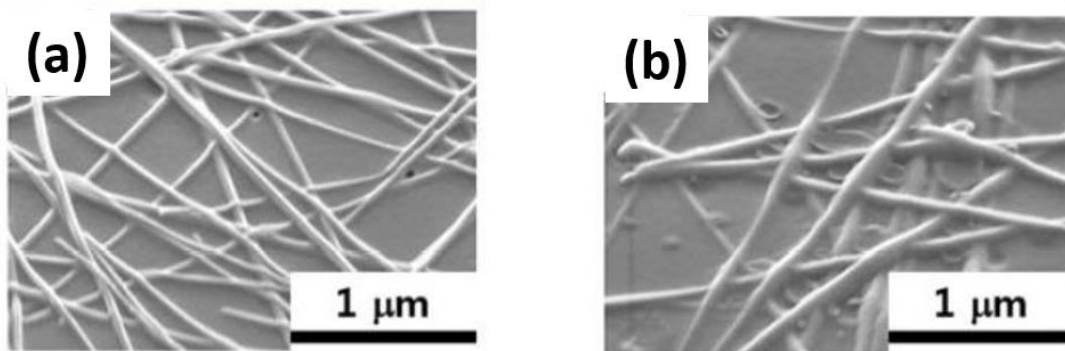
Figure 6.2 Tilted cross-sectional SEM image of transferred Ag NWs (a), a composite Ag NW/IZO film (b) [91].
