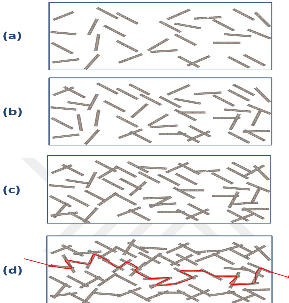
Figure 3.18 Schematics showing how 1D structures can provide suitable paths for charge transport.
