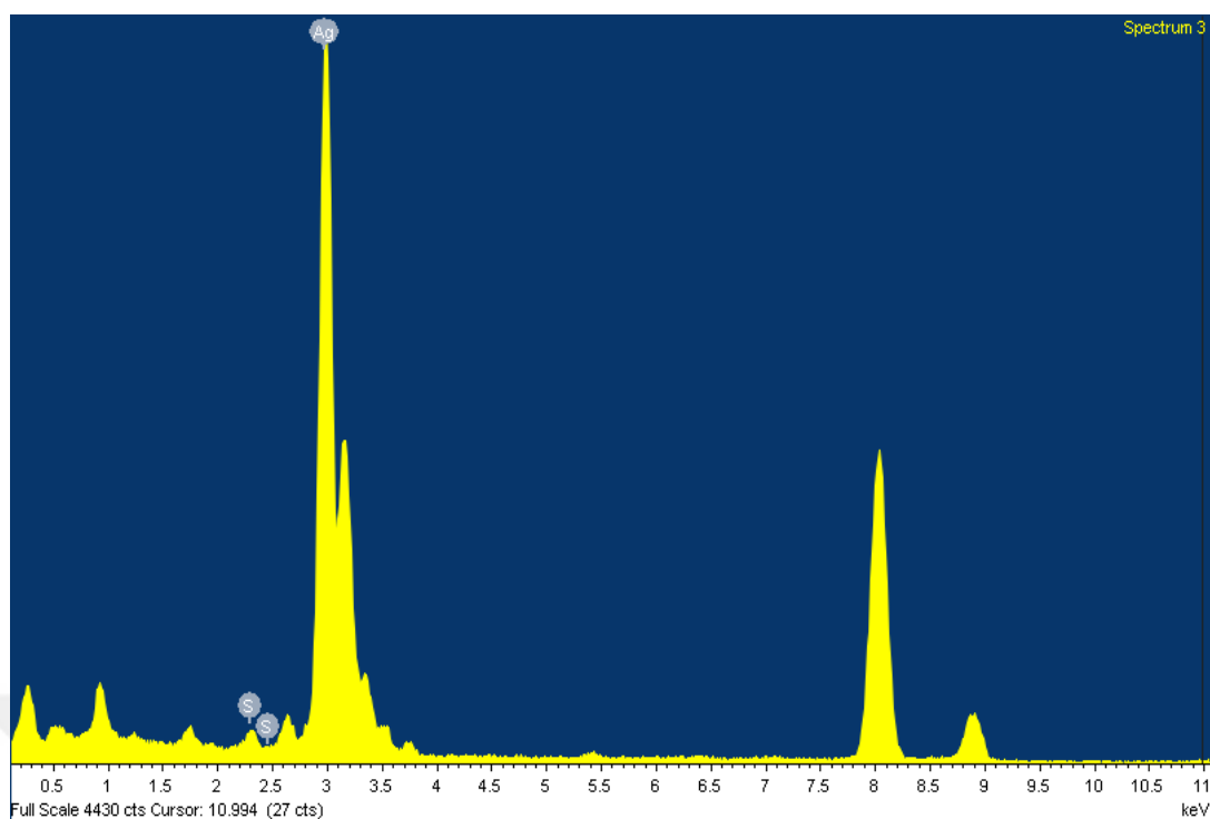
Figure 5.12 EDS analysis of an Ag NW with nanoparticles on its lateral surfaces.
