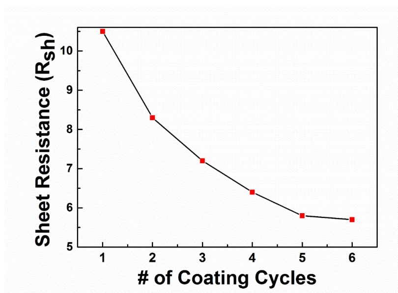
Figure 6. 14 Change in sheet resistance for NiO / Ag NW nano composites with the number of NiO deposition cycles.
