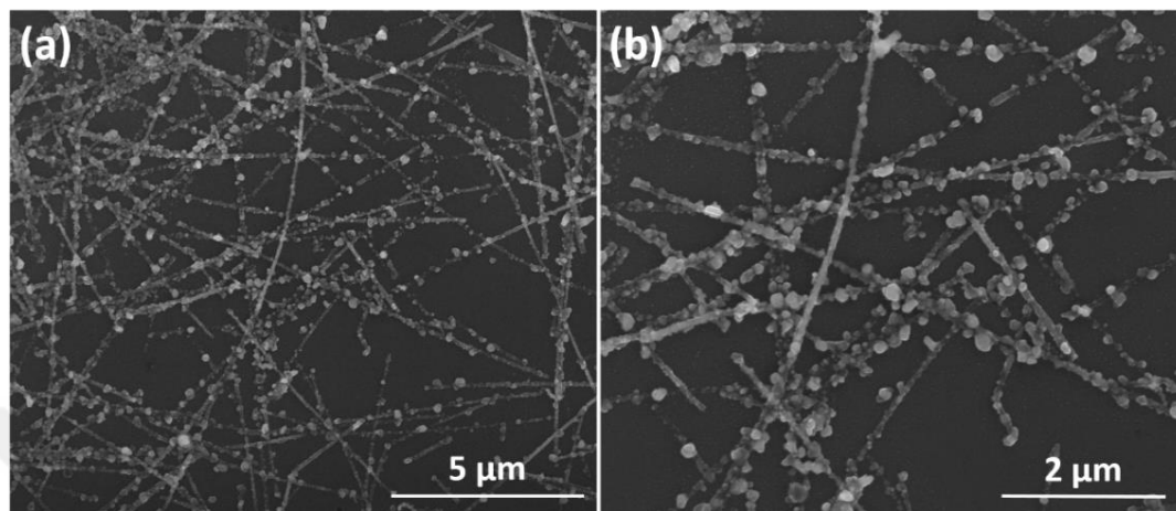
Figure 6.18 SEM images of (a) and (b) 5X (60 nm) NiO deposited Ag NW networks after 18 months storage under ambient conditions.
