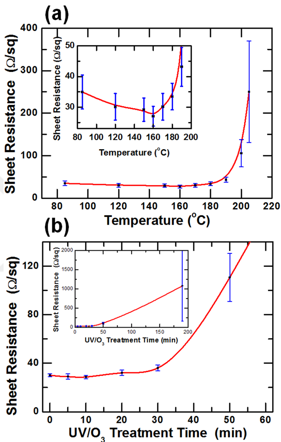
Figure 5.5 Sheet resistance of the Ag NW electrodes as functions of the (a) thermal treatment temperature and (b) UV/O 3 treatment time [89].
