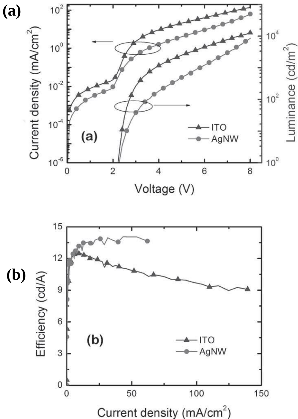
Figure 4.2 I - V - L curves of PLEDs having a sandwich structure of AgNWs (or ITO) anode/PEDOT:PSS/SY-PPV/CsF/Al (a) and the luminous efficacy and current density graph of the fabricated devices (b) [79].
