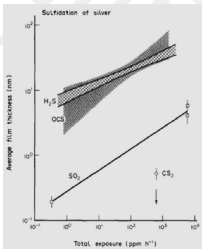
Figure 5.1 Growth rates of \text{Ag}_2\text{S} when exposed to various ambient sulfur-containing gases such as \text{H}_2\text{S} , OCS, \text{SO}_2 and \text{CS}_2 [86].
