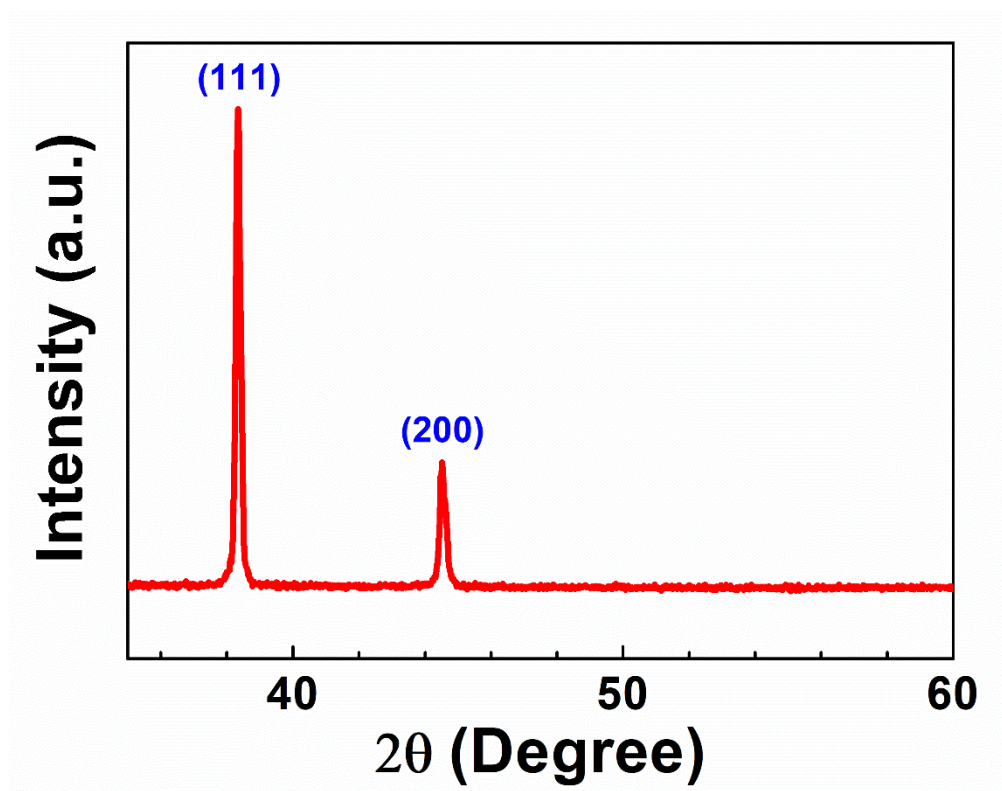
Figure 2.17 XRD spectrum of Ag NWs (JCPDS Card No. 04-0783) synthesized using modified polyol process.
