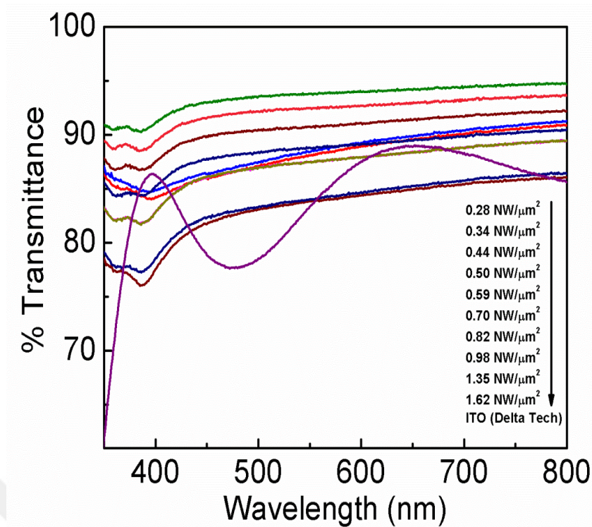
Figure 3.32 Transmittance spectra of Ag NW networks with different densities [76]. Transmittance spectrum for a commercial ITO thin film is also provided for comparison.
