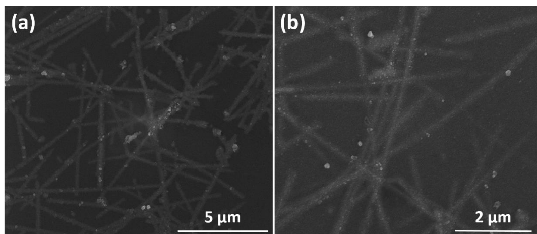
Figure 6.20 SEM images of (a) and (b) 15 times NiO deposited Ag NW networks after 18 months under ambient conditions.
