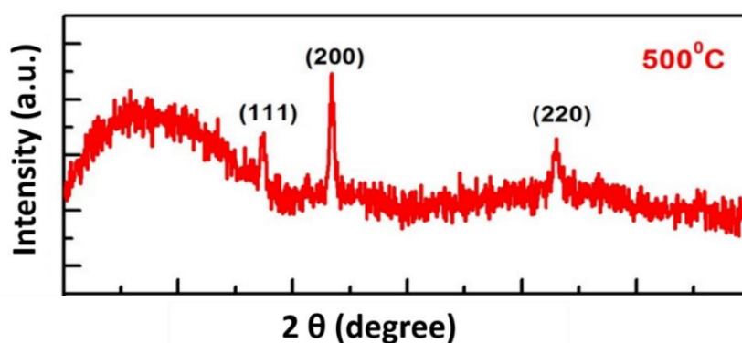
Figure 6.6 XRD pattern of a NiO thin film annealed at 500° C (JCPDS card no 47-1049) [99].
