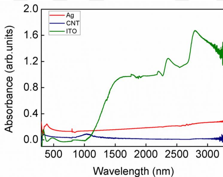
Figure 3.33 Absorption spectra of Ag NW networks, SWCNT thin films and commercial ITO.
