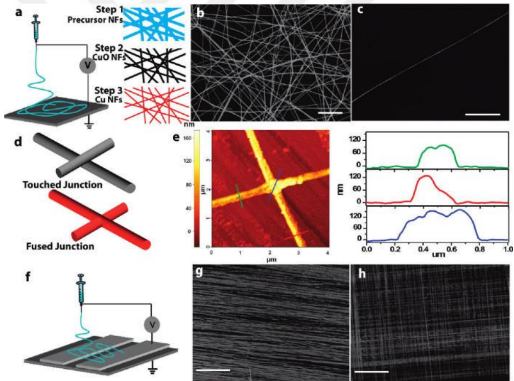
Figure 3. 16 Fabrication and characterization of Cu nanofibers. (a) Schematic of materials preparation method. Left column: Schematic of an electrospinning setup, shown without a syringe pump. Right column: the fabrication process of Cu nanofibers. In the first step, CuAc2/PVA composite fibers were prepared by electrospinning. In step 2, the fibers were calcinated in air to get CuO nanofibers. In
