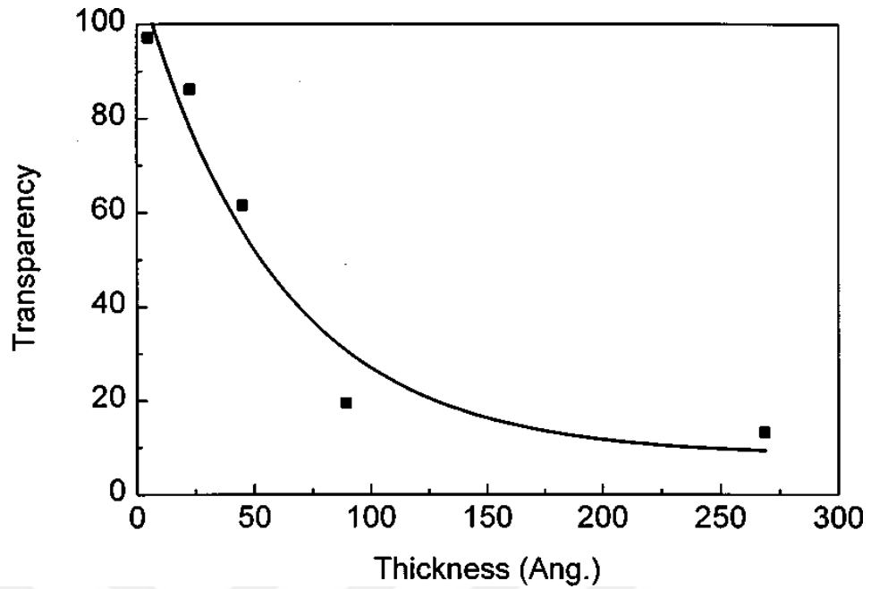
Figure 3.12 Transparency vs. thickness graph for Pt films [61].
