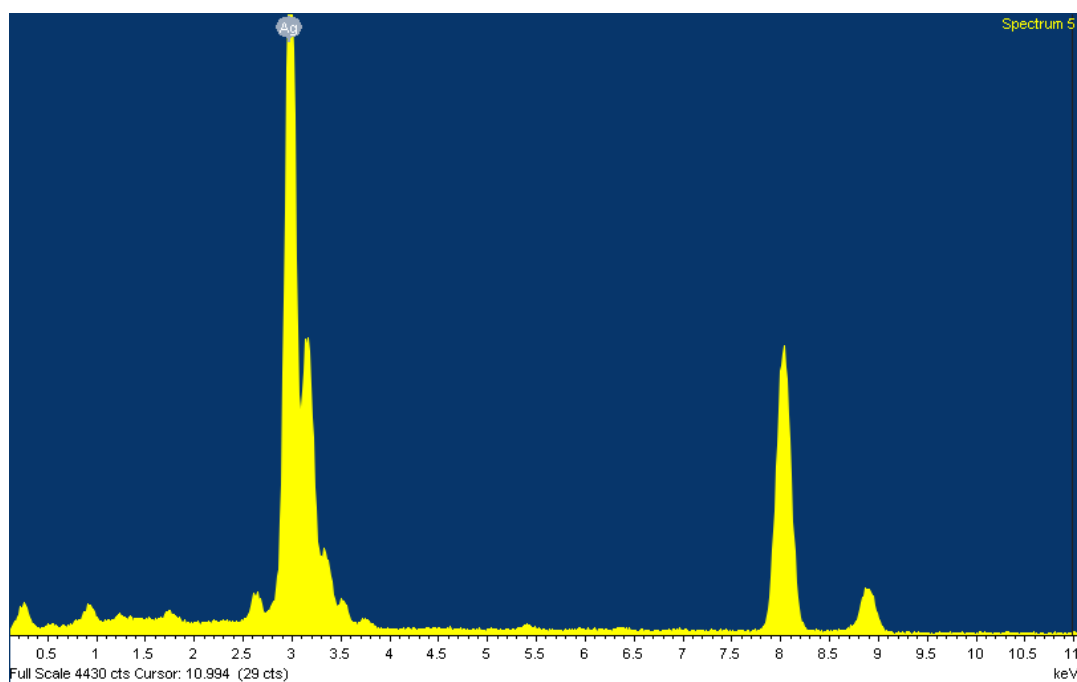
Figure 5.11 EDS analysis of a Ag NW in as-prepared condition.
