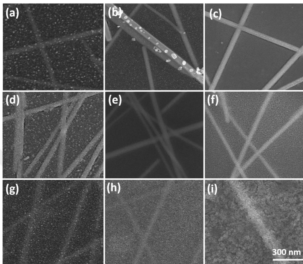
Figure 6.12 SEM images of NiO/Ag NW nano composite films on Si substrates annealed at different temperatures with different coating cycles (a) 5 times, (b) 10 times, (c) 15 times at 400 °C , (d) 5 times, (e) 10 times, (f) 15 times 450 °C, (g) 5 times, (h) 10X times and (I) 15 times 500 °C under argon atmosphere.
