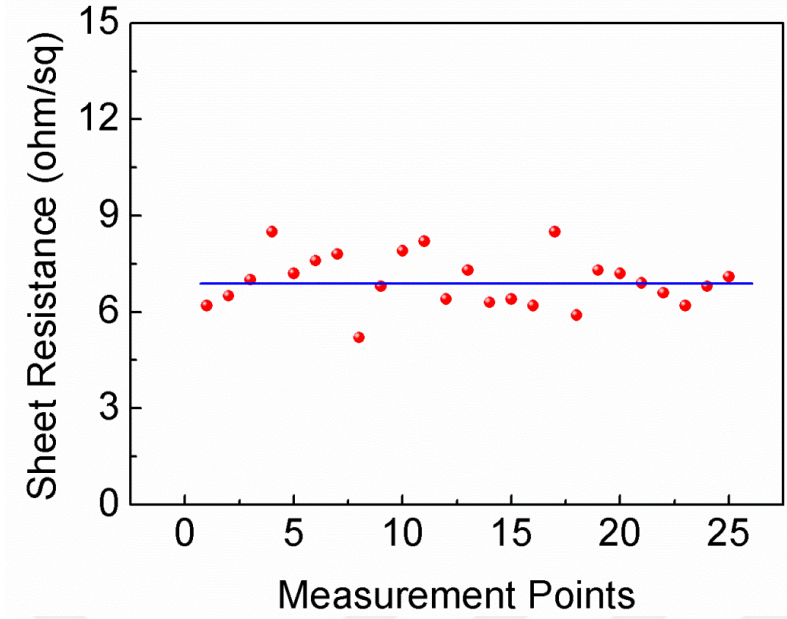
Figure 3.42 Change in sheet resistance of an Ag NW network measured at 25 different spots on the sample [76].
