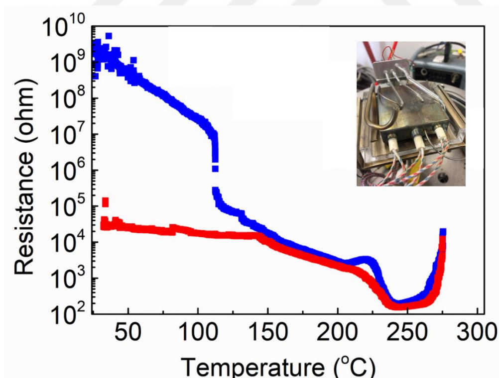
Figure 5.21 Resistance change in Ag NW nanowire networks with increasing temperature. Inset show photograph of the measurement setup.
