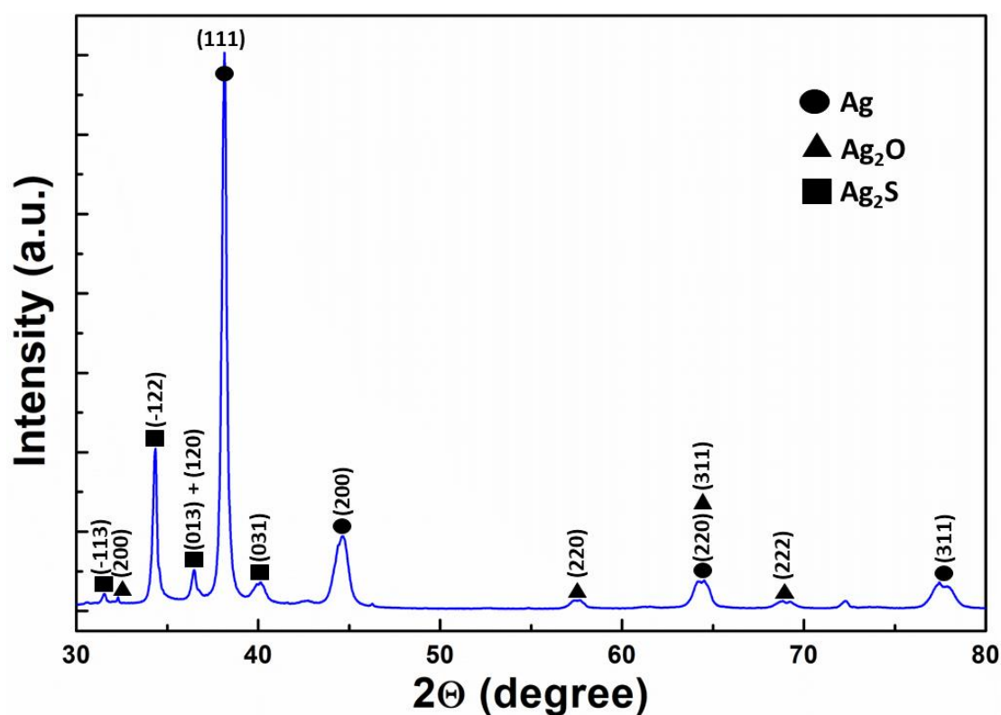
Figure 5.13 XRD spectrum of corroded Ag NWs. (JCPDS card no 04-0783 for pure Ag, 76-1393 for Ag 2 O and 65-2356 for Ag 2 S)
