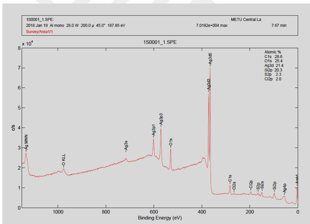
Figure 5.14 XPS survey spectrum of corroded Ag NWs.
