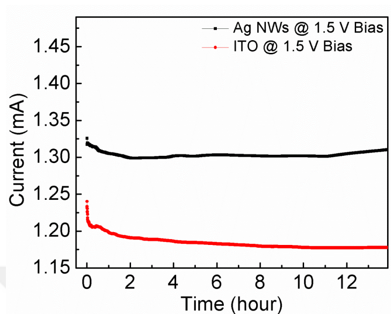
Figure 3.43 Current stability of ITO and Ag NW networks [76].
