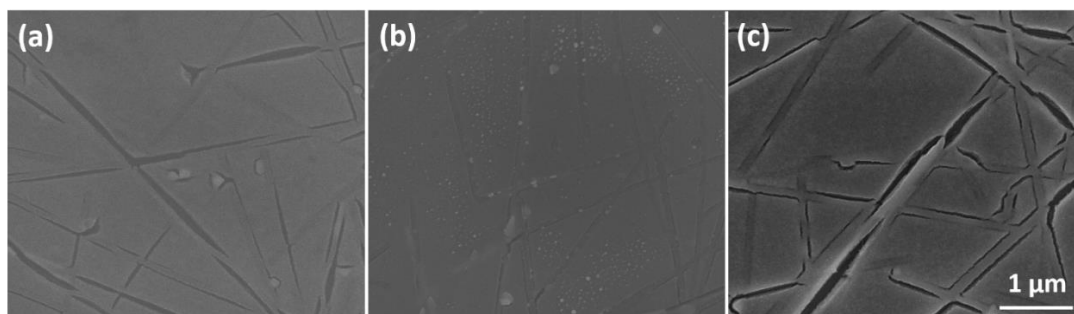
Figure 6.11 SEM images of NiO / Ag NWs thin films on silicon substrates annealed at 500 °C in air atmosphere (a) 5x, (b) 10x and (c) 15x.
