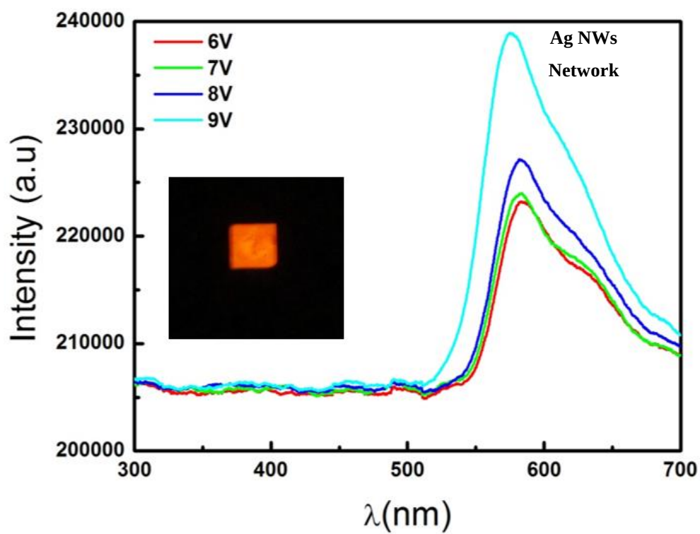
Figure 4.11 Electroluminescence characteristics of PLED device with Ag NWs networks anode [76]. Inset shows a photo of emission.
