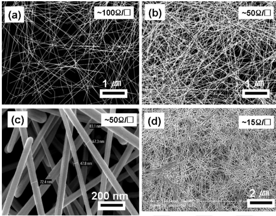
Figure 3.21 SEM images of Ag NW films with different densities. The different densities of Ag NW films lead to different sheet resistances: (a) 100, (b and c) 50, and (d) 15 \Omega /sq. The diameters of the Ag NWs are in the range of 40-100 nm [75].
