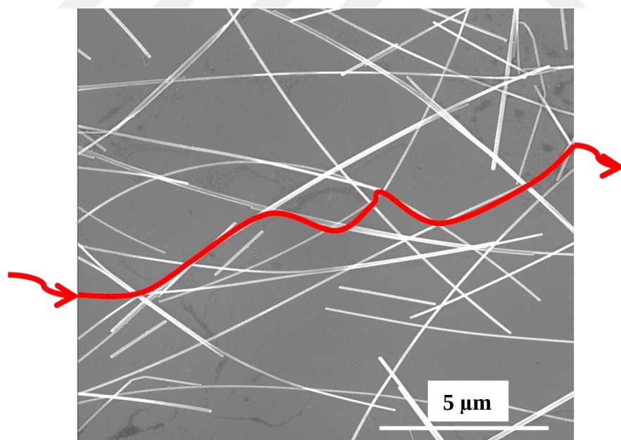
Figure 3.27 Representative SEM image of Ag NW network and possible path for charge transport.
