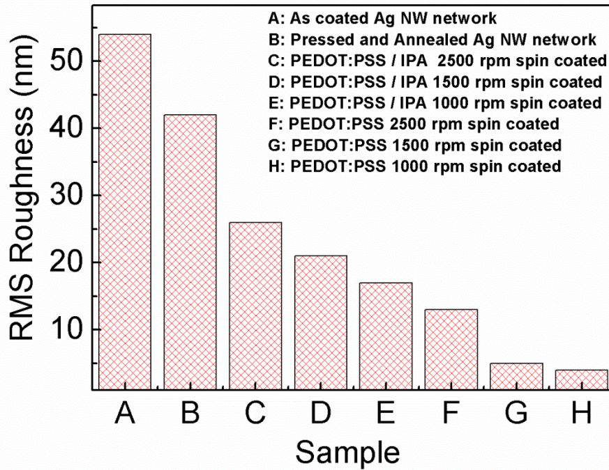
Figure 4.6 RMS roughness change of different Ag NW network samples [76].
