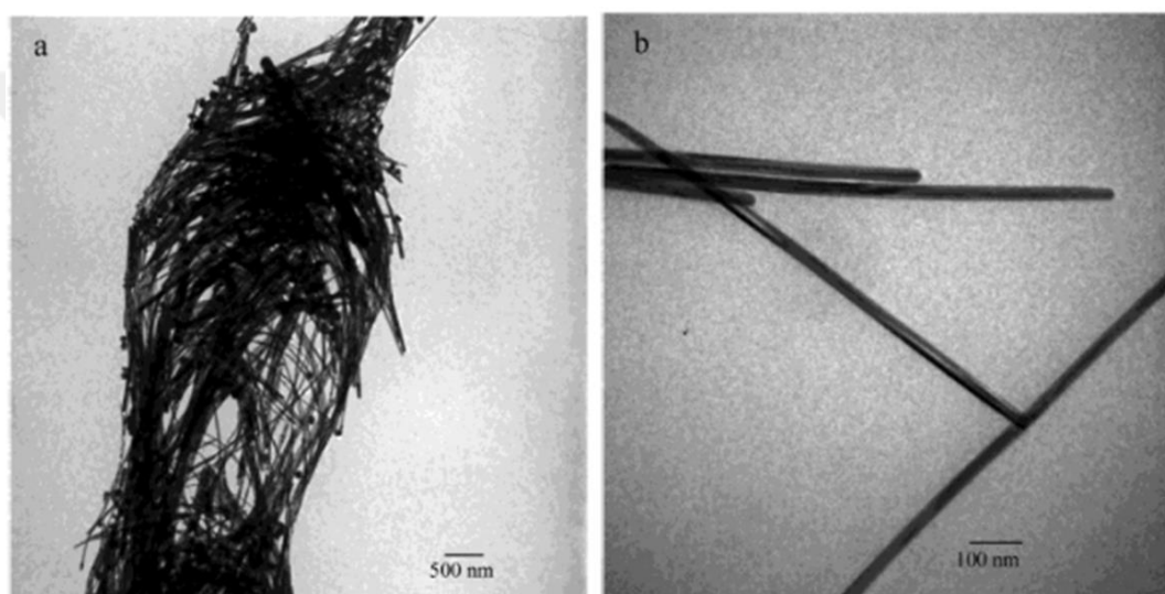
Figure 2.5 TEM micrographs of Ag NWs synthesized with 3 \mu\text{L} of NaOH added at magnifications of (a) 15 kX and (b) 100 kX [40].
