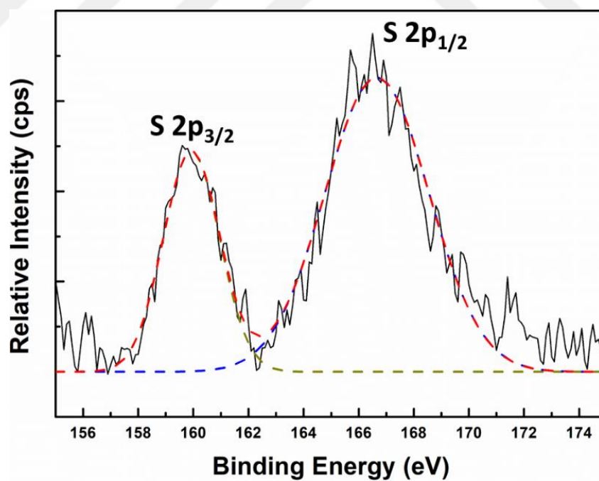
Figure 5.18 High resolution XPS spectrum of S 2p.
