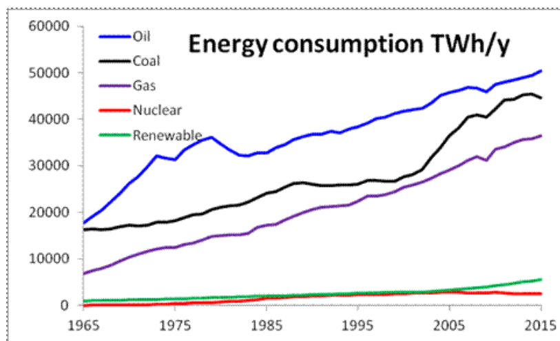
Figure 3.2 Energy consumption vs. year [51].
