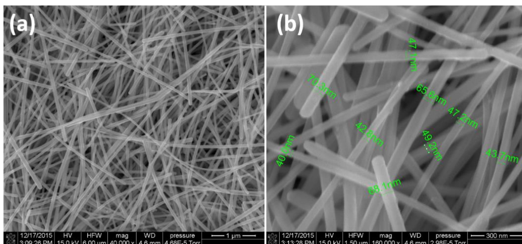
Figure 2.15 (a) Low and (b) high resolution SEM images of as synthesized Ag NWs using modified polyol process.
