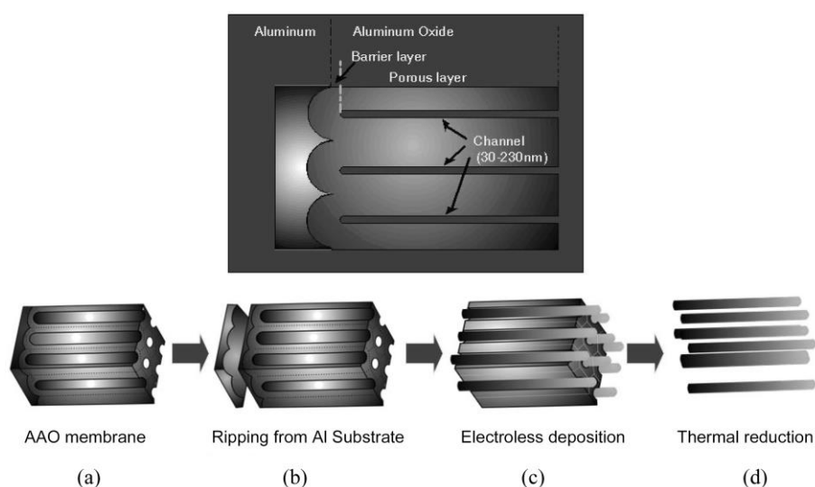
Figure 2.1 Schematic presentation of Ag NW formation in AAO prepared by electroless deposition and thermal reduction. (a) The AAO membrane was fabricated by a two-step anodization process through pore widening. (b) Ripping the aluminum
