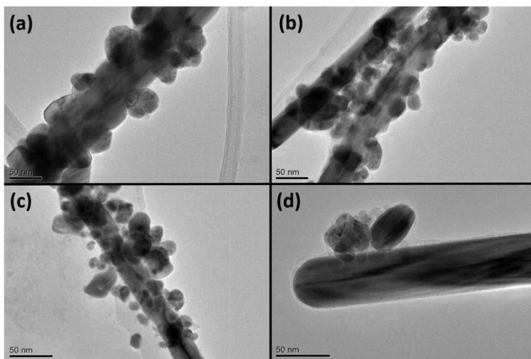
Figure 5.9 TEM images of various corroded Ag NWs with as formed nanoparticles on their lateral surfaces (a), (b), (c) and (d).
