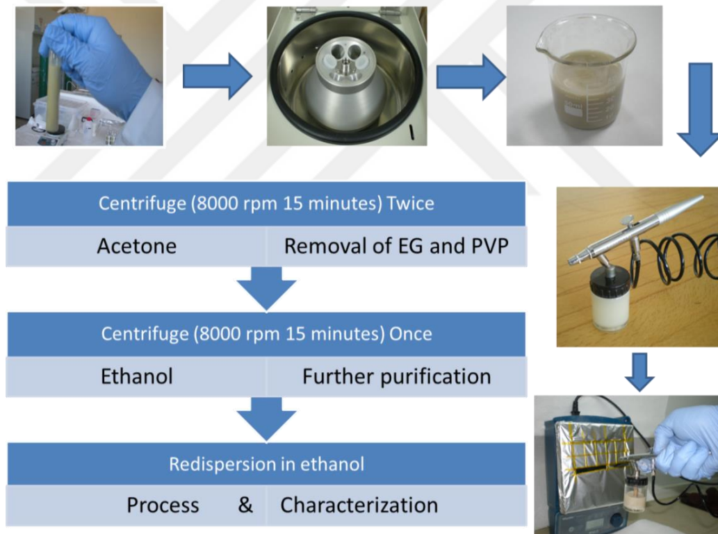
Figure 3.26 Flow chart showing the nanowire purification and deposition of Ag NWs onto substrates [48].
