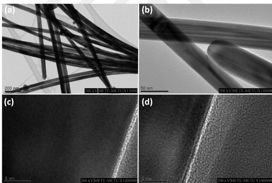
Figure 2.16 (a) and (b) TEM and (c) and (d) HRTEM images of as synthesized Ag NWs using modified polyol process.
