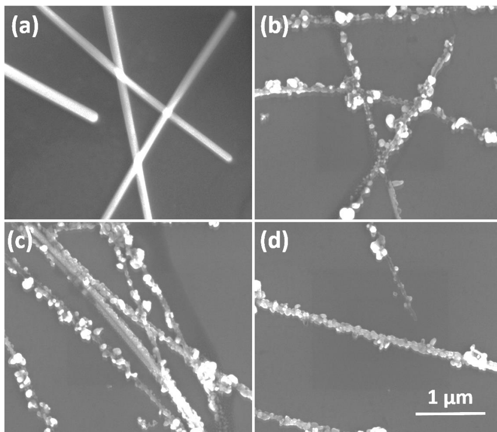
Figure 5.7 SEM images of Ag NW networks that are (a) as-prepared and kept in ambient conditions for 6 months (b), (c) and (d).
