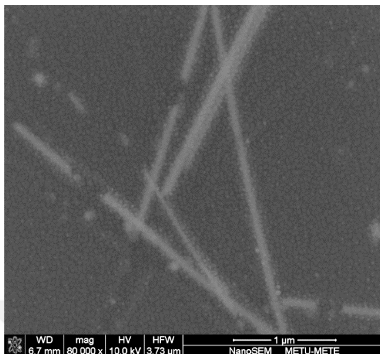
Figure 5.8 SEM image of Ag NW networks spin coated with PEDOT:PSS and kept under protective atmosphere for 1 month.
