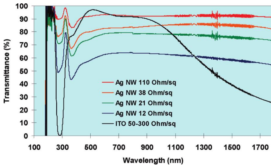
Figure 3.22 Optical transmittance of Ag NW network electrodes compared to a commercial ITO thin film [75].
