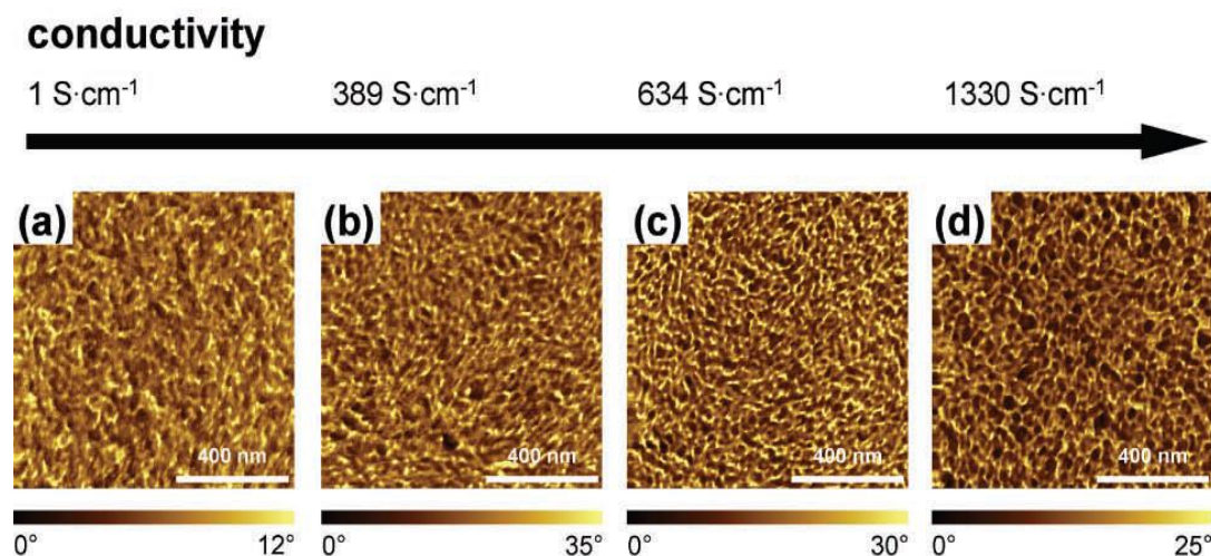
Figure 3. 9 AFM phase images of PEDOT:PSS films with various solvent treatments. (a) Pristine PEDOT:PSS (PH1000) ( \sigma < 1 \text{ S cm}^{-1} ). (b) PEDOT:PSS (PH 510) doped with DMSO 5 vol% ( \sigma = 389 \text{ S cm}^{-1} ). (c) PEDOT:PSS (PH 1000) doped with EG 6 vol% ( \sigma = 634 \text{ S cm}^{-1} ). (d) solvent post-treated PEDOT:PSS (PH 1000) doped with EG 6 vol% ( \sigma = 1330 \text{ S cm}^{-1} ) [58].
