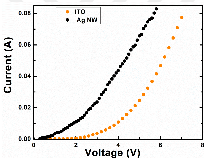
Figure 4.9 Current-voltage (I-V) characteristics of the PLED devices fabricated in this work [76].
