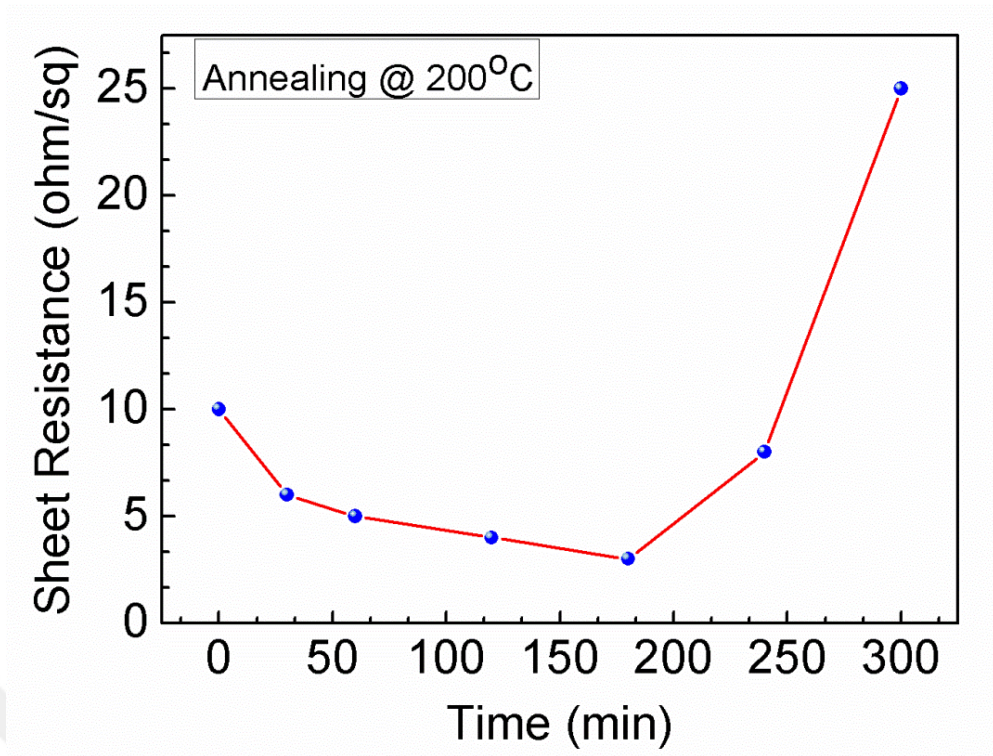
Figure 3.41 Change in sheet resistance of Ag NW networks annealed at 200°C with time [76].
