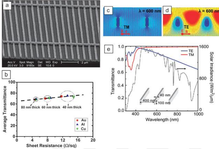
Figure 3.13 (a) SEM image of as-fabricated metal electrodes. (b) Average transmittance versus sheet resistance of metal grids with a line width of 120 nm. Absolute value of the modeled optical electric field and power flow for light (600 nm wavelength) incident on a freestanding Ag grating (400 nm period, 40 nm line width, 100 nm high) for both (c) transverse magnetic (TM) and (d) transverse electric (TE) polarization. (e) Simulated transmittance versus wavelength for two modes. The AM 1.5 solar irradiance data (black line) are plotted for comparison [62].
