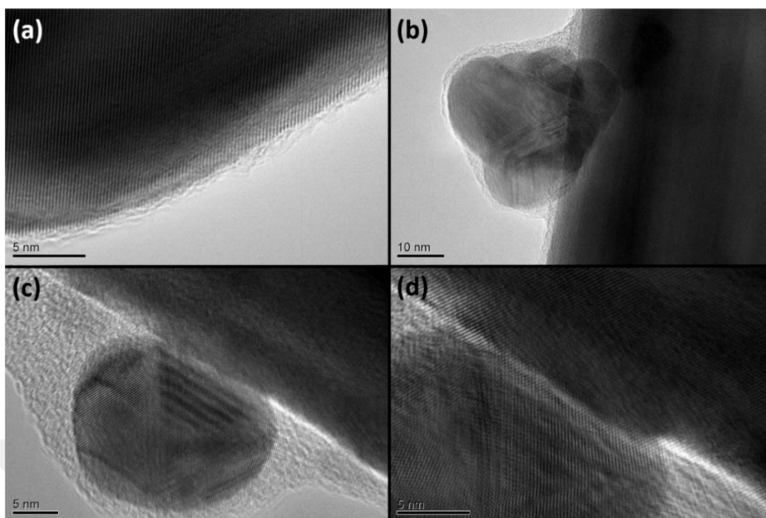
Figure 5.10 HRTEM images of (a) as-prepared and (b), (c) and (d) various corroded Ag NWs with as formed nanoparticles on their lateral surfaces.
