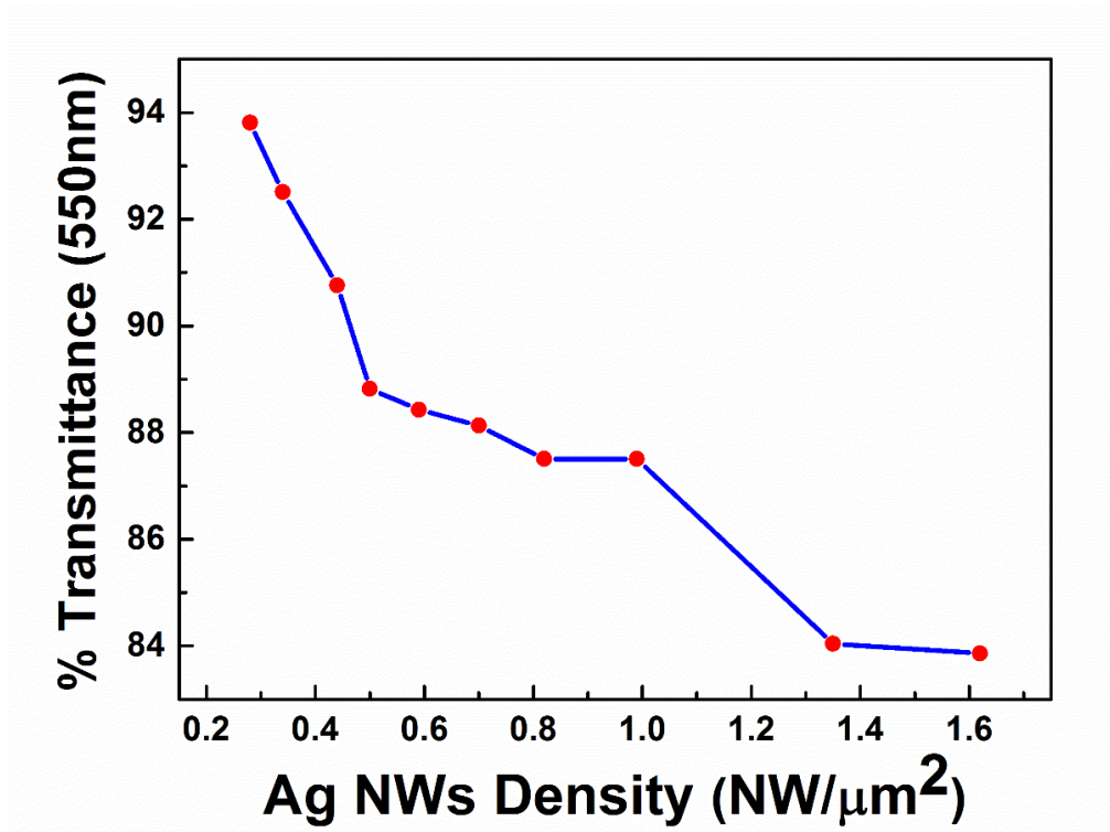
Figure 3.34 Change in transmittance of Ag NW networks at different nanowire densities.
