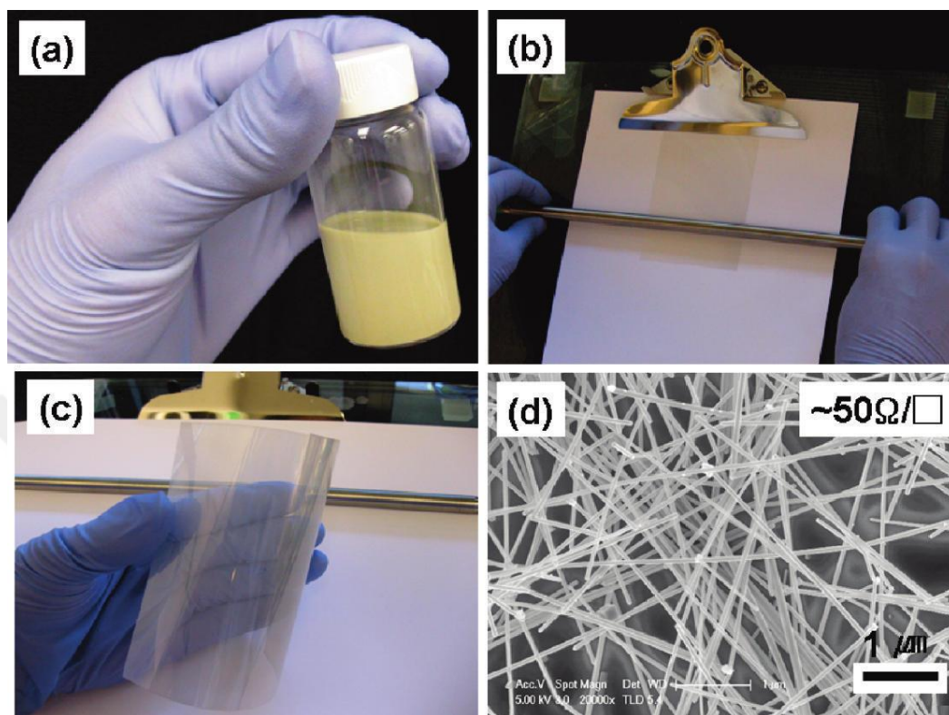
Figure 3. 20 (a) Photograph of Ag NW ink in ethanol. (b) Meyer rod coating setup for scalable Ag NW coating onto plastic substrates. (c) Finished Ag NW film coating on PET substrate. The Ag NW coating looks uniform over the entire substrate shown in the figure. (d) A SEM image of Ag NW coating shown in panel (c). The sheet resistance was 50 \Omega/\text{sq} [75].
