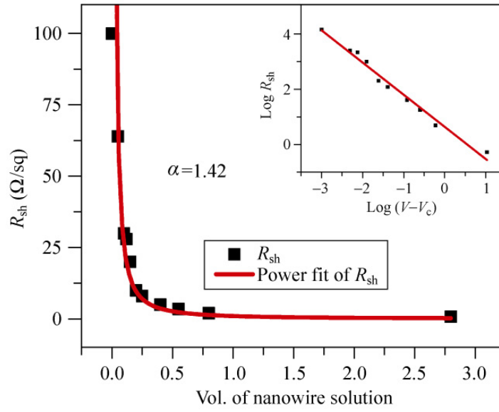
Figure 3.19 Graph of the sheet resistance versus volume of Ag NW solution. The onset of conduction across the sample occurs for V_c = 0.2 mL. The power fit of the data indicated value of critical exponent \alpha = 1.42 . The inset shows the logarithmic plot of the data with a linear fit [73].
