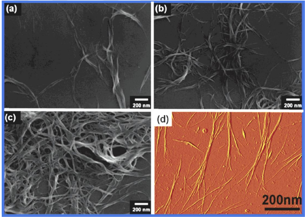
Figure 3.14 SEM images of SWNT films deposited from 40 mL SWNT solutions of (a) 0.2 mg/L, (b) 1 mg/L and (c) 2 mg/L concentrations. (d) AFM image of the 1 mg/L SWCNT thin films showing a mixture of bundled and individual SWNTs [63].
