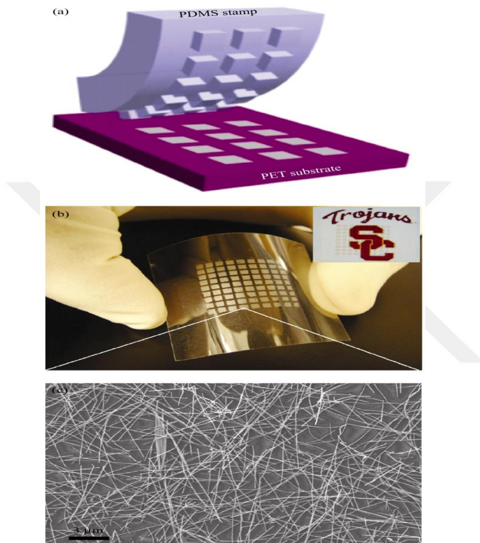
Figure 3.24 Patterned transfer of Ag NW film. (a) Schematic diagram of the patterned PDMS stamp in contact with the nanowire film. (b) Photograph of patterned nanowire film transferred to the PET substrate. The size of each pixel is 1 mm \times 1 mm. (c) SEM image showing the nanowire network in one pixel [73].
