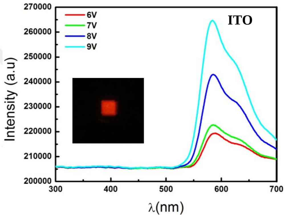
Figure 4.10 Electroluminescence characteristics of PLED device with ITO anode [76]. Inset shows a photo of emission.
