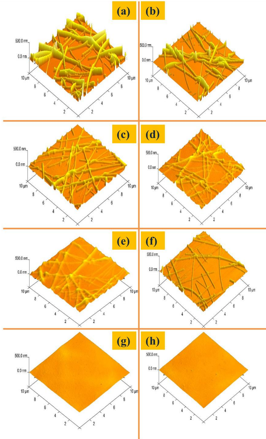
Figure 4.5 AFM 3D images of Ag NW networks that are (a) as deposited, (b) pressed during annealing, (c) PEDOT:PSS/IPA spin coated at 2500 rpm, (d) 1500 rpm (e) 1000 rpm, (f) PEDOT:PSS spin coated at 2500 rpm, (g) 1500 rpm, (h) 1000 rpm, respectively [76].
