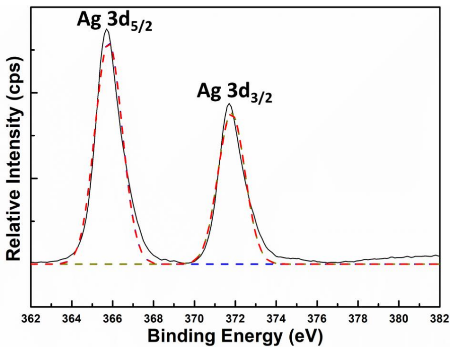
Figure 5.15 High-resolution XPS spectrum of Ag 3d.
