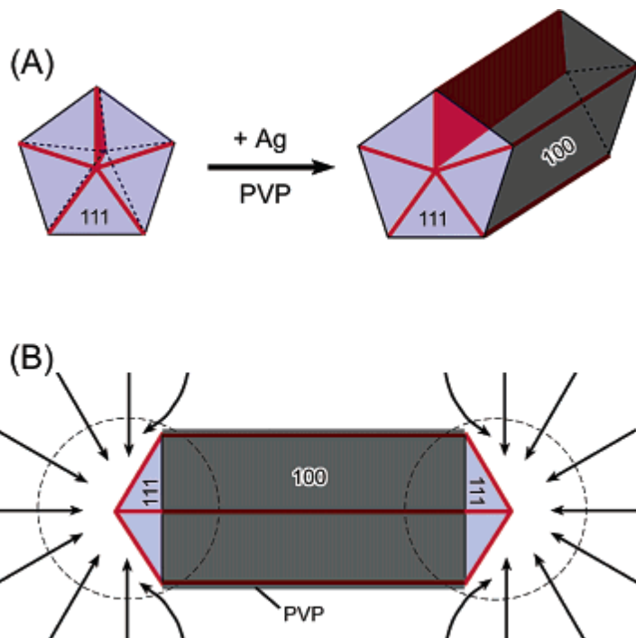
Figure 2.8 Schematic illustration of the mechanism proposed to account for the growth of silver nanowires with pentagonal cross sections: (a) Evolution of a nanorod from a MTP of silver under the confinement of five twin planes and with the assistance of PVP. The ends of this nanorod are terminated by \{111\} facets, and the side surfaces are bounded by \{100\} facets. The strong interaction between PVP and the \{100\} facets is indicated with a dark-gray color, and the weak interaction with the \{111\} facets is marked by a light-blue color. The red lines on the end surfaces represent the twin boundaries that can serve as active sites for the addition of silver atoms. The plane marked in red shows one of the five twin planes that can serve as the internal confinement for the evolution of nanorods from MTP. (B) Schematic model illustrating the diffusion of silver atoms toward the two ends of a nanorod, with the side surfaces completely passivated by PVP. This drawing shows a projection perpendicular to one of the five side facets of a nanorod, and the arrows represent the diffusion fluxes of silver atoms [42].
