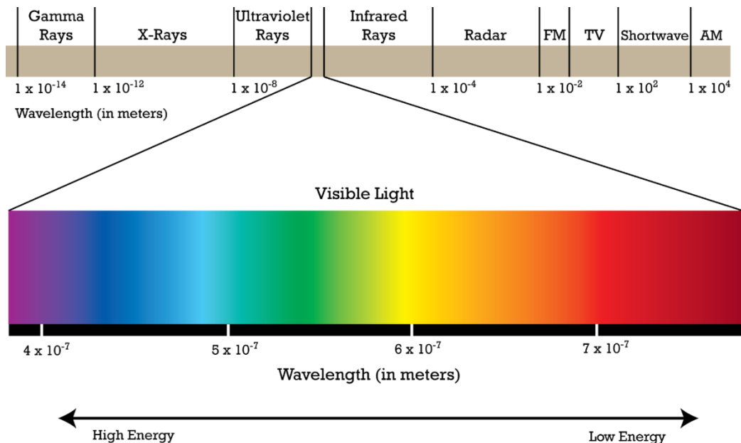
Figure 3.3 Electromagnetic spectrum of light [52].
