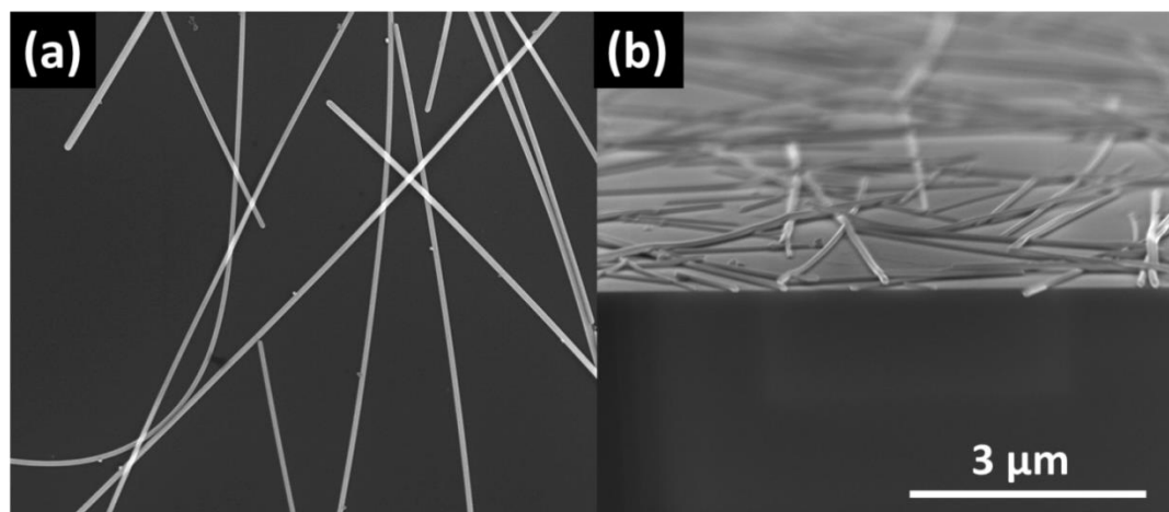
Figure 4.3 Top and cross-sectional SEM images of Ag NW networks on Si wafer. Both scales are the same [76].
