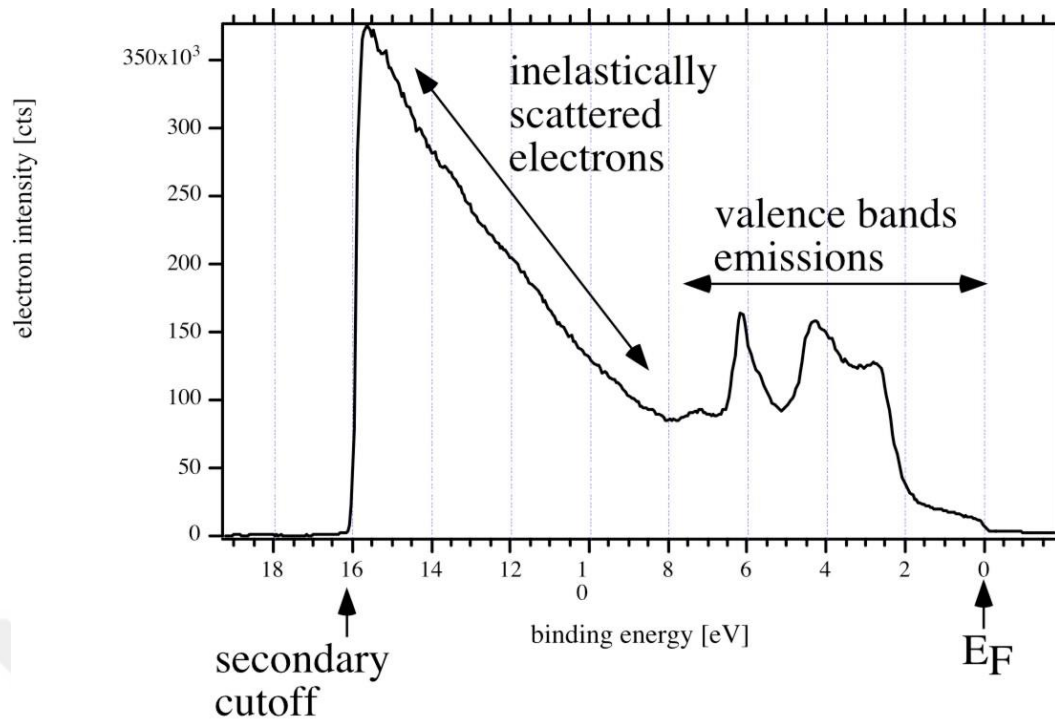
Figure 3.7 UP-spectrum of Au surface [53].
