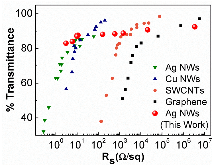
Figure 3.38 Sheet resistance versus transmittance of annealed Ag NW networks in comparison to various transparent electrodes reported in literature, modified from Ref. 77.
