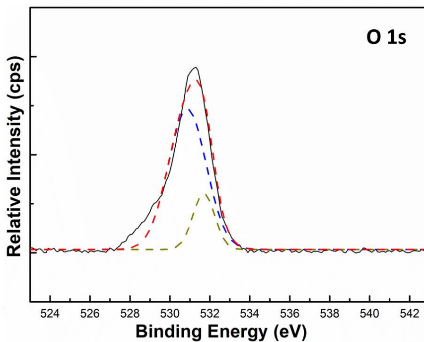
Figure 5.17 High resolution XPS spectrum of O 1s.
