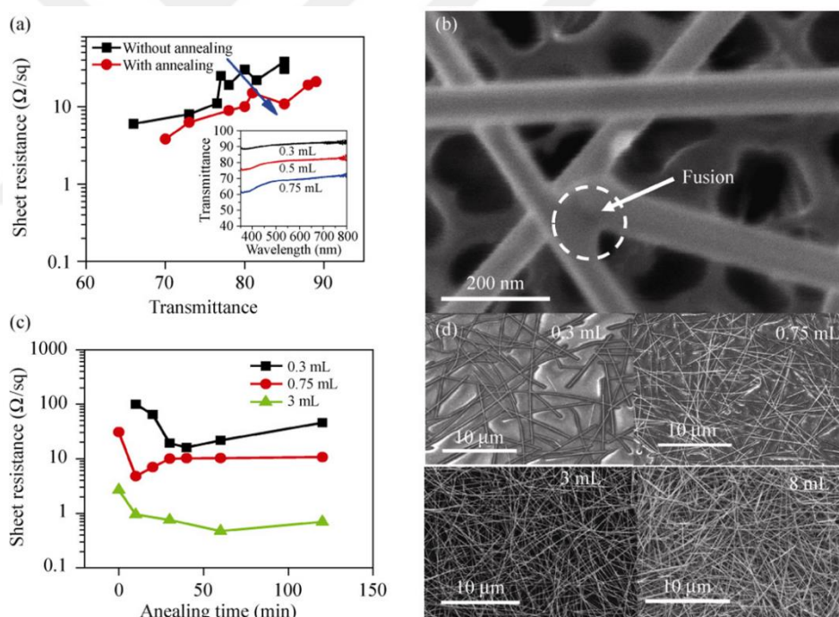
Figure 3.25 (a) Plot of sheet resistance versus transmittance at a wavelength of 550 nm of Ag NW networks. Black dots represent resistance values for films without annealing and red dots represent resistance values after annealing the film samples at 200 °C for 20 min in air. Inset shows the transmittance spectra of nanowire networks with different thicknesses. (b) SEM image of an annealed nanowire sample showing melting of nanowires at the ends and subsequent joining with neighboring nanowires.
