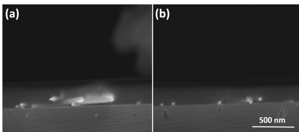
Figure 6.10 Cross-sectional SEM images of NiO coated Ag NWs from 2 different spots.
