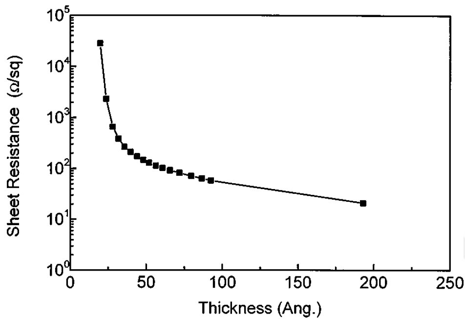
Figure 3.11 Sheet resistance vs. thickness graph for Pt films [61].
