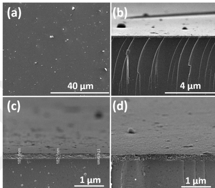
Figure 6.7 (a) Top-view, (b) – (d) cross-sectional SEM images of NiO thin films on silicon substrates [99].
