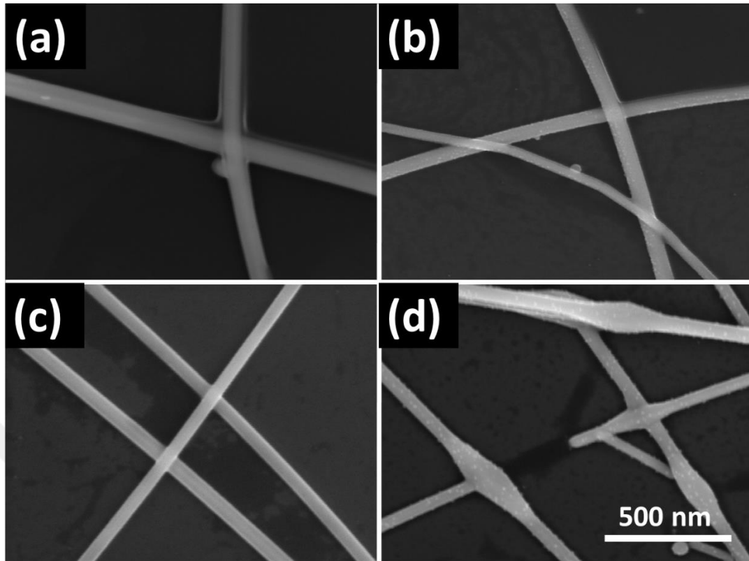
Figure 3.35 SEM images of (a) as deposited, (b) 100, (c) 200, (d) 300°C annealed Ag NE networks (30 minutes) [76]. All scales are the same.
