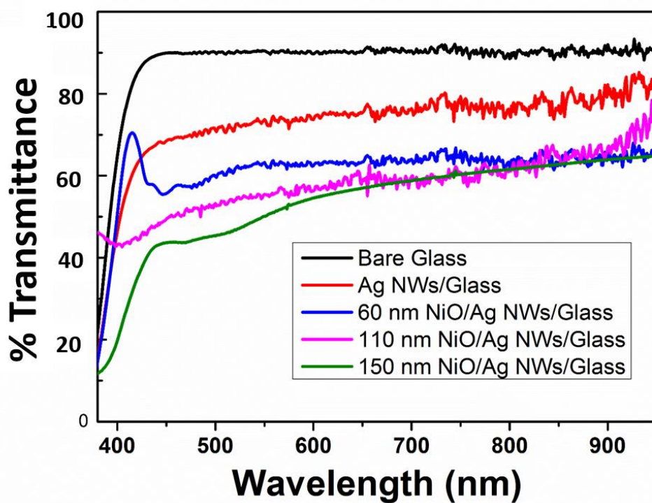
Figure 6.16 Percent transmittance of NiO / Ag NW nano composites.
