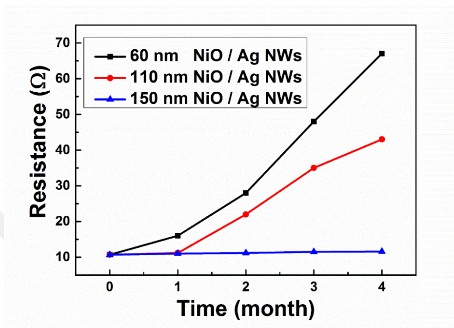
Figure 6.15 Change in sheet resistance for NiO / Ag NW nano composites with time.
