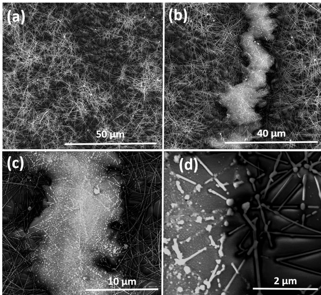
Figure 5.20 SEM images of failed Ag NW networks under high current.
