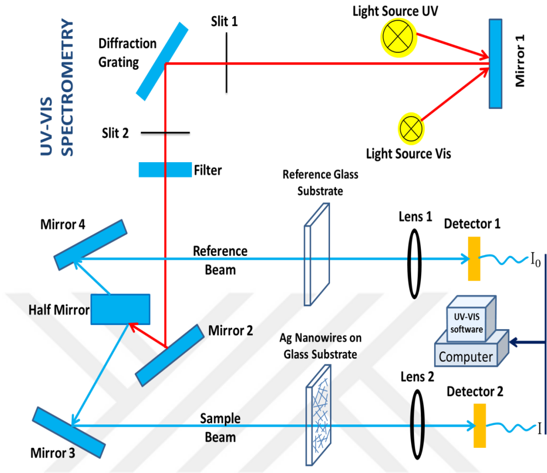
Figure 3. 29 UV-VIS spectroscopy set-up for transparency measurements of Ag NW networks [48].
