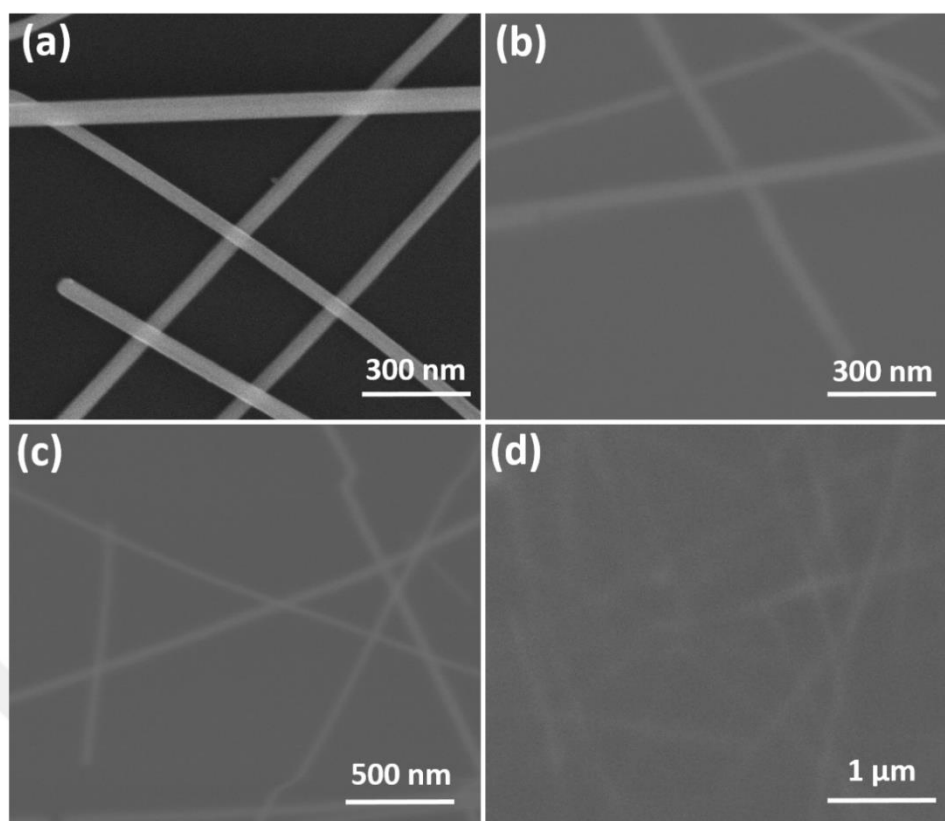
Figure 6.9 Top-view SEM images of (a) bare Ag NWs networks, (b) 5, (c) 10 and (d) 15 times spin coated NiO thin films.
