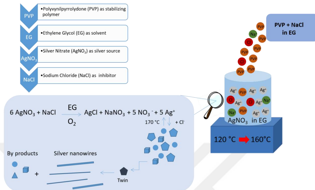
Figure 2.11 Schematic representation for the formation of Ag NWs in modified polyol process.
