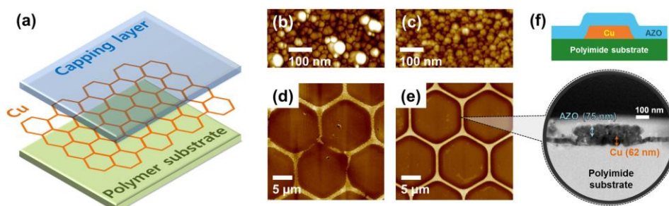
Figure 3. 17 (a) Structure of the Cu mesh hybrid electrode. (b) and (c) AFM topography images of Cu thin films on polyimide substrates fabricated using a polycrystalline Cu target and a single-crystal Cu target, respectively. (d) and (e)
