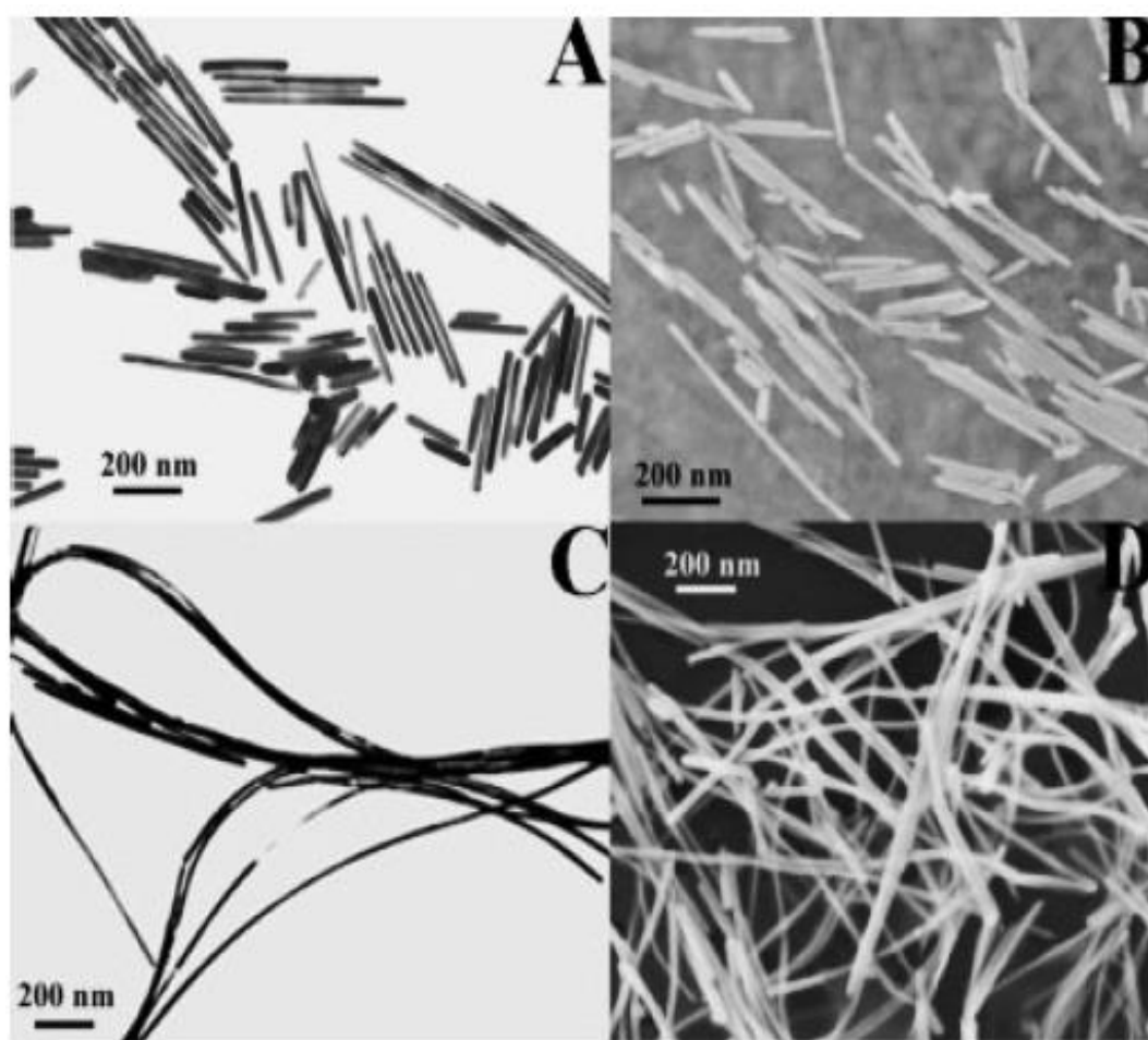
Figure 2.6 TEM and SEM images of silver nanorods and nanowires prepared using a,b) 0.8 mM \text{Na}_3\text{C}_6\text{H}_5\text{O}_7 and c,d) 1.2 mM \text{Na}_3\text{C}_6\text{H}_5\text{O}_7 [41].
