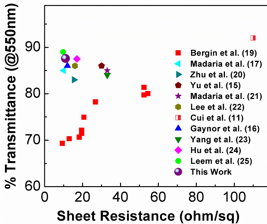
Figure 3.39 A literature comparison showing lowest sheet resistances versus transmittance at 550 nm of Ag NW networks reported by other groups [76].
