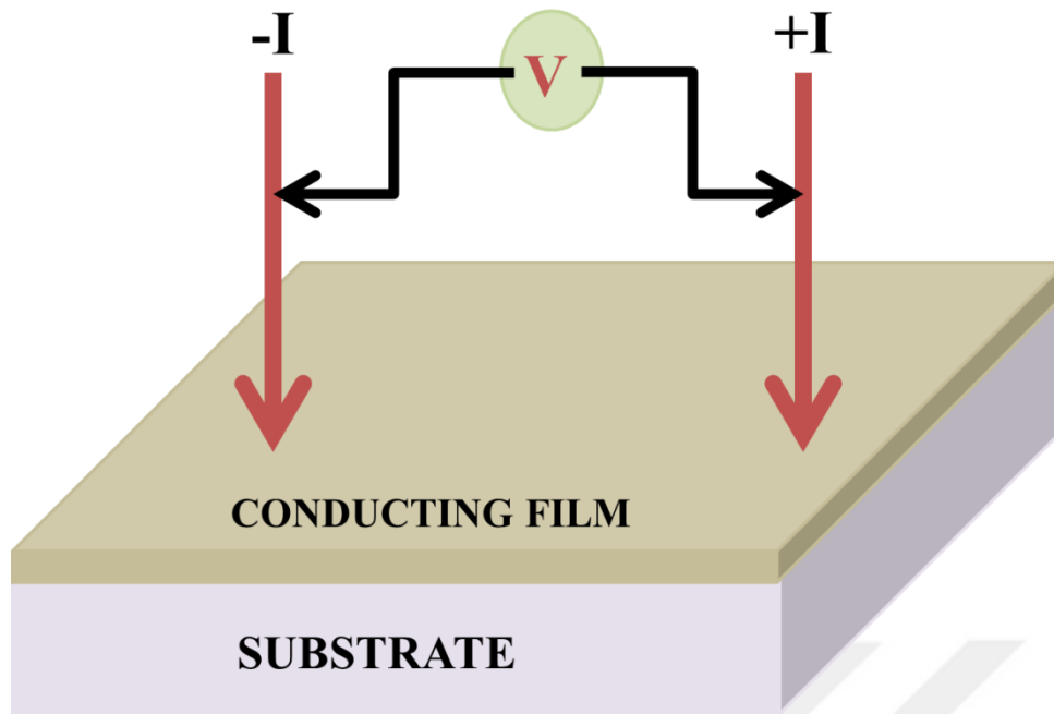
Figure 3.4 Representative set-up for 2-probe measurements [48].
