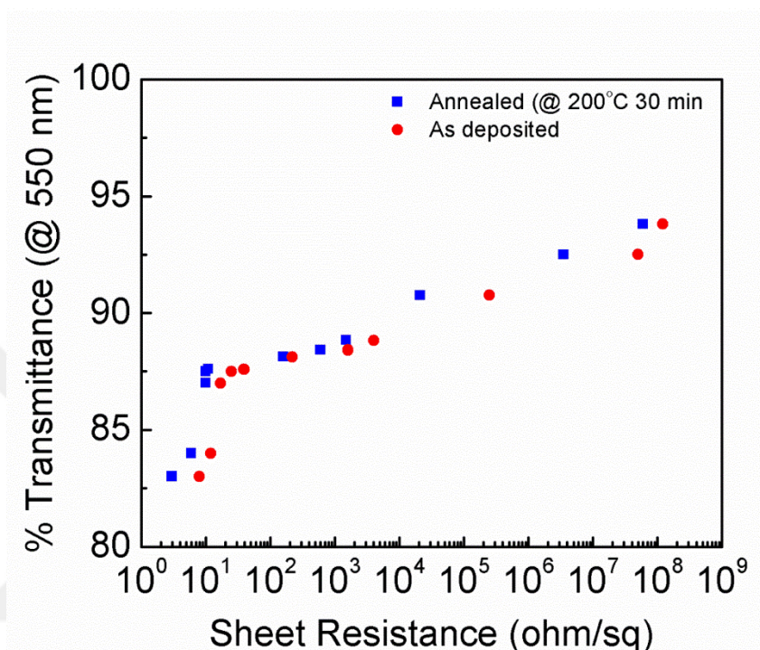
Figure 3.37 Sheet resistance versus transparency of as deposited and annealed (200 °C for 20 min.) Ag NWs networks [76].
