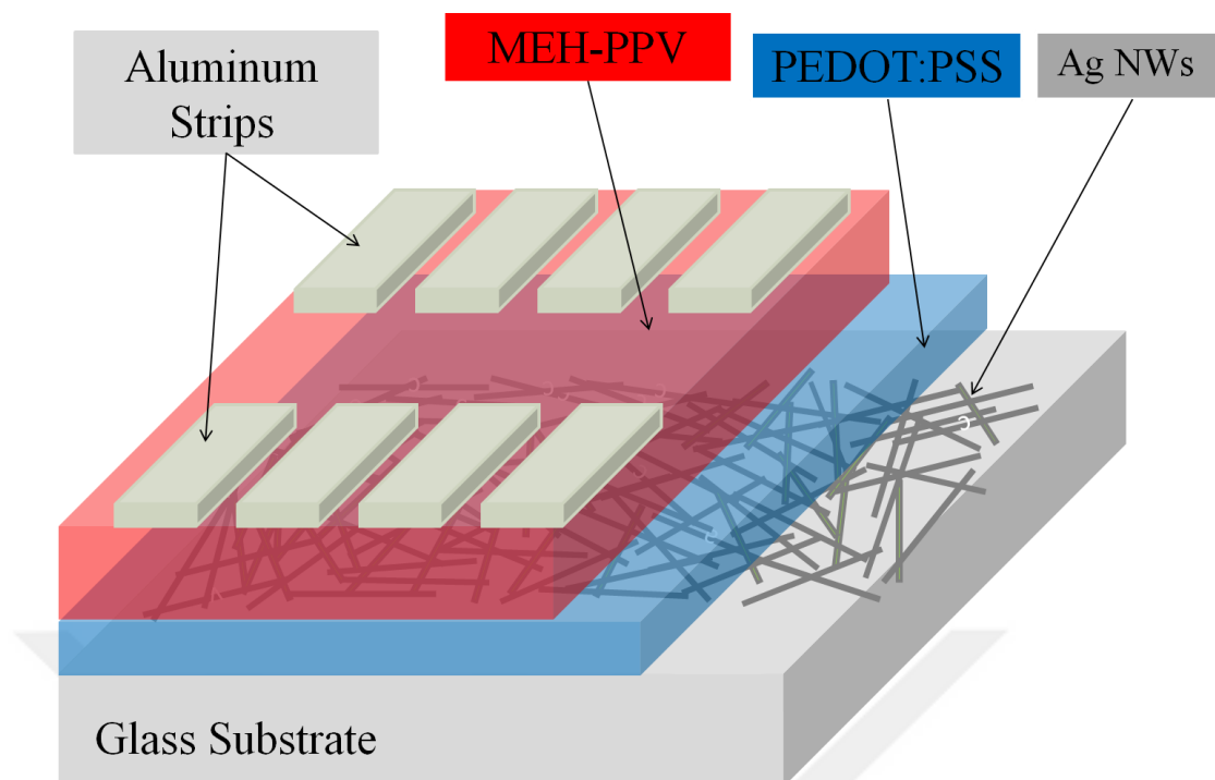
Figure 4.7 Schematic structure of PLED in which Ag NW networks were used as anode.
