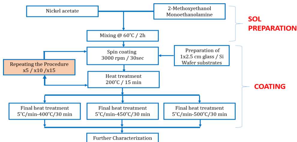
Figure 6.5 Flowchart showing sol preparation and spin coating procedure of NiO thin films [99].
