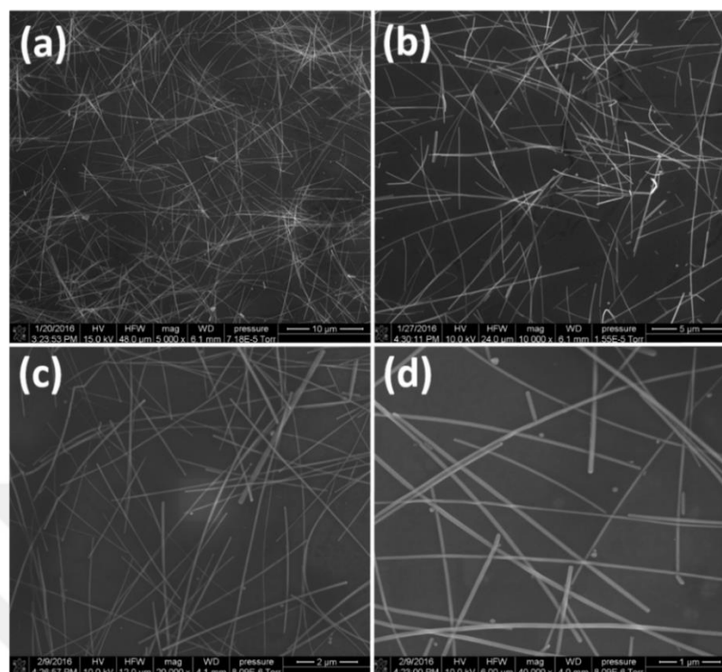
Figure 6.4 (a) – (d) SEM images of silver nanowire based transparent conductors.
