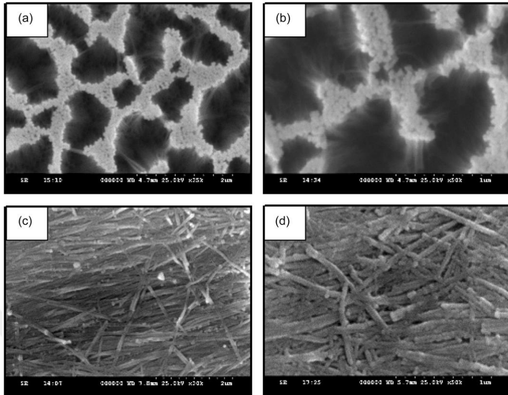
Figure 2.3 Top view SEM image of Ag NW arrays grown on the surface of AAO membrane: (a) low magnification image, (b) high magnification image, SEM image of (c) and (d) silver nanowires after eliminating the AAO membrane in a NaOH solution [33].
