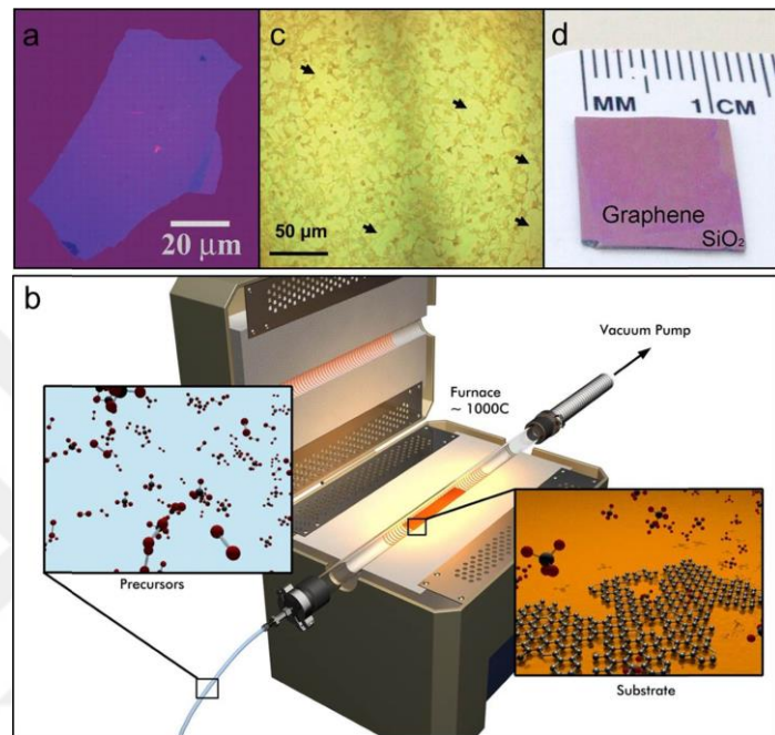
Figure 3.10 (a) An optical image of mechanically exfoliated graphene flake [59]. (b) Schematic illustration of graphene synthesis by CVD method. (c) Graphene synthesized on nickel thin film; arrows indicate thin monolayer regions. (d) Monolayer graphene synthesized on copper foil and transferred onto a SiO 2 /Si substrate [60].
