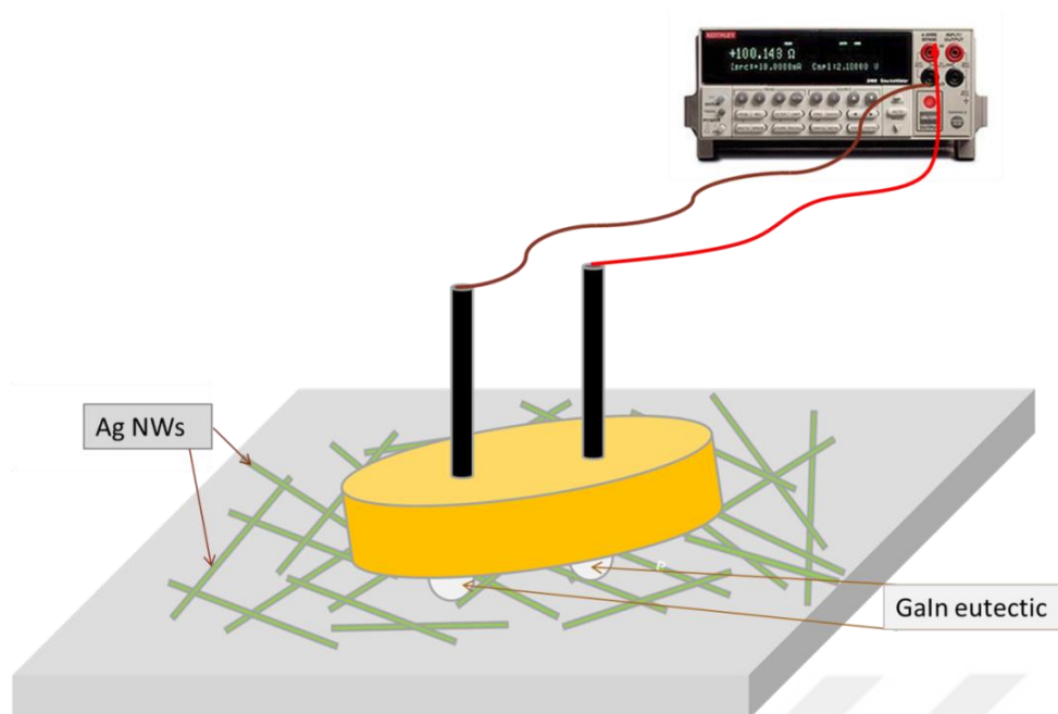
Figure 3.28 Schematic of the two probe measurement set-up used for obtaining the sheet resistance values of Ag NW networks [48].
