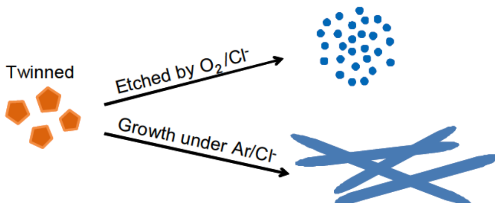
Figure 2.9 Illustration of the proposed mechanism by which twinned decahedron was etched with the existence of \text{O}_2/\text{Cl}^- and Ag NWs were obtained under argon protection [45].
