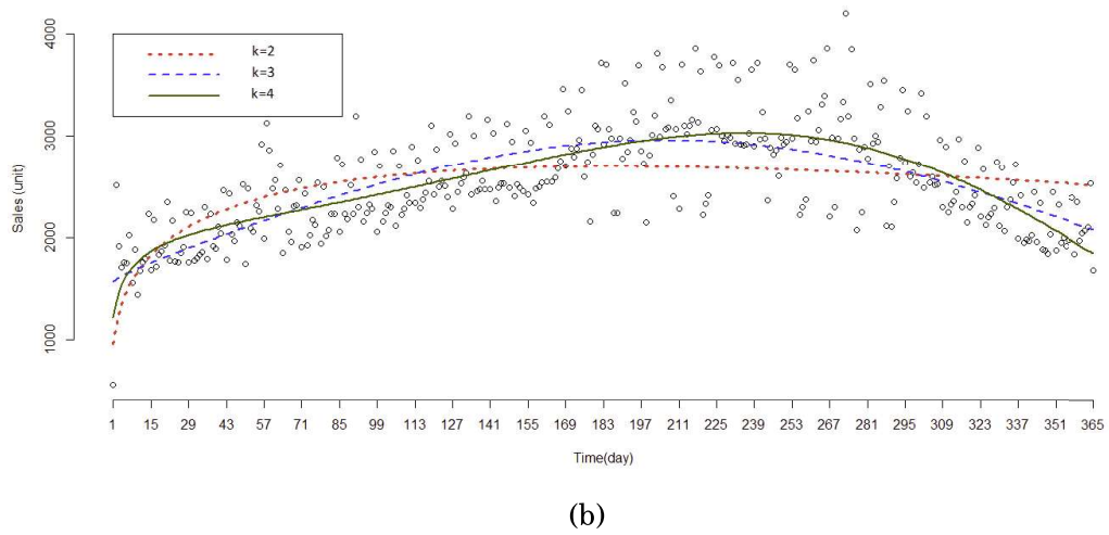
Figure 4.9: The multiplicative models fitted over average daily sales data of product A (a) and product B (b)
