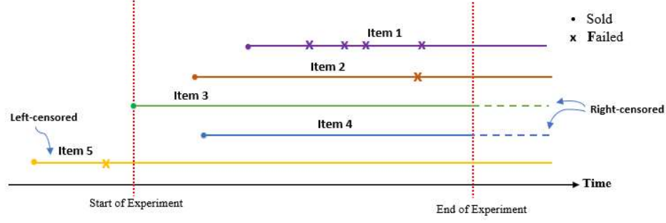
Figure 2.1: Censoring within the failure times data
