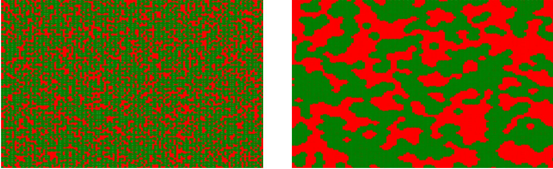
Figure 2.5: Initial (left) and equilibrium (right) networks for 120x120 square lattice with periodic boundary conditions and Moore Neighborhood. Red colors are X agents and green colors are Y agents. w=1 .
