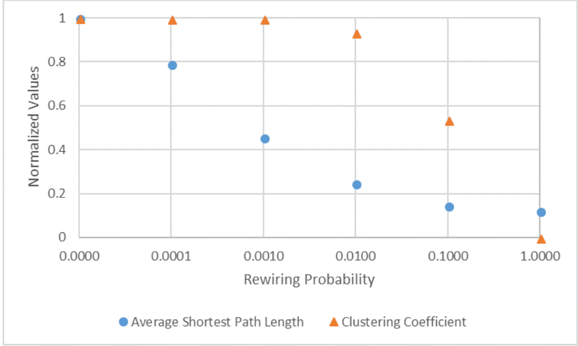
Figure 3.2: Clustering coefficient and average shortest path length values for different rewiring probabilities. Initial network is 120x120 regular square lattice with periodic boundary conditions and Moore Neighborhood, w=1 .
