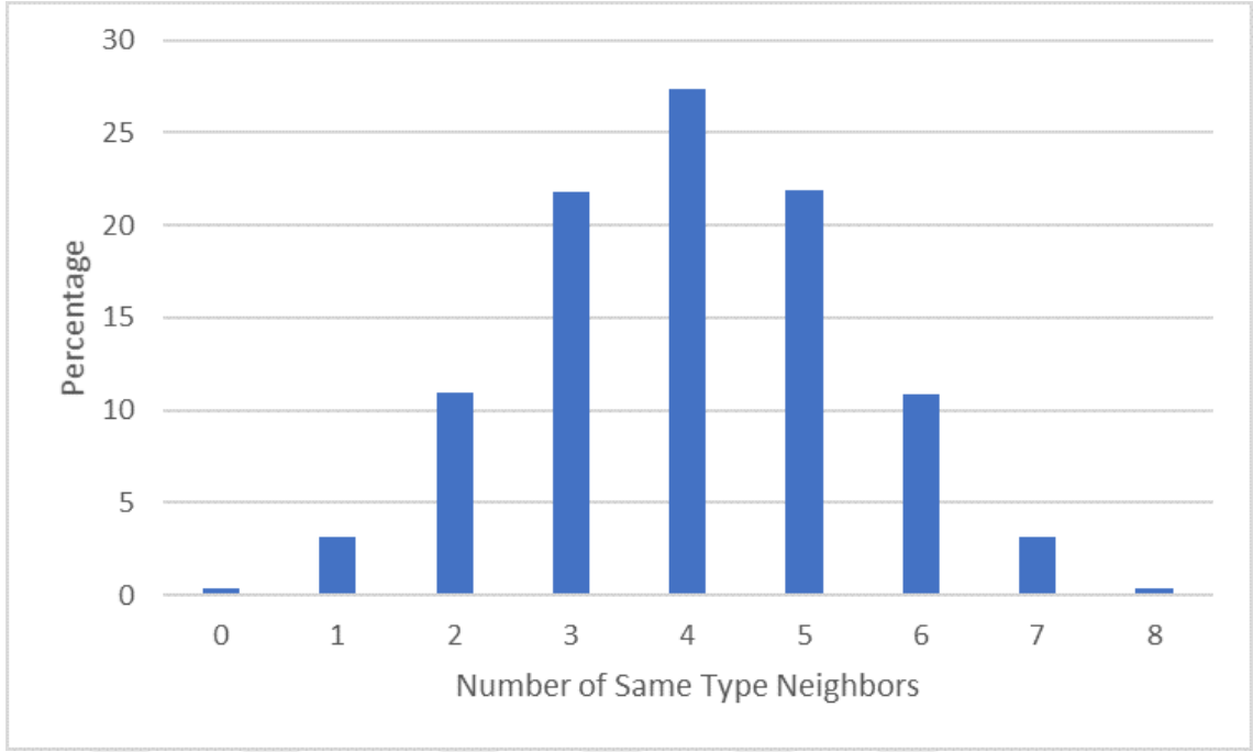
Figure 2.4: Same type neighbor distribution of agents in the initial network. Same type neighbors are X agents in the neighbors for an agent X and Y agents in the neighbors for an agent Y. Network is 120x120 square lattice. Periodic boundary conditions and Moore neighborhood are employed. w=1 . Distributions obtained from 500 runs.
