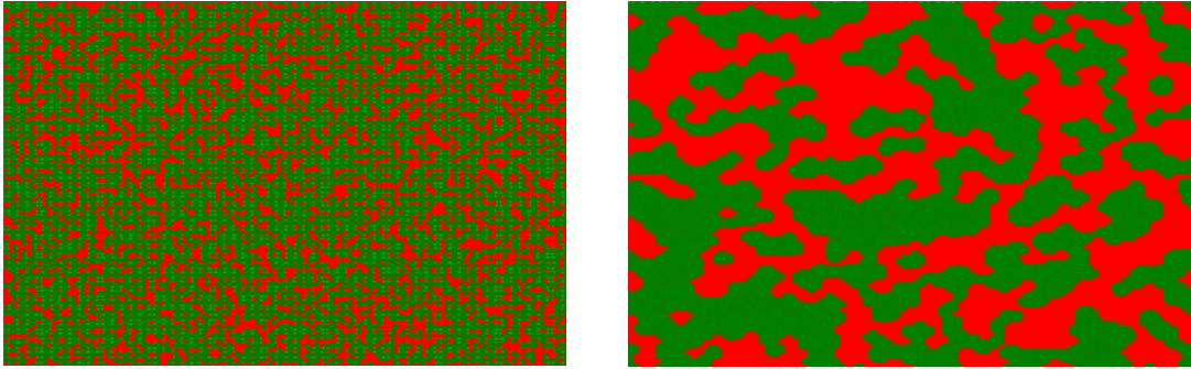
Figure C.3: Third example of initial and equilibrium networks. Network is 120 \times 120 square lattice with periodic boundary conditions and Moore neighborhood. w=1 . Figure on the left is the initial network and figure on the right is the equilibrium network.
