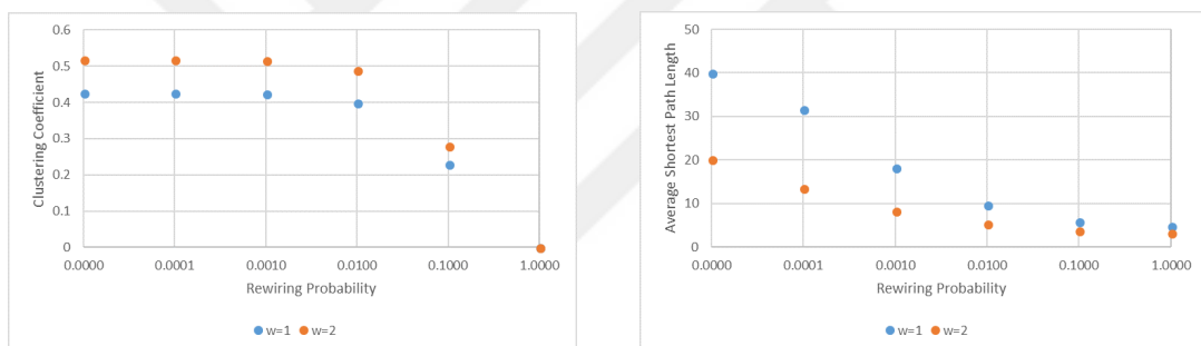
Figure D.1: Figure on the left shows clustering coefficient values and figure on the right shows average shortest path length for different rewiring probabilities. Initial network is 120x120 square lattice with periodic boundary conditions and Moore neighborhood.
