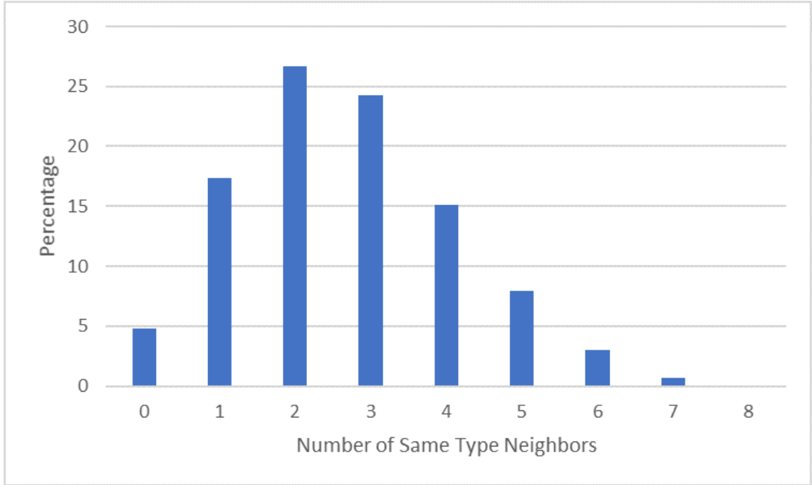
Figure 4.2: Same type neighbor distribution of XY agents in the initial network. Same type neighbors are XY agents in the neighbors for an agent XY. Network is 120x120 square lattice. Periodic boundary conditions and Moore neighborhood are employed. w=1 . Distributions obtained from 500 runs.
