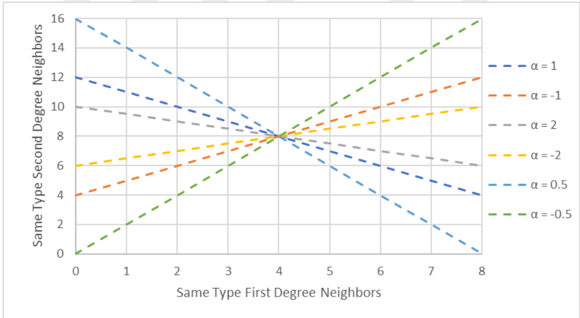
Figure 5.1: Inequalities show the numbers of same type first degree and second degree neighbors agents need to satisfy their utility functions for different \alpha values.
