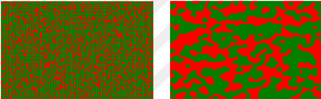
Figure C.1: First example of initial and equilibrium networks. Network is 120x120 square lattice with periodic boundary conditions and Moore neighborhood. w=1 . Figure on the left is the initial network and figure on the right is the equilibrium network.
