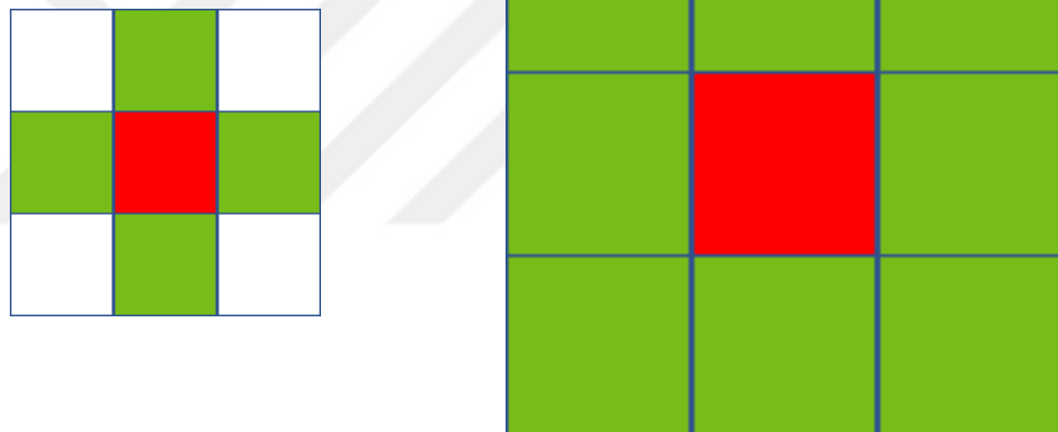
Figure B.1: Differences between these two neighborhoods are demonstrated in 3x3 part of a square lattice. Green nodes are the neighbors of the red nodes. Figure on the left demonstrates Von Neumann Neighborhood and figure on the right demonstrates Moore Neighborhood.
