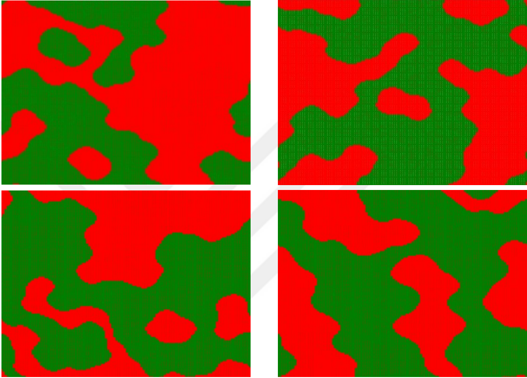
Figure 5.2: Equilibrium networks for the positive values of \alpha . Networks are 120x120 square lattices with periodic boundary conditions and Moore neighborhood. Figure on the top left is for \alpha = 0.125 , figure on the top right is for \alpha = 0.5 , figure on the bottom left is for \alpha = 1 and figure on the bottom right is for \alpha = 2 .
