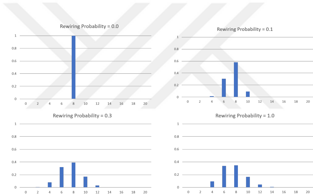
Figure E.1: Degree distributions for different rewiring probabilities. Initial network is 120x120 square lattice with periodic boundary conditions and Moore neighborhood. w=1 .
