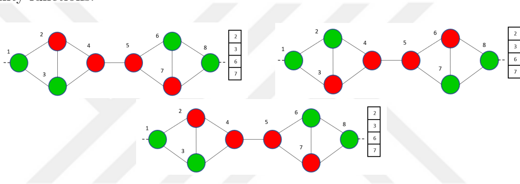
Figure 2.1: Network consists of 8 nodes and each node has 3 neighbors. Periodic boundary conditions and synchronous change are employed. Figure on the top left is the initial network, figure on the top right is the network after the first iteration and the bottom figure is the network after the second iteration. Array shows the unhappy list.
