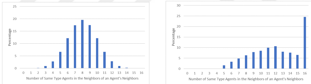
Figure 2.8: Initial (left) and Equilibrium (right) network distributions of neighbors of an agent's neighbors. 120x120 square lattice with periodic boundary conditions and Moore neighborhood is employed. w=1 . Distributions obtained from 500 runs.
