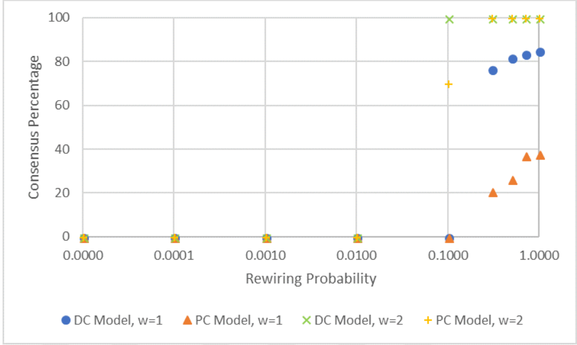
Figure 4.4: Percentage of communities that reach a consensus for DC and PC models and for different neighborhood ranges. Initial network is 120x120 regular square lattice with periodic boundary conditions. All networks are connected.
