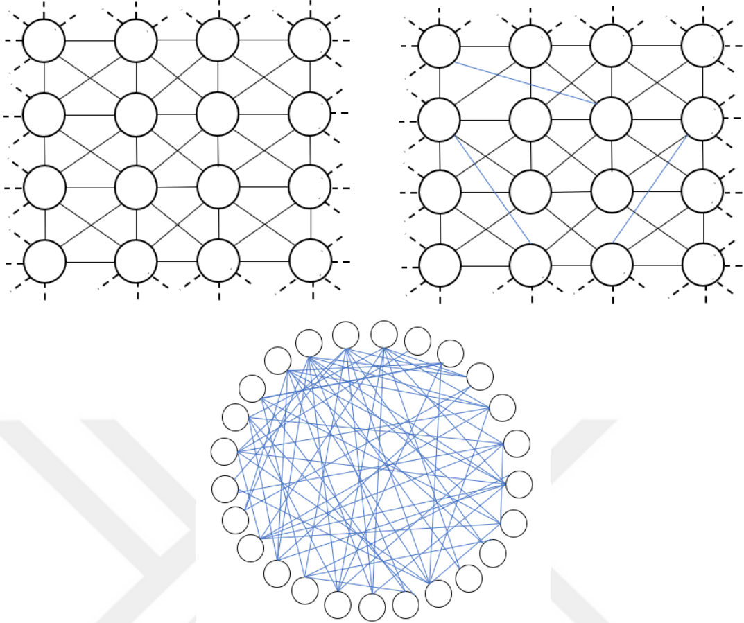
Figure 3.1: Figure on the left displays regular square lattice ( p = 0 ) with periodic boundary conditions and Moore neighborhood ( w=1 ) where the degrees of all nodes are equal. Dotted lines represent periodic boundaries. Figure on the right shows the small-world network where some links (blue) from square lattice are broken and rewired to nodes that are randomly chosen. Number of links is preserved. Clustering coefficient is still high as regular square lattice but the average shortest path length is decreased. Figure on the bottom displays random network ( p = 1 ) where all edges are rewired.
