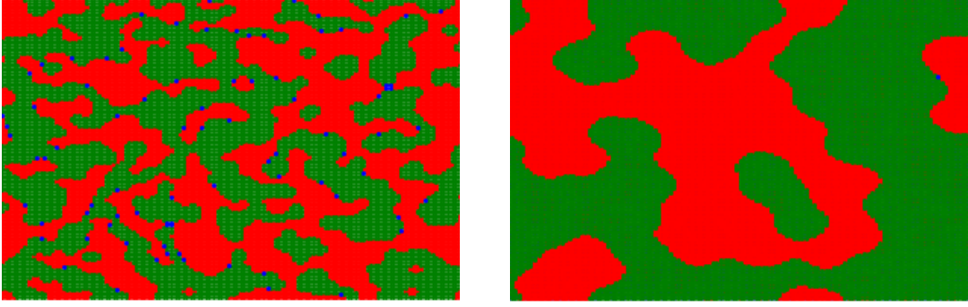
Figure 4.3: PC model on 120x120 square lattice with periodic boundary conditions and Moore neighborhood. Figure on the left shows w=1 and figure on the right shows w=2 . Red colors are X agents, green colors are Y agents and blue colors are XY agents.
