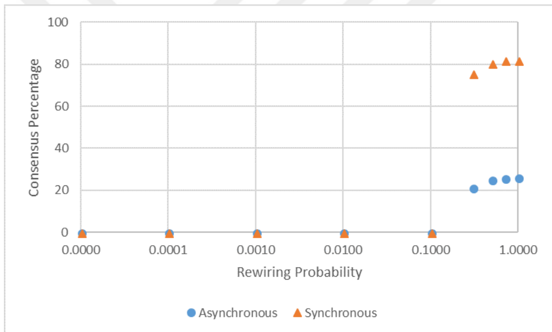
Figure 3.3: Percentage of communities that reach a consensus for synchronous and asynchronous change. Initial network is 120x120 regular square lattice with periodic boundary conditions and Moore neighborhood. w=1 . All networks are connected.
