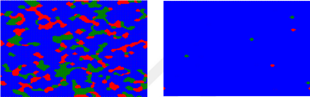
Figure 4.5: DC models with persistence step. Network is 120x120 square lattice with periodic boundary conditions and Moore neighborhood. w=1 . Figure on the left shows the equilibrium network for persistence step 1, and figure on the right shows the equilibrium network when persistence step is equal to the number of iterations until equilibrium.
