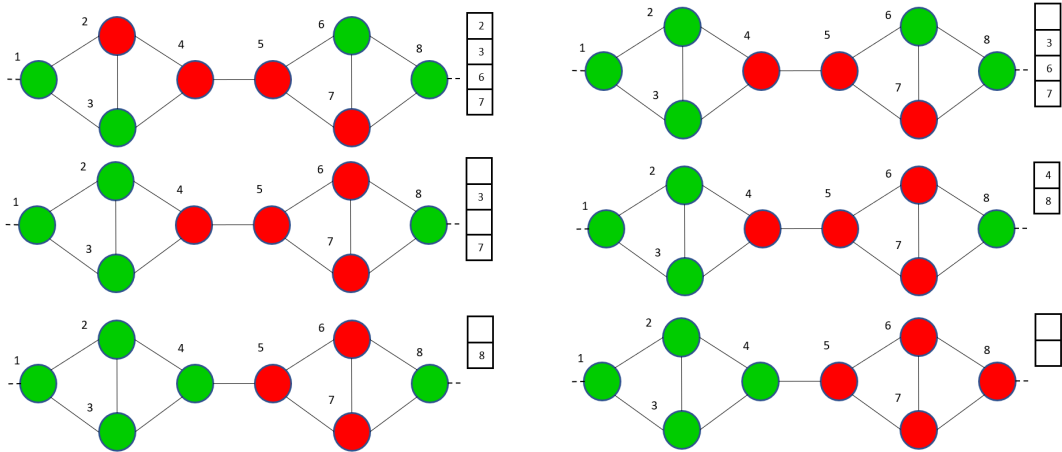
Figure 2.2: Network consists of 8 nodes and each node has 3 neighbors. Periodic boundary conditions and asynchronous change are employed. Figure on the top left is the initial network and figure on the top right is the network after agent 2 changes its type. Figure on the bottom right is the equilibrium network. Array shows the unhappy list.
