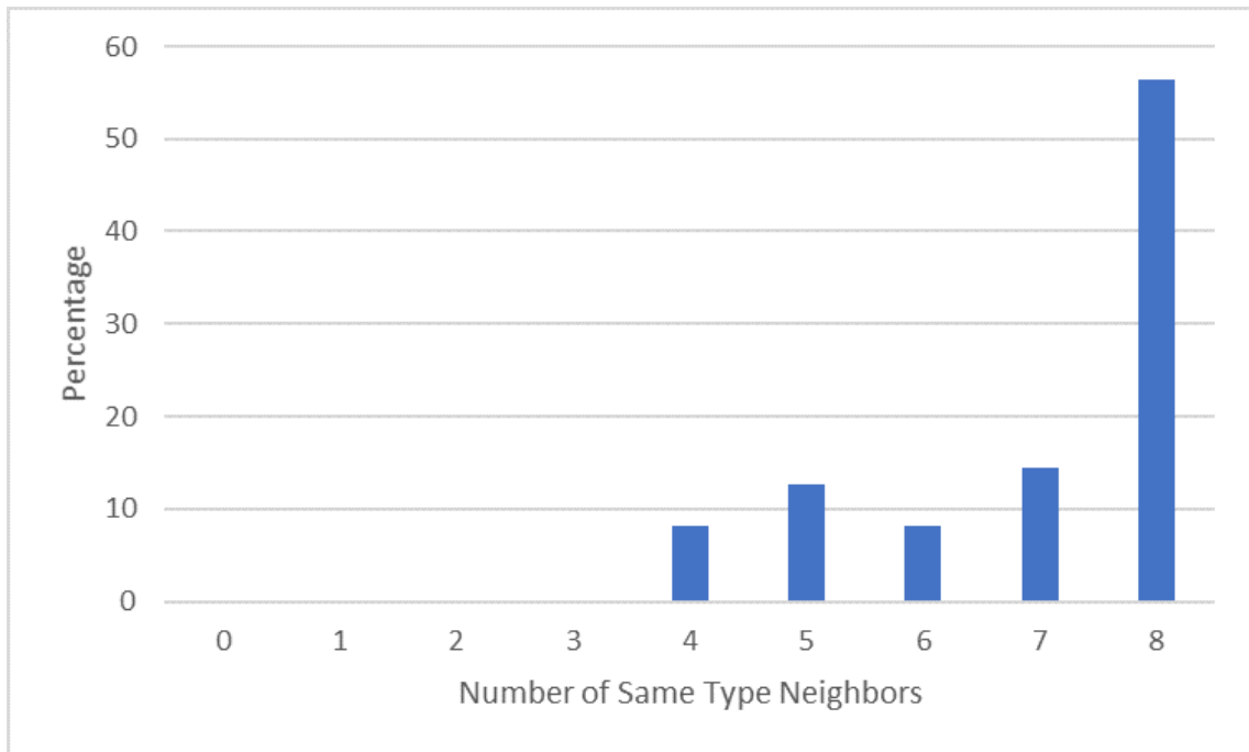
Figure 2.6: Same type neighbor distribution of agents in the equilibrium network. Same type neighbors are X agents in the neighbors for an agent X and Y agents in the neighbors for an agent Y. Network is 120x120 square lattice. Periodic boundary conditions and Moore neighborhood are employed. w=1 . Distributions obtained from 500 runs.
