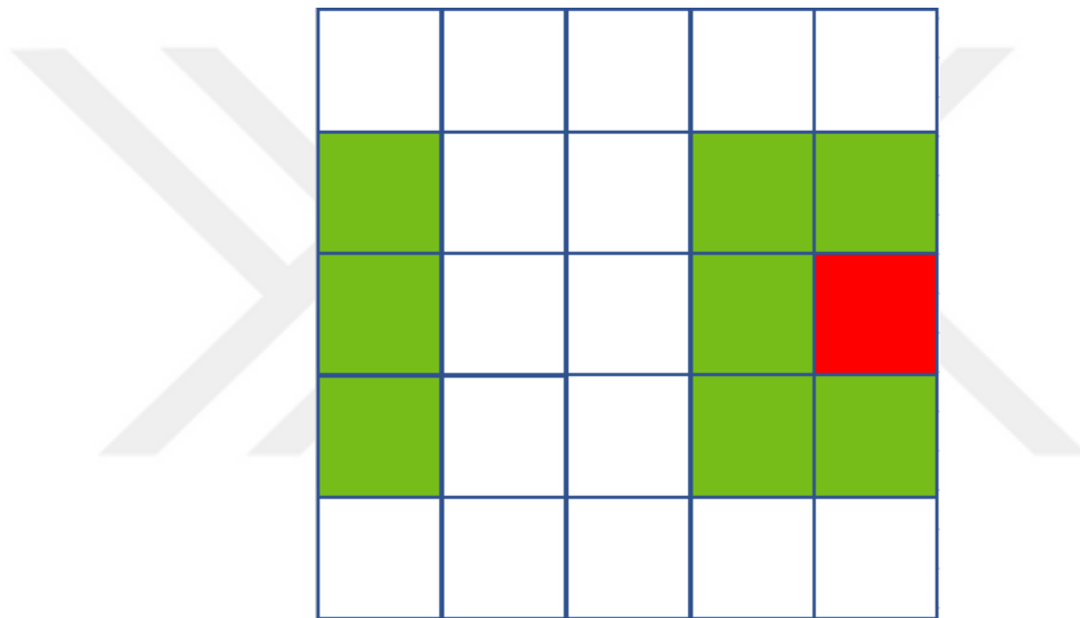
Figure A.1: Representation of periodic boundary conditions on a 5x5 square lattice. Green nodes are the neighbors of the red node.
