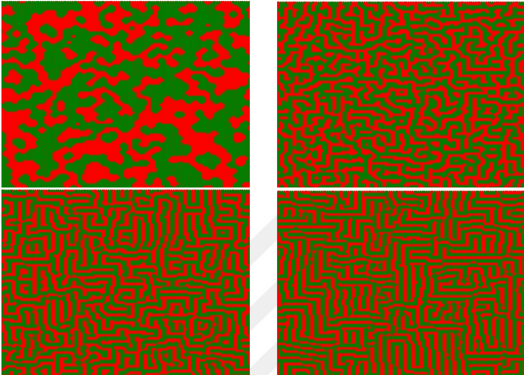
Figure 5.3: Equilibrium networks for the negative values of \alpha . Networks are 120x120 square lattices with periodic boundary conditions and Moore neighborhood. Figure on the top left is for \alpha = -0.125 , figure on the top right is for \alpha = -0.5 , figure on the bottom left is for \alpha = -1 and figure on the bottom right is for \alpha = -2 .
