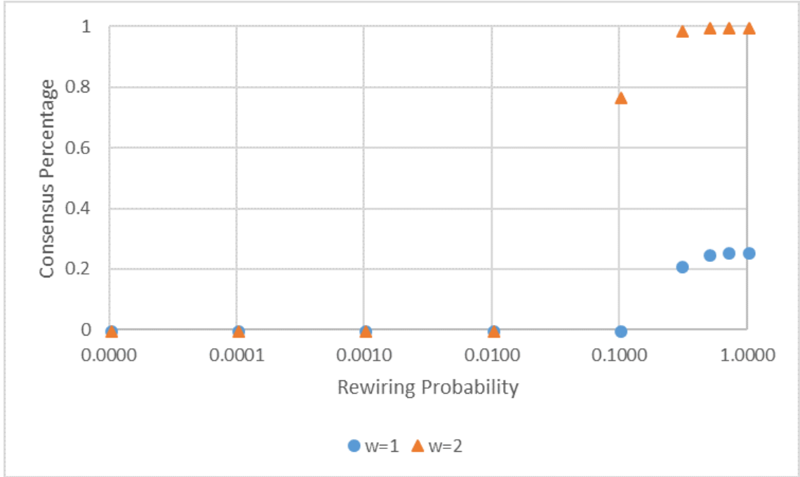
Figure 3.4: Percentage of communities that reach a consensus for w=1 and w=2 . Initial network is 120 \times 120 square lattice with periodic boundary conditions and asynchronous change.
