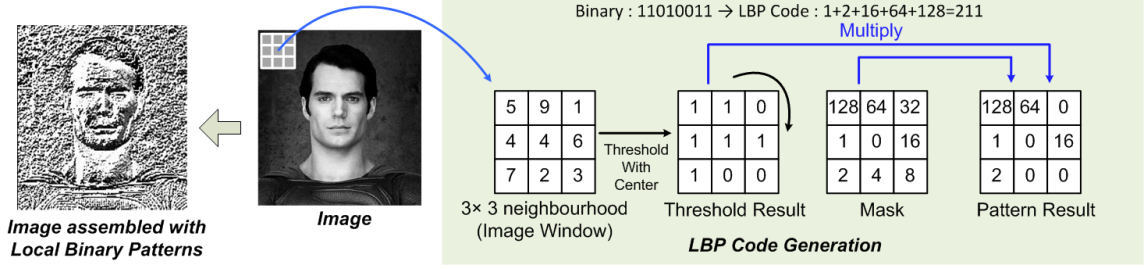
FIGURE 4.2: Local Binary Patterns (LBP) feature extraction process [13]
