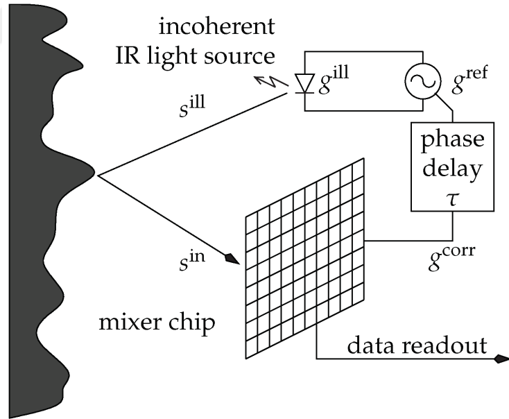
FIGURE 3.7: The time of flight (ToF) phase-measurement principle [9]
