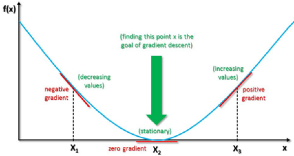
FIGURE 4.9: Illustration of gradient descent algorithm [17]
