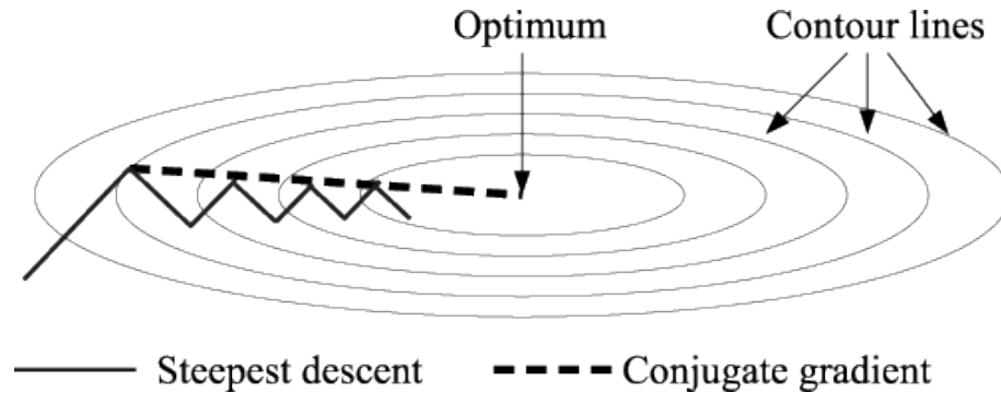
FIGURE 4.10: Search paths of the steepest descent and the conjugate gradient methods on a 2D plane [18]
