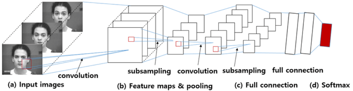
FIGURE 2.7: Block diagram for a CNN based FER approach (face images are taken from CK+ dataset [4])
