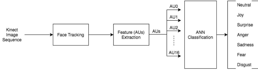
FIGURE 4.12: Schematic representation of the methodology
