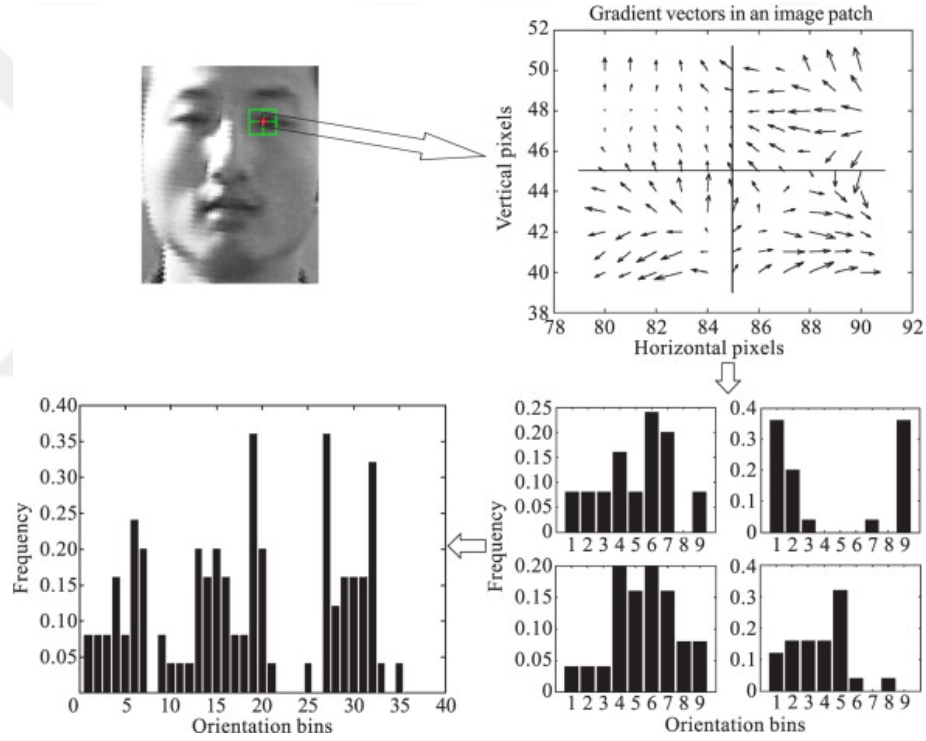
FIGURE 4.3: Histogram Oriented Gradient feature extraction stages[14]
