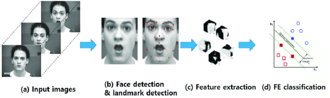
FIGURE 2.6: Block diagram for conventional FER approaches [5] (face images are taken from CK+ dataset [4])
