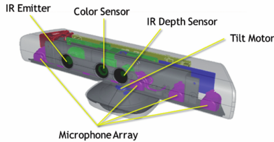
FIGURE 3.5: Construction of structured-light Kinect [10]
