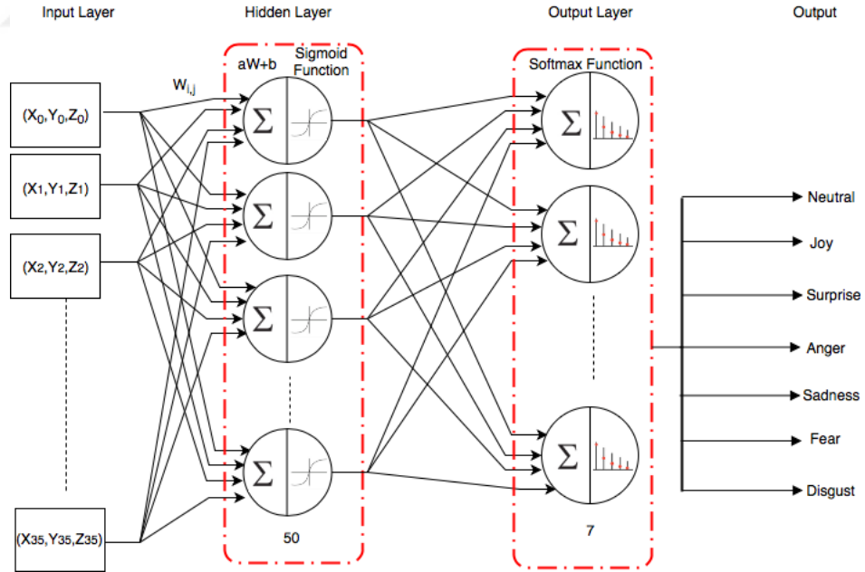
FIGURE 4.14: Architecture of the second neural network classifier
