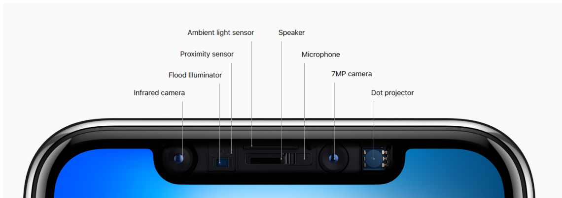
FIGURE 3.6: The components of Apple's TrueDepth camera [11]
