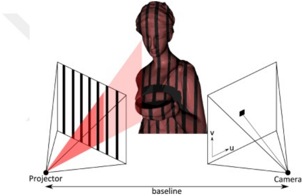
FIGURE 3.4: Structured light approach [9]
