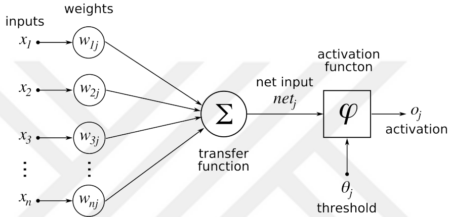
FIGURE 4.7: Simple neural network model [16])
