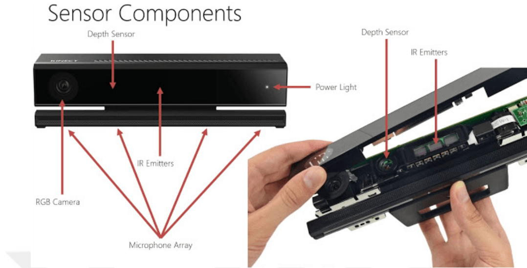
FIGURE 3.9: Sensor components of Kinect v2
