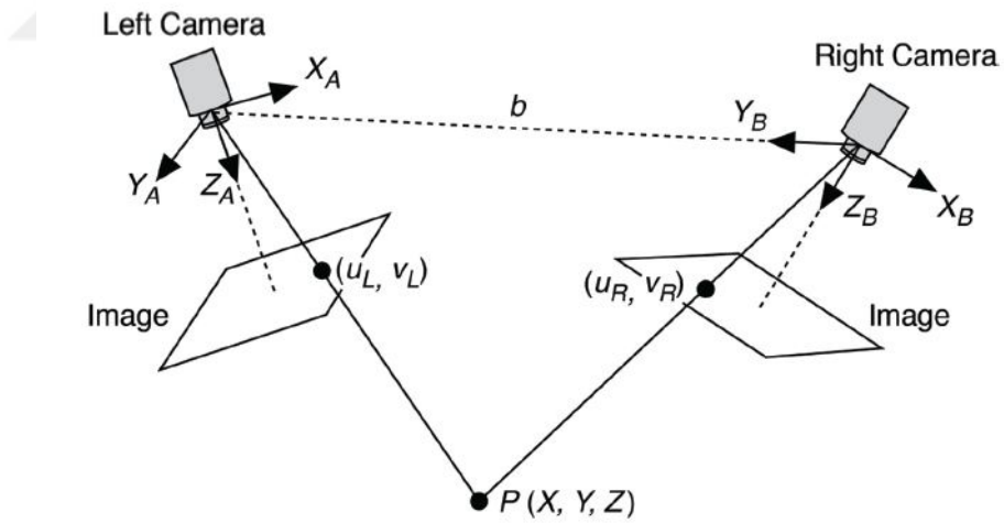
FIGURE 3.3: Stereo vision model [8]
