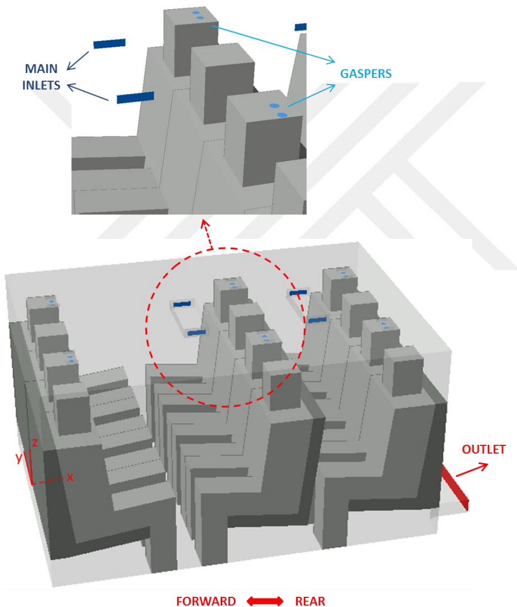
Figure 5-1 Simplified model of the investigated helicopter cabin
