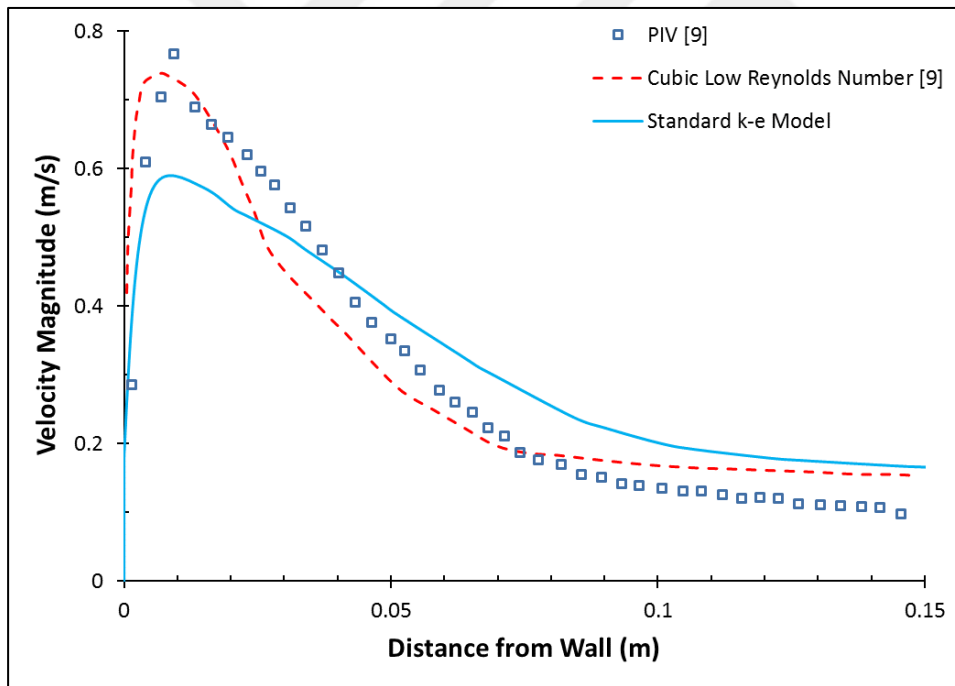
Figure 4-17 Velocity magnitude comparison on Line A – Standard k- \epsilon turbulence model with Günther et al.'s [9] experimental data and the best numerical result
