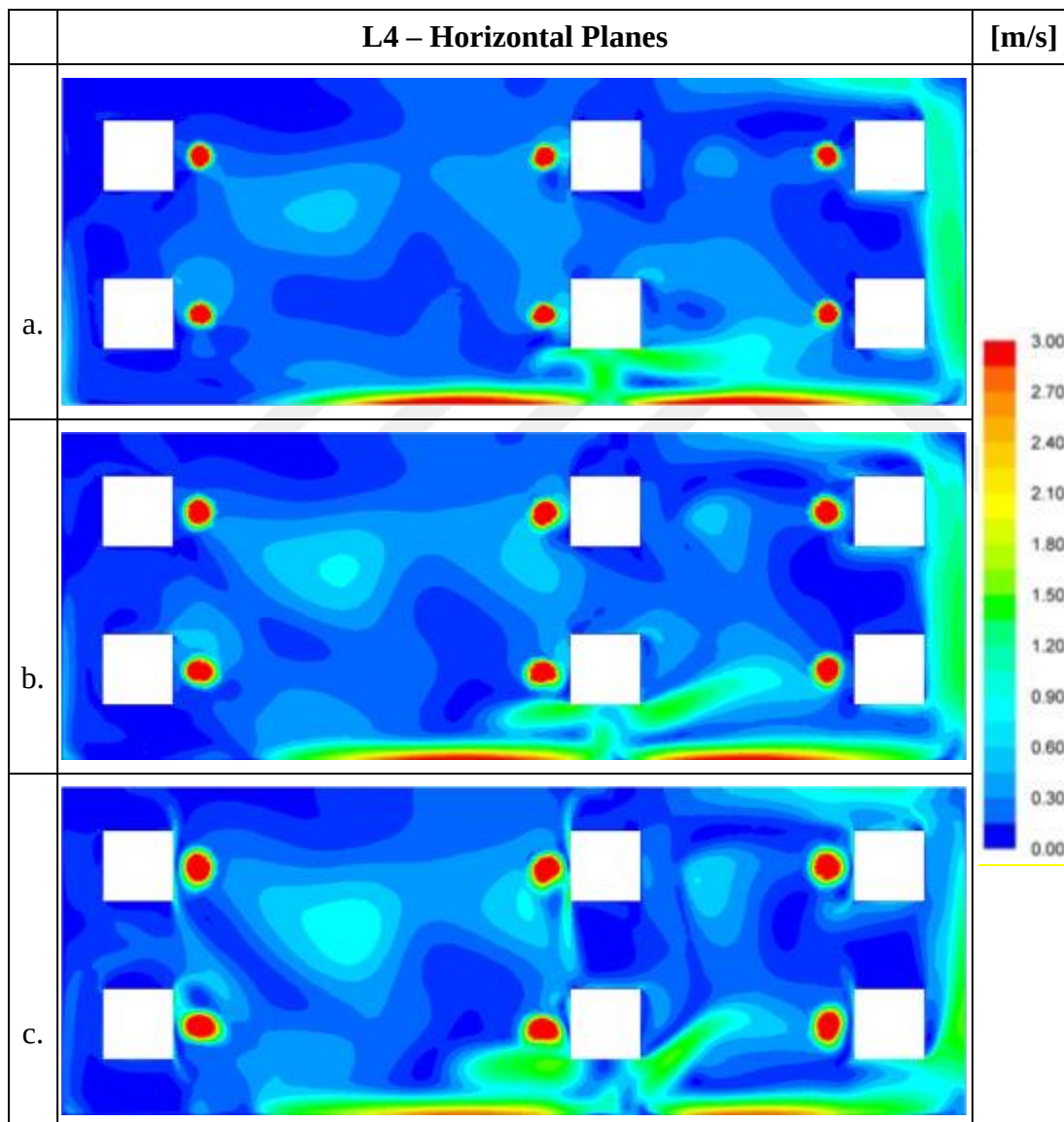
Figure 6-6 Velocity magnitude contours for L4 on the horizontal plane at; (a) z = 1196 \text{ mm} ; (b) z = 1121 \text{ mm} ; (c) z = 1046 \text{ mm}
