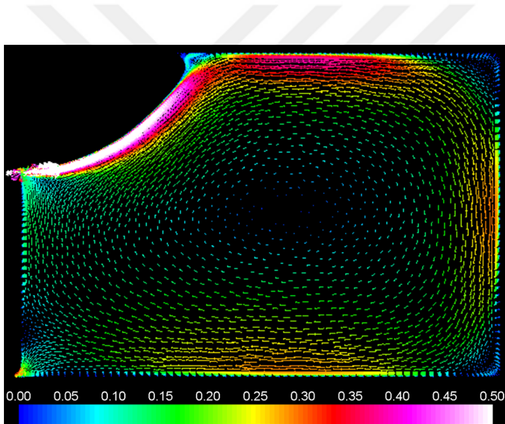
Figure 4-21 Velocity vector fields on symmetry plane predicted by standard k- \epsilon model of the present study
