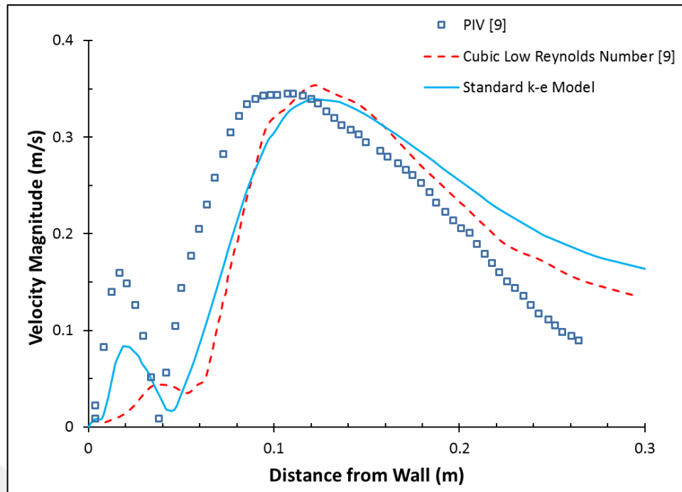
Figure 4-18 Velocity magnitude comparison on Line B – Standard k- \epsilon turbulence model with Günther et al.'s [9] experimental data and the best numerical result
