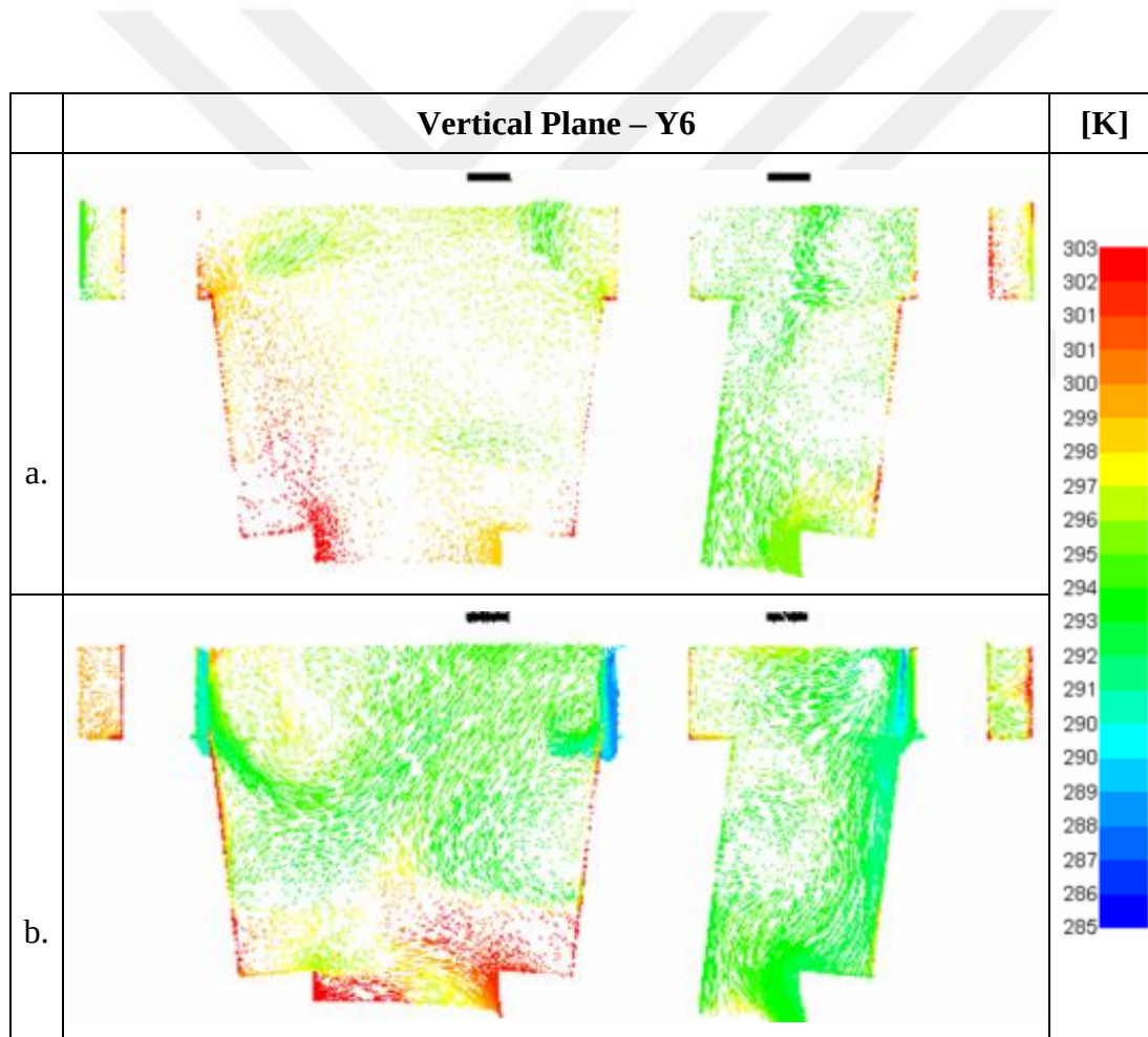
Figure 7-12 Velocity vector fields colored by temperature on Y6 plane for; (a) L0; (b) L9 (50-50)
