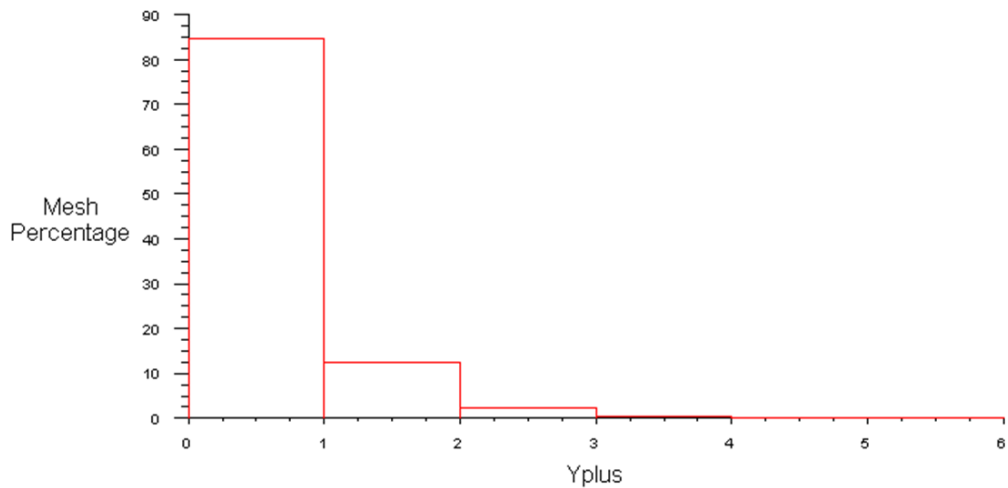
Figure 4-8 Y^+ histogram of the coarsest mesh of the mesh independence part of the turbulence model performance evaluation study
