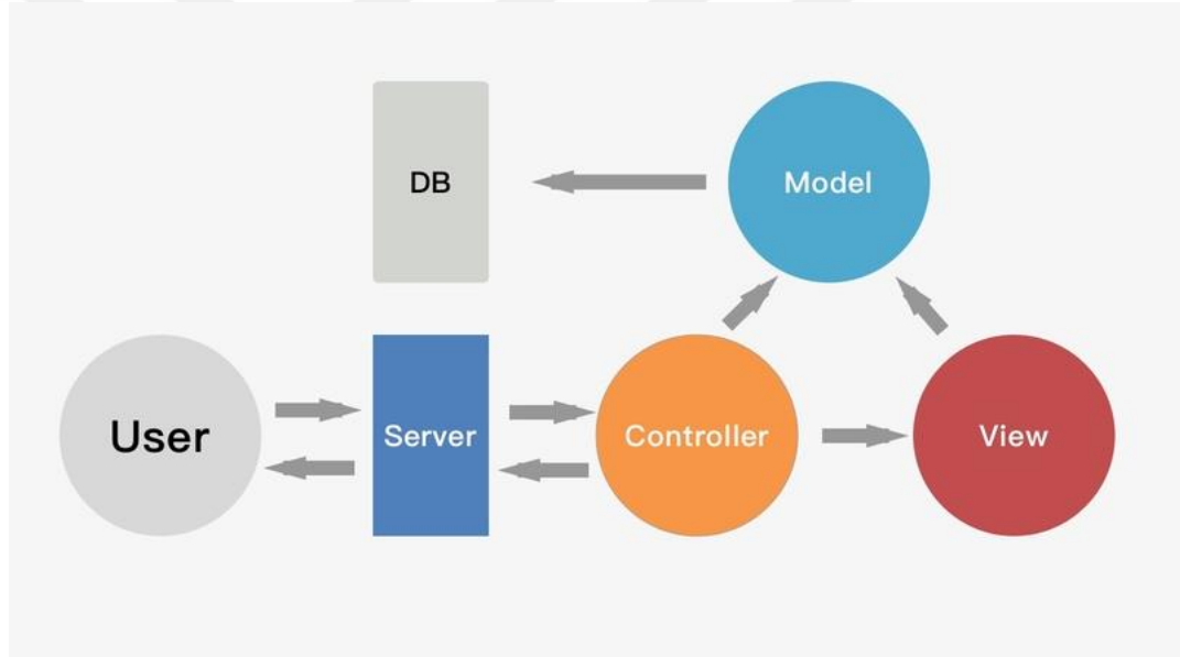
Şekil 3.3. APS.NET MVC mimarisi ( http://www.webdevelopmenthelp.net/2013/10/difference-between-asp-net-webform-and-asp-net-mvc.html ).
