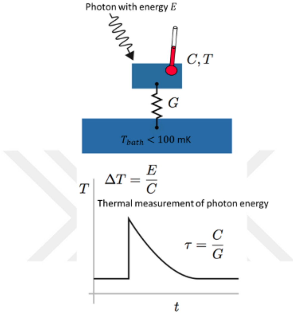
Figure 2.3: Transition Edge Sensor Schematic. [53]
