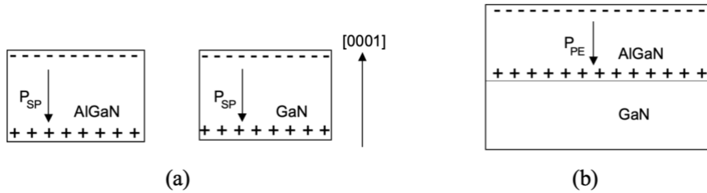
Figure 3.4: Electric field and sheet charges present (a) due to only spontaneous polarization in GaN and AlGaIn crystals; and (b) due to only piezoelectric polarization in a AlGaIn layer.
