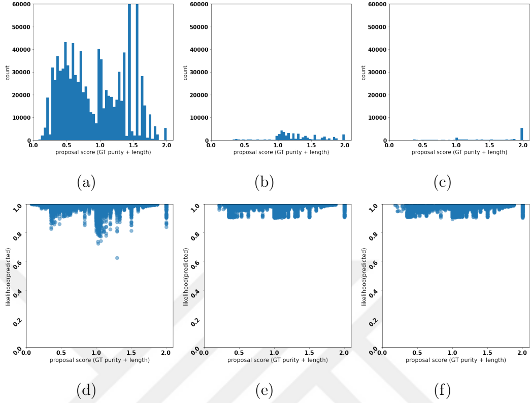
Figure 5.2: Investigating proposal quality distribution during (a): training, (b): inference and (c): when starting walks at nodes with out-degree > 1 . Showing correlation between proposal likelihoods and ground truth score during (d): training, (e): inference and (f): when starting walks at nodes with out-degree > 1 . All results are on sequences unseen when training. We show an enrichment in proposal quality by purging at the node level rather than thresholding at the proposal level.
