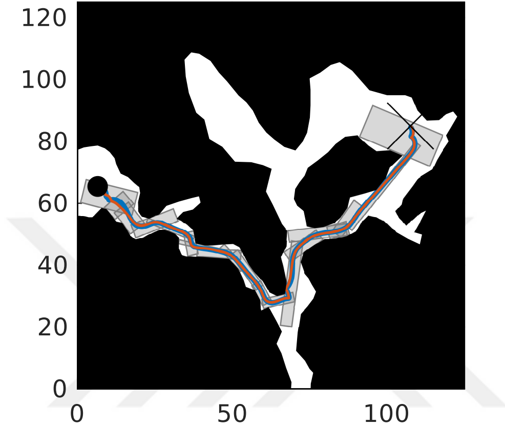
Figure 4.46: Heron USV position trajectory for Map 3. Orange curve is the nominal position trajectory and blue curve is the real position trajectory of Heron.
