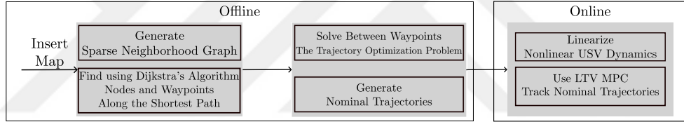
Figure 4.1: The Overall Algorithm
