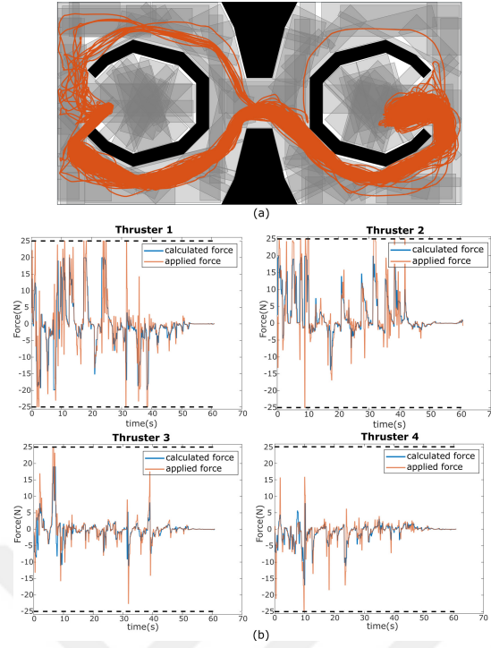
Figure 4.64: The Monte Carlo Experiment results presented in [6] for the fully actuated USV. (a) shows the successful trials that end up at the goal position. (b) shows the thruster commands for all four thrusters of the fully actuated USV. MPC-Graph shows 98% success during the trials with the fully actuated USV.
