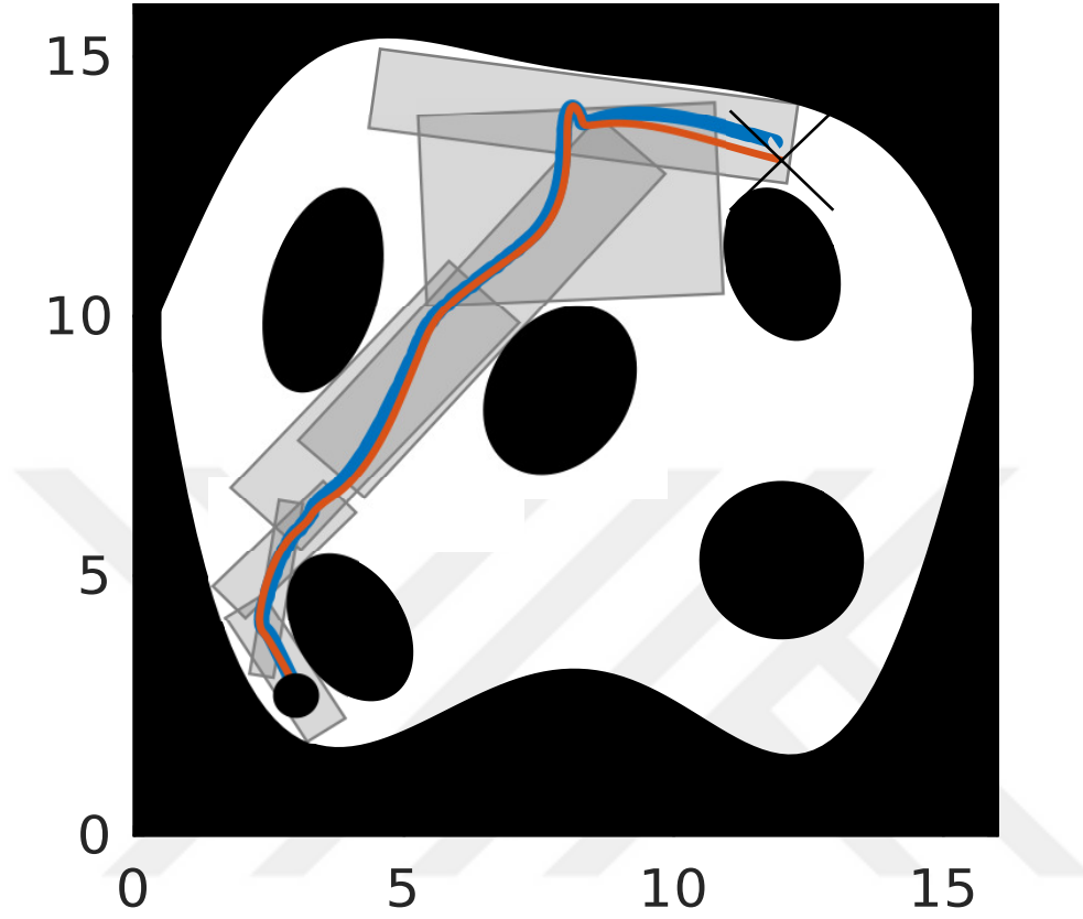
Figure 4.56: Heron USV position trajectory for Map 4. Orange curve is the nominal position trajectory and blue curve is the real position trajectory of Heron.
