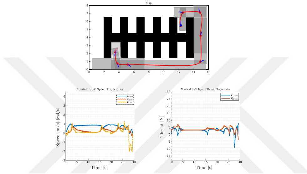
Figure 4.22: Nominal trajectories for the Monte Carlo experiments.
