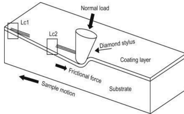
Figure 3 11. Diagram illustrating the workpiece being scratched by an indenter.
