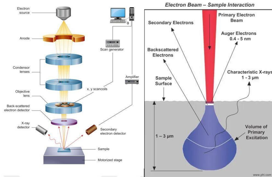
Figure 3.8. a. SEM, EDS device b. Interaction area of an incident beam.
