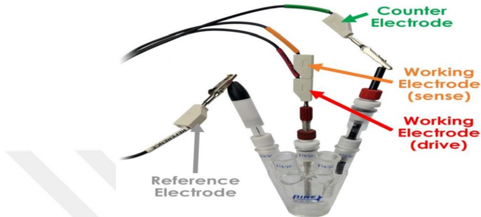
Figure 3 13. Corrosion cell
