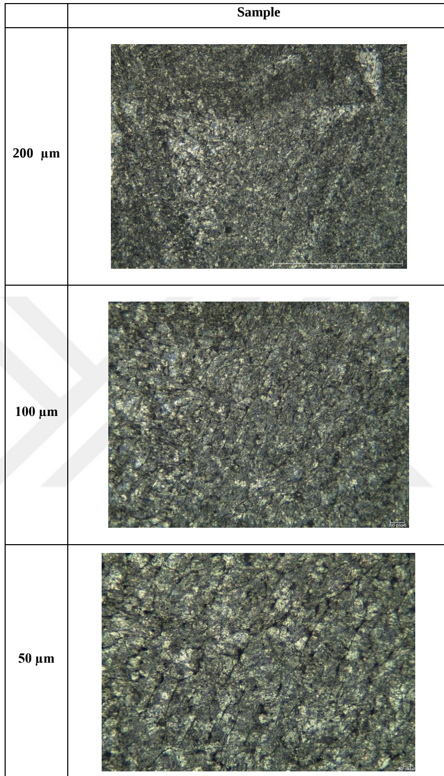
Figure 5.1 ASTM 1008 steel images by optical microscopy
