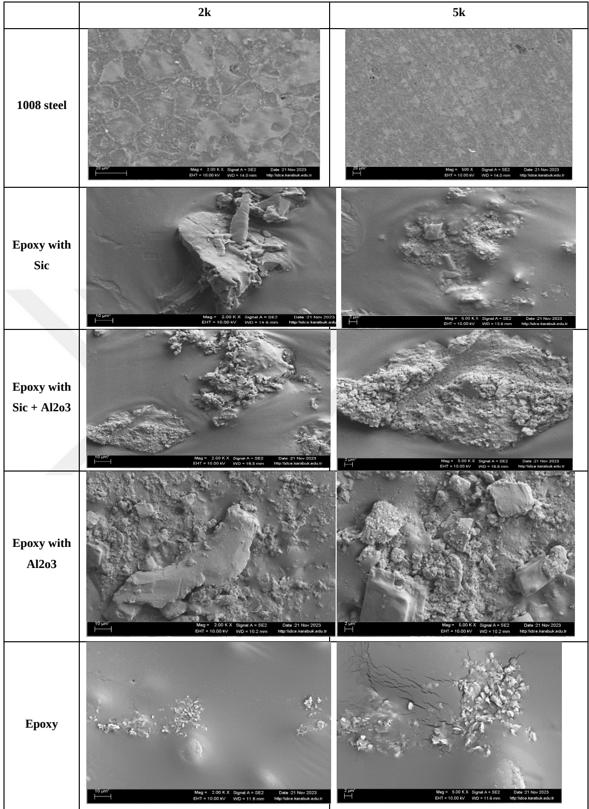
Figure 5 2. SEM images of samples
