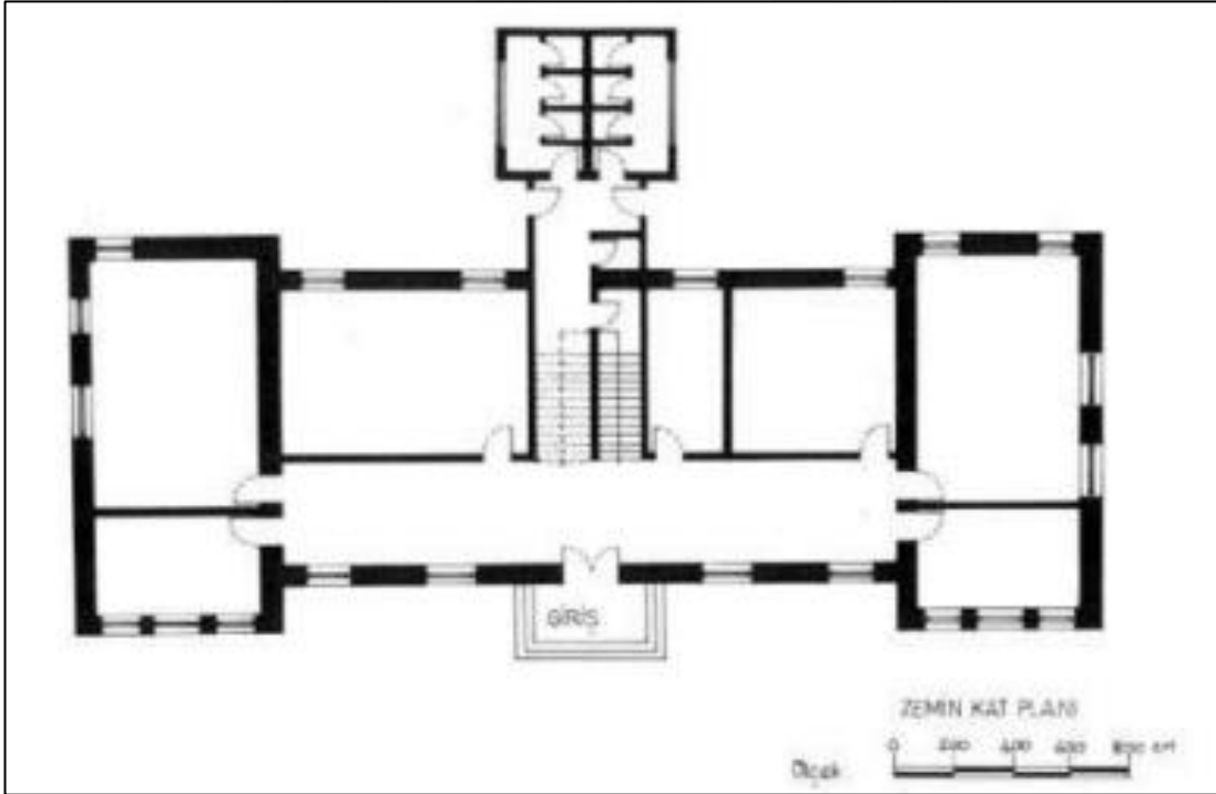
Plan 4.5. Kayseri Gazipaşa İlkokulu
