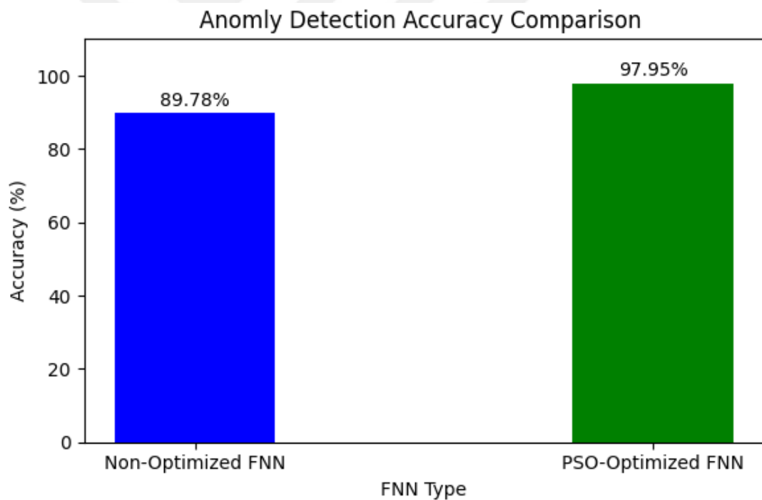
Figure 5.7. Anomaly Detection Performance (Accuracy) Comparison.
