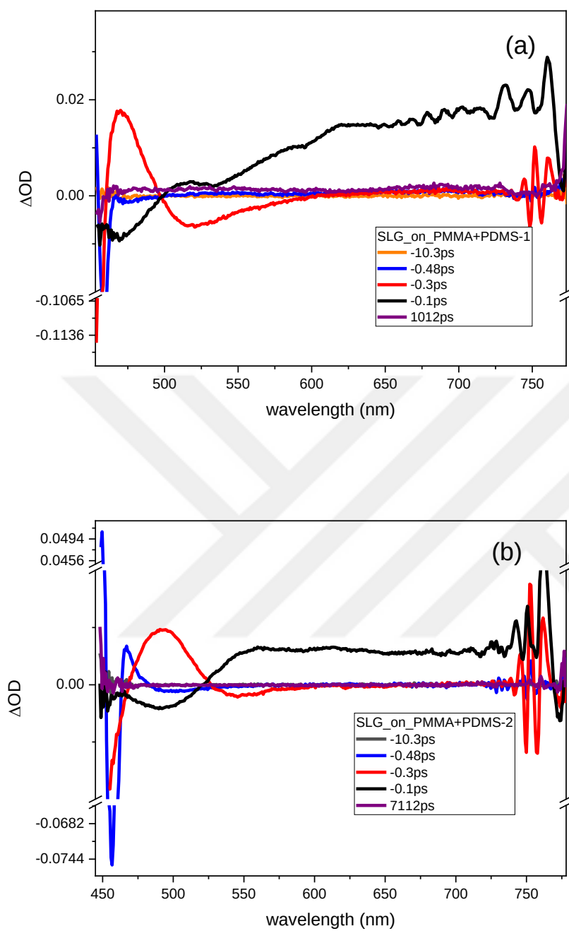
Figure 7.11. (a), (b) Transient spectra in the visible range for different time scales for SLG on PMMA+PDMS of sample-1 and 2 respectively.
