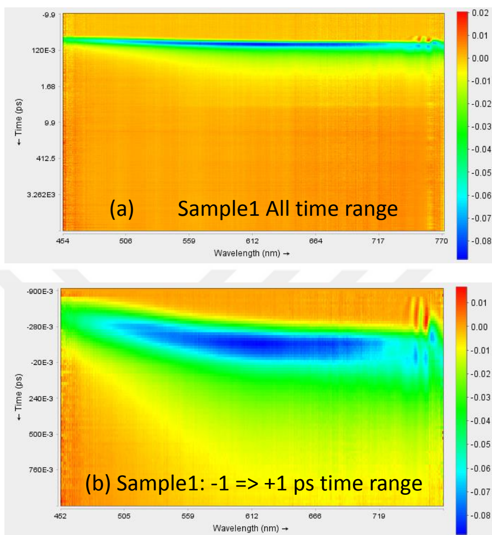
Figure 7.27. (a), (b) TAS contour plot spectrum of 400 nm excited MLG950 sample-1 at visible (white) probe wavelengths in 7ns and 2ps timespan respectively
