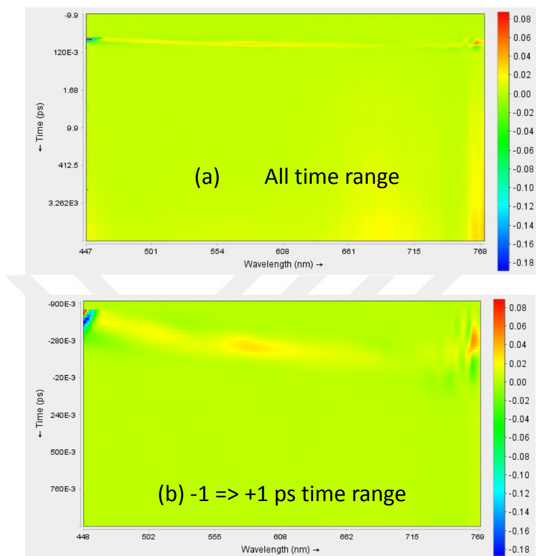
Figure 7.3. (a) and (b) TAS contour plot spectrum of 400 nm excited SLG on PDMS at visible (white) probe wavelengths in \sim 7 ns and 2 ps timespan respectively
