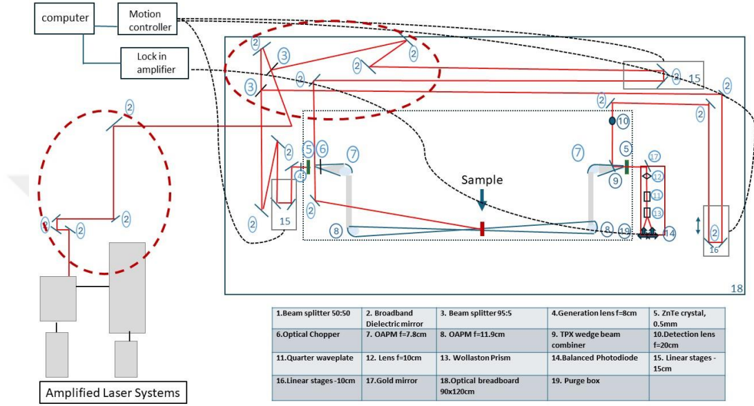
Figure 4.6. TRTS system with the adapted modifications to the laser lab in the TARLA facility
