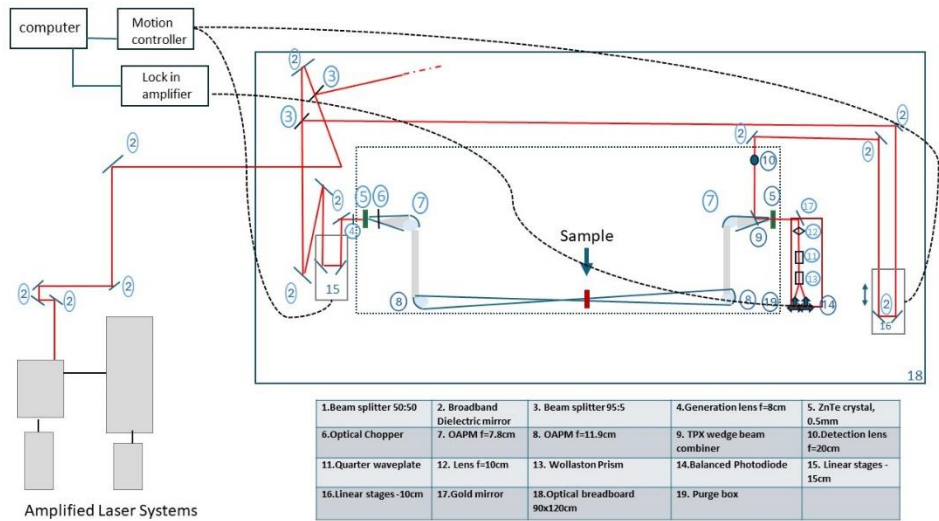
Figure 3.1. THz-TDS setup in TARLA
