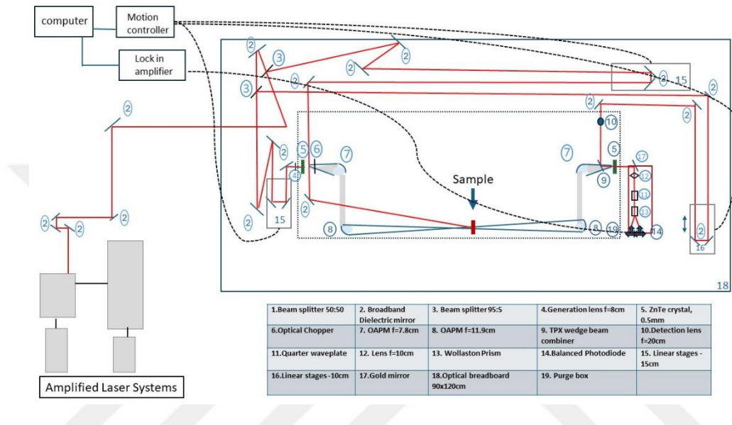
Figure 4.9. TRTS system with the adapted modifications to the laser lab in the TARLA facility
