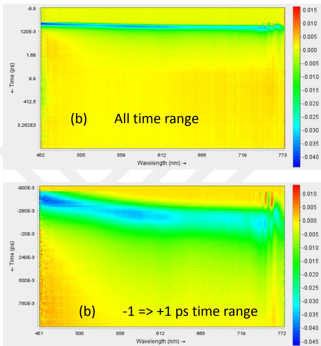
Figure 7.21. (a) and (b) TAS contour plot of 400 nm excited MLG900 sample at visible (white) probe wavelengths in \sim 7 ns and 2 ps timespan respectively
