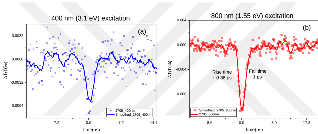
Figure 7.41 Differential THz transmission, \Delta T/T_0 , of Sample 2705 as a function of pump-probe delay recorded a) at a fluence of 195 \mu\text{J}/\text{cm}^2 for 400nm excitation and b) at a fluence of 255 \mu\text{J}/\text{cm}^2 for 800nm excitation.
