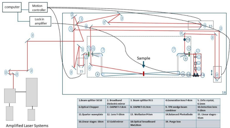
Figure 3.2. TRTS setup in TARLA
