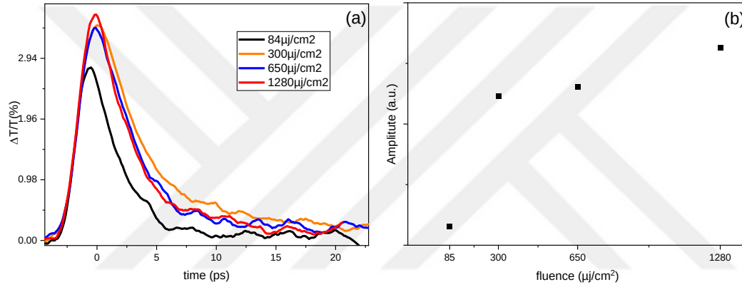
Figure 7.1 (a) Differential THz peak transmission response of SLG sample on Si/SiO 2 at pump fluences of 84, 300, 650, and 1280 \mu\text{j}/\text{cm}^2 (b) peak amplitude vs fluence showing saturation after 300 \mu\text{j}/\text{cm}^2
