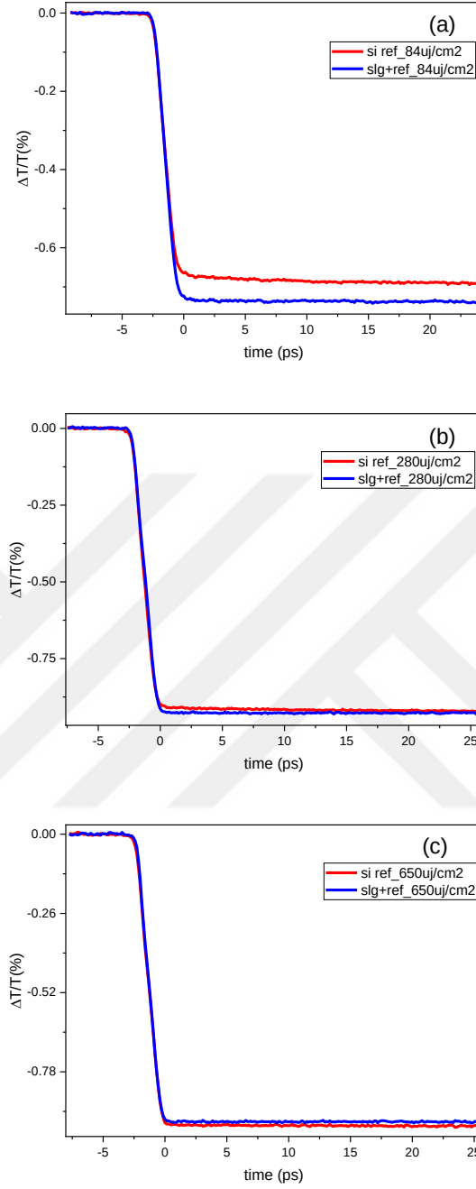
Figure 5.9. Differential THz peak transmission response, \Delta T/T_0 , of Si/SiO 2 as reference and SLG on Si/SiO 2 as a function of pump–probe delay recorded at pump fluences of a) 84 \mu\text{J}/\text{cm}^2 , b) 280 \mu\text{J}/\text{cm}^2 , and c) 650 \mu\text{J}/\text{cm}^2 .
