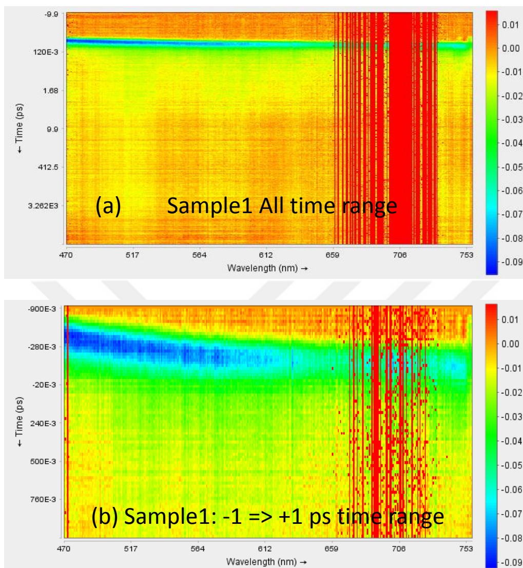
Figure 7.35. (a), (b) TAS contour plot spectrum of 400 nm excited MLG1000 sample-1 at visible (white) probe wavelengths in 7ns and 2ps timespan respectively
