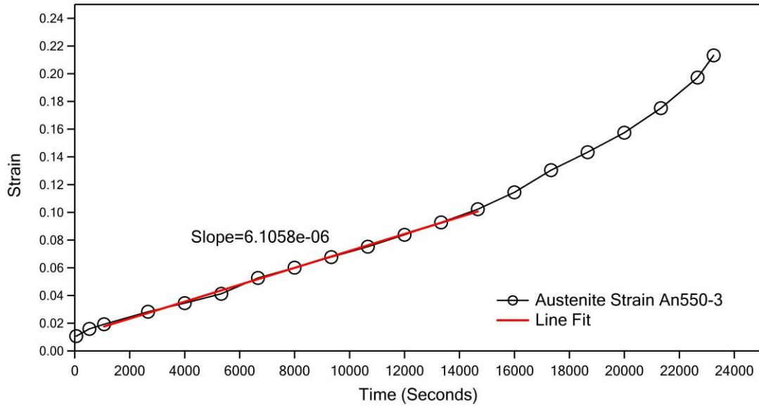
Figure 4.41. Austenite Strain data from An550-3 Sample 3 Functional Fatigue Experiments
