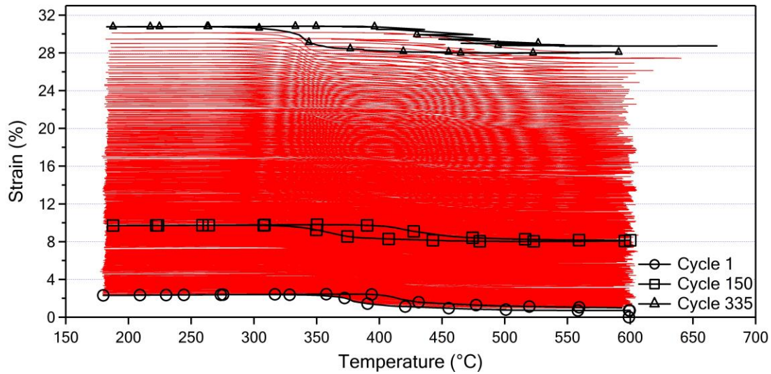
Figure 4.19. Functional fatigue experiment results of GG800-10 Sample
