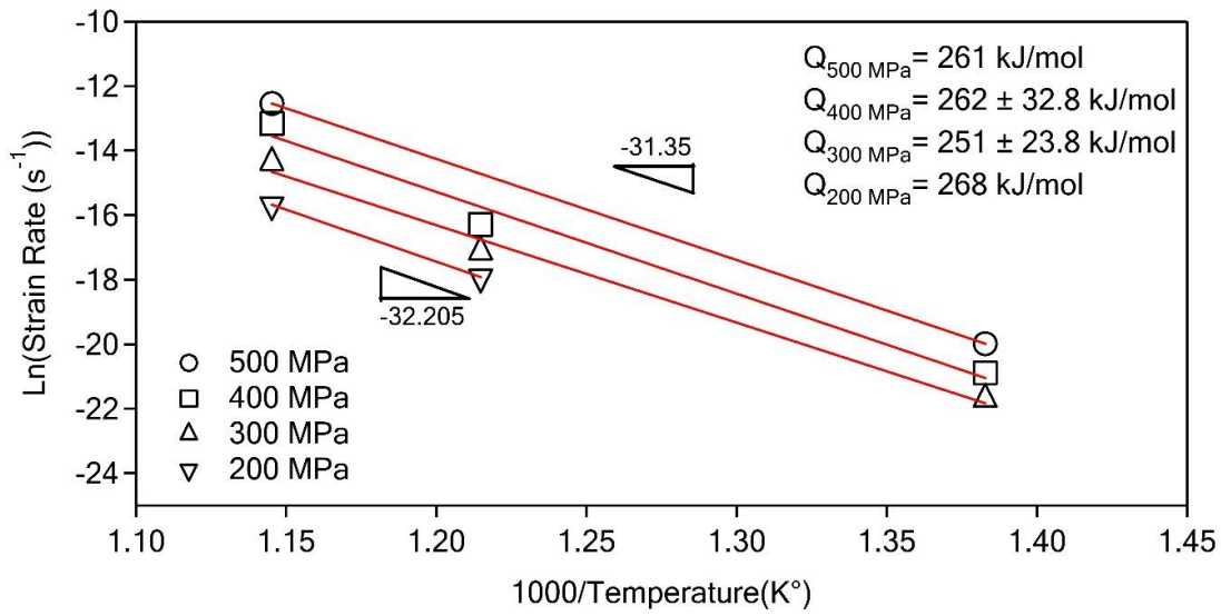
Figure 4.35. Natural logarithm of Strain Rate vs 1000/\text{Temperature} plot for An550-3 samples.
