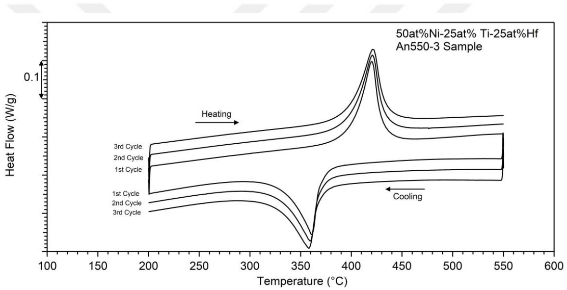
Figure 4.2. DSC results of An550-3 sample [68].
