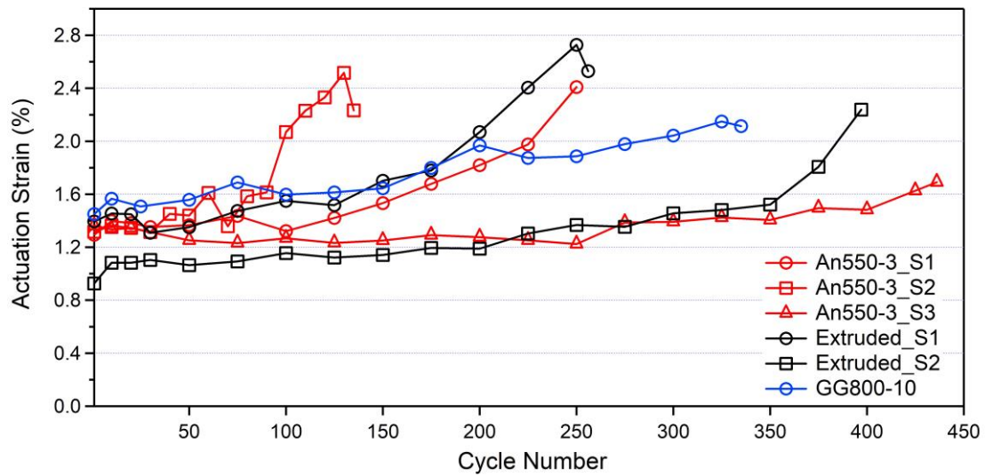
Figure 4.20. Actuation Strain of all samples which were thermally cycled throughout the functional fatigue experiments
