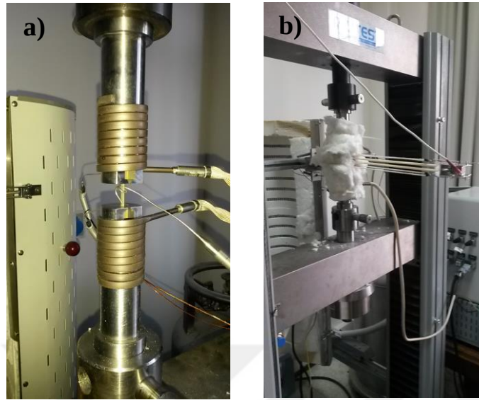
Figure 3.6. Utest Mechanical Testing Equipment with custom made heating system a) heaters attached to grips b) during experiment
