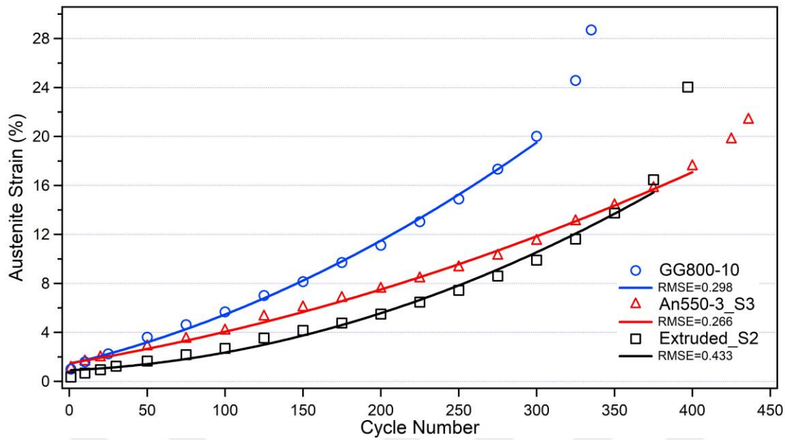
Figure 4.23. Austenite Strain comparison for selected samples
