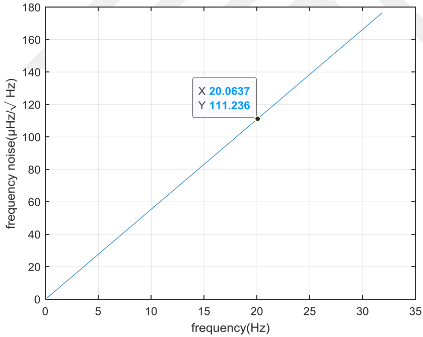
Figure 5.15. Frequency noise result of the first mode of the FM gyroscope. 111μHz/√Hz at 20Hz frequency split.
