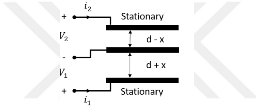
Figure 2.4. Varying gap capacitor.
