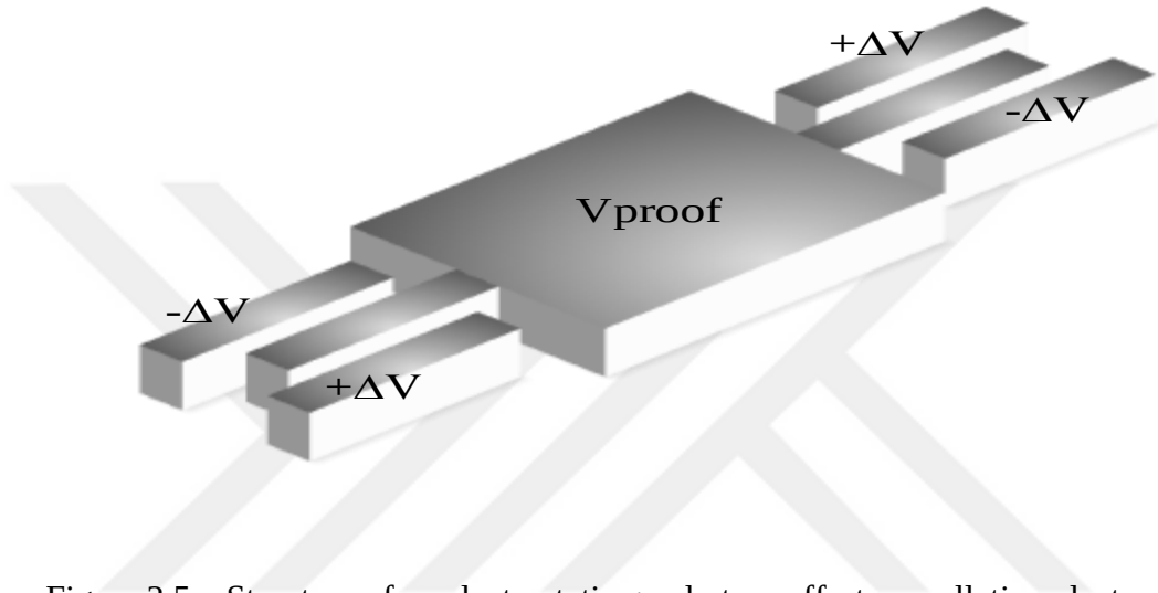
Figure 2.5. Structure of an electrostatic quadrature offset cancellation electrode.
