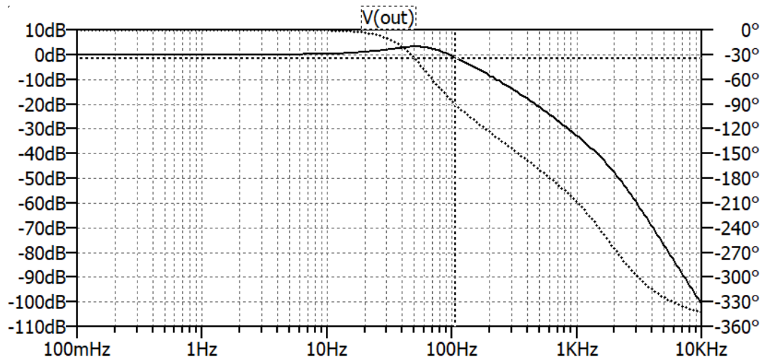
Figure 5.12. The closed loop transfer function of the designed PLL control loop. 90° phase shift bandwidth: 104Hz, -3dB bandwidth: 125Hz.
