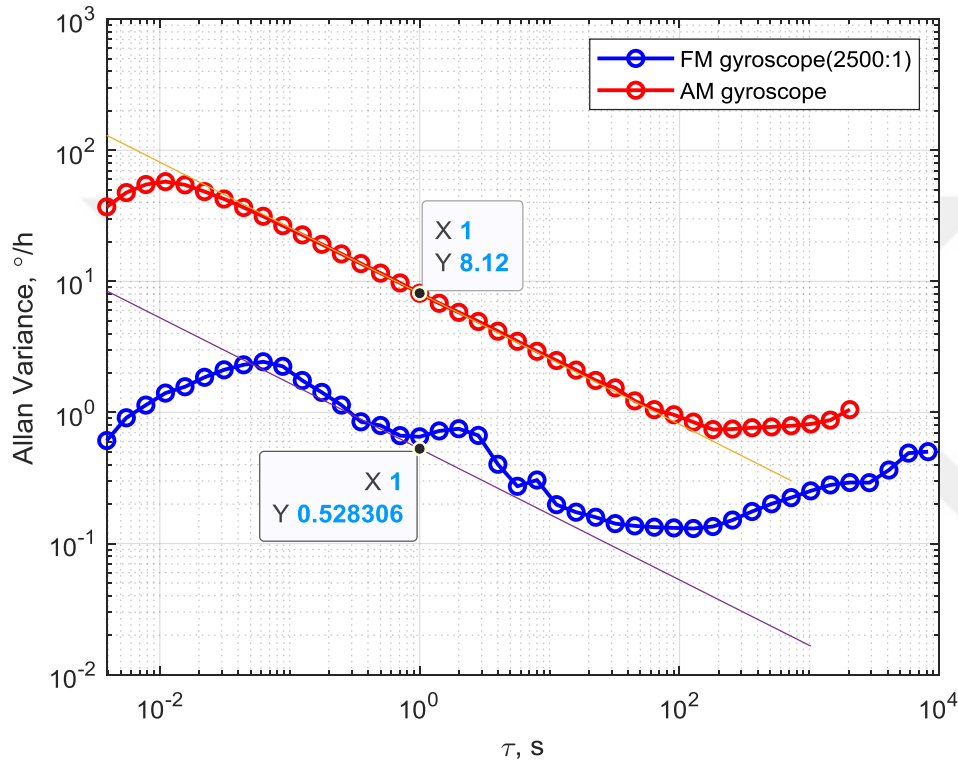
Figure 5.31. The comparison of the digitally operated FM and AM gyroscopes. ARW of FM: 0.52^\circ/\text{hr}/\sqrt{\text{Hz}} , ARW of AM: 8.12^\circ/\text{hr}/\sqrt{\text{Hz}} .
