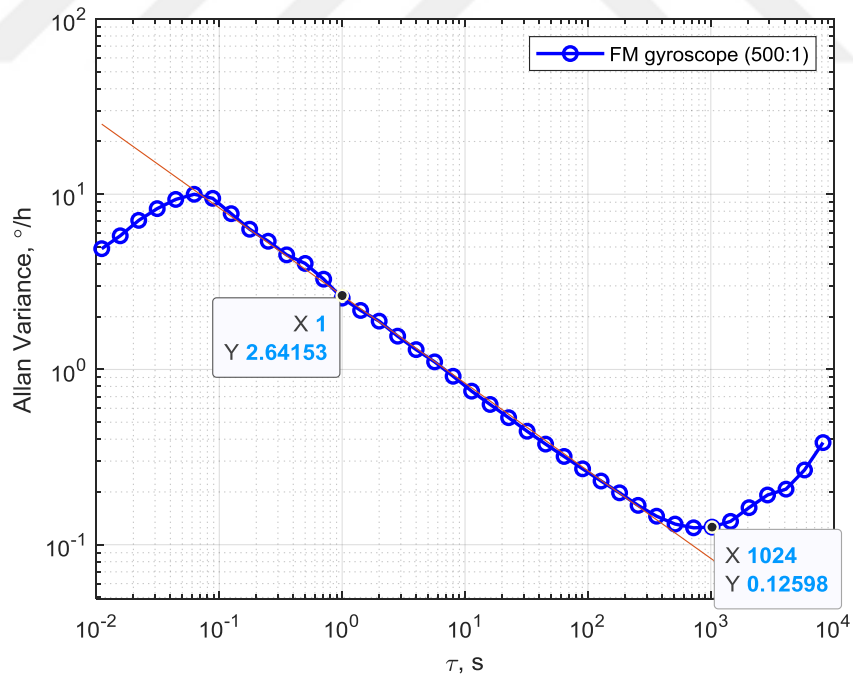
Figure 5.27. Allan Variance Analysis result for FM gyroscope operated with 500:1 amplitude ratio. ARW: 2.6^\circ/\text{hr}/\sqrt{\text{Hz}} , BI: 0.13^\circ/\text{hr} .
