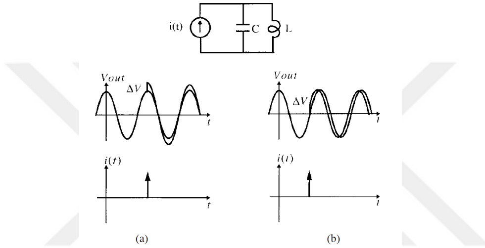
Figure 4.5. Time variant impulse effect on oscillator (a) Impulse injected at the peak, (b) impulse injected at the zero crossing [25].
