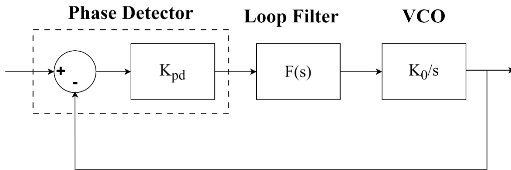
Figure 5.2. Block diagram of a linear PLL.
