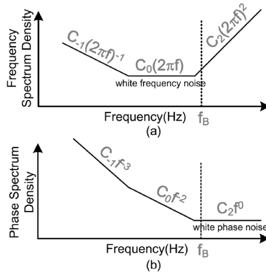
Figure 4.4. Frequency noise density of FM gyroscope's oscillator.
