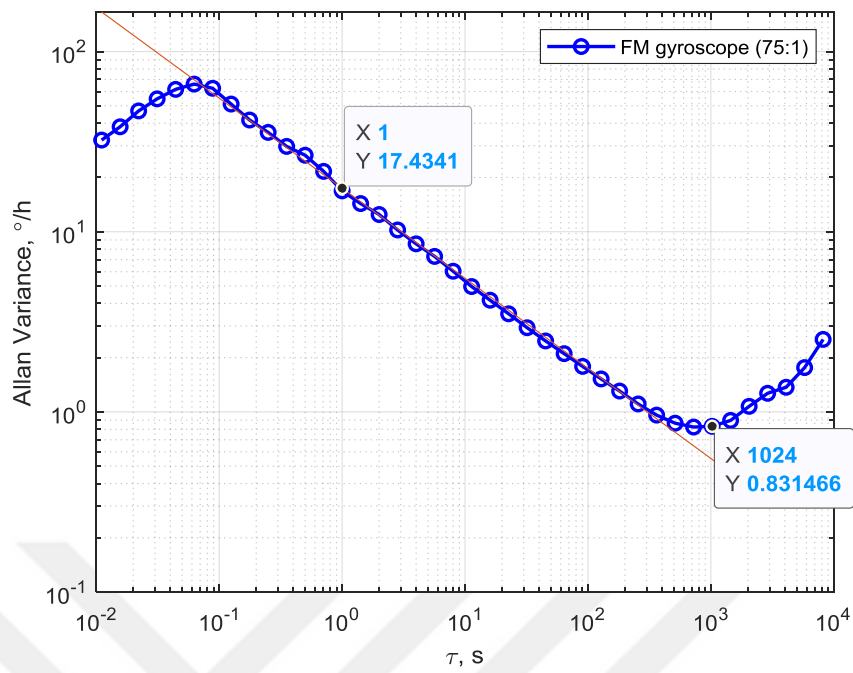
Figure 5.26. Allan Variance Analysis result for FM gyroscope operated with 75:1 amplitude ratio. ARW: 17.4^\circ/\text{hr}/\sqrt{\text{Hz}} , BI: 0.83^\circ/\text{hr} .
