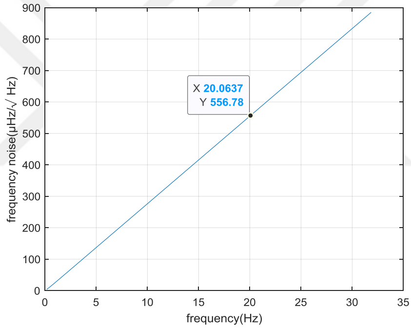
Figure 5.16. Frequency noise result of the second mode of the FM gyroscope. 556μHz/√Hz at 20Hz frequency split.
