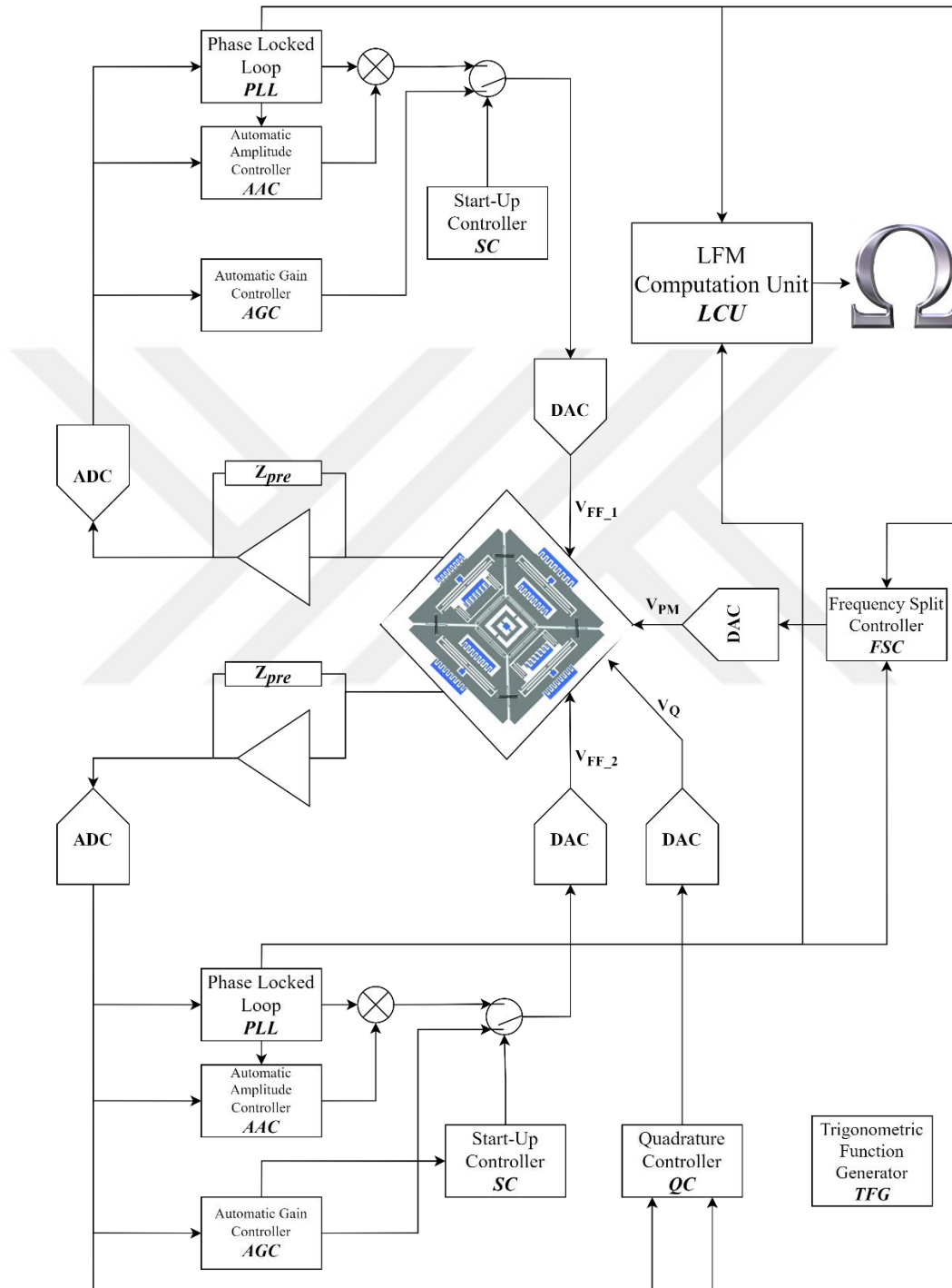
Figure 5.1. The block diagram of the digitally controlled FM gyroscope.
