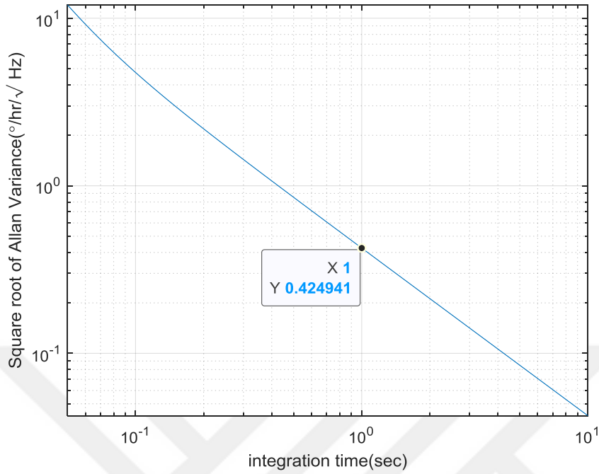
Figure 5.18. The Allan Variance analysis obtained from rate noise spectrum. ARW: 0.42^\circ/\text{hr}/\sqrt{\text{Hz}} .
