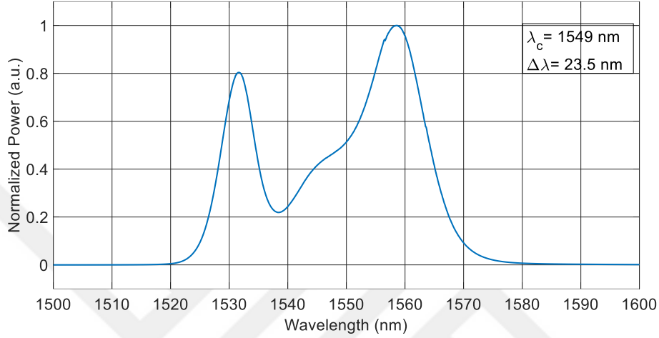
Optical Spectrum of 10m Er-fiber ASE Light Source with Coreless Fiber Termination
