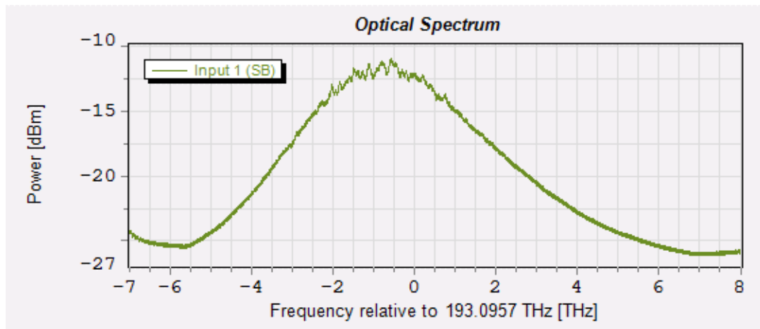
Figure 3.7. Optical spectrum of SLD with VPI-photonics
