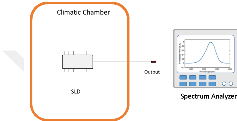
Figure 3.30. Temperature characterization setup of SLD
