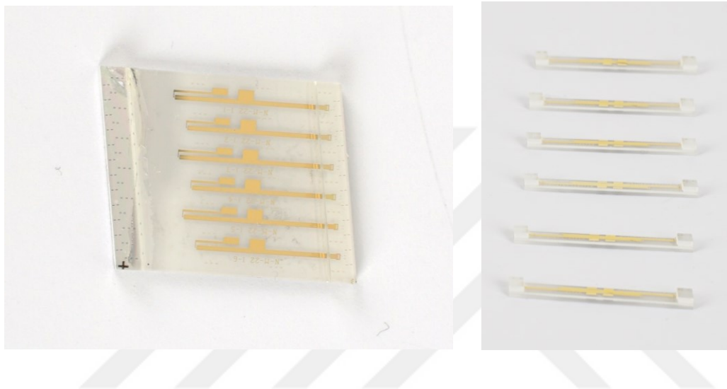
Figure 3.58. A diced LiNbO 3 wafer piece for lapping and polishing process
