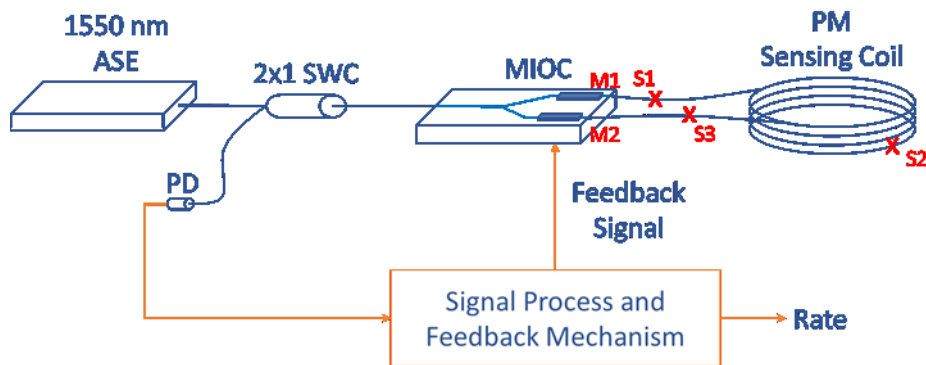
Figure 4.1. Optical configuration of ISP-IFOG
