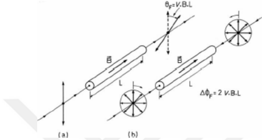
Figure 2.7. Faraday effect of a piece of fiber: (a) rotation of linear polarity and (b) phase difference between two opposing circular polarities
