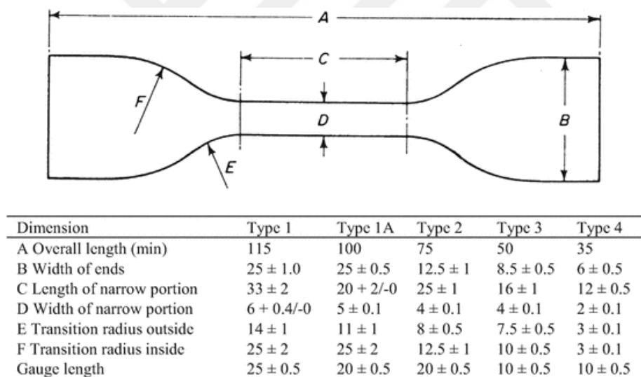
Figure 3.68. ISO-37 specimen geometry
