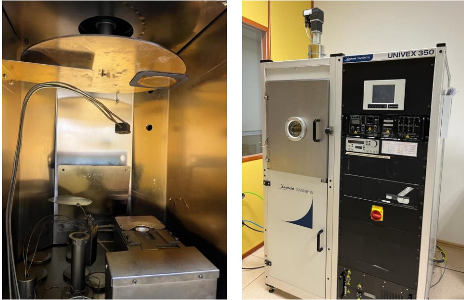
Figure 3.44. PVD system
