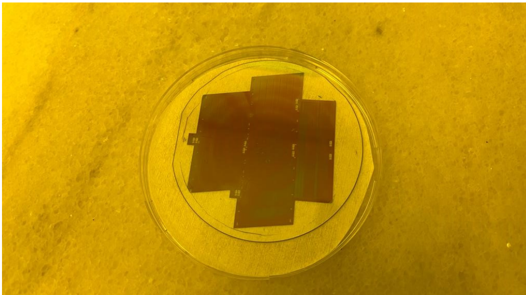
Figure 3.55. \text{LiNbO}_3 wafer after proton exchange
