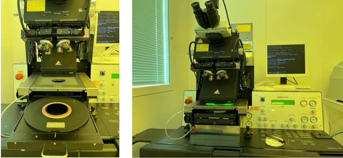
Figure 3.46. Mask aligner and photolithography system (Karl Suss MA6)
