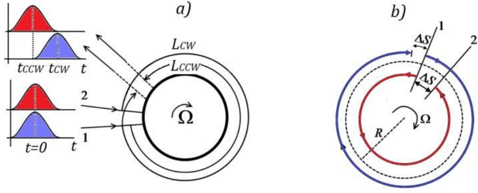
Figure 2.1. In a disk rotating with a CW angular velocity (a) different rotation induced optical paths of the clockwise and counter-clockwise CCW optical beams, L_{CW} and L_{CCW} , respectively; and (b) identical difference, \Delta S , between the rotation induced optical paths of the clockwise and counter-clockwise optical beam, and the standing optical path
