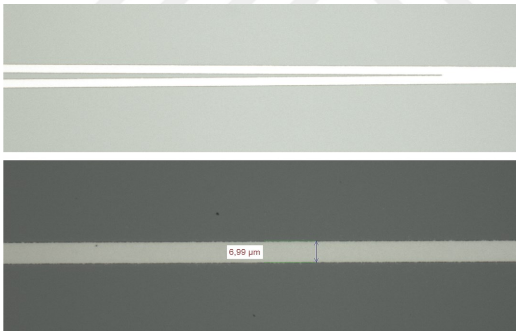
Figure 3.49. Microscope image of waveguides patterned with Ti-metals (a) y-coupler region (b) 7 um waveguide
