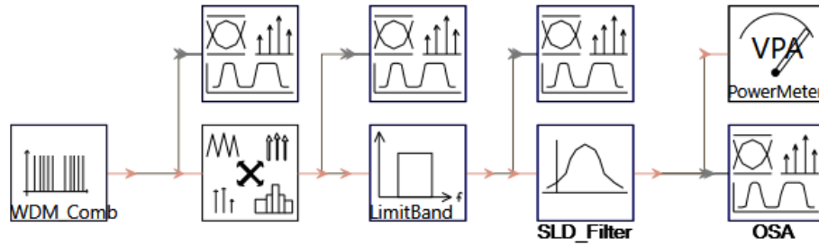
Figure 3.6. Schematic diagram of SLD with VPI-photonics
