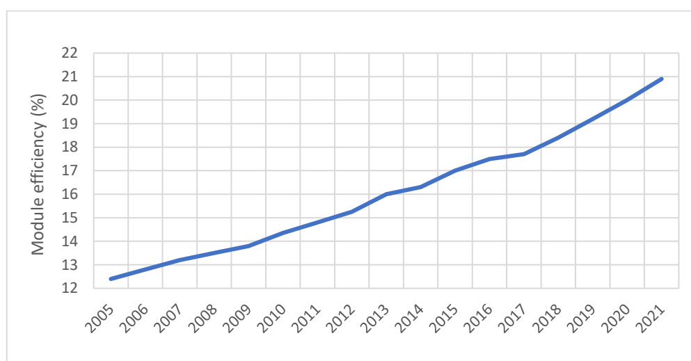
Figure 2.5. The evolution of industrial c-Si module efficiencies
