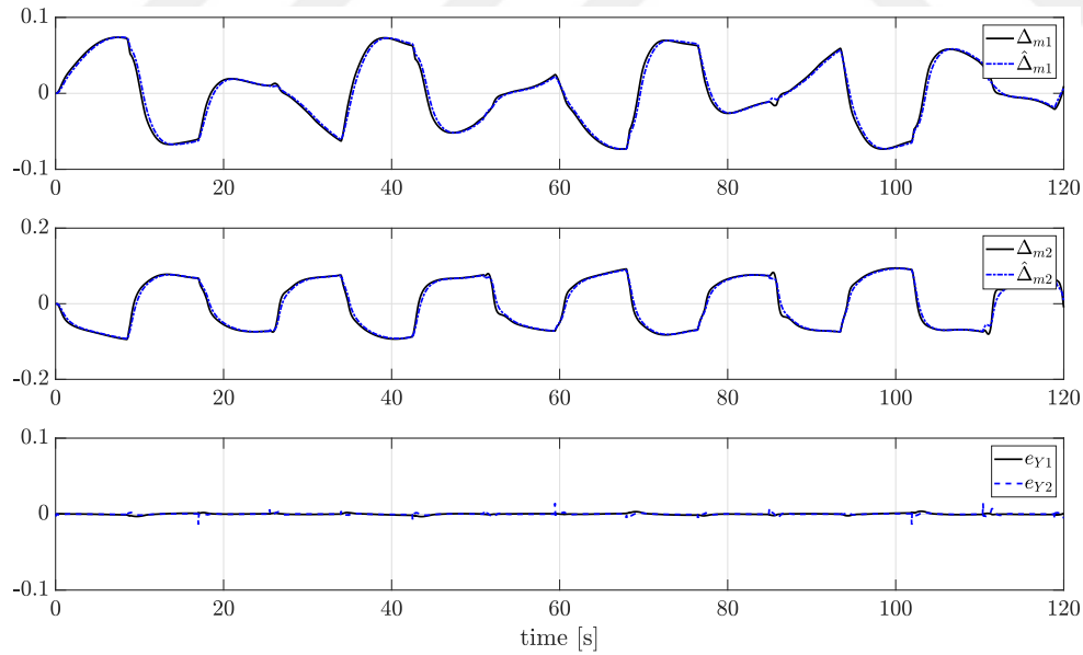
Figure 7.7: Matched Uncertainty Estimation for the CMRAC
