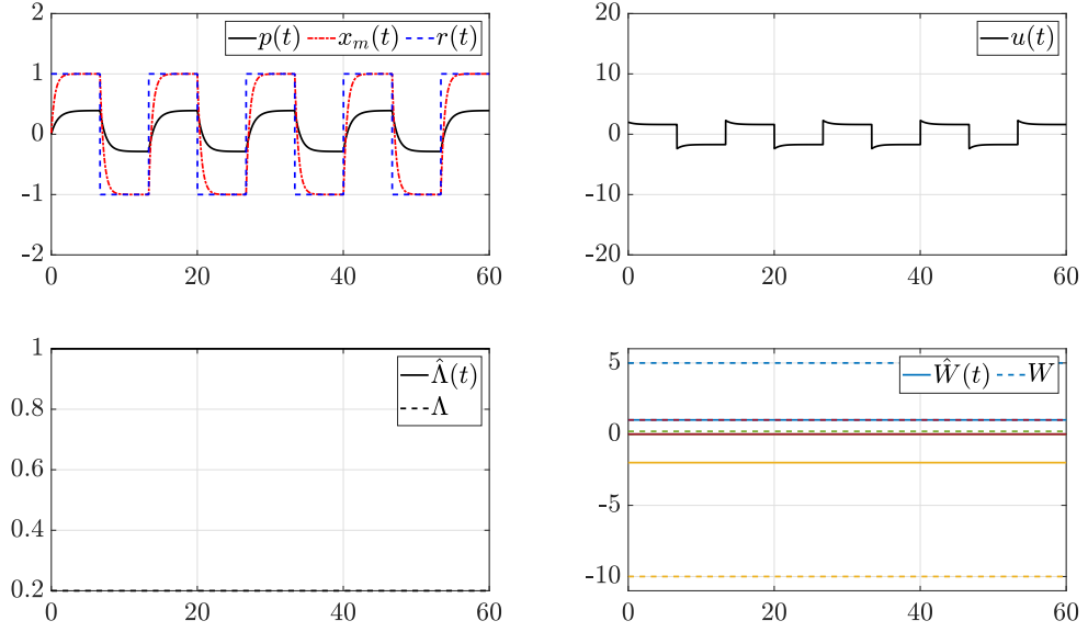
Figure 4.1: Example 1: Response of Nominal Controller in Eq 2.4
