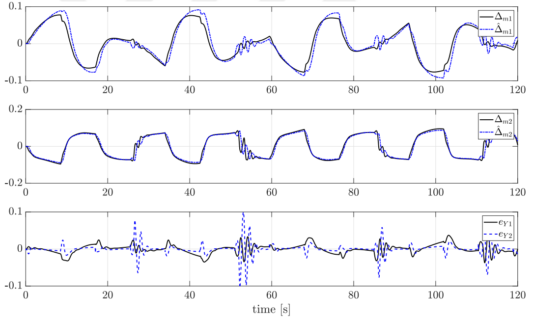
Figure 7.5: Matched Uncertainty Estimation for the Standard MRAC
