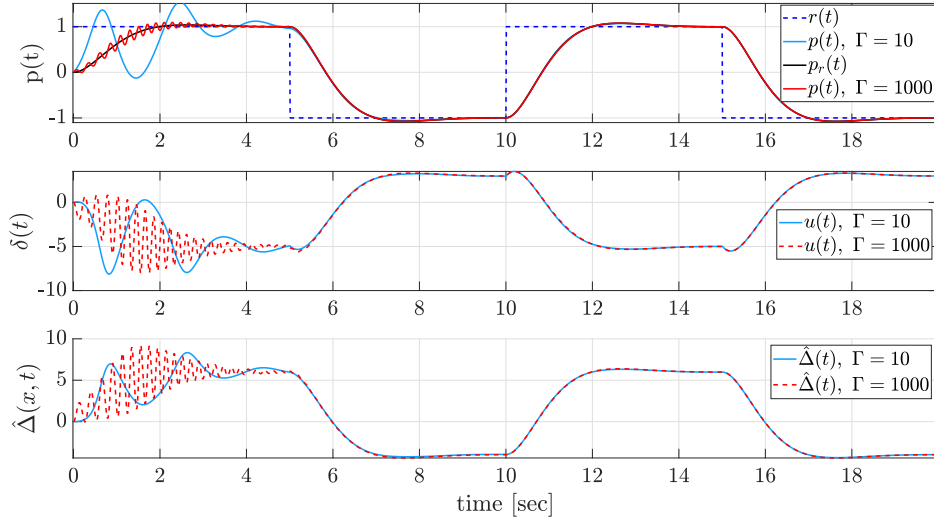
Figure 4.7: Example 2: Performance Comparison for Standard MRAC
