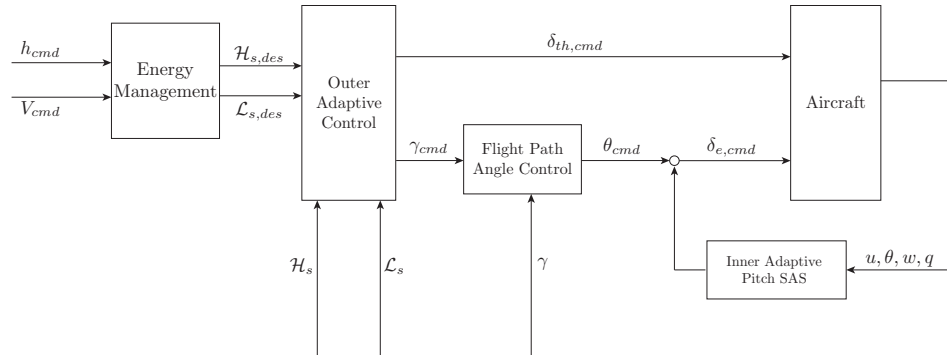
Figure 6.1: Block Diagram of the Proposed Longitudinal Flight Control Algorithm
