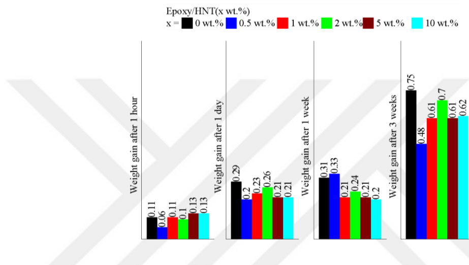
Figure S3.5 Bar graphs for the amount of water absorbed by H0, H1, H2, H3, H5, and H10 after 1 hour, 1 day, 1 week and 3 weeks.
