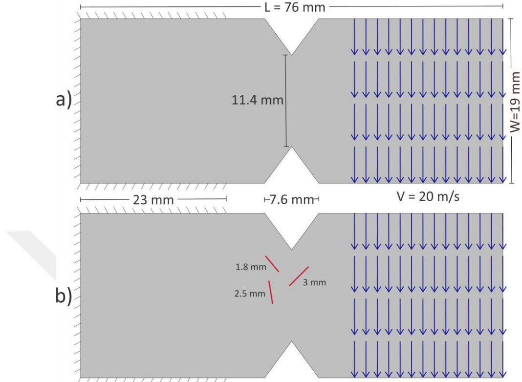
Figure 4.18 Geometric properties of the v-notched plate and its loading condition, (a) without cracks, (b) with three randomly generated microcracks.
