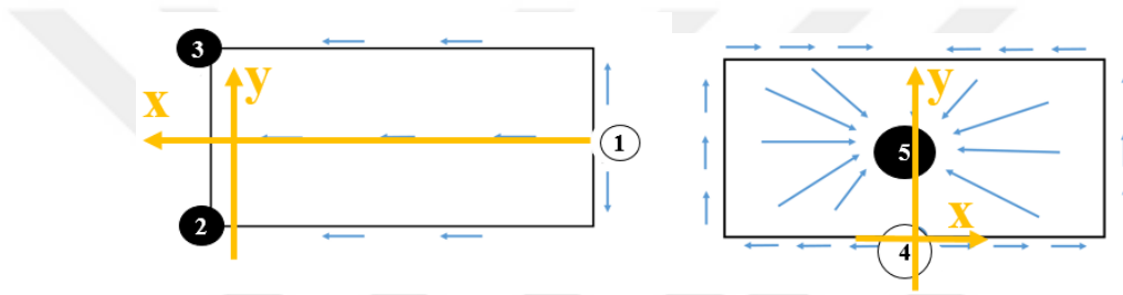
Figure S5.1 Scheme of RTM(I) and RTM(II) composite plates showing the assigned x, y axes.
