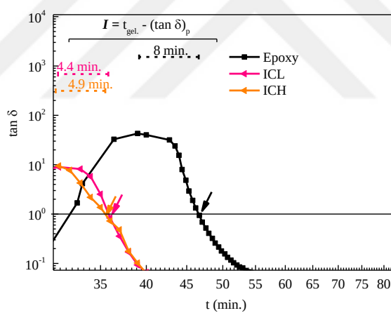
Figure S3.7 \tan \delta vs. t during complex viscosity measurements for H0, ICL, and ICH.
