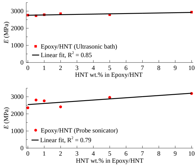
Figure 3.3 flexural muduls for three-point bending tests for H0, H0.5, H1, H2, H5, and H10 nanocomposites that are prepared either by (a) ultrasonic bath, and (b) by probe sonicator with the linear fit and R^2 value.
