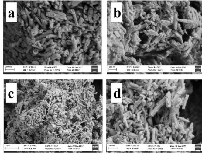
Figure S3.4 SEM micrographs of a) HNTs and b) mHNTs.
