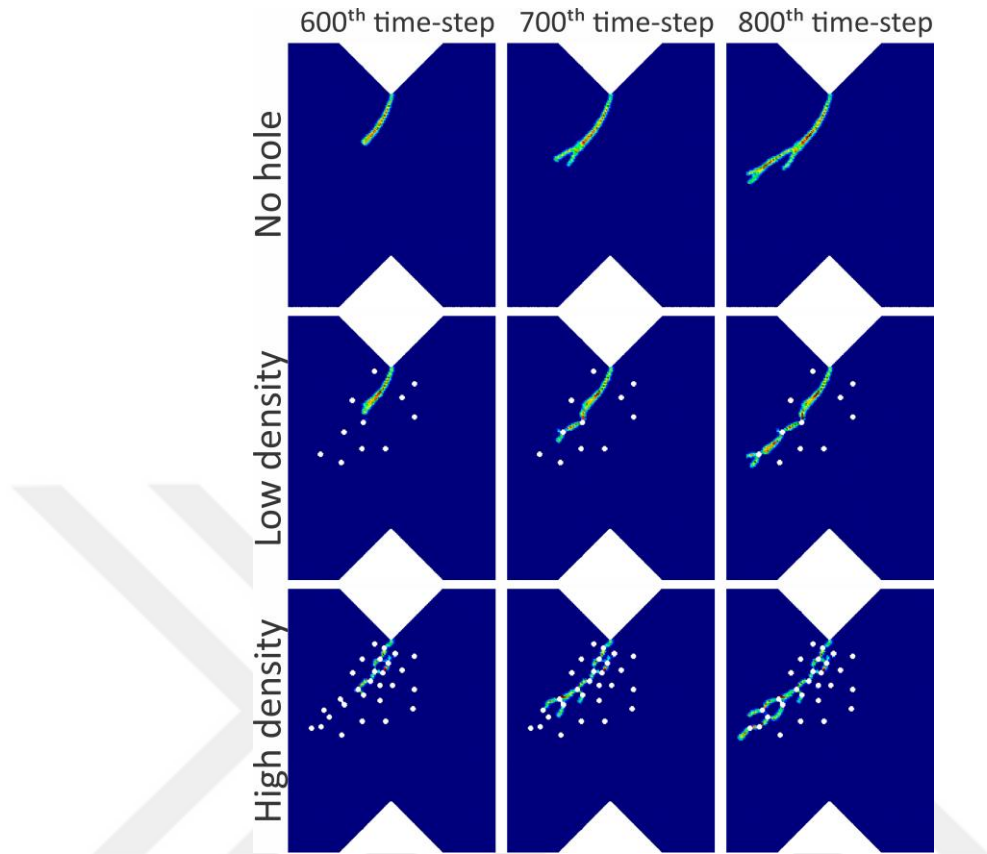
Figure 4.19 Propagation of the cracks after 600 th , 700 th , and 800 th time-steps at the central portion of plates with zero, low and high density of randomly generated holes.
