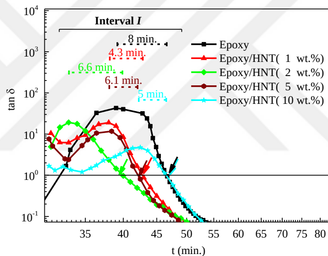
Figure 2.8 \tan \delta for epoxy/HNT(0, 1, 2, 5, and 10 wt.%) with I intervals indicated by horizontal dashed lines, and t_{gel} indicated by arrows at the intersection of each graph with the horizontal line at \tan \delta = 1 .
